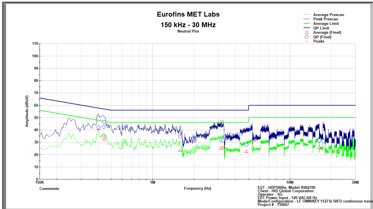
Conducted Emissions, Neutral, Test Results
