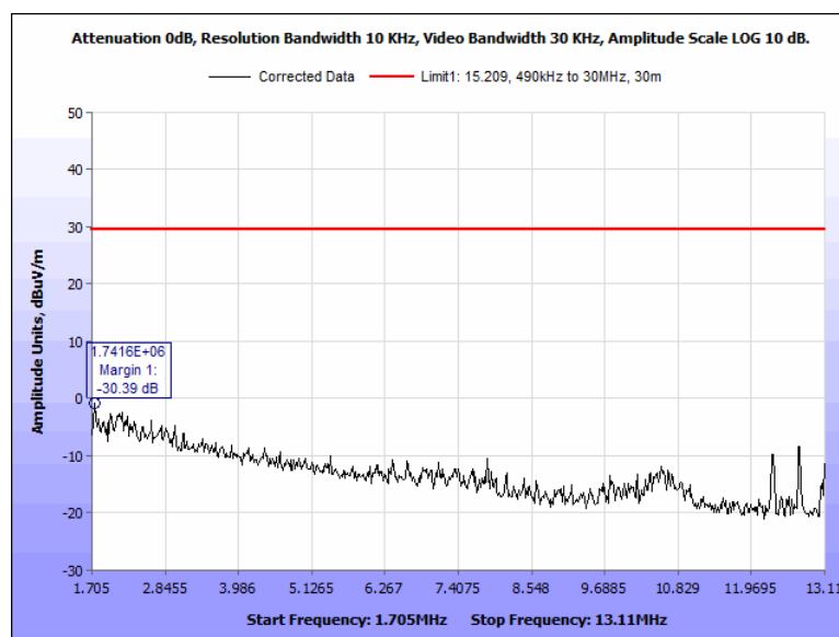
Figure 31. Spurious Emissions, Outside the Bands, 13.110 - 14. 010 MHz, 1.705 – 13.110 MHz, 90 degrees
