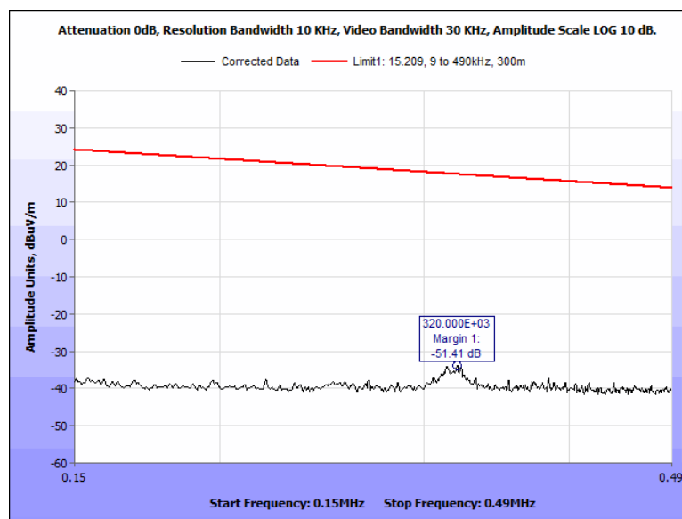
Figure 25. Spurious Emissions, Outside the Bands 13.110 - 14.010 MHz, 0.150 – 0.490 MHz, 90 degrees
