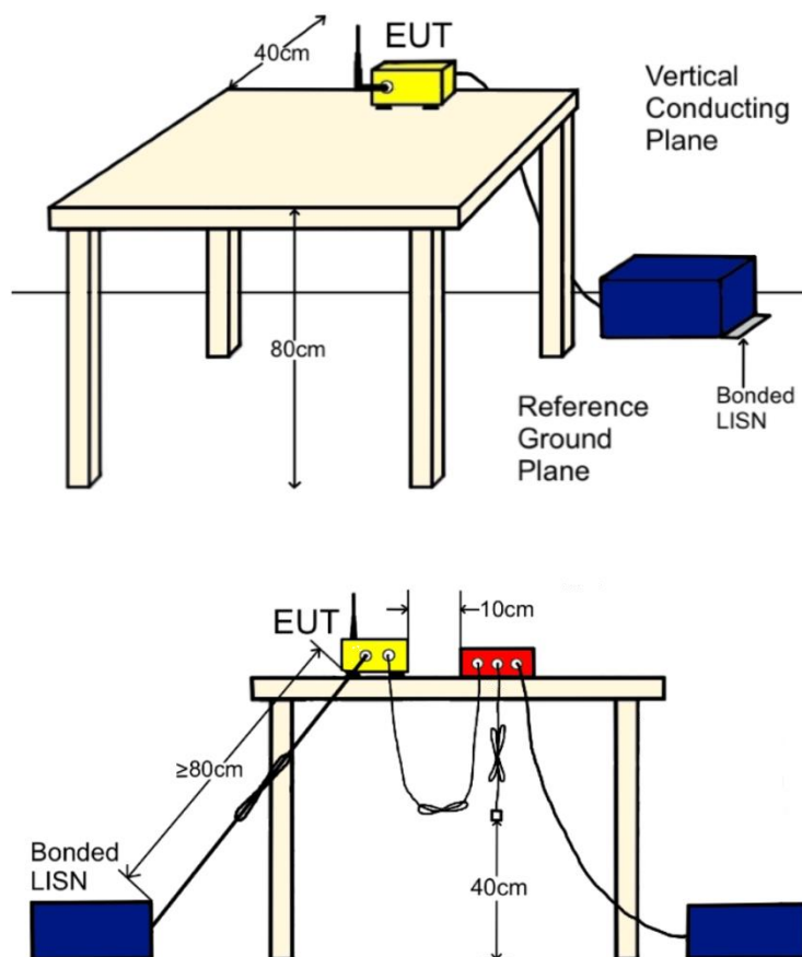
Figure 10. CEV Test Setup
