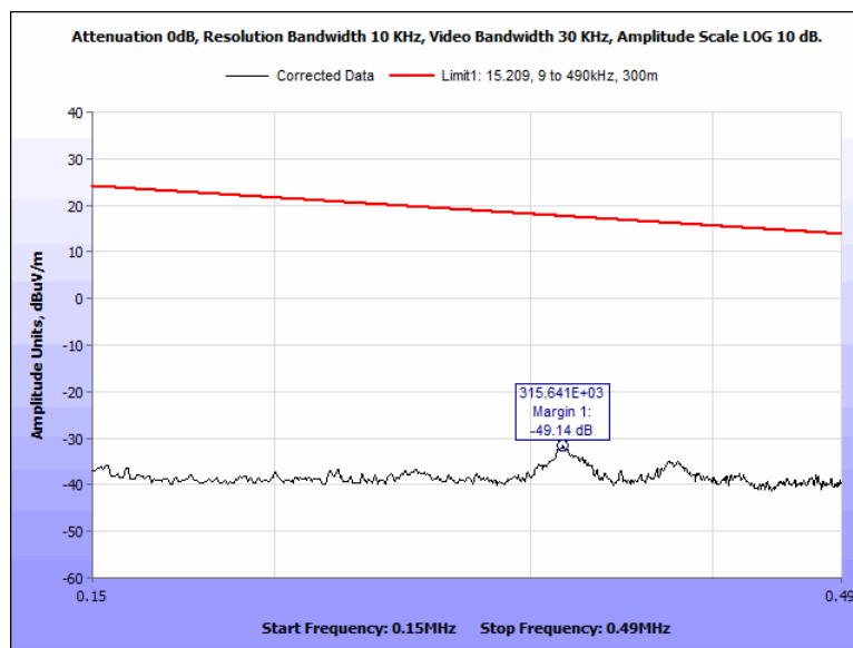
Figure 24. Spurious Emissions, Outside the Bands 13.110 - 14.010 MHz, 0.150 – 0.490 MHz, 0 degrees
