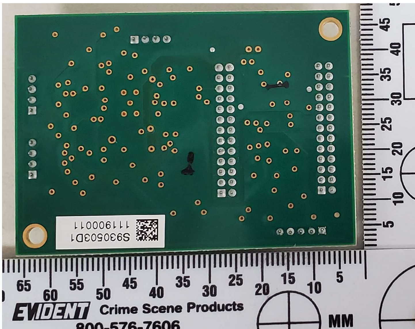
Output Controller Board Bottom Side
