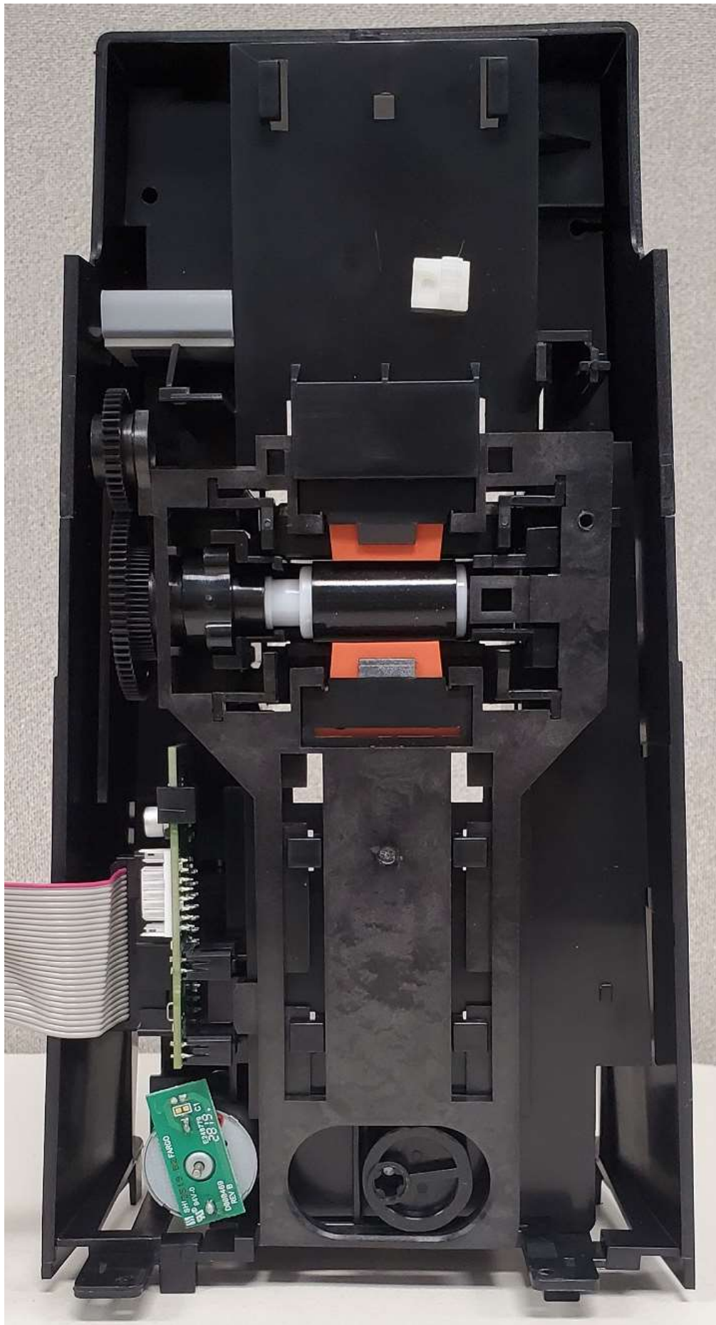
Input Hopper Controller Mounted
