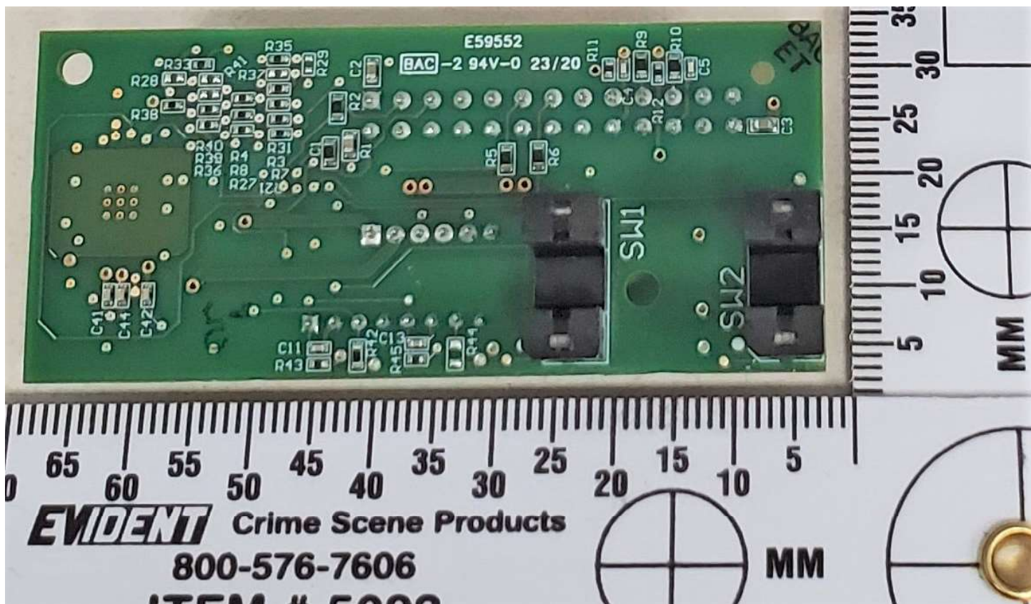
Input Hopper Controller Board Bottom Side
