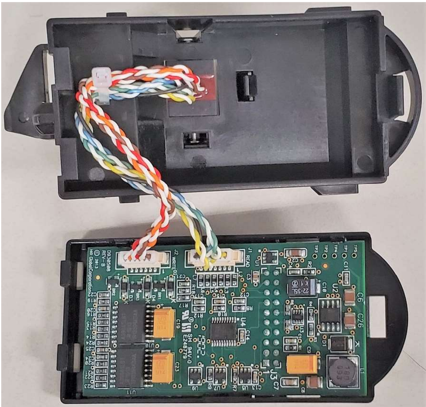
Magnetic Encoder Mounted
