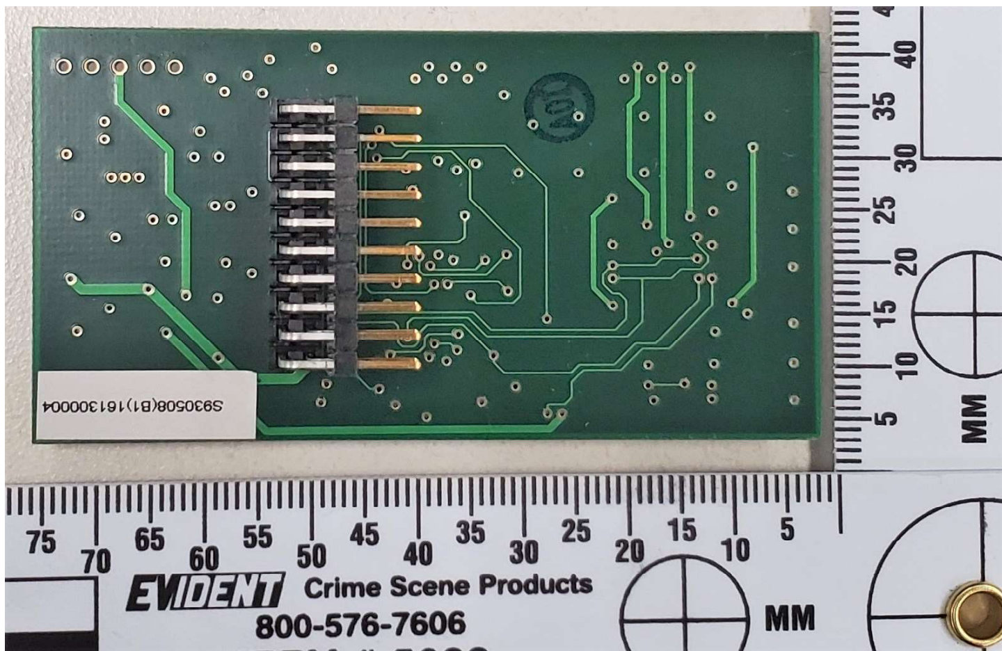
Magnetic Encoder Board Bottom
