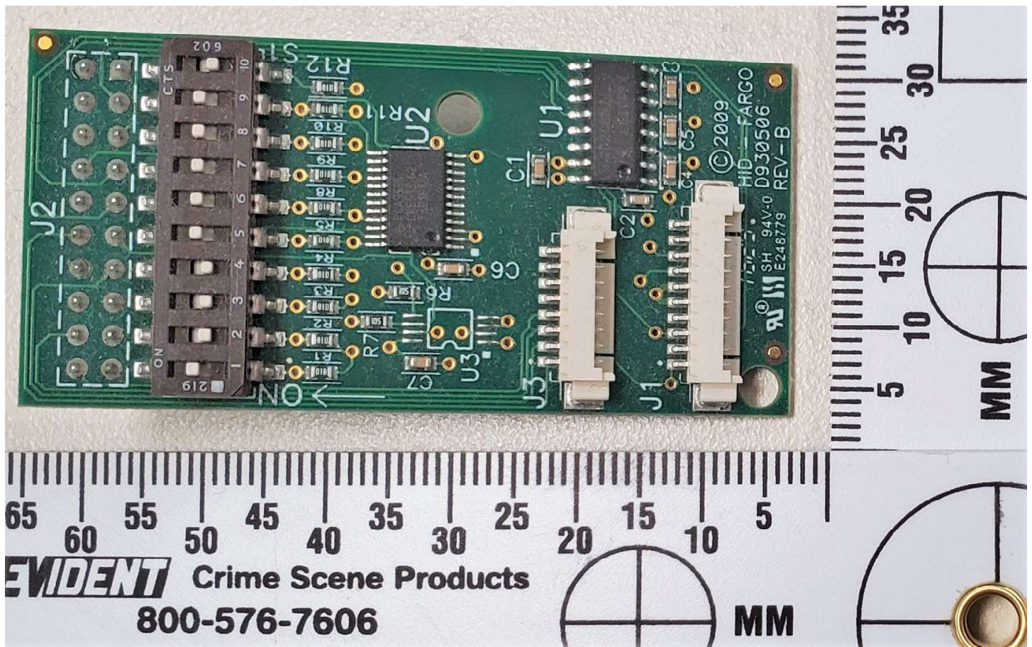
E-Card Encoder Interface Board Top Side
