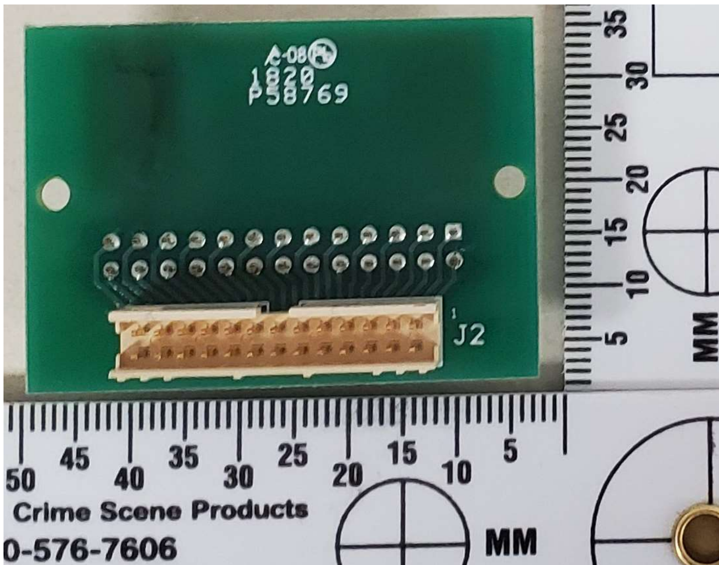
Flipper Regulator Interface Board Bottom Side
