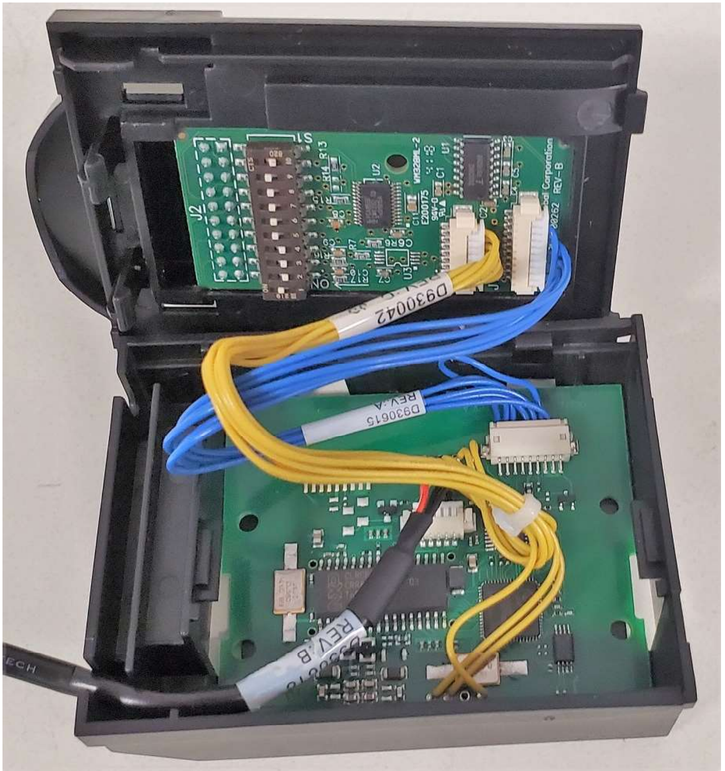
E-Card Encoder and Interface Mounted
