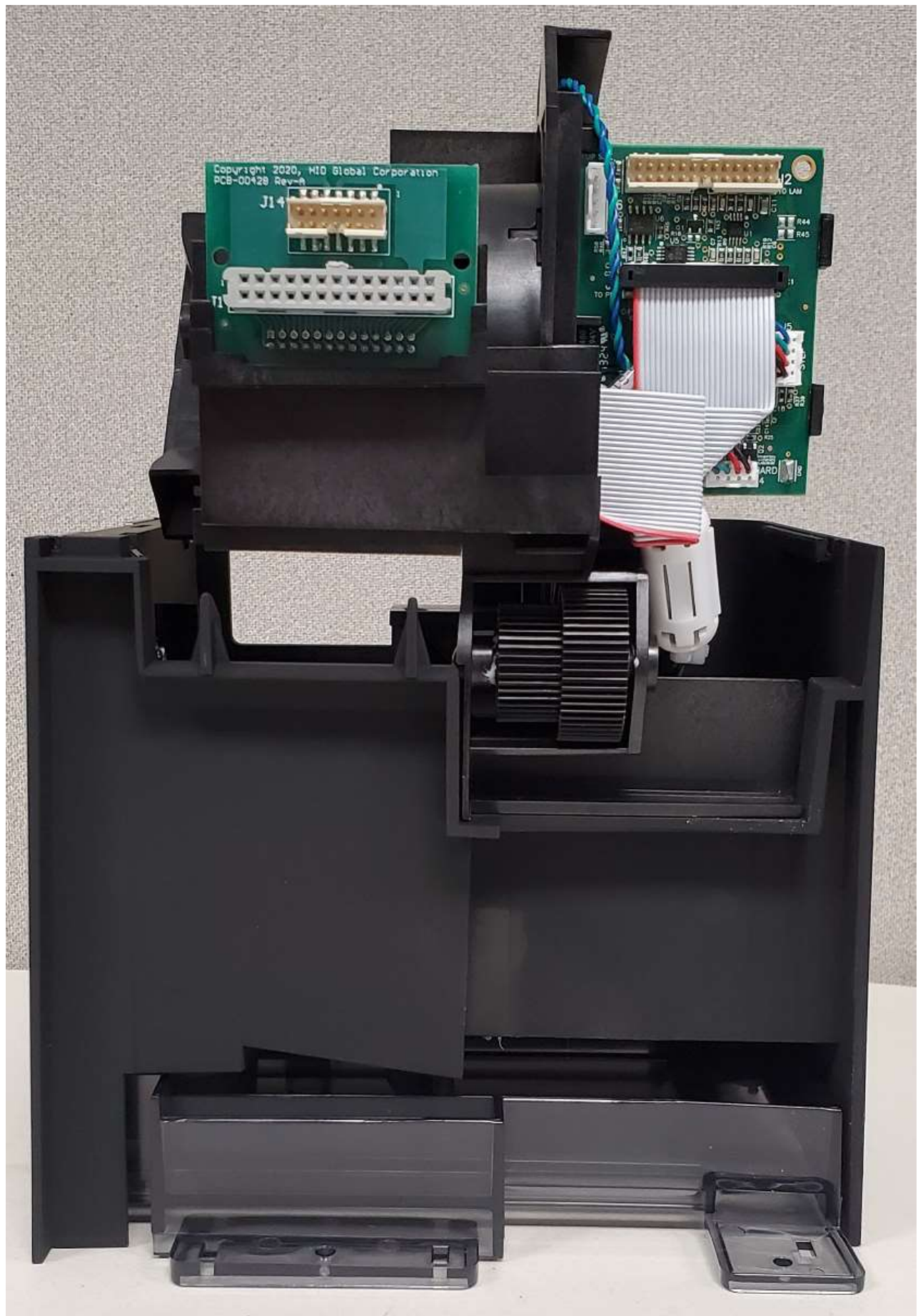
Output Controller and Flipper Regulator Interface Mounted
