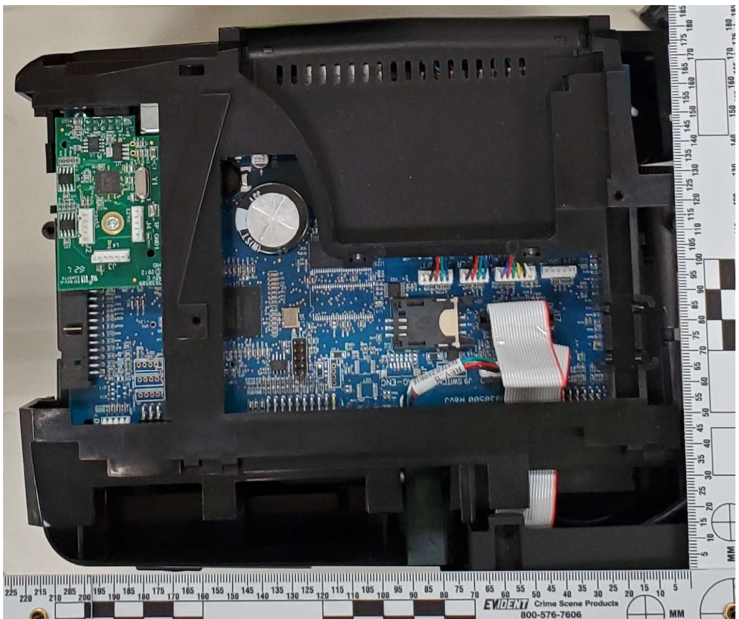
Main Board and USB Hub with top cover removed
