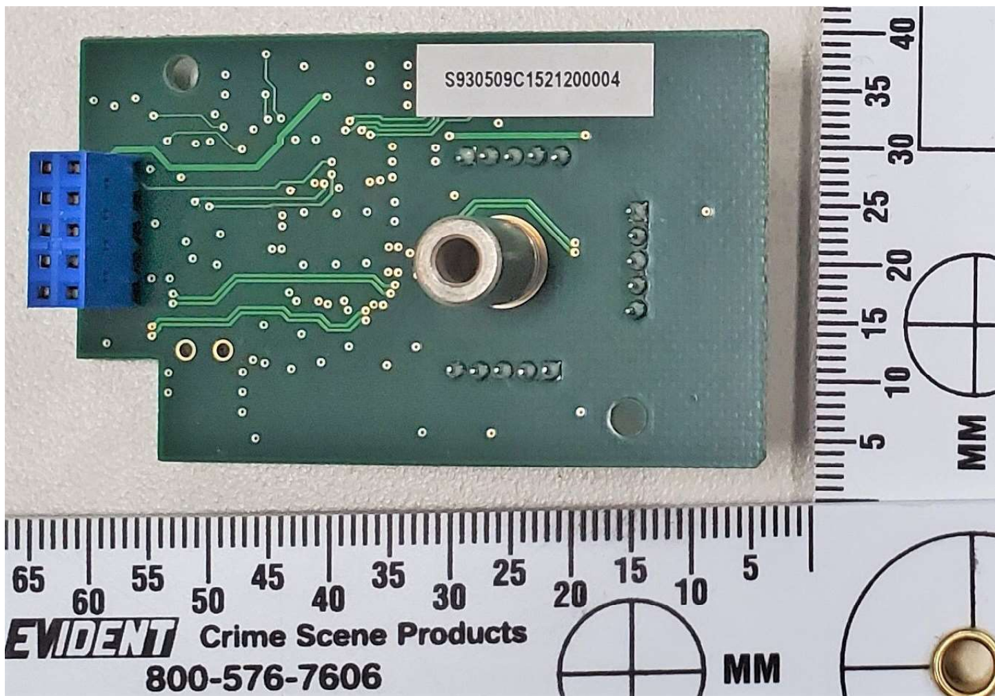
USB Hub Board Bottom Side
