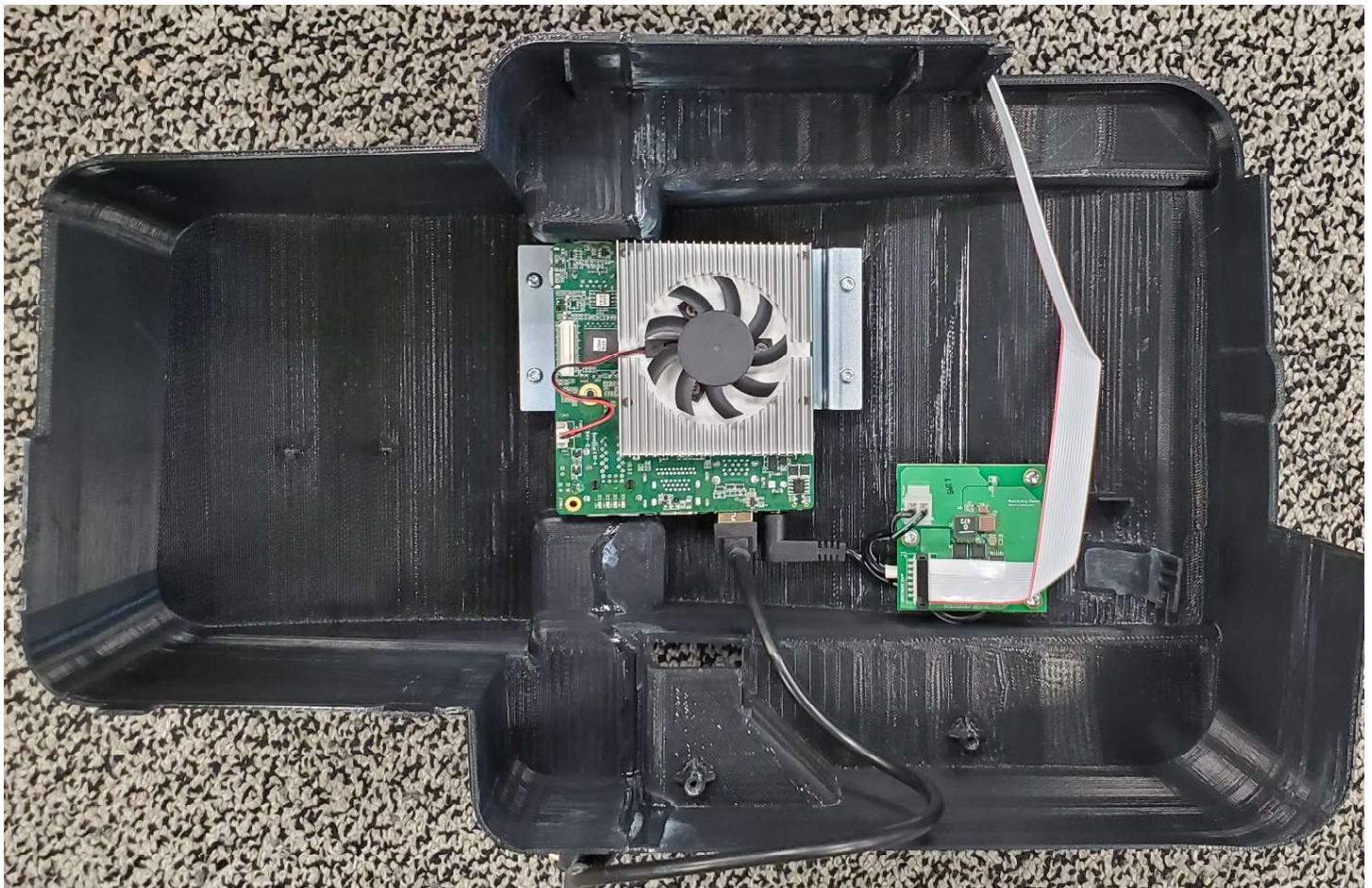
PC board and auxiliary power board mounted inside top cover
