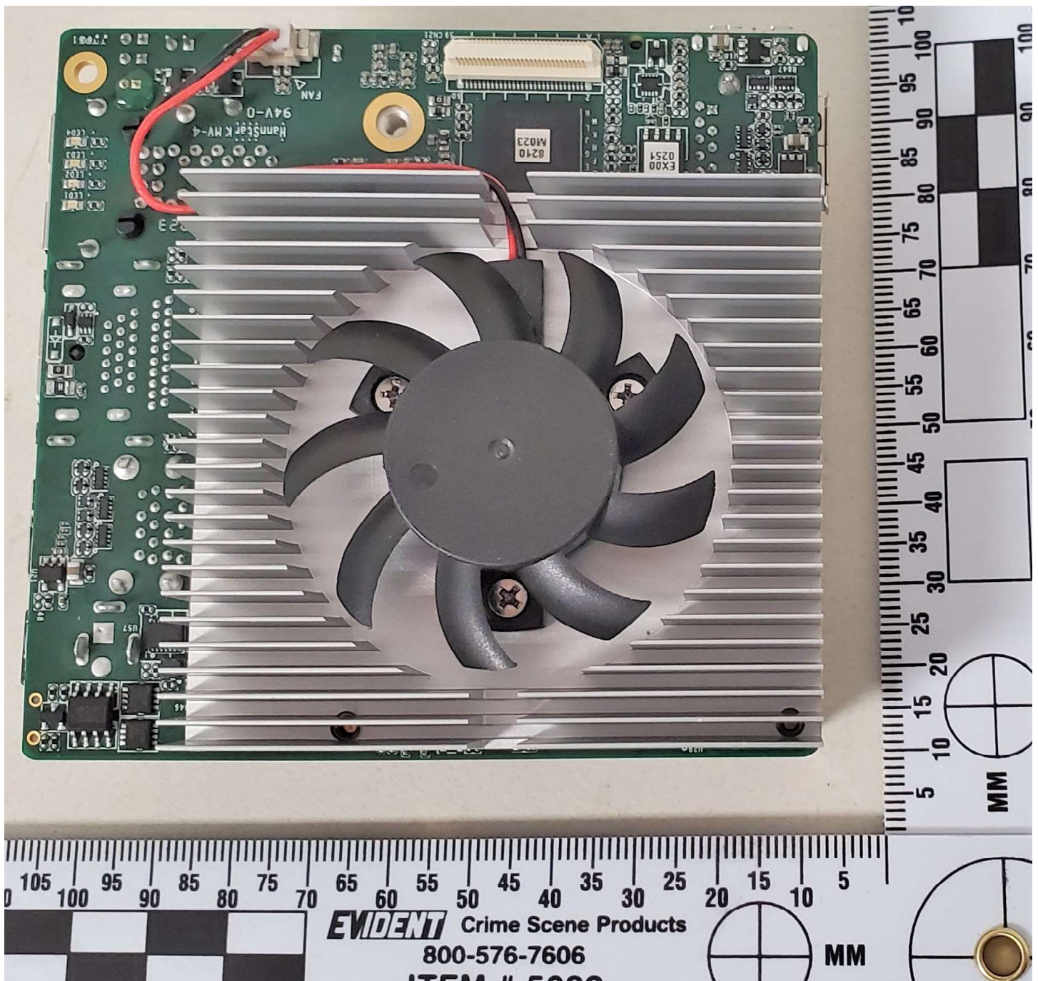
PC Board Bottom Side
