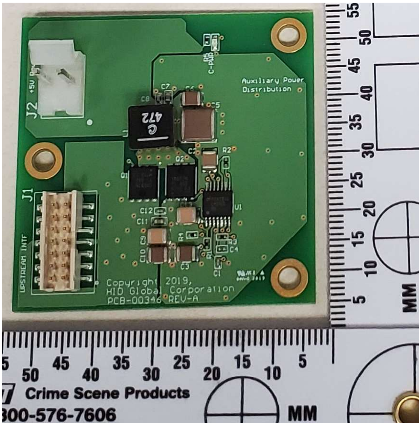
Auxiliary Power Board Top Side
