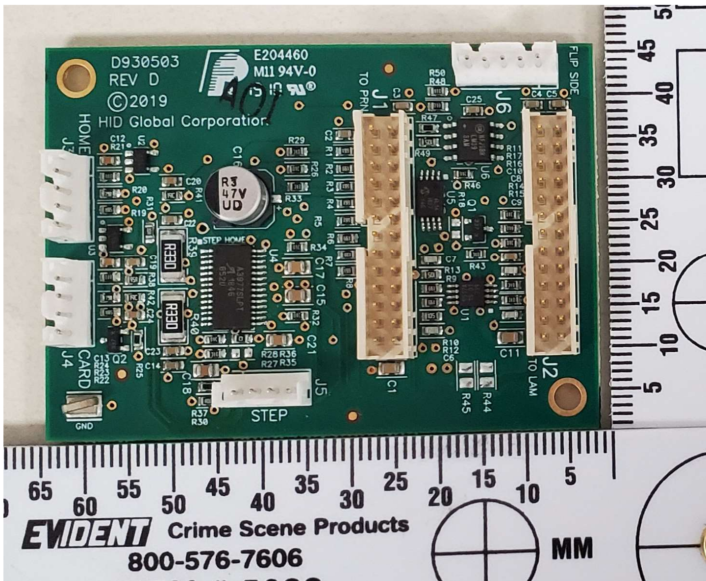
Output Controller Board Top Side
