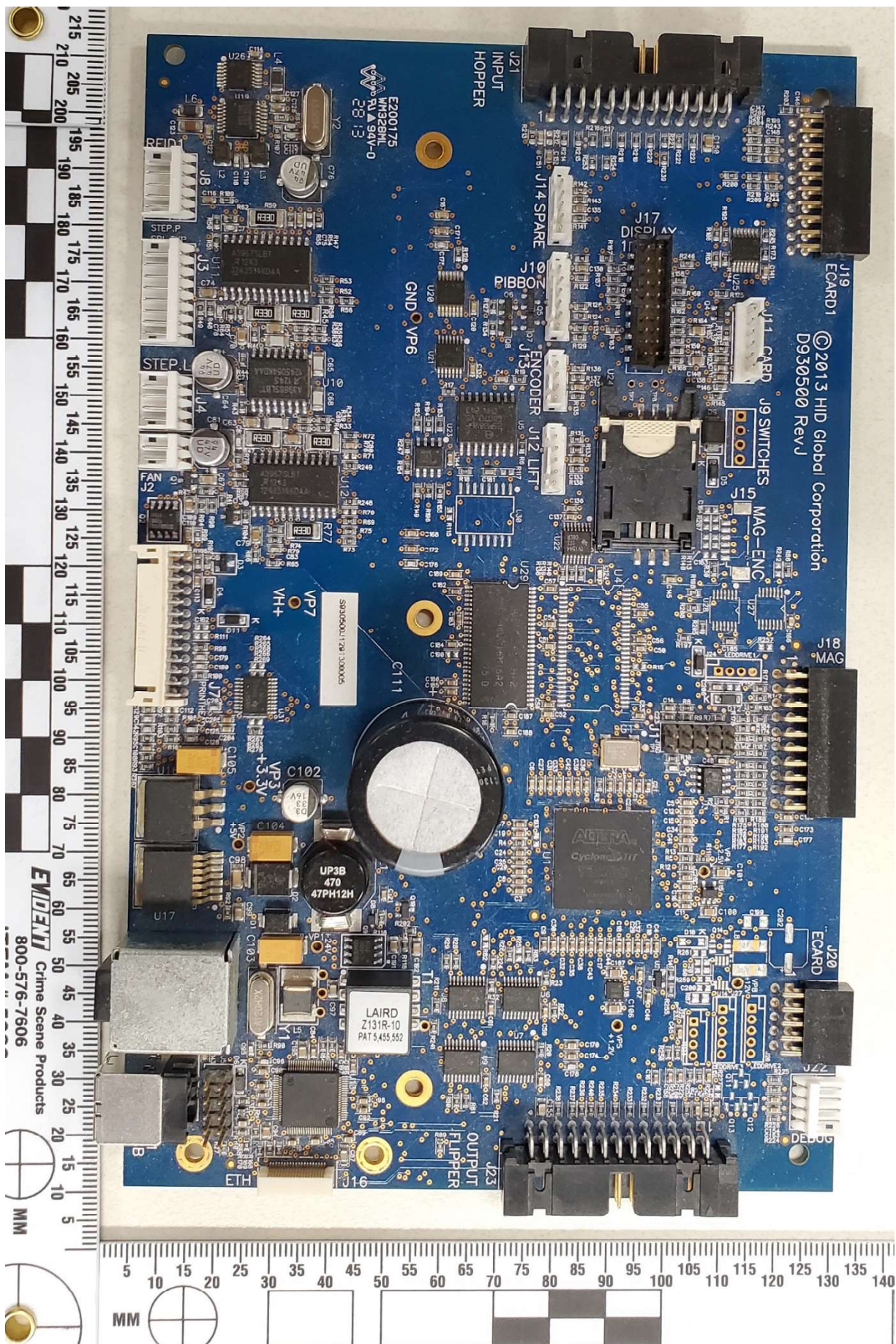
Main Board Top Side
