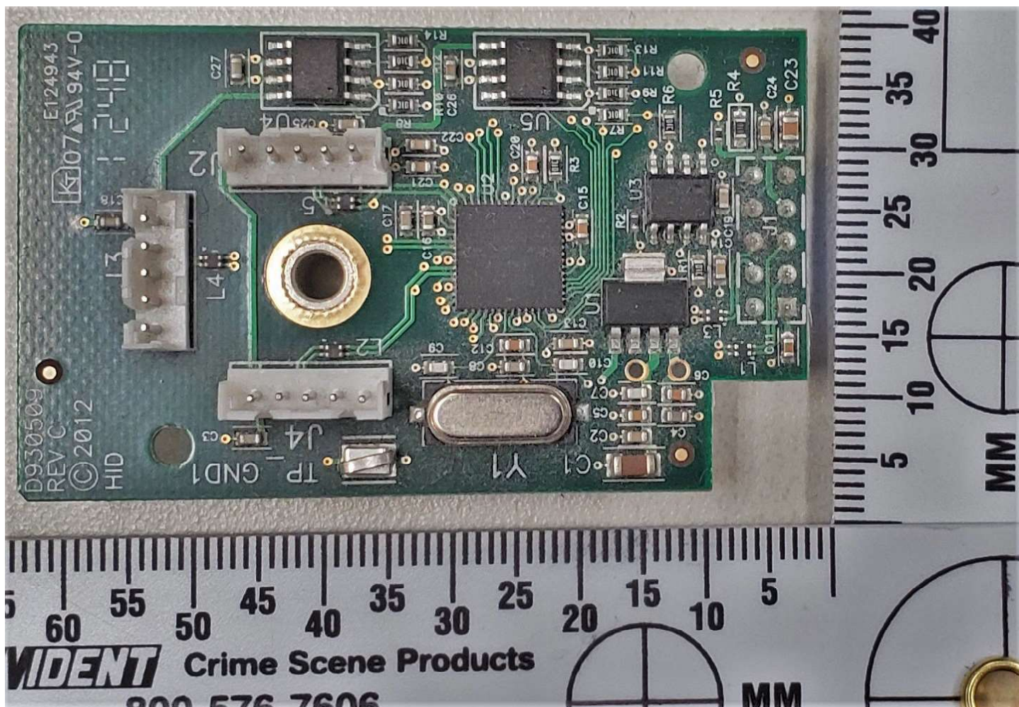
USB Hub Board Top Side
