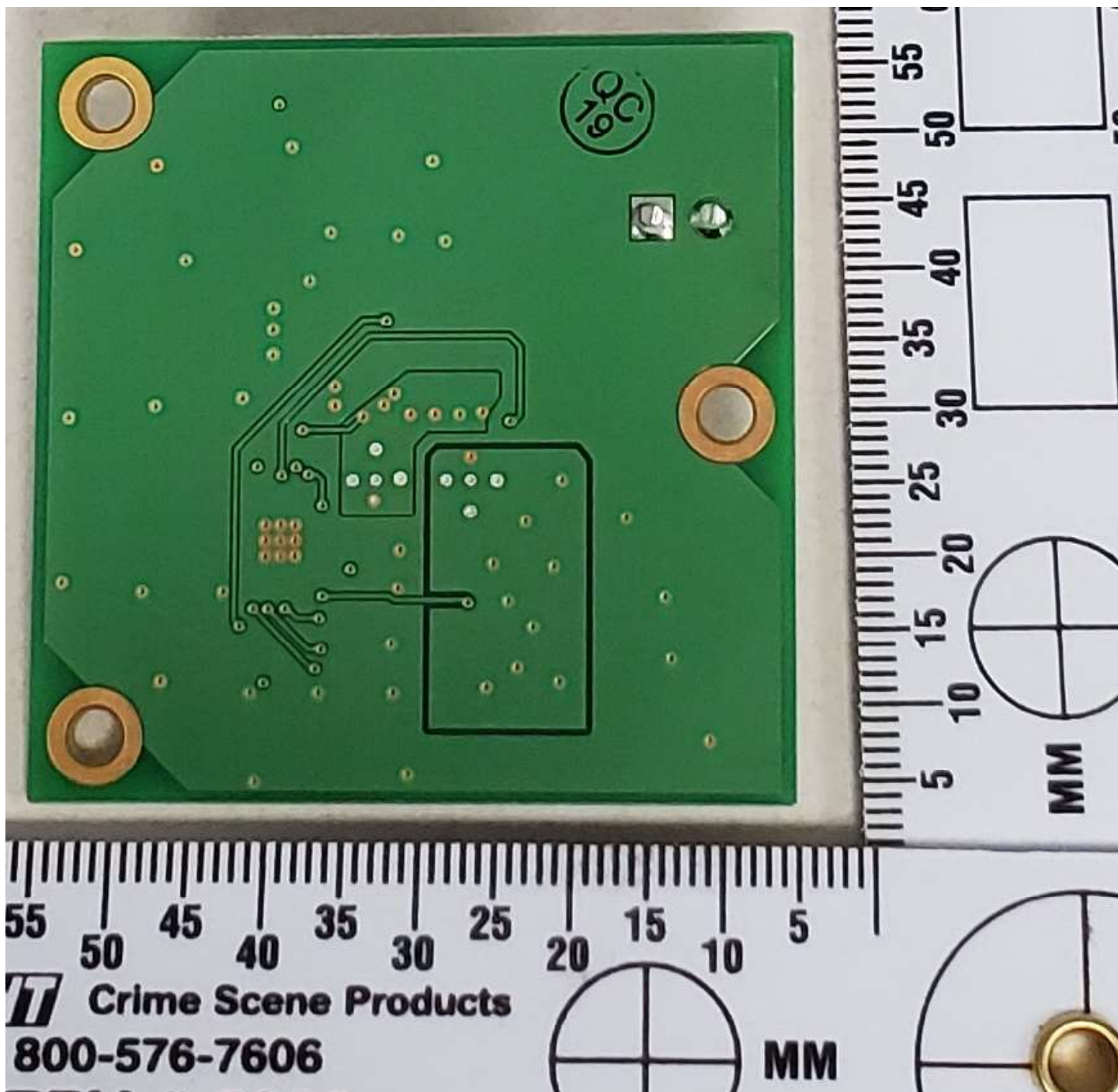
Auxiliary Power Board Bottom
