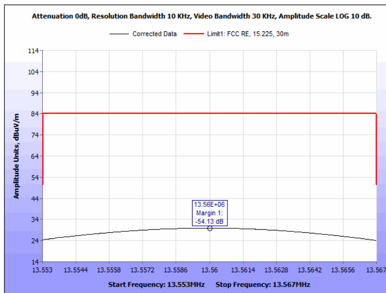
Plot 7. Field Strength Within the Band 13.553 -13.567 MHz, 0 Degrees, Ribbon
