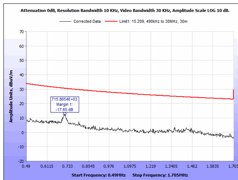
Plot 30 Field Strength Outside the Band 13.110 – 14.010 MHz band, 0.490 – 1.705 MHz, 90 degrees, Encoder, Peak Scan
