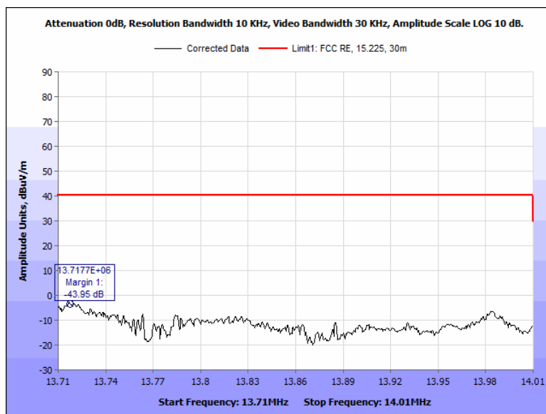
Plot 19. Field Strength Within the Band 13.710-14.010 MHz, 0 Degrees, Encoder, Peak Scan
