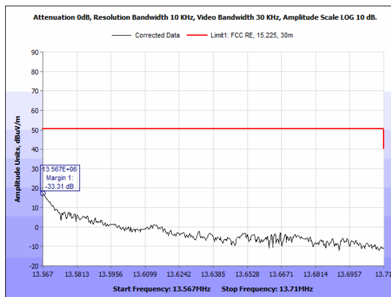
Plot 12. Field Strength Within the Band 13.567-13.710 MHz, 90 Degrees, Encoder, Peak Scan
