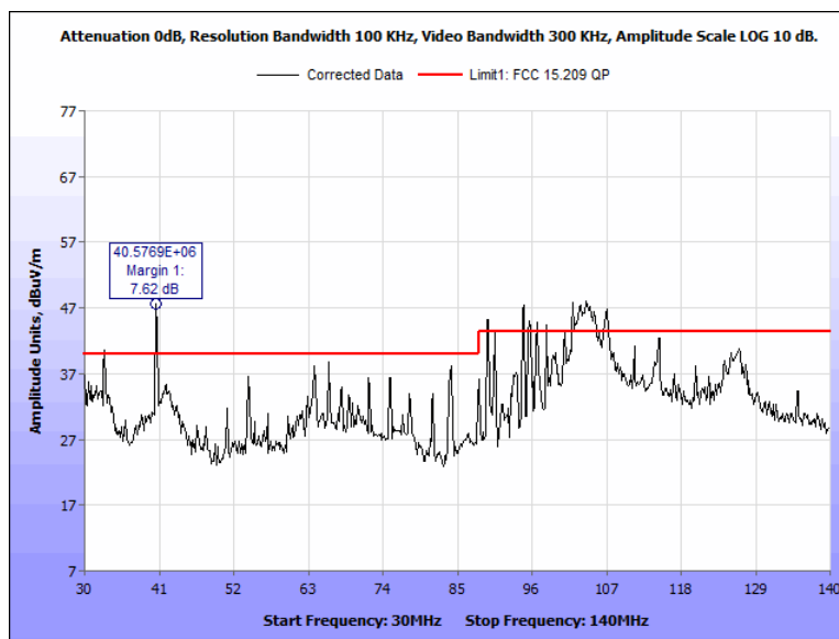
Plot 43. Field Strength Outside the Band 13.110 – 14.010 MHz band, 30-140 MHz, Vertical, Ribbon, Peak Scan
