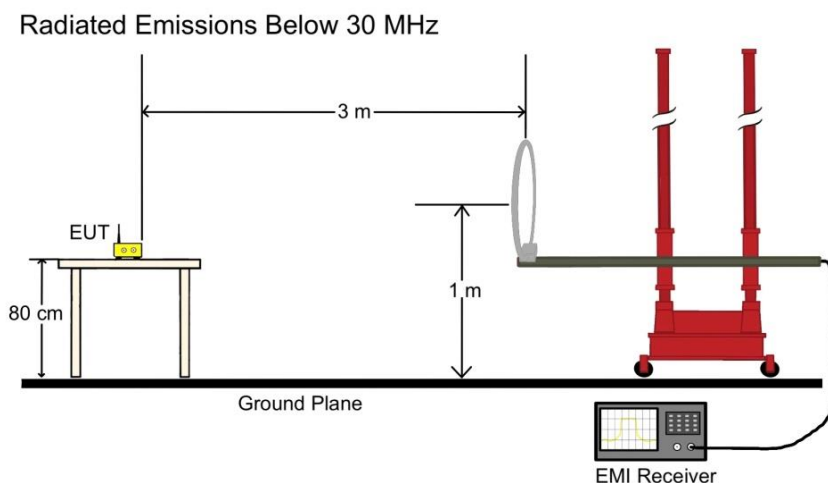
Figure 5: Radiated Emissions, Test Setup
