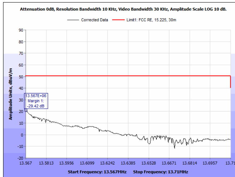
Plot 11. Field Strength Within the Band 13.567-13.710 MHz, 0 Degrees, Encoder, Peak Scan
