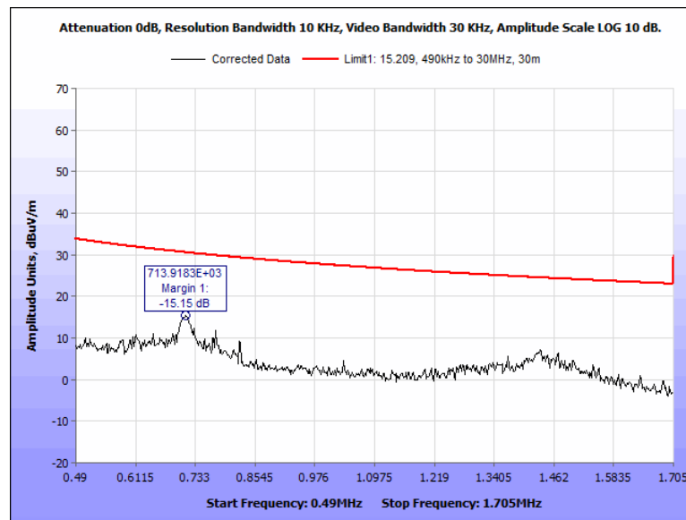
Plot 29. Field Strength Outside the Band 13.110 – 14.010 MHz band, 0.490 – 1.705 MHz, 0 degrees, Encoder, Peak Scan
