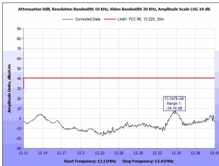
Plot 21. Field Strength Within the Band 13.110-13.410 MHz, 0 Degrees, Ribbon, Peak Scan
