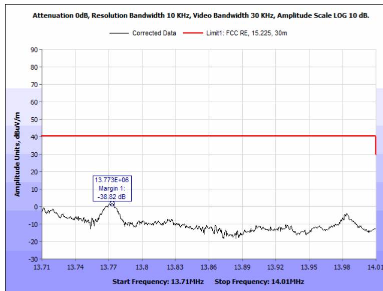
Plot 23. Field Strength Within the Band 13.710-14.010 MHz, 0 Degrees, Ribbon, Peak Scan
