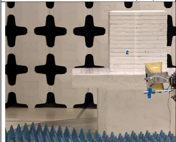
Radiated Emission-Above 1GHz-Front (X-axis)
