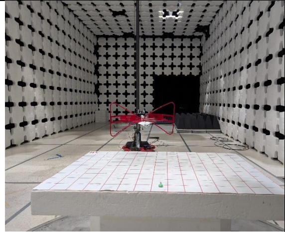
Radiated Emission-Below 1GHz-Back View (X-axis)
