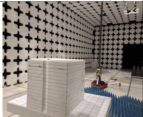
Radiated Emission-Above 1GHz-Back (X-axis)
