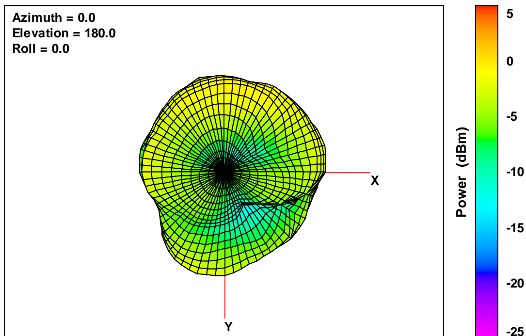
40 V2 Free-Space Total EIRP, Bottom View, 2482 MHz
