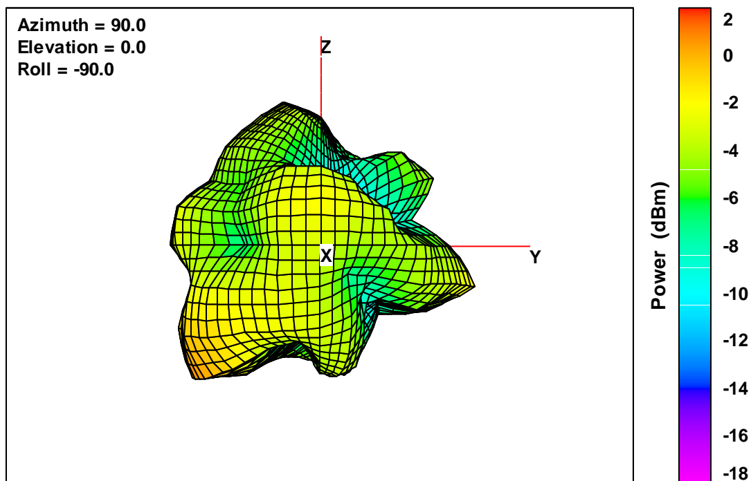
40 V2 Free-Space Total EIRP, Front Face View, 2442 MHz
