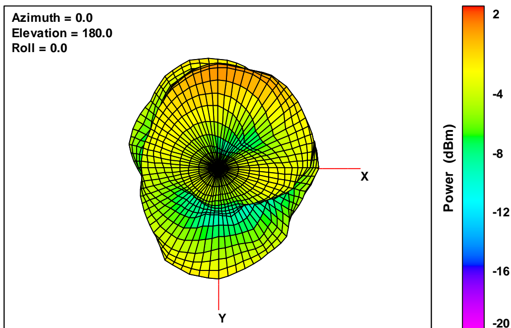
40 V2 Free-Space Total EIRP, Bottom View, 2402 MHz
