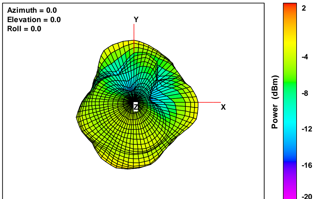
40 V2 Free-Space Total EIRP, Top View, 2402 MHz
