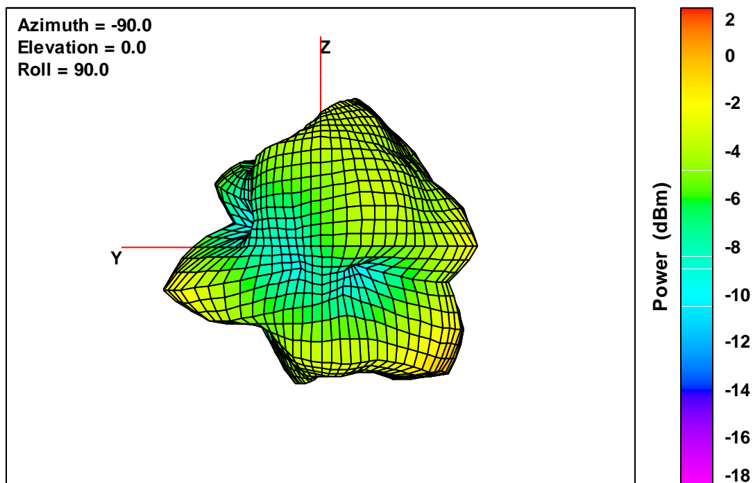
40 V2 Free-Space Total EIRP, Back Face View, 2442 MHz
