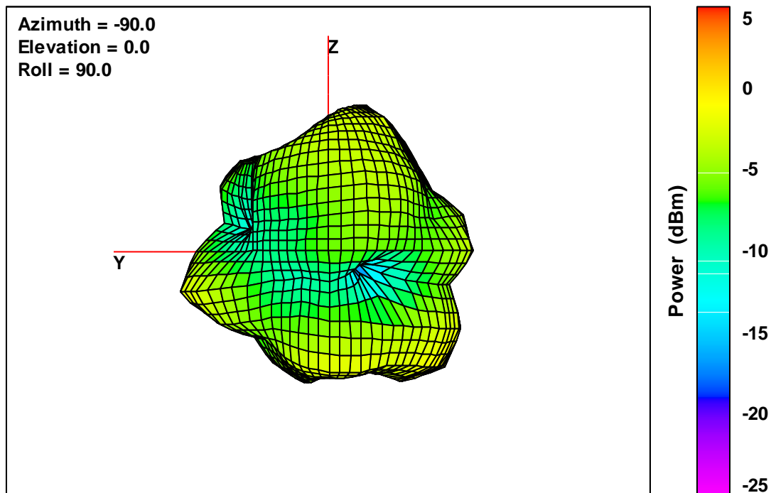
40 V2 Free-Space Total EIRP, Back Face View, 2482 MHz
