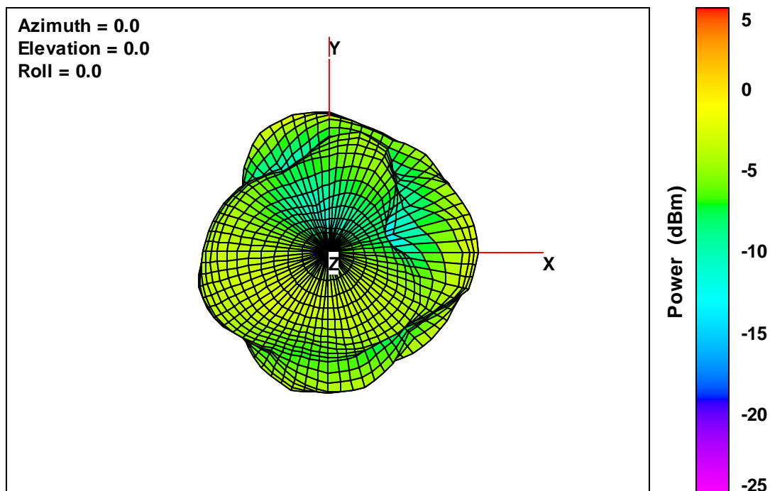
40 V2 Free-Space Total EIRP, Top View, 2482 MHz
