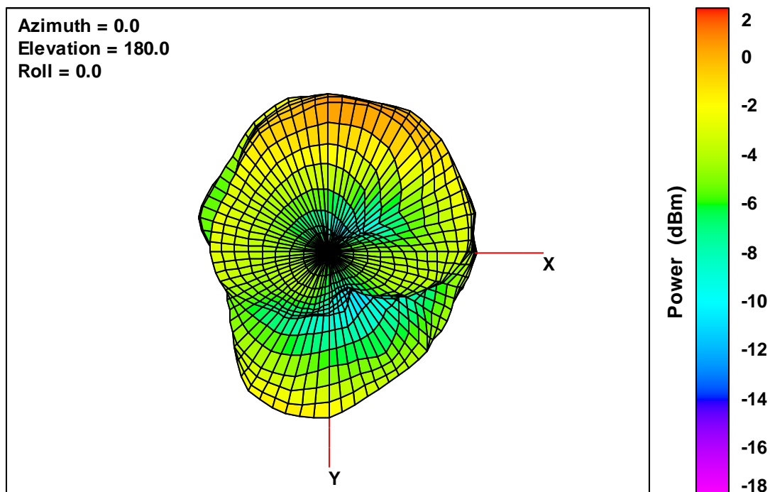
40 V2 Free-Space Total EIRP, Bottom View, 2442 MHz
