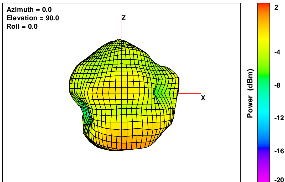
40 V2 Free-Space Total EIRP, Left Side View, 2402 MHz
