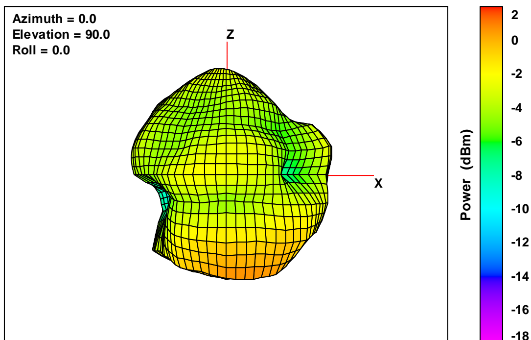
40 V2 Free-Space Total EIRP, Left Side View, 2442 MHz
