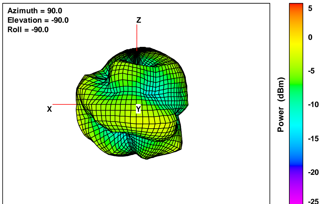
40 V2 Free-Space Total EIRP, Right Side View, 2482 MHz
