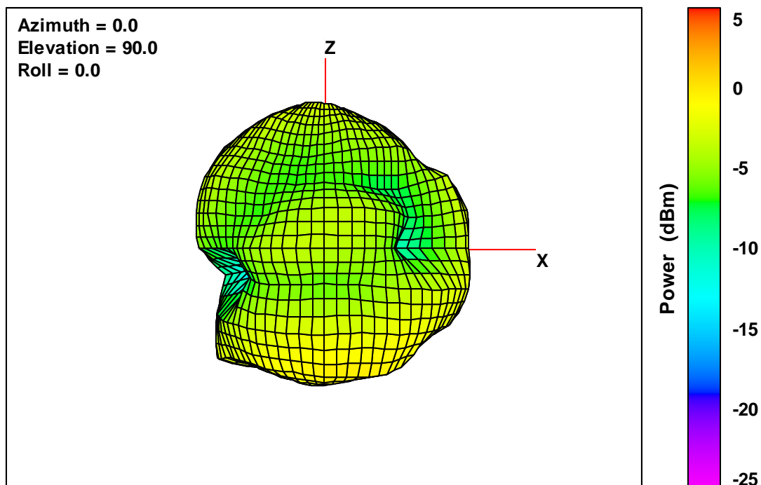
40 V2 Free-Space Total EIRP, Left Side View, 2482 MHz
