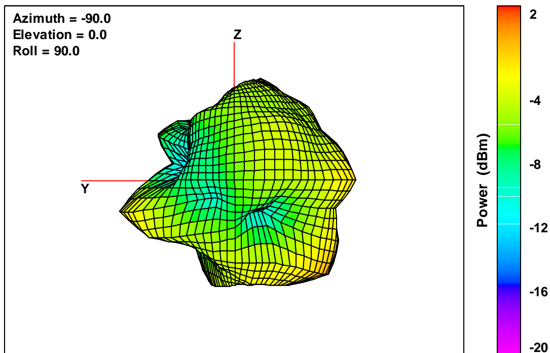
40 V2 Free-Space Total EIRP, Back Face View, 2402 MHz
