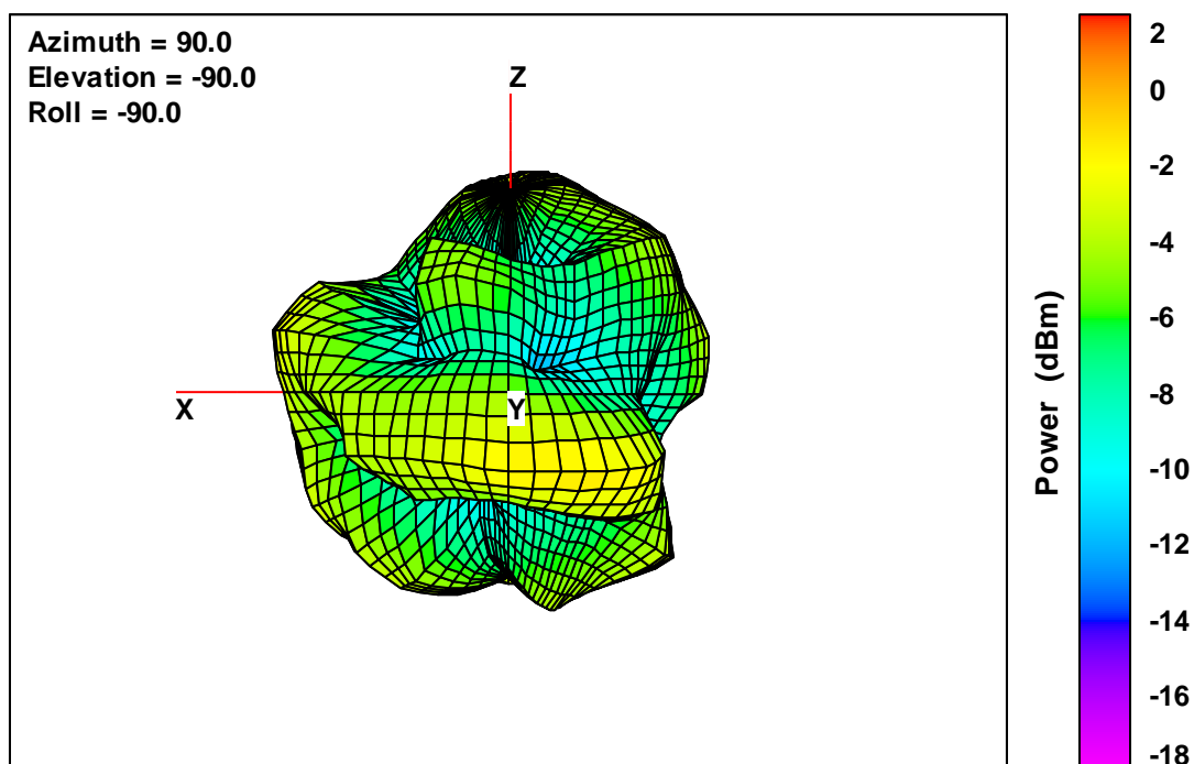
40 V2 Free-Space Total EIRP, Right Side View, 2442 MHz
