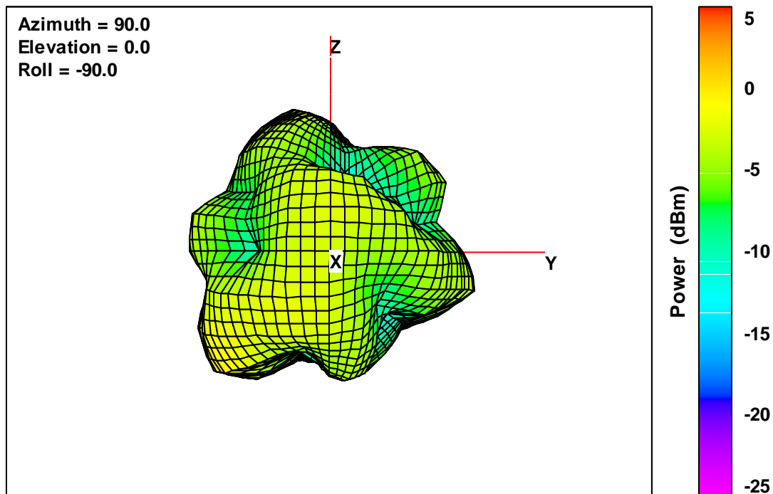
40 V2 Free-Space Total EIRP, Front Face View, 2482 MHz
