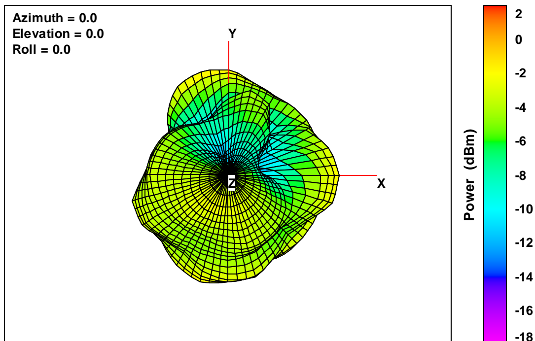
40 V2 Free-Space Total EIRP, Top View, 2442 MHz
