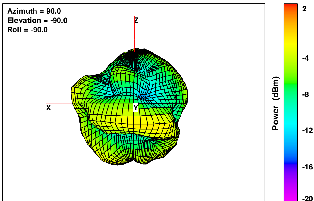
40 V2 Free-Space Total EIRP, Right Side View, 2402 MHz
