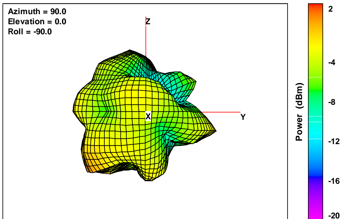
40 V2 Free-Space Total EIRP, Front Face View, 2402 MHz
