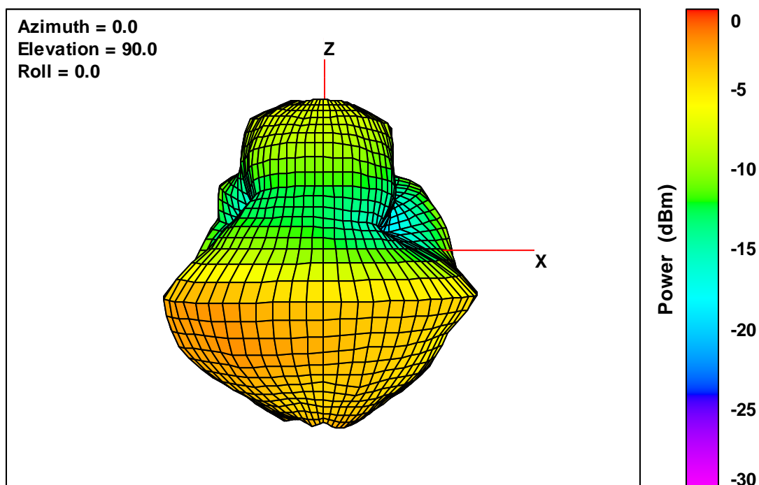
40T V2 Free-Space Total EIRP, Left Side View, 2402 MHz
