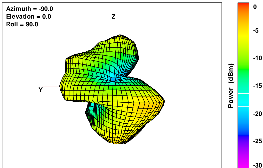
40T V2 Free-Space Total EIRP, Back Face View, 2482 MHz
