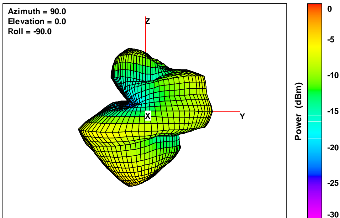
40T V2 Free-Space Total EIRP, Front Face View, 2482 MHz
