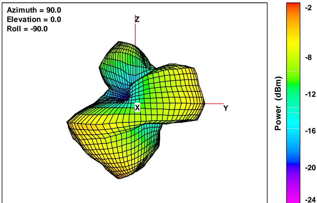
40T V2 Free-Space Total EIRP, Front Face View, 2442 MHz
