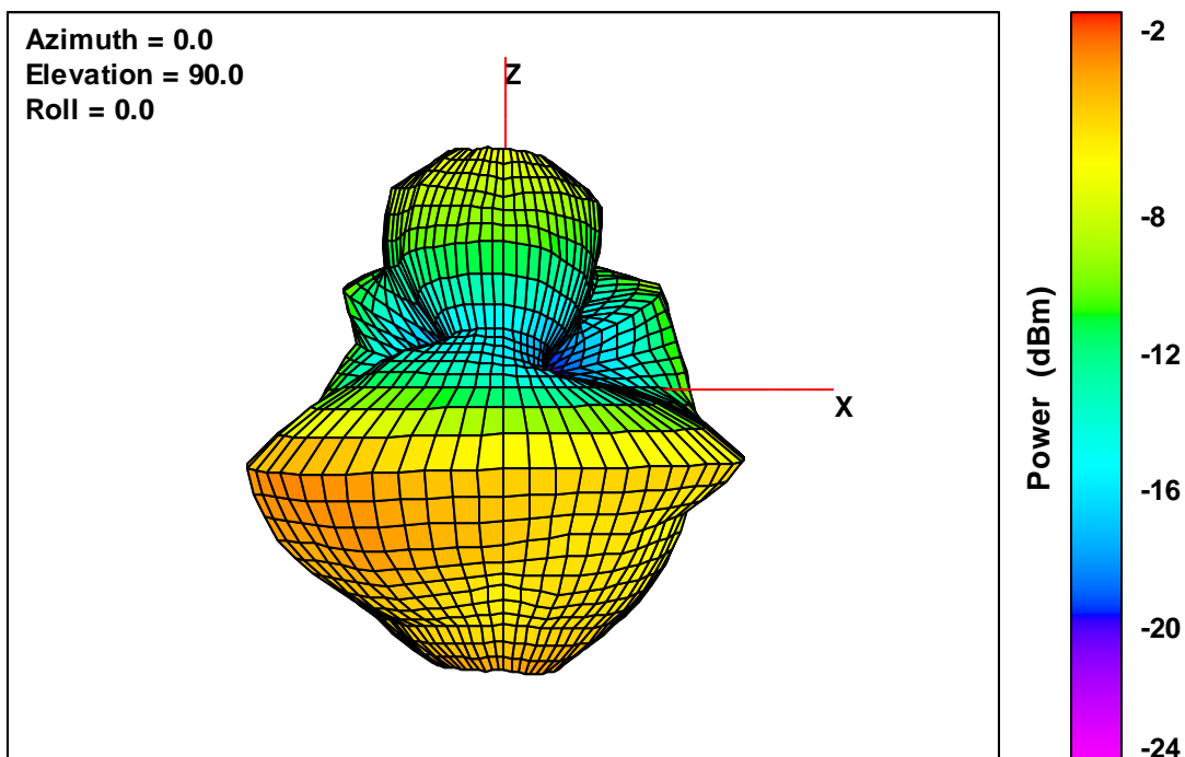
40T V2 Free-Space Total EIRP, Left Side View, 2442 MHz
