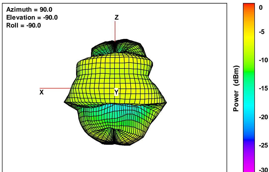
40T V2 Free-Space Total EIRP, Right Side View, 2482 MHz
