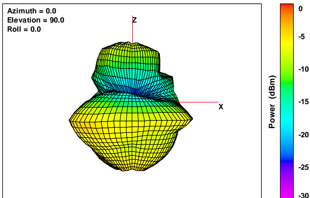
40T V2 Free-Space Total EIRP, Left Side View, 2482 MHz
