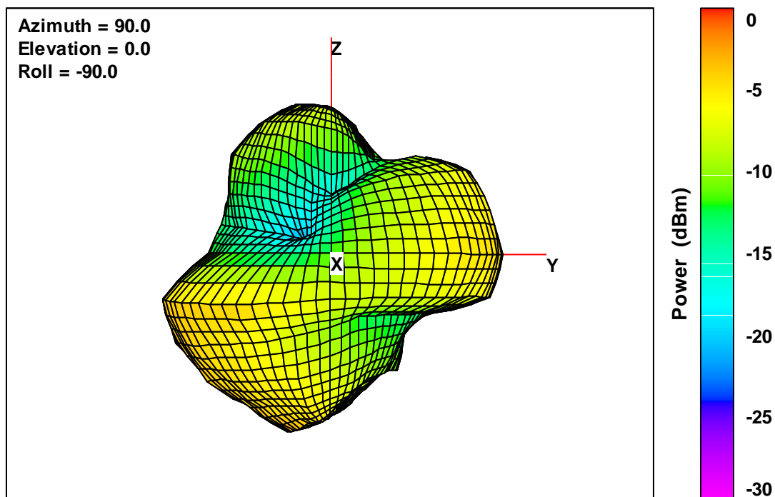
40T V2 Free-Space Total EIRP, Front Face View, 2402 MHz
