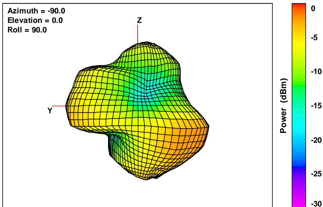
40T V2 Free-Space Total EIRP, Back Face View, 2402 MHz
