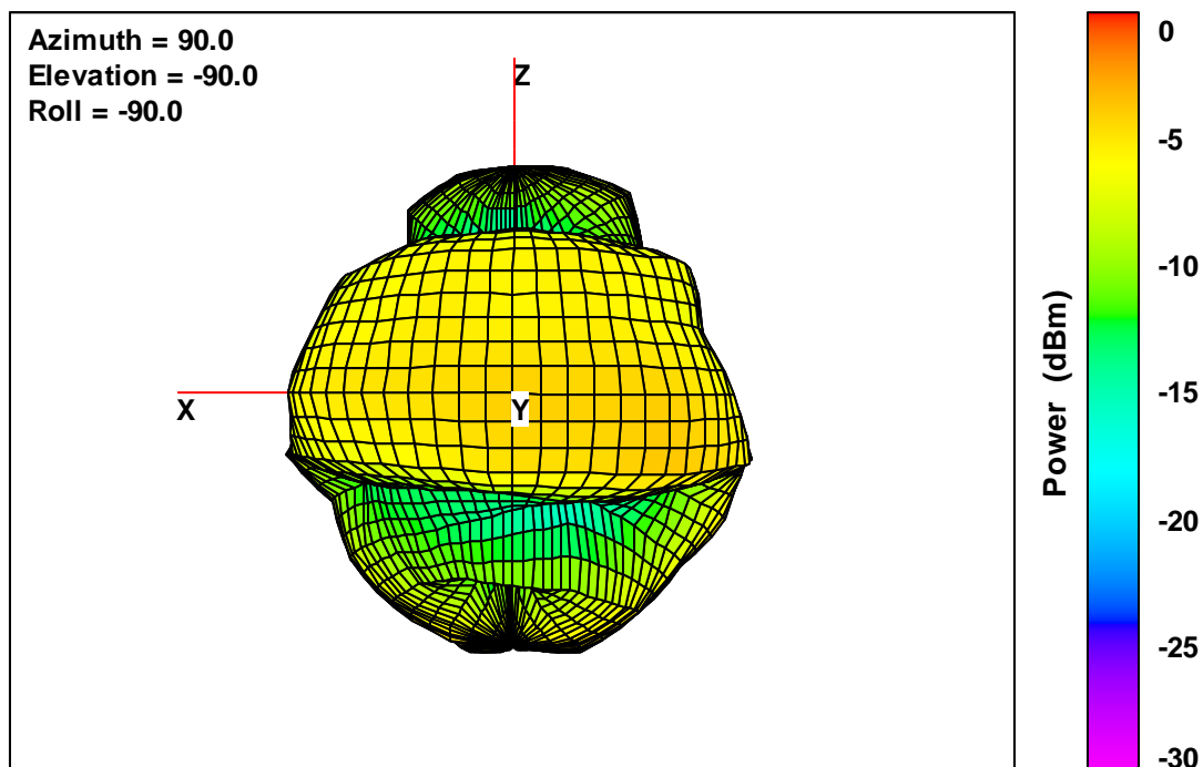
40T V2 Free-Space Total EIRP, Right Side View, 2402 MHz
