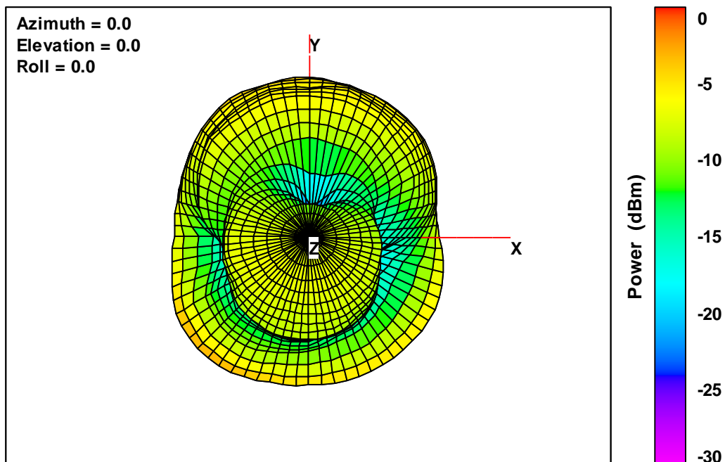
40T V2 Free-Space Total EIRP, Top View, 2402 MHz
