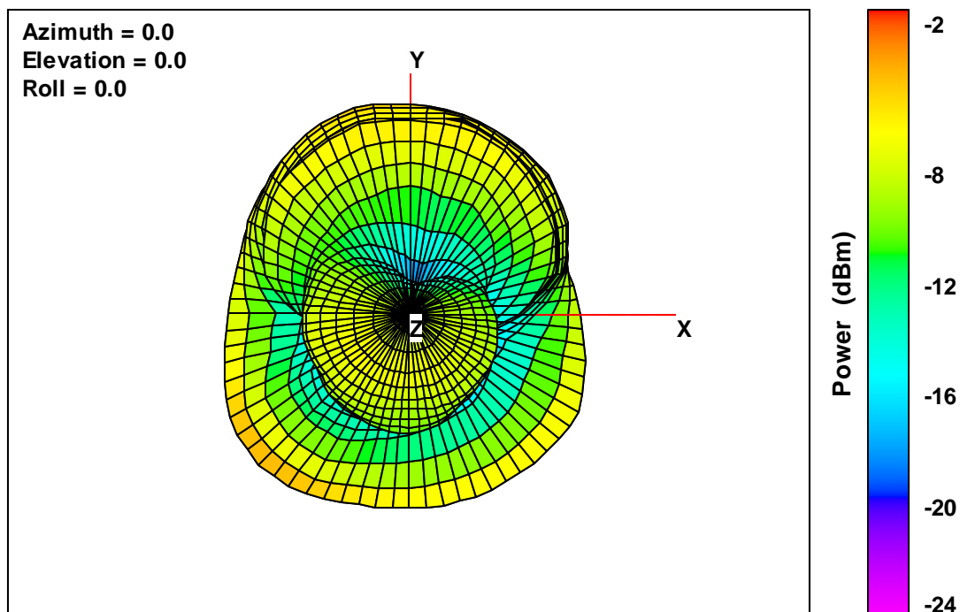
40T V2 Free-Space Total EIRP, Top View, 2442 MHz
