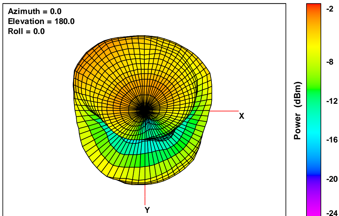
40T V2 Free-Space Total EIRP, Bottom View, 2442 MHz
