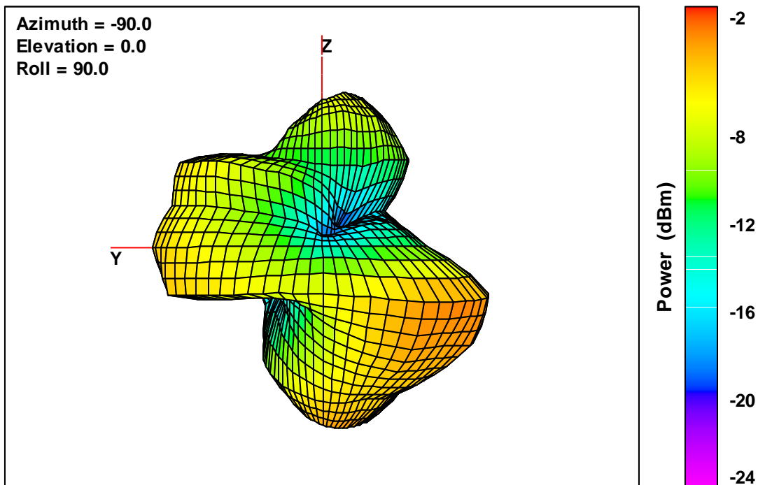
40T V2 Free-Space Total EIRP, Back Face View, 2442 MHz
