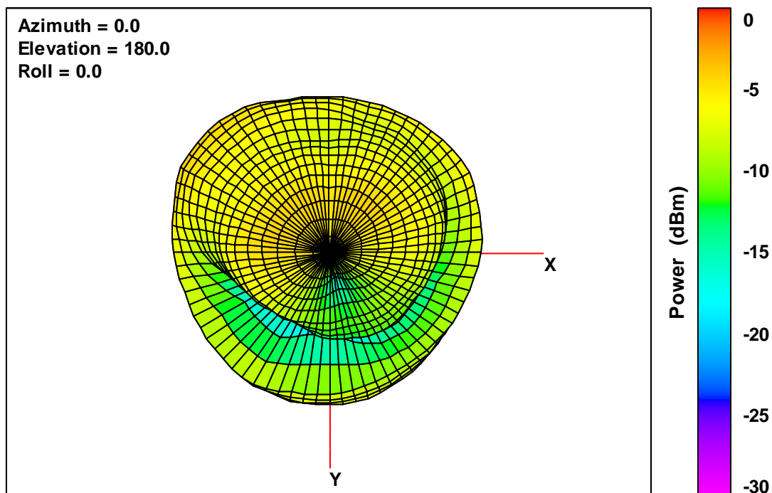
40T V2 Free-Space Total EIRP, Bottom View, 2482 MHz
