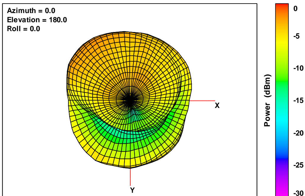
40T V2 Free-Space Total EIRP, Bottom View, 2402 MHz
