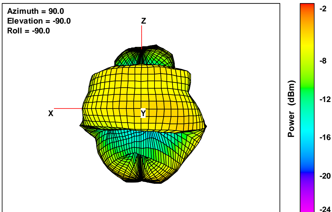
40T V2 Free-Space Total EIRP, Right Side View, 2442 MHz
