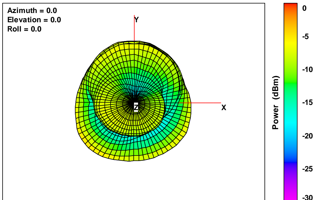
40T V2 Free-Space Total EIRP, Top View, 2482 MHz
