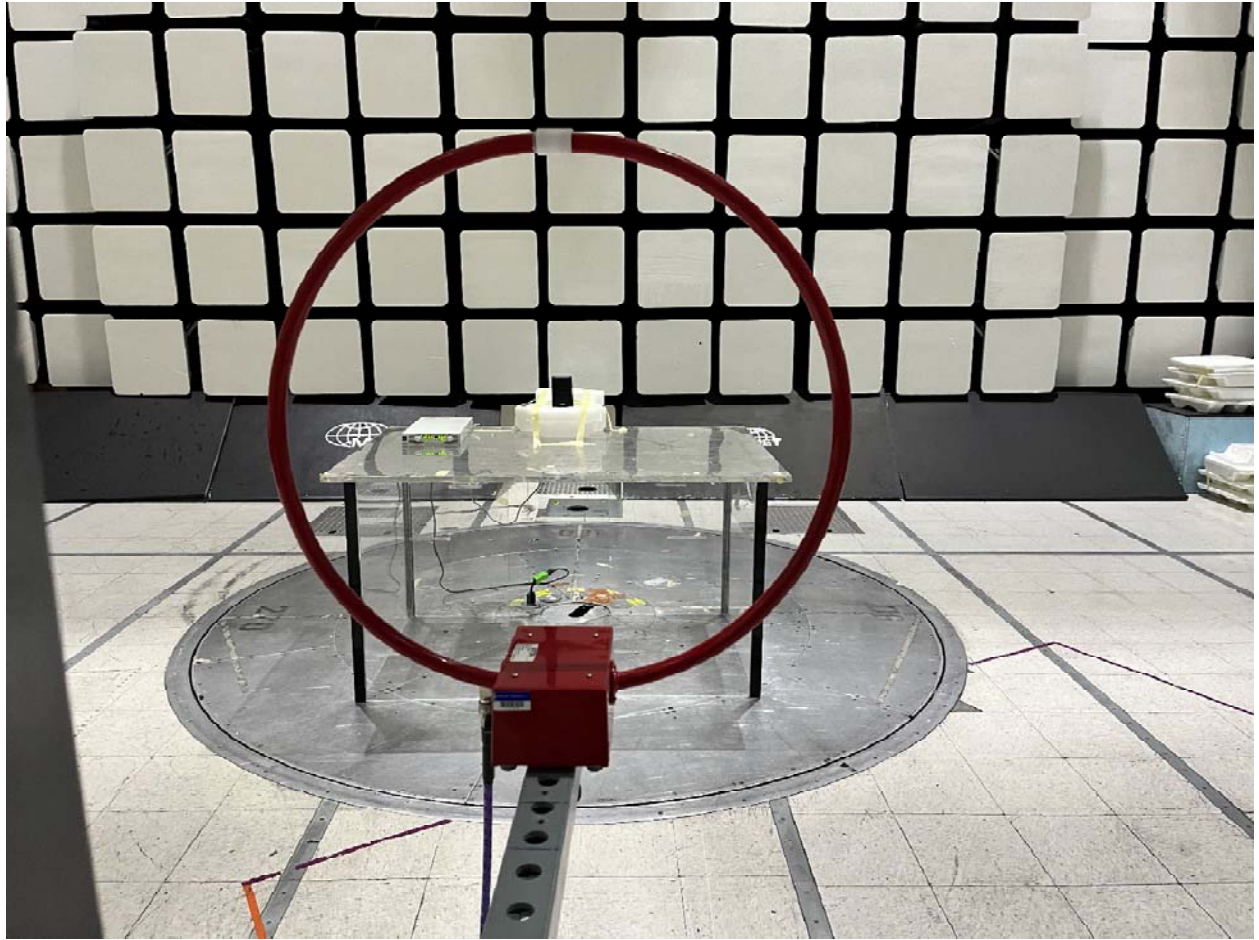
Radiated Emissions Below 30 MHz Antenna View
