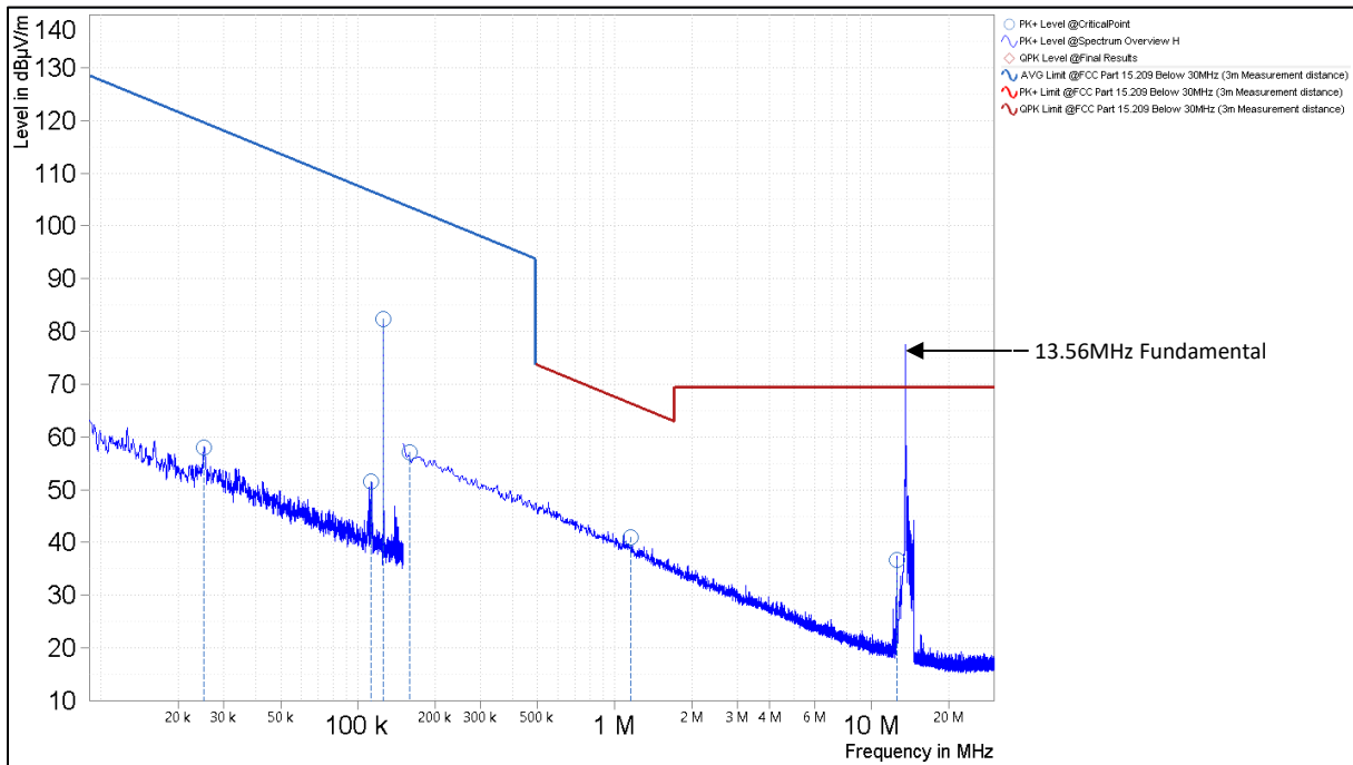
Figure 6. Spurious Emissions Below 30MHz, (Terminal, Coplanar Loop 5 )
