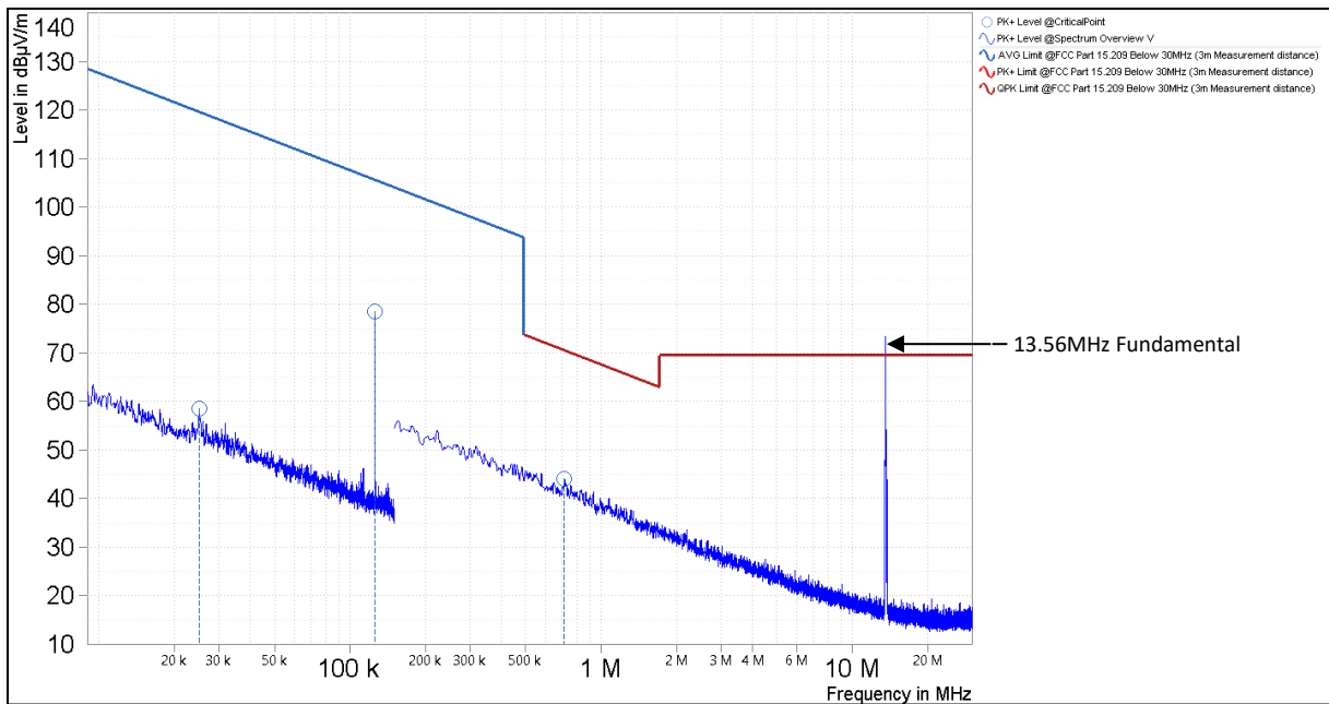
Figure 11. Spurious Emissions Below 30MHz, (Pigtail, Coaxial Loop 5 )
