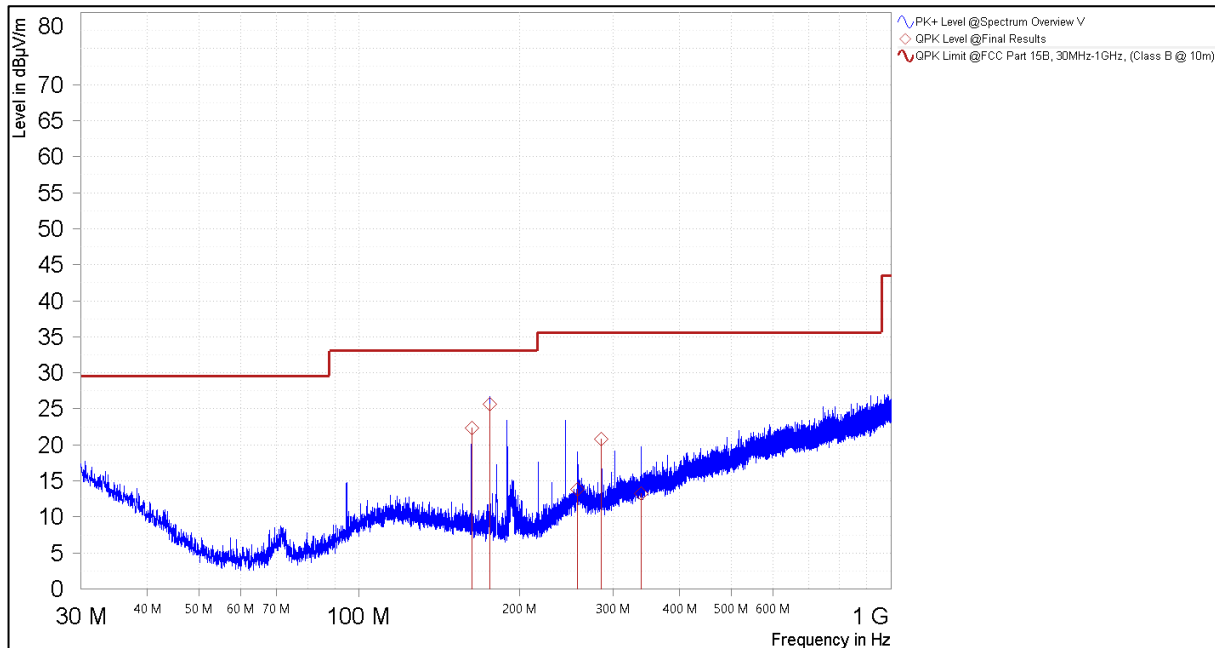
Figure 12. Spurious Emissions 30MHz – 1GHz, (Pigtail, Vertical Polarity)
