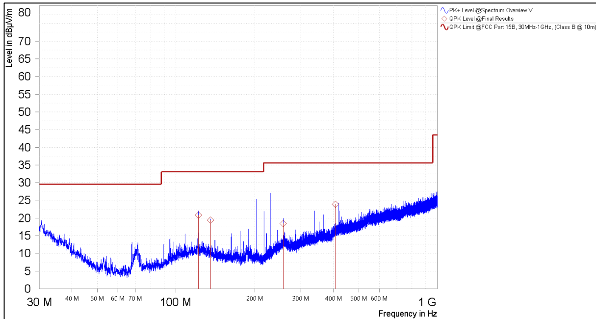
Figure 8. Spurious Emissions 30MHz – 1GHz, (Terminal, Vertical Polarity)
