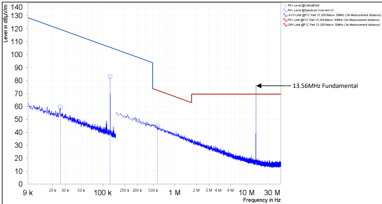
Figure 10. Spurious Emissions Below 30MHz, (Pigtail, Coplanar Loop 6 )
