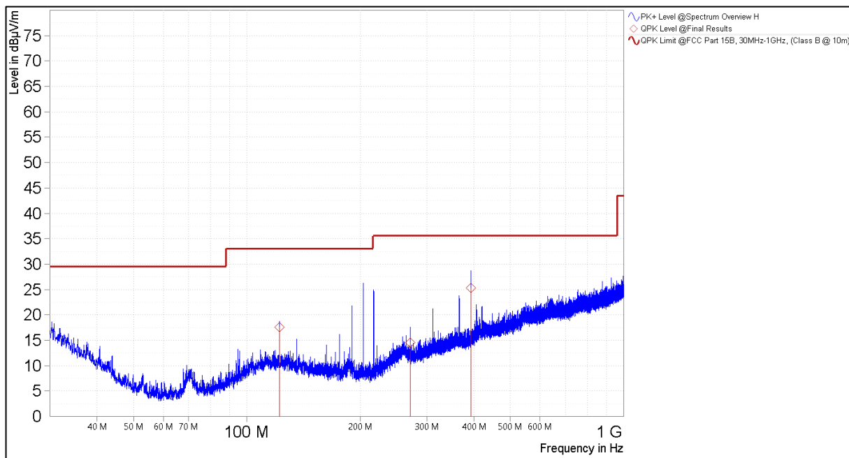
Figure 9. Spurious Emissions 30MHz – 1GHz, (Terminal, Horizontal Polarity)
