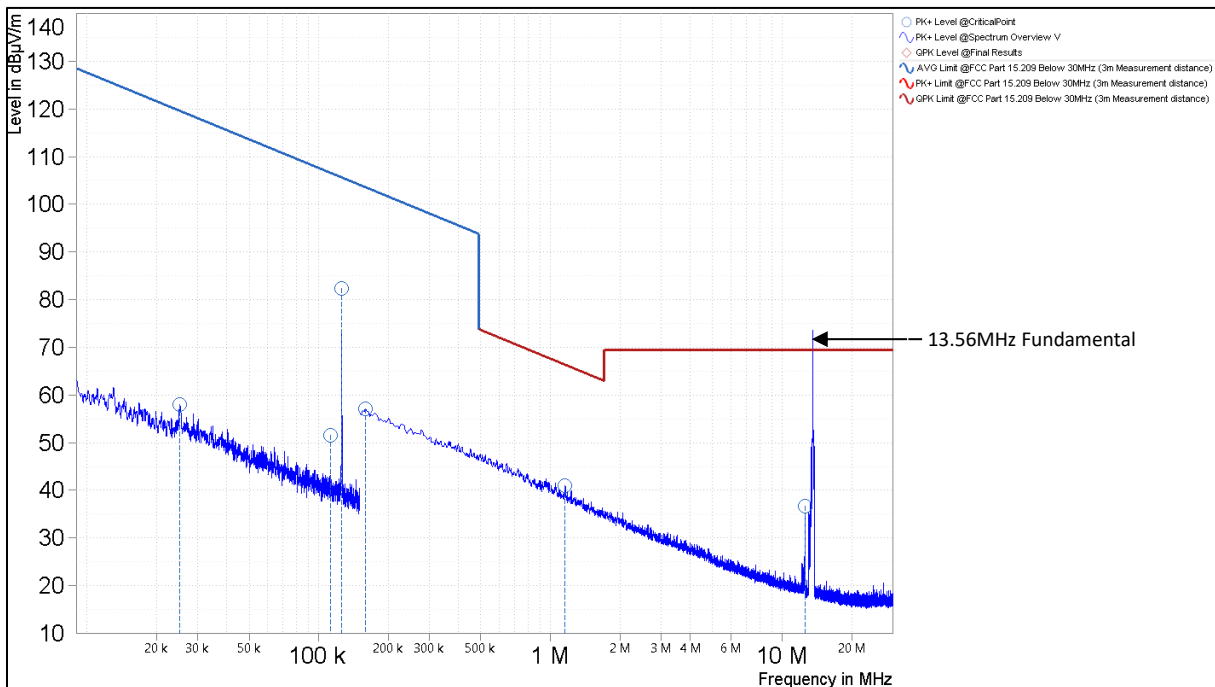
Figure 7. Spurious Emissions Below 30MHz, (Terminal, Coaxial Loop 5 )
