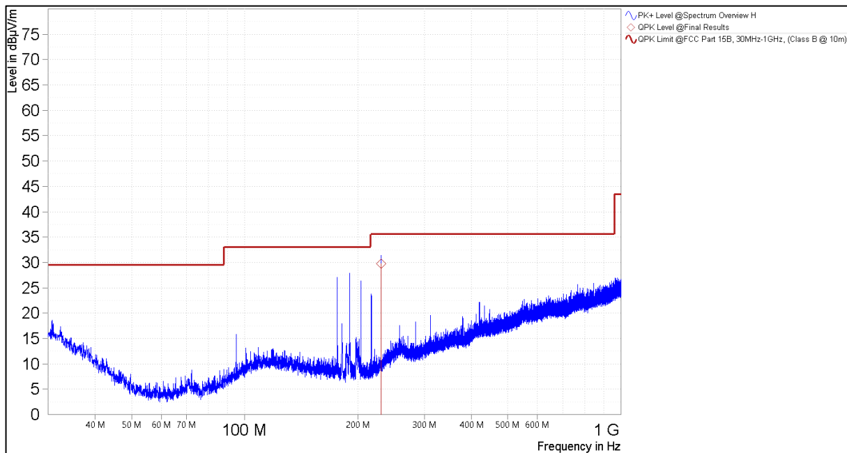
Figure 13. Spurious Emissions 30MHz – 1GHz, (Pigtail, Horizontal Polarity)
