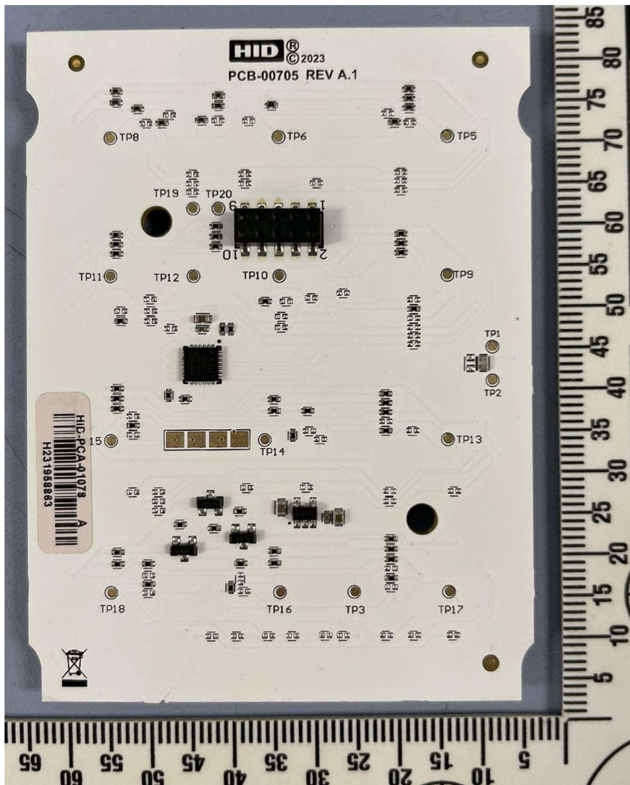
Keypad board reverse
