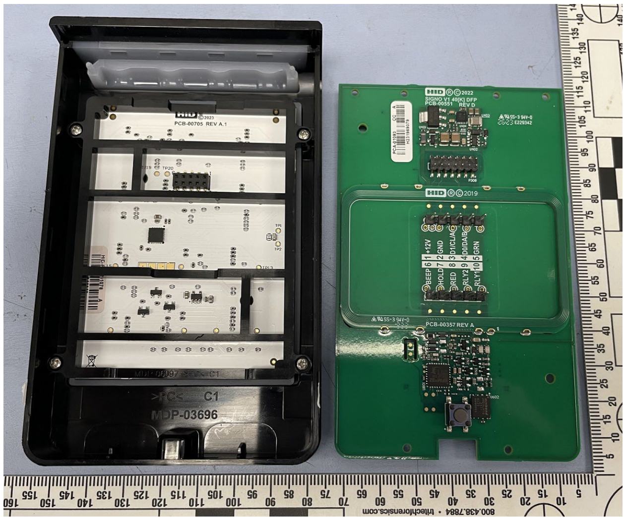
Main board removed
