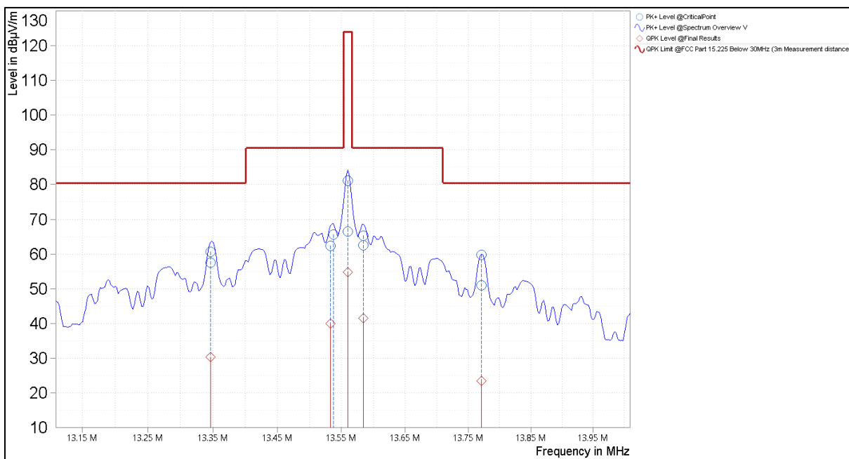
Figure 19. In-Band Emission Mask (Coaxial Loop, Pluggable Pigtail)
