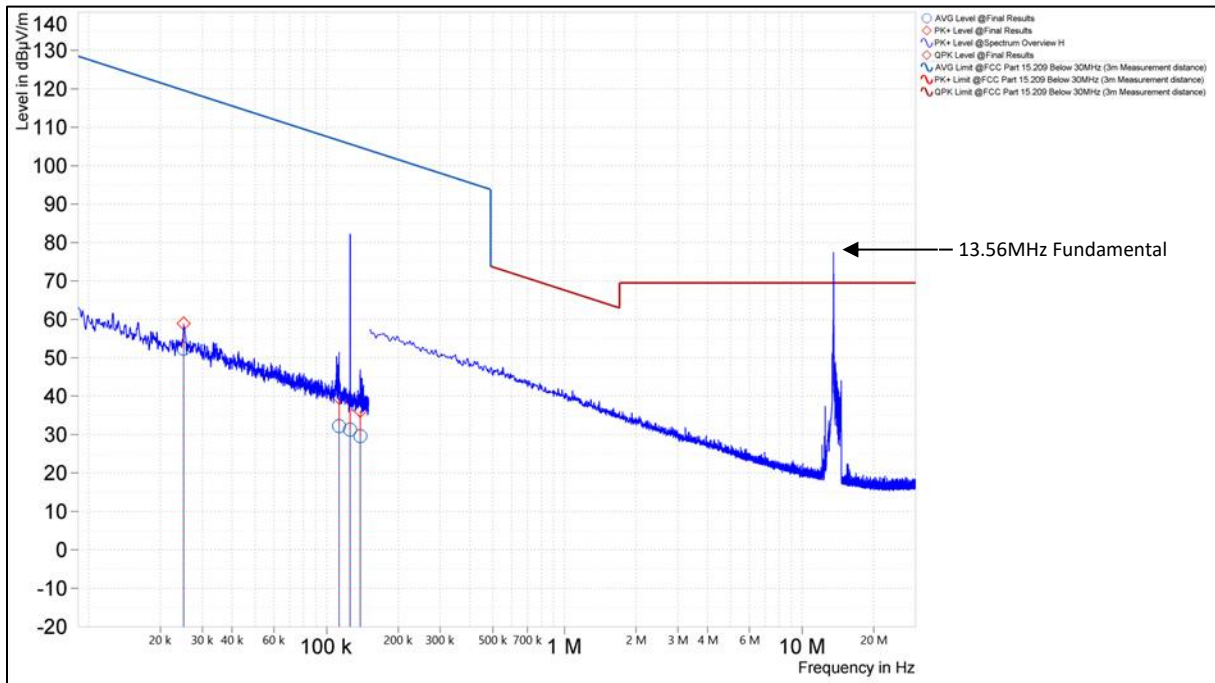
Figure 14. Out of Band Emissions Below 30MHz (Coplanar Loop, Terminal)
