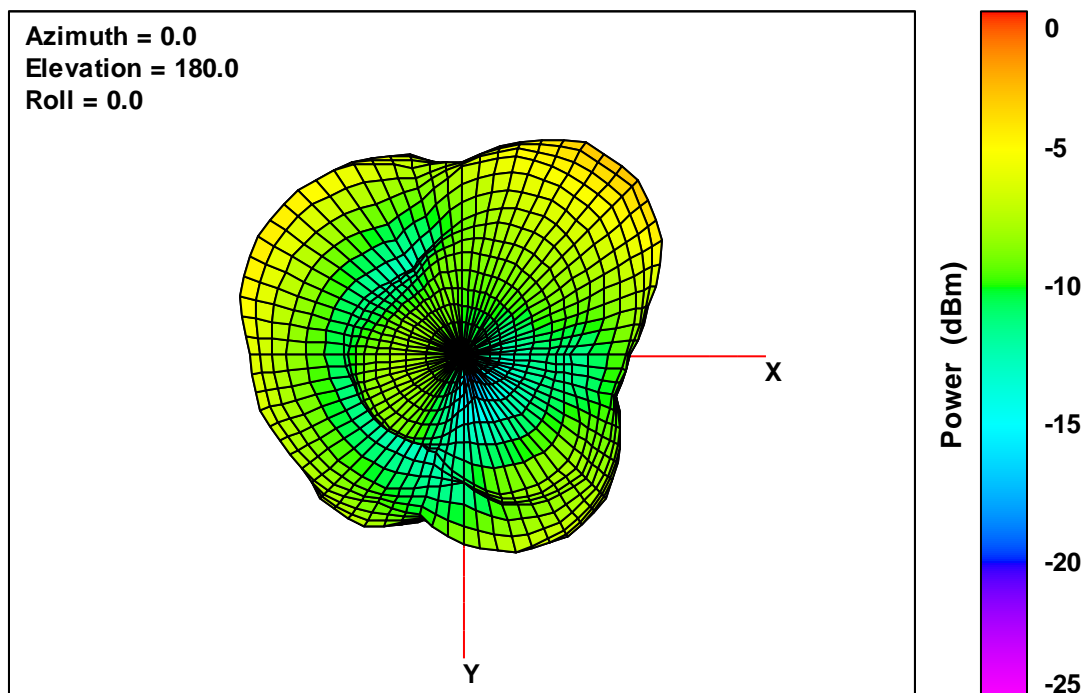
40K V2 Free-Space Total EIRP, Bottom View, 2482 MHz
