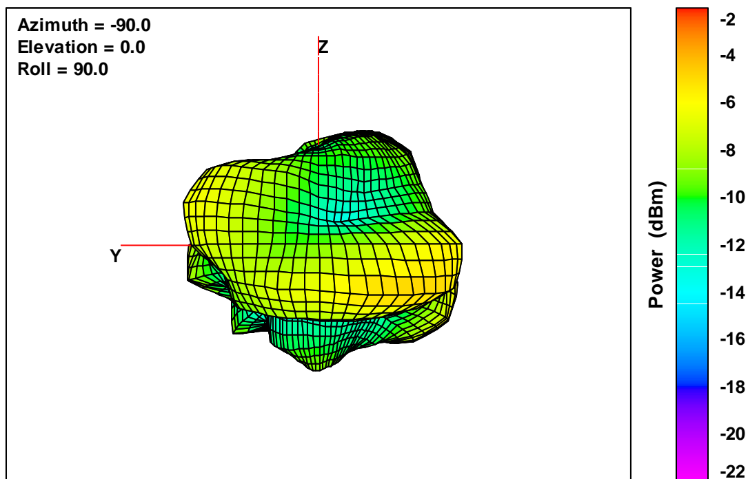
40K V2 Free-Space Total EIRP, Back Face View, 2442 MHz
