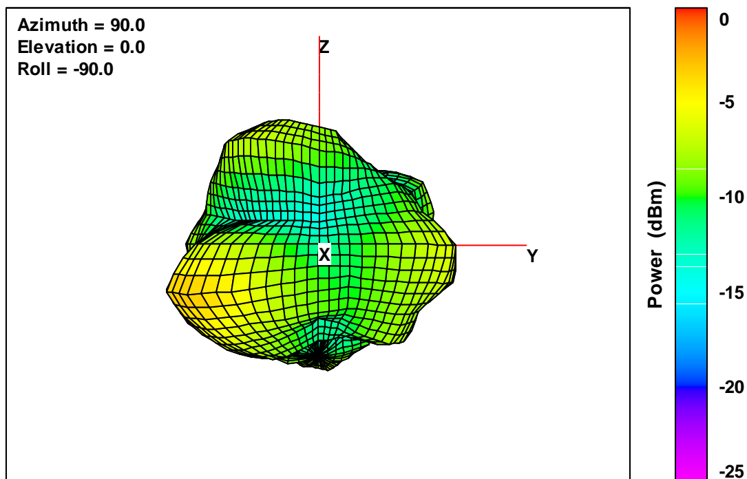
40K V2 Free-Space Total EIRP, Front Face View, 2482 MHz
