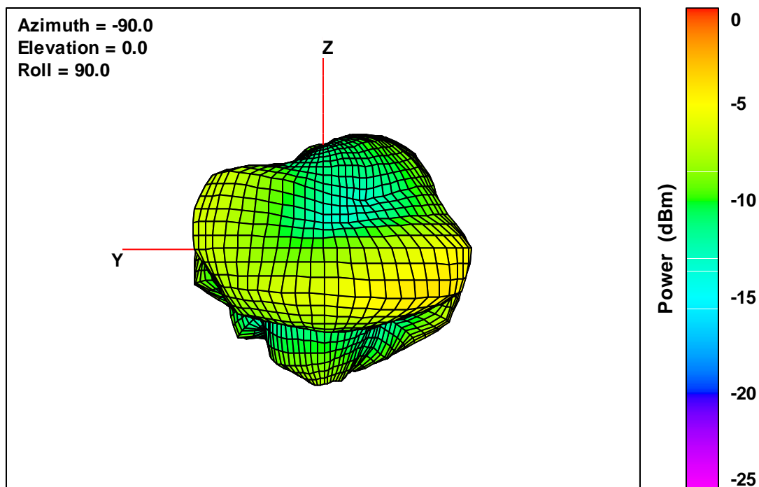
40K V2 Free-Space Total EIRP, Back Face View, 2482 MHz
