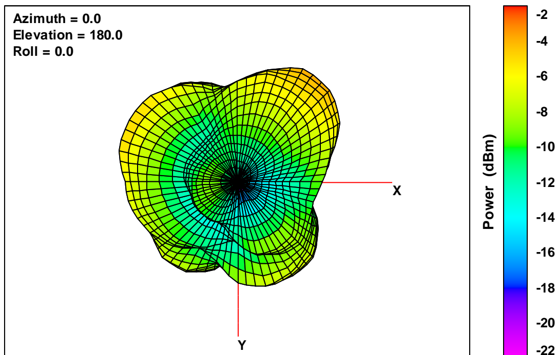
40K V2 Free-Space Total EIRP, Bottom View, 2442 MHz
