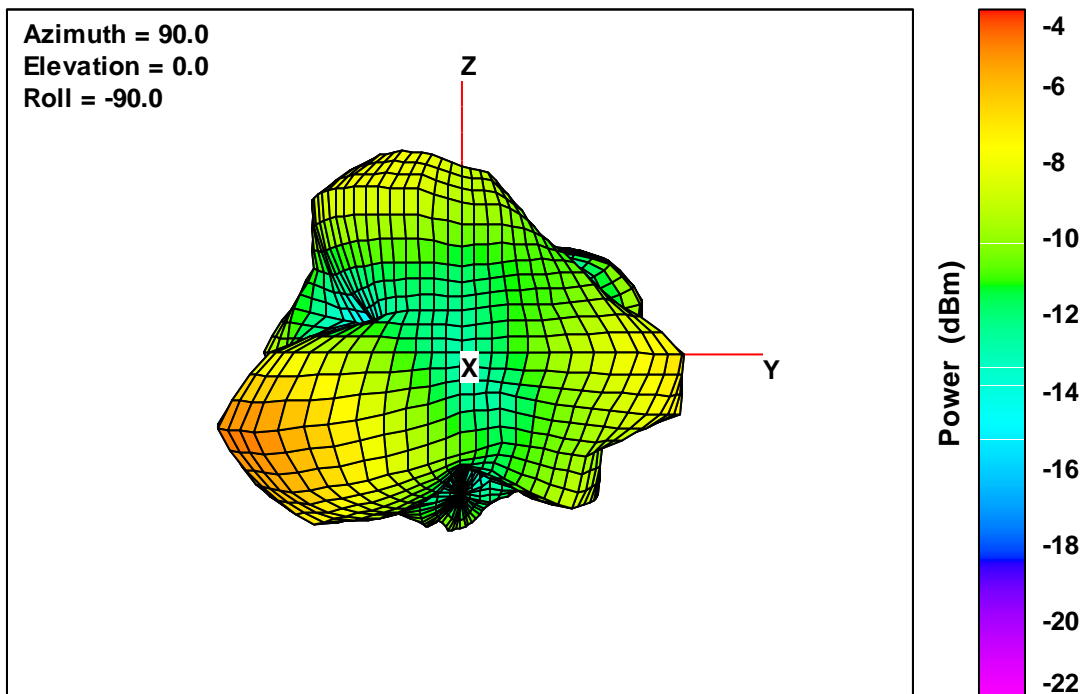
40K V2 Free-Space Total EIRP, Front Face View, 2402 MHz
