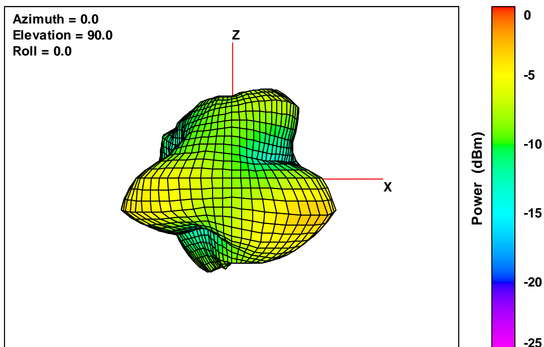
40K V2 Free-Space Total EIRP, Left Side View, 2482 MHz
