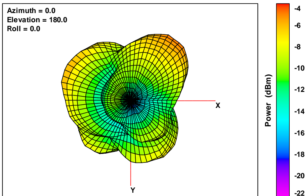
40K V2 Free-Space Total EIRP, Bottom View, 2402 MHz
