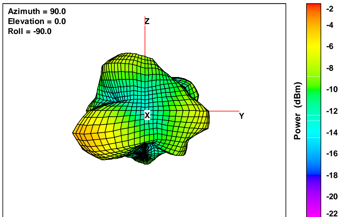
40K V2 Free-Space Total EIRP, Front Face View, 2442 MHz
