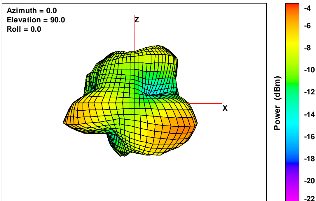
40K V2 Free-Space Total EIRP, Left Side View, 2402 MHz
