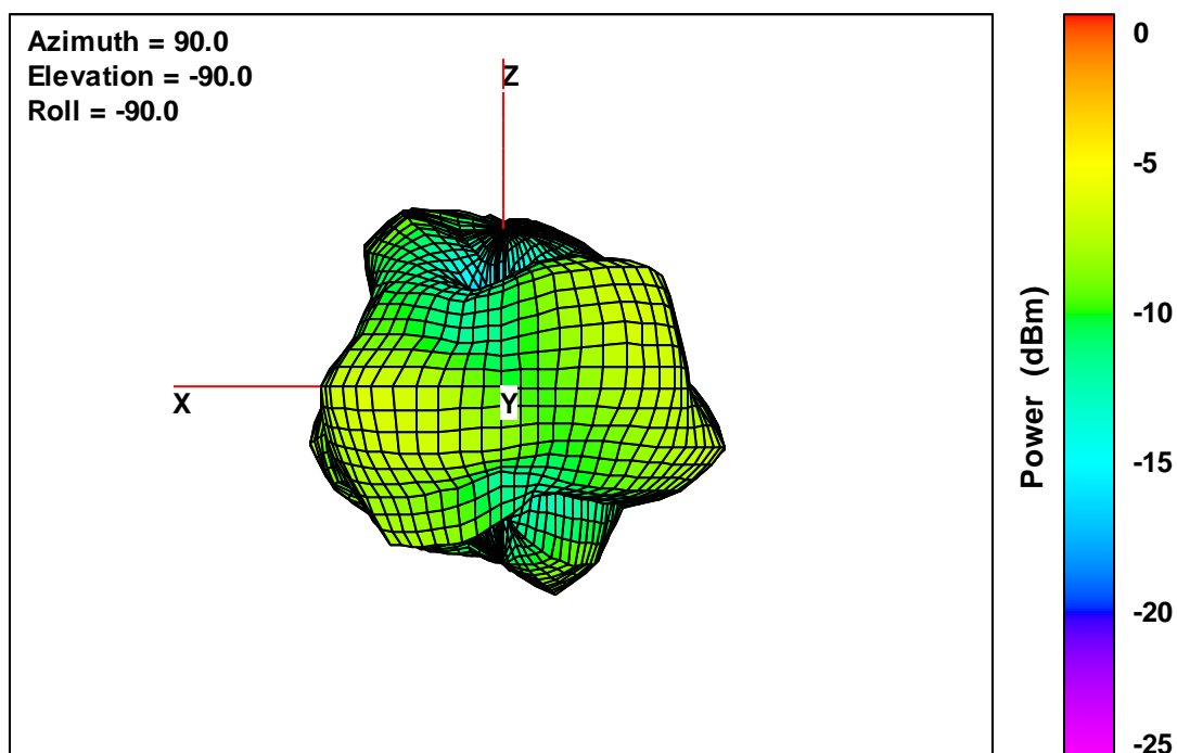
40K V2 Free-Space Total EIRP, Right Side View, 2482 MHz
