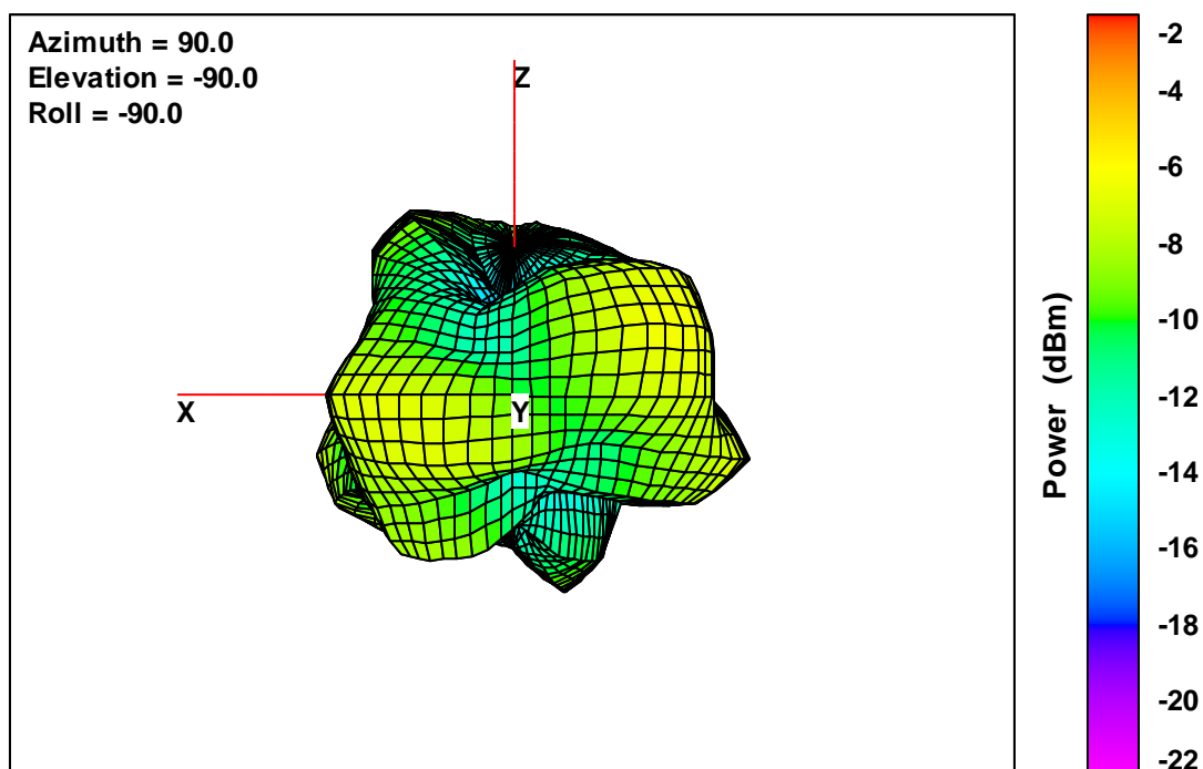
40K V2 Free-Space Total EIRP, Right Side View, 2442 MHz
