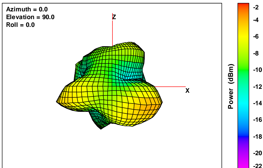
40K V2 Free-Space Total EIRP, Left Side View, 2442 MHz
