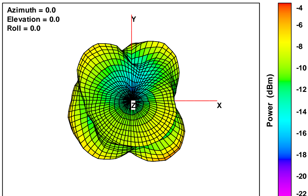
40K V2 Free-Space Total EIRP, Top View, 2402 MHz
