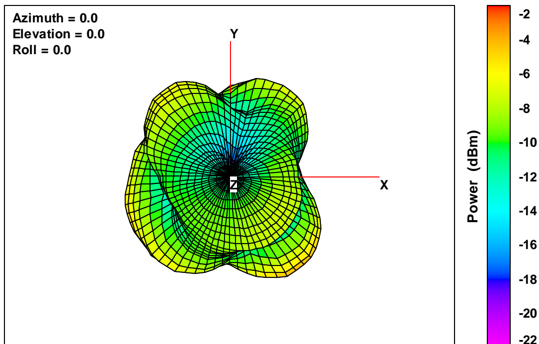
40K V2 Free-Space Total EIRP, Top View, 2442 MHz
