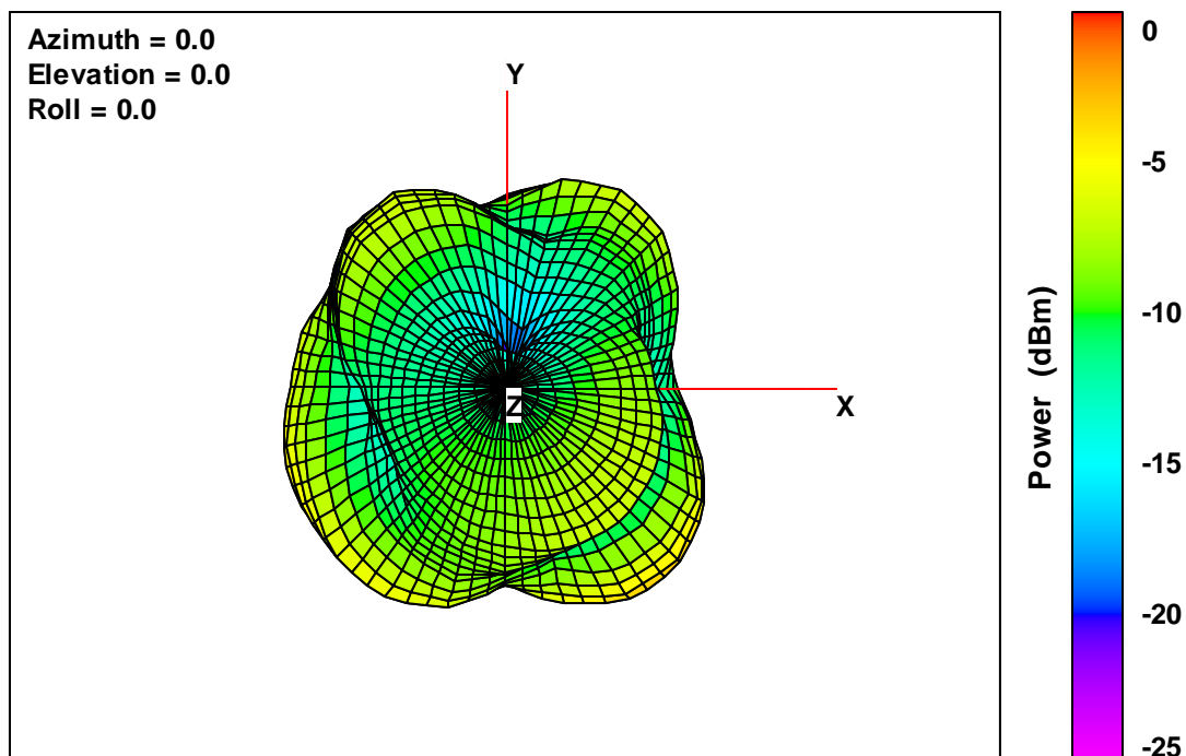
40K V2 Free-Space Total EIRP, Top View, 2482 MHz
