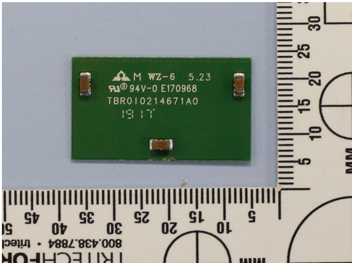
Model 40K (pigtail version) patch antenna reverse
