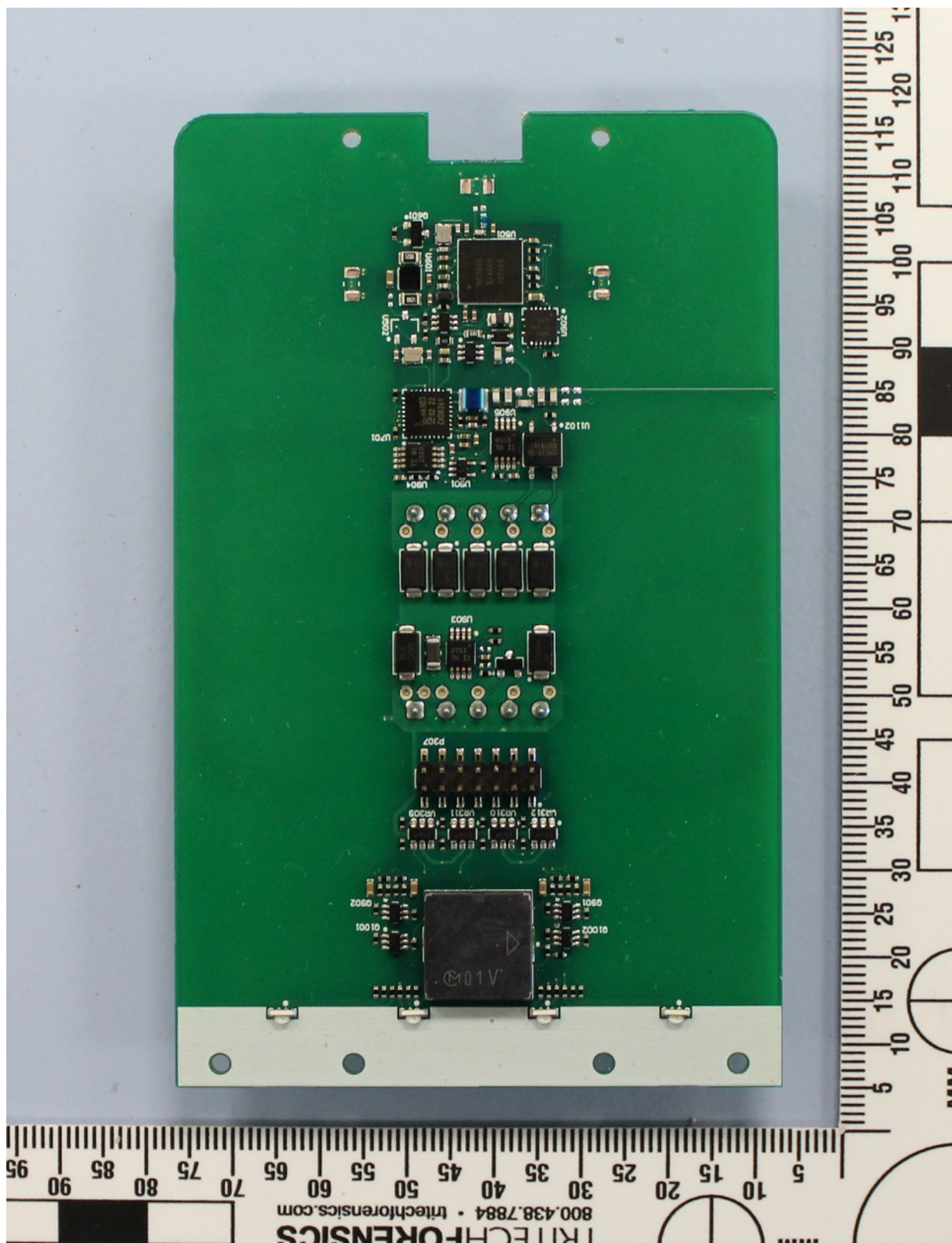
Model 40K (pigtail version) main board obverse without patch antenna
