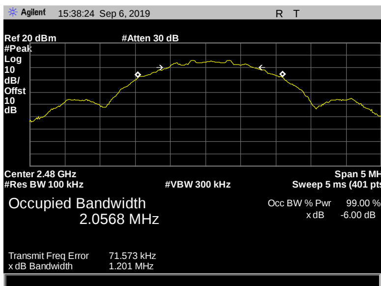
Figure 32: 6 dB Bandwidth, Terminal, 2480 MHz, 2 Mbps, 1.201 MHz
