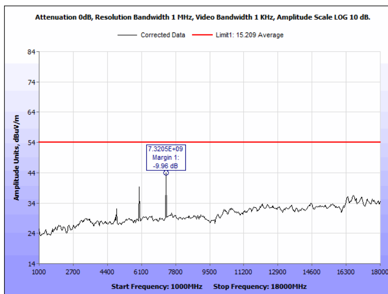
Figure 96: Radiated Spurious Emissions, Terminal, 2442 MHz, 1 GHz - 18 GHz, Average, Vertical
