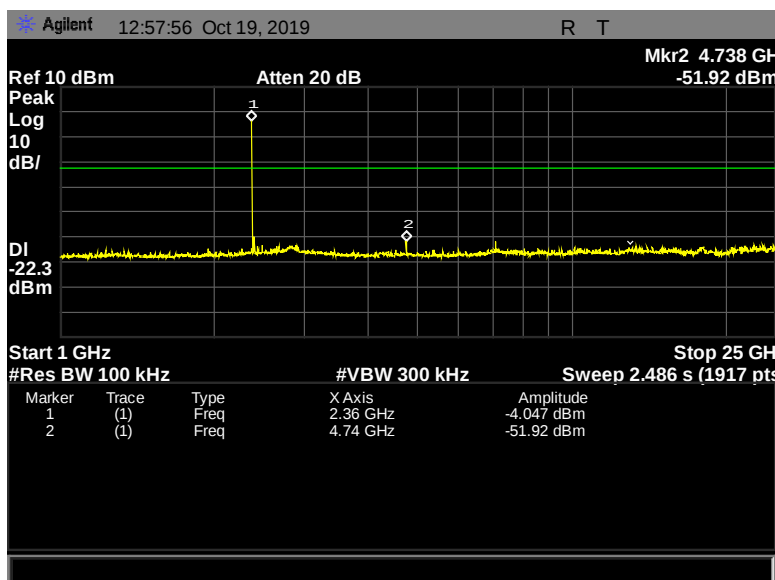
Figure 128: Conducted Spurious Emissions, Pigtail, 2402 MHz, 2 Mbps, 1 GHz - 25 GHz
