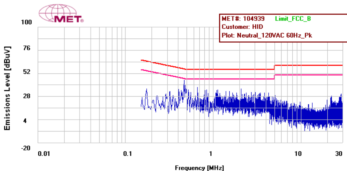
Figure 17: Conducted Emissions Limits, Terminal, Neutral Line, Prescan
