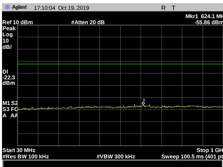
Figure 131: Conducted Spurious Emissions, Pigtail, 2442 MHz, 2 Mbps, 30 MHz - 1000 MHz
