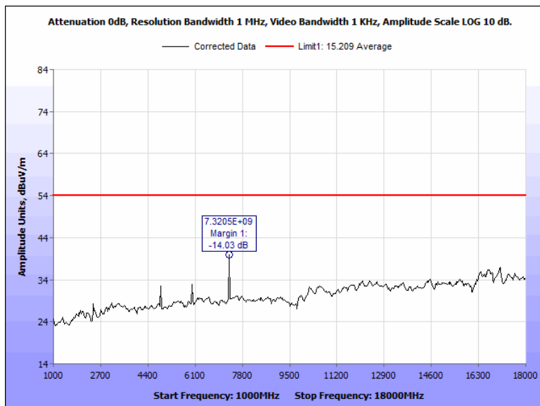
Figure 95: Radiated Spurious Emissions, Terminal, 2442 MHz, 1 GHz - 18 GHz, Average, Horizontal
