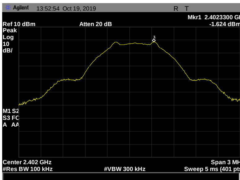
Figure 166: Peak Power Spectral Density, Terminal, 2402 MHz, 1 Mbps, -1.624 dBm
