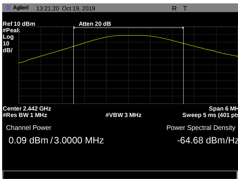
Figure 45: Peak Power Output, Terminal, 2442 MHz, 1 Mbps, 0.09 dBm
