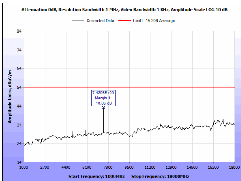
Figure 103: Radiated Spurious Emissions, Terminal, 2480 MHz, 1 GHz - 18 GHz, Average, Horizontal
