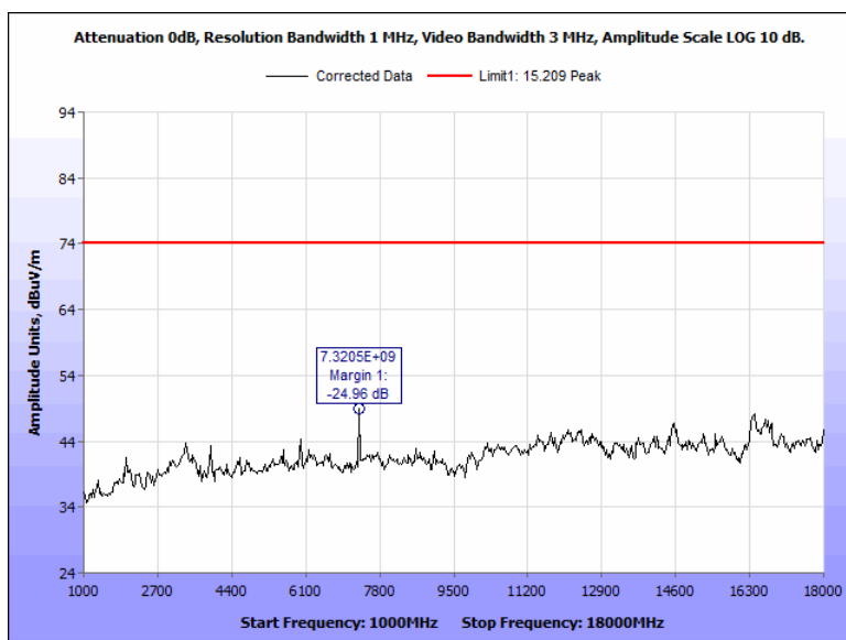
Figure 99: Radiated Spurious Emissions, Terminal, 2442 MHz, 1 GHz - 18 GHz, Peak, Vertical
