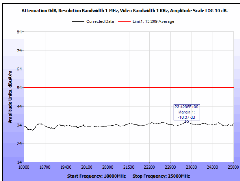
Figure 89: Radiated Spurious Emissions, Terminal, 2402 MHz, 18 GHz - 25 GHz, Average, Vertical
