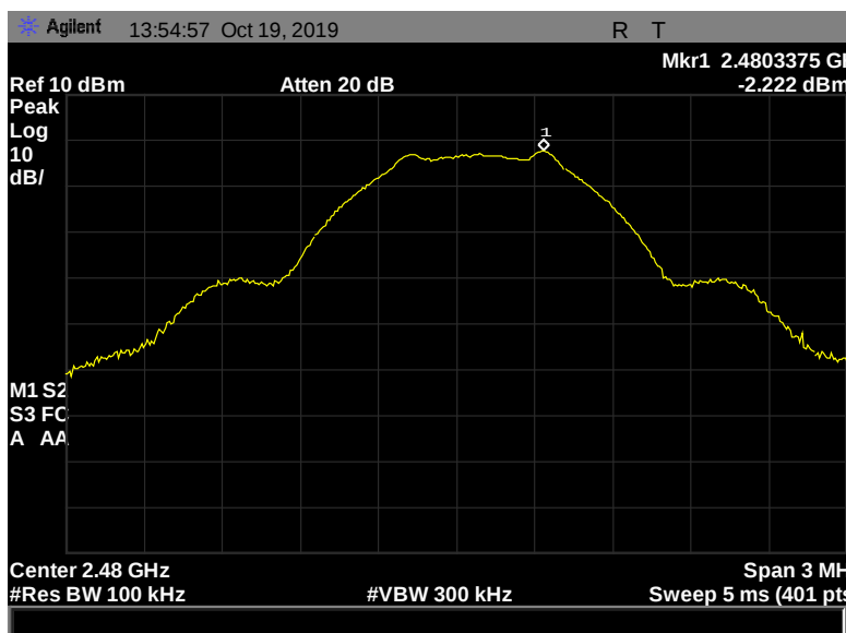
Figure 170: Peak Power Spectral Density, Terminal, 2480 MHz, 1 Mbps, -2.222 dBm
