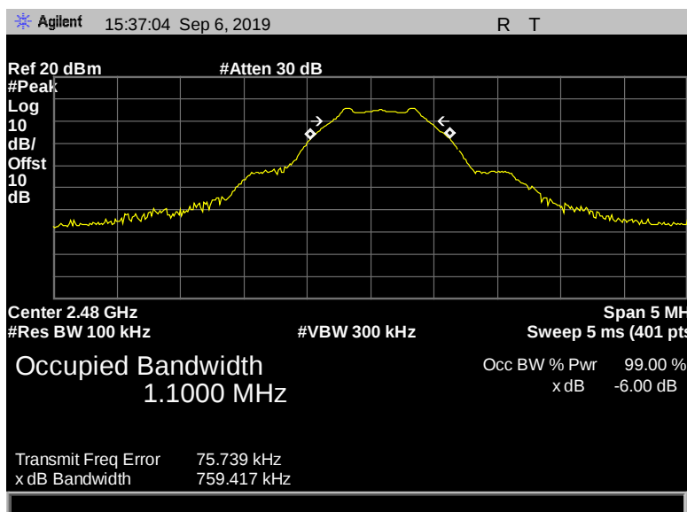
Figure 31: 6 dB Bandwidth, Terminal, 2480 MHz, 1 Mbps, 759.417 kHz
