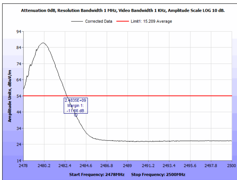
Figure 112: Radiated Band Edge, Pigtail, 2480 MHz, Average, Horizontal
