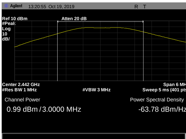
Figure 46: Peak Power Output, Terminal, 2442 MHz, 2 Mbps, 0.99 dBm
