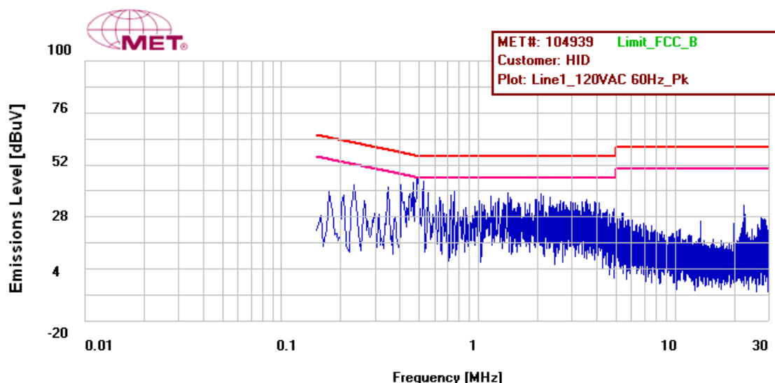
Figure 15: Conducted Emissions Limits, Terminal, Phase Line, Prescan
