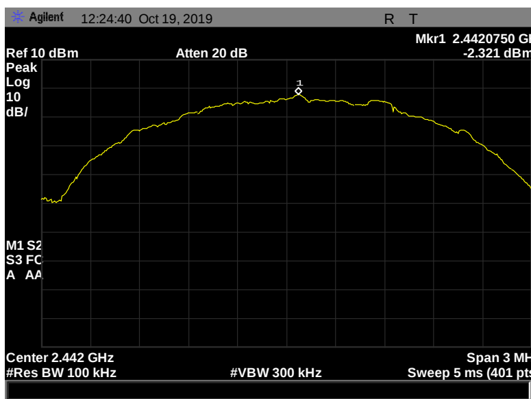
Figure 162: Peak Power Spectral Density, Pigtail, 2442 MHz, 2 Mbps, -2.321 dBm
