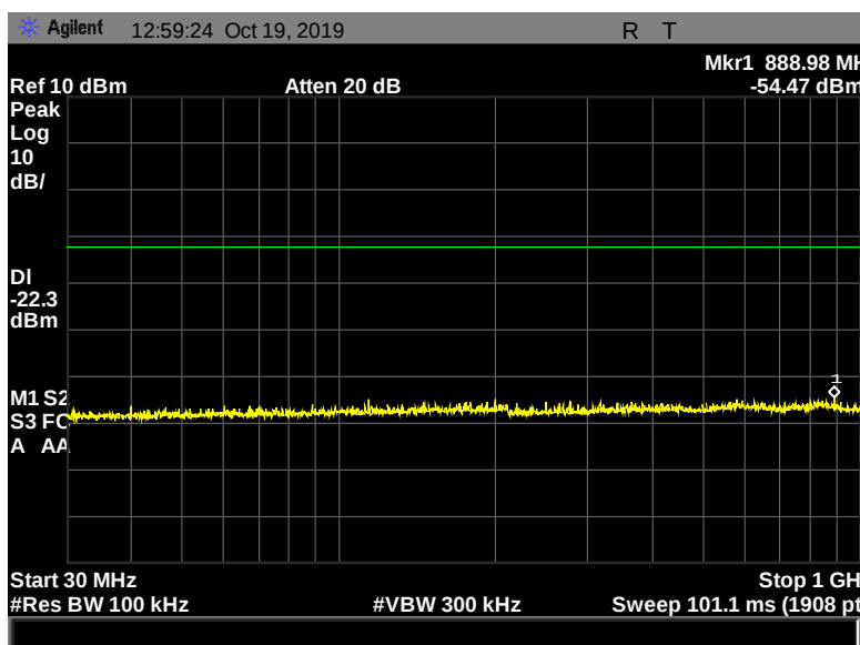
Figure 127: Conducted Spurious Emissions, Pigtail, 2402 MHz, 2 Mbps, 30 MHz - 1000 MHz
