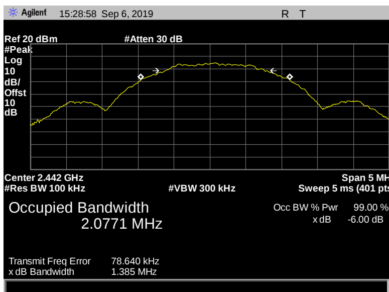
Figure 30: 6 dB Bandwidth, Terminal, 2442 MHz, 2 Mbps, 1.385 MHz
