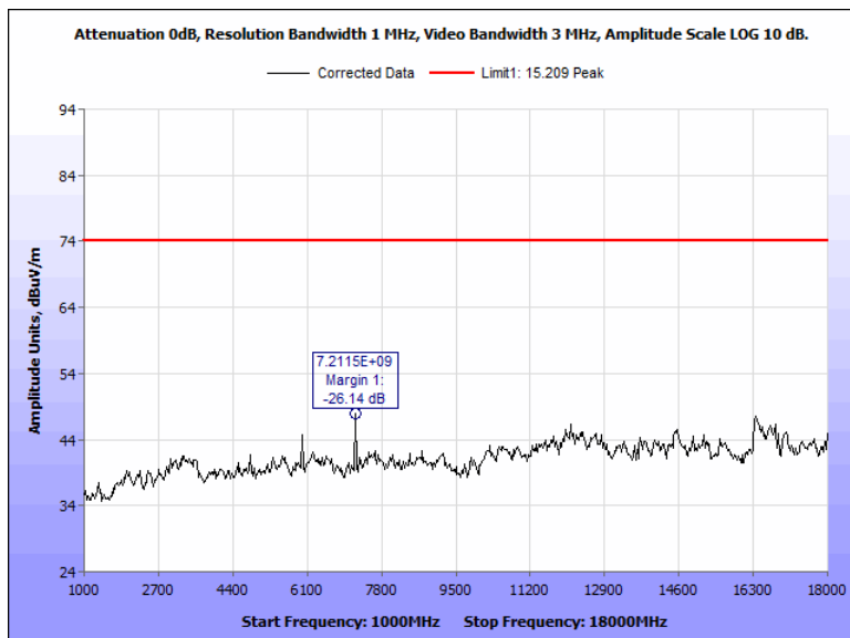
Figure 86: Radiated Spurious Emissions, Terminal, 2402 MHz, 1 GHz - 18 GHz, Peak, Horizontal
