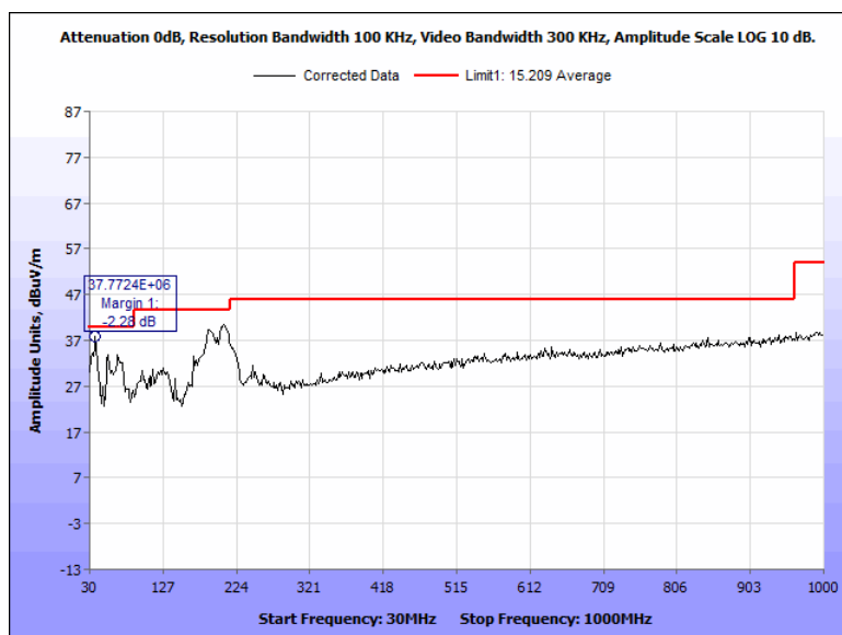
Figure 65: Radiated Spurious Emissions, Pigtail, 2442 MHz, 30 MHz - 1000 MHz, Vertical
