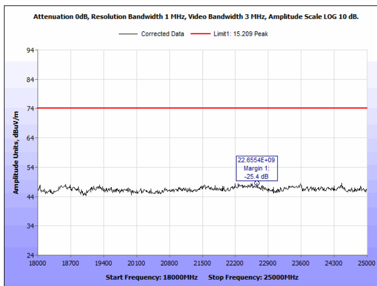
Figure 63: Radiated Spurious Emissions, Pigtail, 2402 MHz, 18 GHz - 25 GHz, Peak, Vertical
