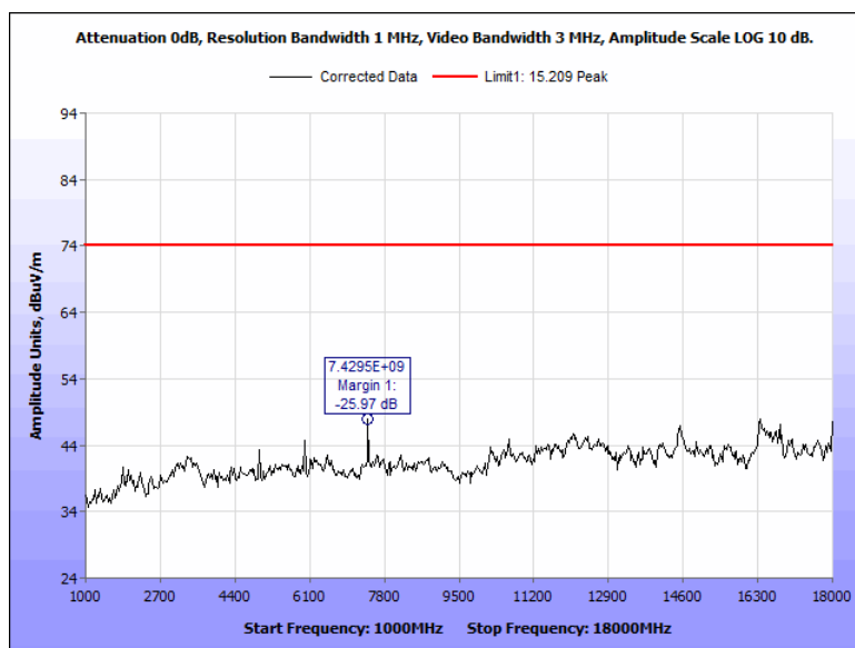
Figure 79: Radiated Spurious Emissions, Pigtail, 2480 MHz, 1 GHz - 18 GHz, Peak, Vertical
