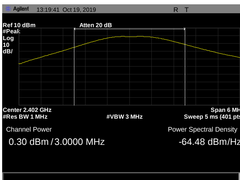
Figure 43: Peak Power Output, Terminal, 2402 MHz, 1 Mbps, 0.30 dBm
