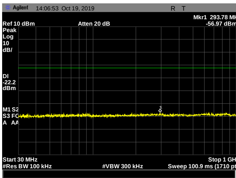
Figure 149: Conducted Spurious Emissions, Terminal, 2480 MHz, 1 Mbps, 30 MHz- 1000 MHz
