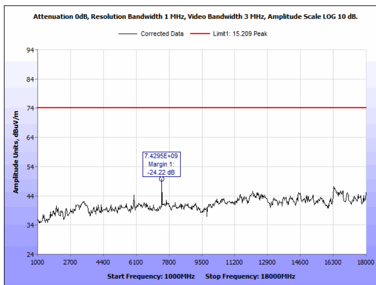
Figure 107: Radiated Spurious Emissions, Terminal, 2480 MHz, 1 GHz - 18 GHz, Peak, Vertical
