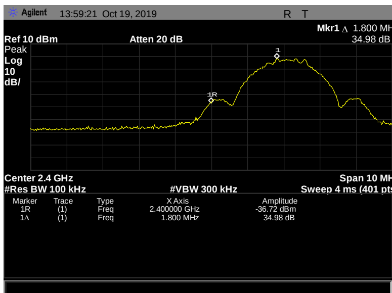
Figure 154: Conducted Band Edge, Terminal, 2402 MHz, 2 Mbps
