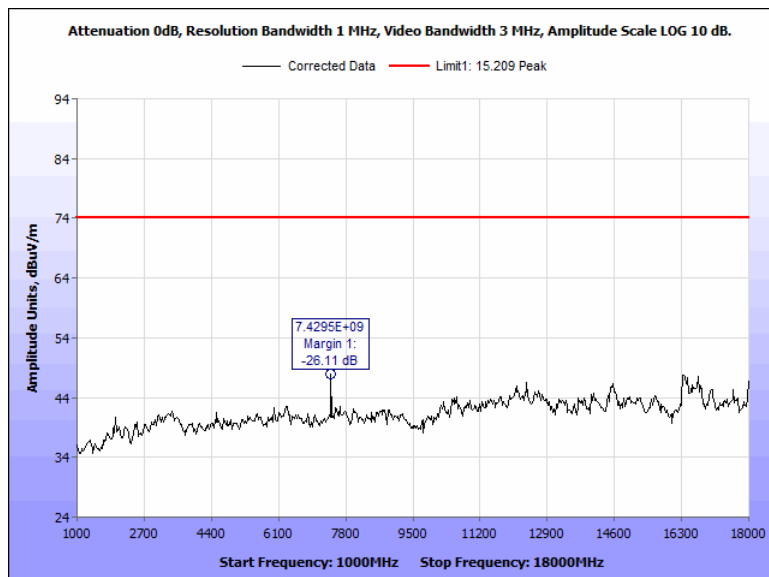
Figure 106: Radiated Spurious Emissions, Terminal, 2480 MHz, 1 GHz - 18 GHz, Peak, Horizontal
