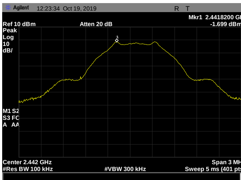
Figure 161: Peak Power Spectral Density, Pigtail, 2442 MHz, 1 Mbps, -1.699 dBm
