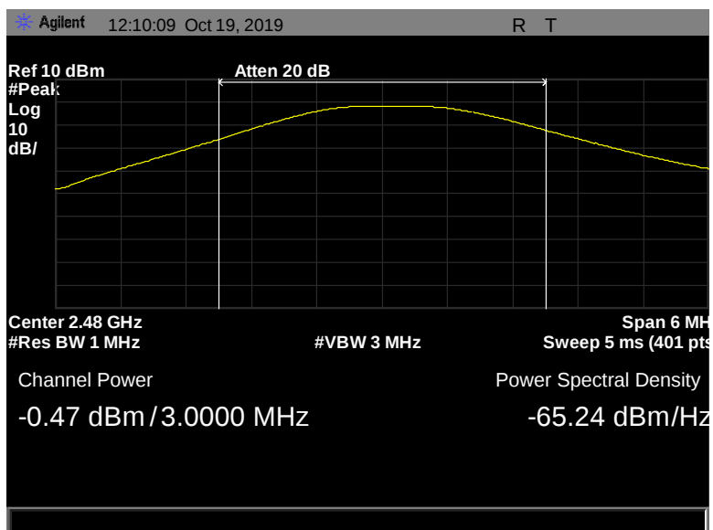
Figure 40: Peak Power Output, Pigtail, 2480 MHz, 1 Mbps, -0.47 dBm
