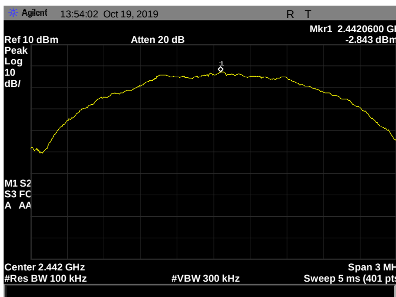
Figure 169: Peak Power Spectral Density, Terminal, 2442 MHz, 2 Mbps, -2.843 dBm
