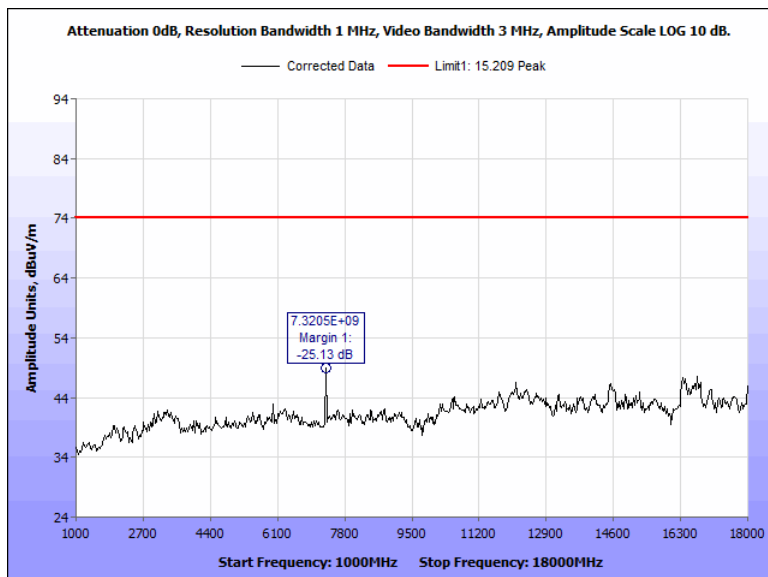
Figure 98: Radiated Spurious Emissions, Terminal, 2442 MHz, 1 GHz - 18 GHz, Peak, Horizontal
