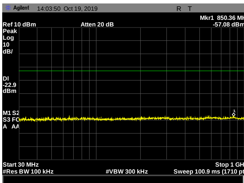
Figure 145: Conducted Spurious Emissions, Terminal, 2442 MHz, 1 Mbps, 30 MHz – 1000 MHz
