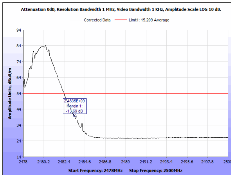
Figure 113: Radiated Band Edge, Pigtail, 2480 MHz, Average, Vertical
