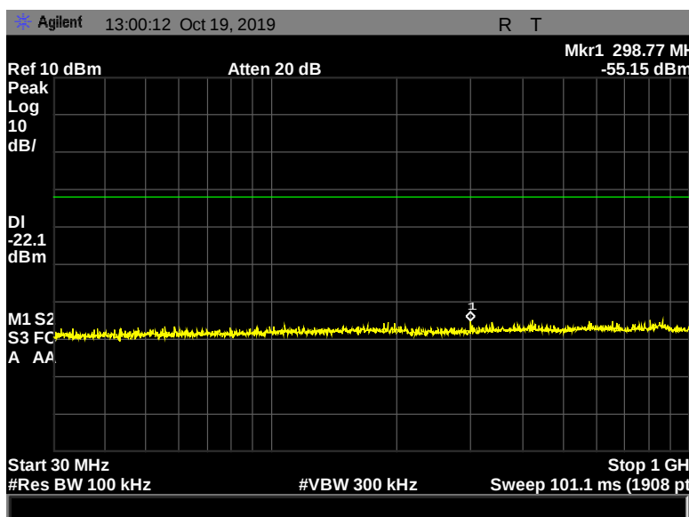
Figure 133: Conducted Spurious Emissions, Pigtail, 2480 MHz, 1 Mbps, 30 MHz - 1000 MHz
