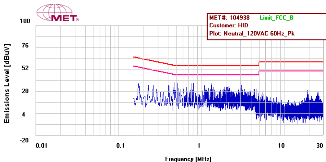
Figure 13: Conducted Emissions Limits, Terminal, Neutral Line, Prescan
