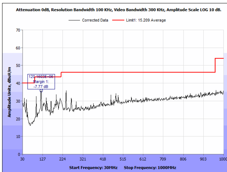
Figure 80: Radiated Spurious Emissions, Terminal, 2402 MHz, 30 MHz - 1000 MHz, Horizontal
