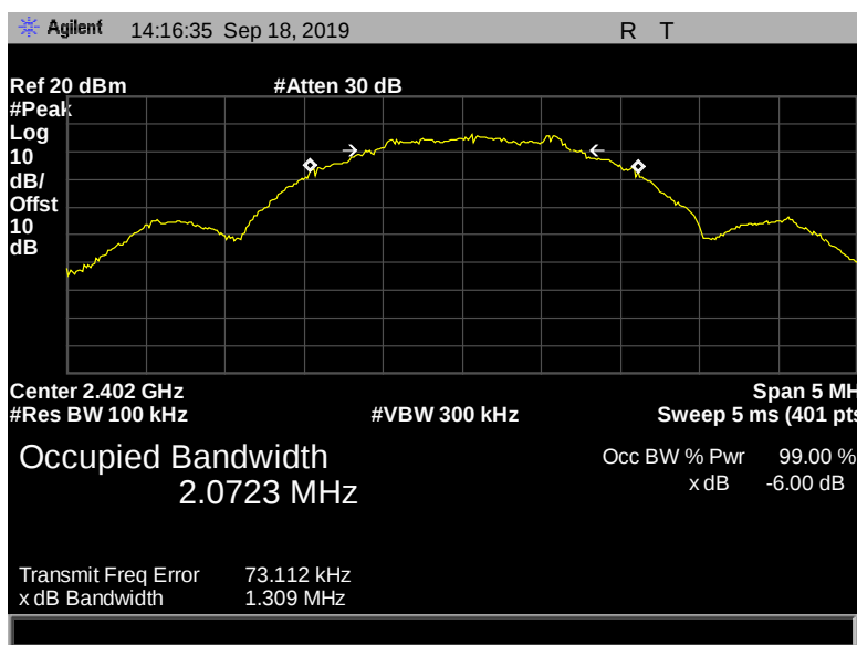
Figure 21: 6 dB Bandwidth, Pigtail, 2402 MHz, 2 Mbps, 1.309 MHz
