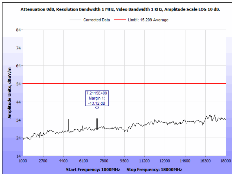
Figure 83: Radiated Spurious Emissions, Terminal, 2402 MHz, 1 GHz - 18 GHz, Average, Horizontal
