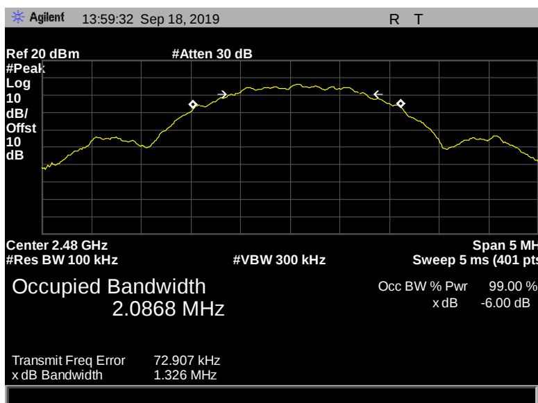
Figure 25: 6 dB Bandwidth, Pigtail, 2480 MHz, 2 Mbps, 1.326 MHz
