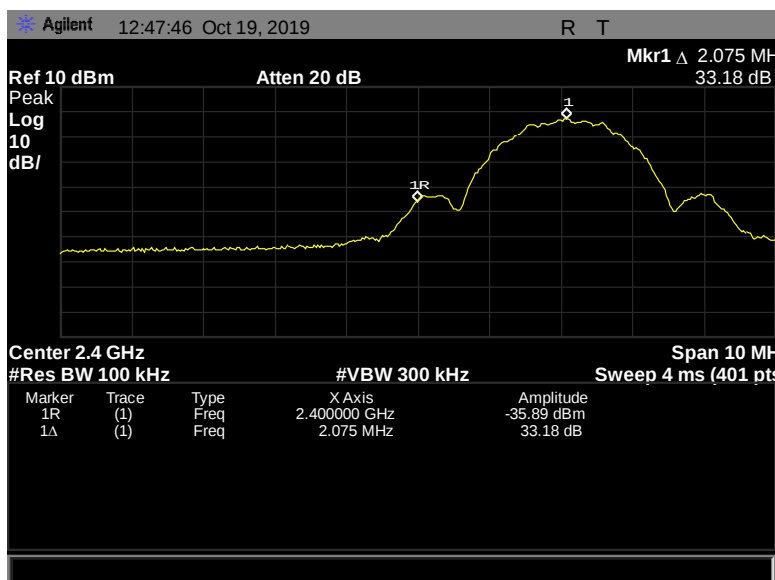
Figure 138: Conducted Band Edge, Pigtail, 2402 MHz, 2 Mbps
