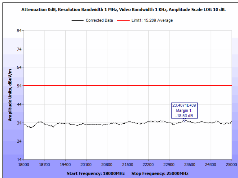
Figure 88: Radiated Spurious Emissions, Terminal, 2402 MHz, 18 GHz - 25 GHz, Average, Horizontal
