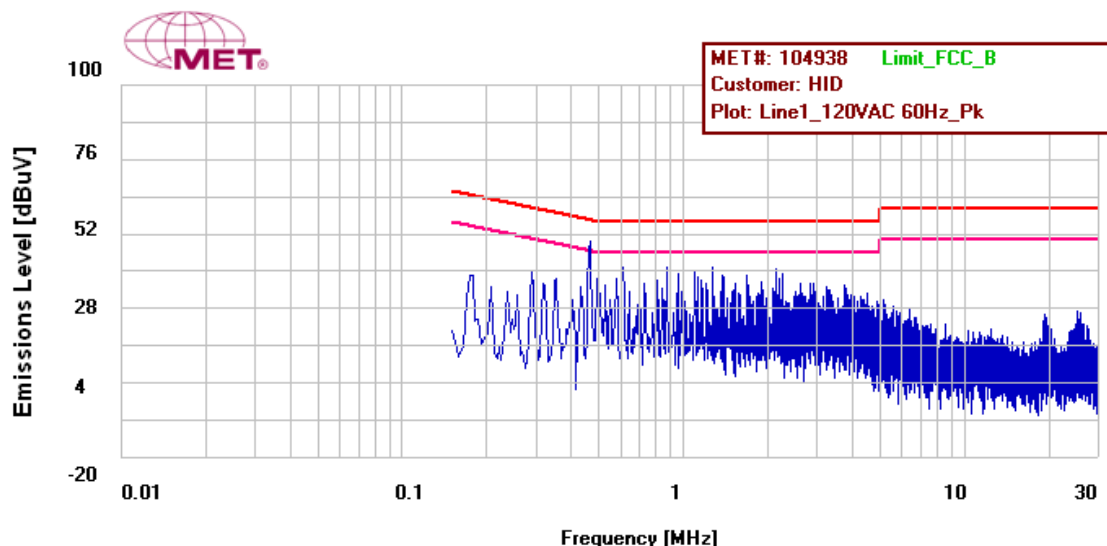
Figure 11: Conducted Emissions Limits, Pigtail, Phase Line, Prescan
