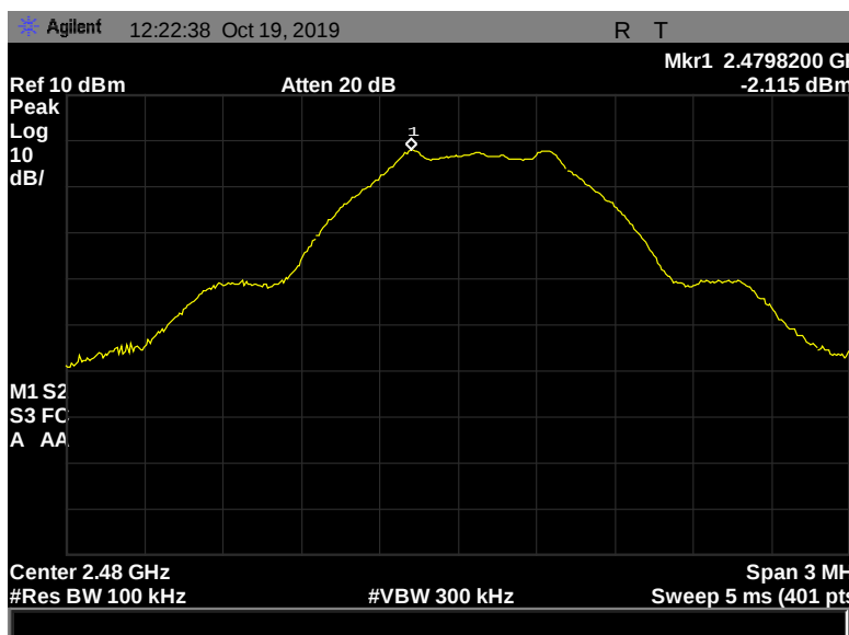
Figure 163: Peak Power Spectral Density, Pigtail, 2480 MHz, 1 Mbps, -2.115 dBm
