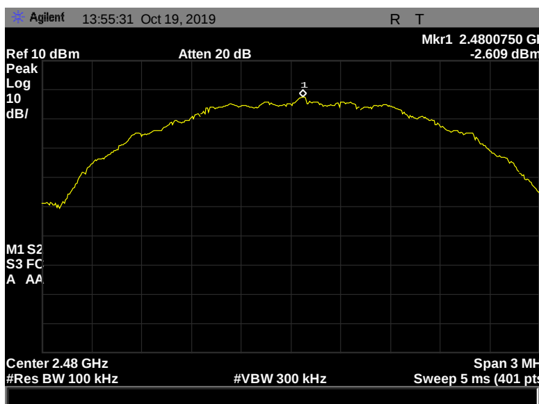
Figure 171: Peak Power Spectral Density, Terminal, 2480 MHz, 2 Mbps, -2.609 dBm
