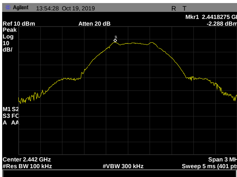
Figure 168: Peak Power Spectral Density, Terminal, 2442 MHz, 1 Mbps, -2.288 dBm
