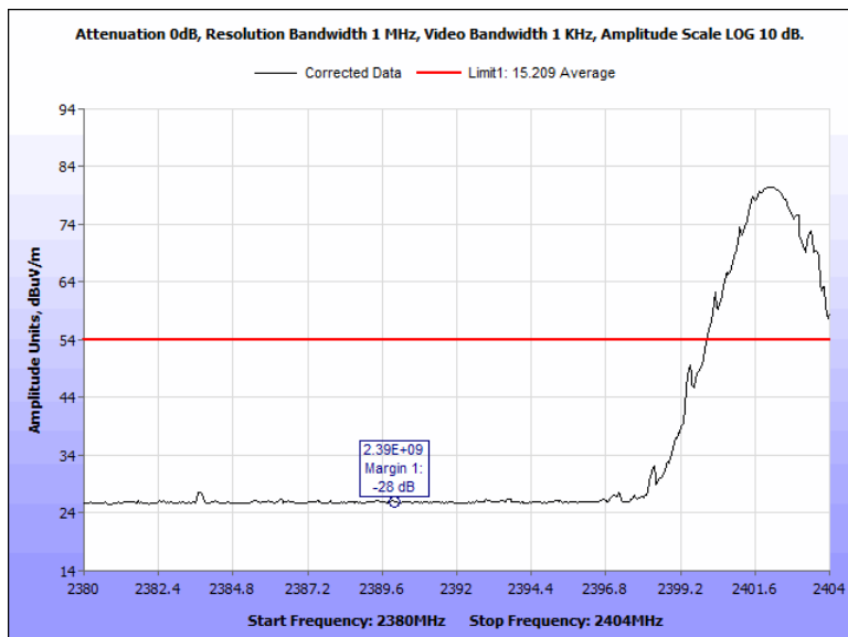
Figure 109: Radiated Band Edge, Pigtail, 2402 MHz, Average, Vertical
