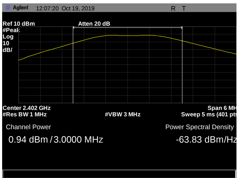
Figure 37: Peak Power Output, Pigtail, 2402 MHz, 2 Mbps, 0.94 dBm
