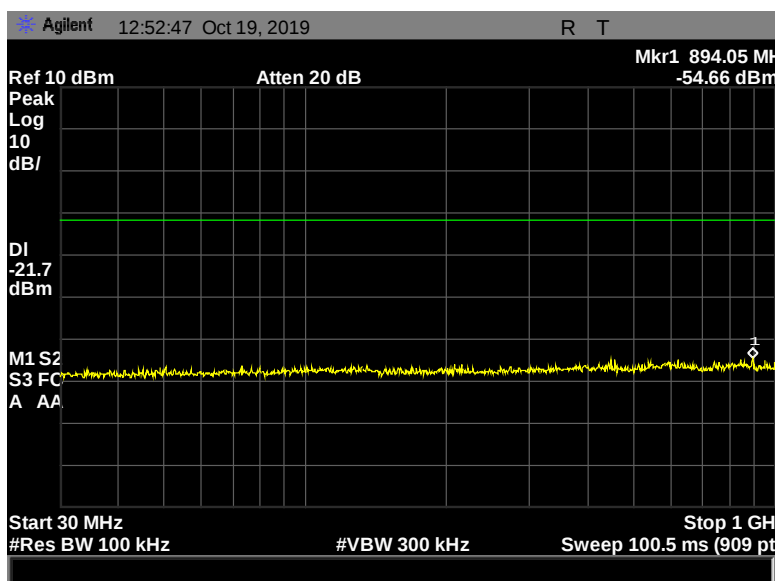
Figure 129: Conducted Spurious Emissions, Pigtail, 2442 MHz, 1 Mbps, 30 MHz - 1000 MHz
