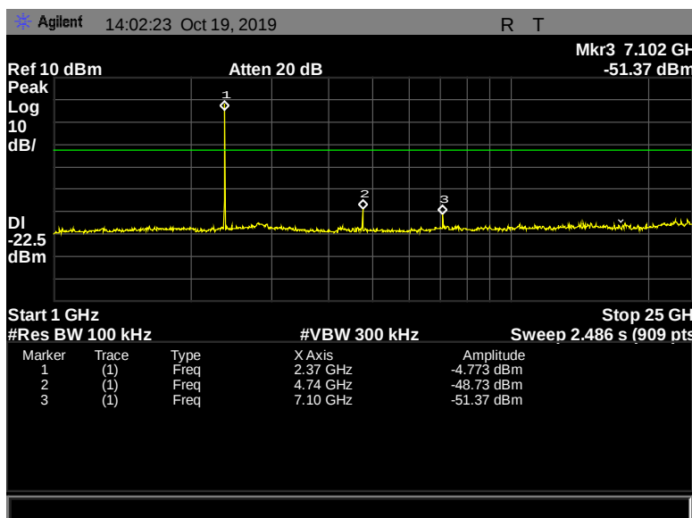
Figure 144: Conducted Spurious Emissions, Terminal, 2402 MHz, 2 Mbps, 1 GHz – 25 GHz
