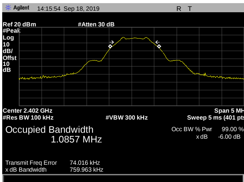
Figure 20: 6 dB Bandwidth, Pigtail, 2402 MHz, 1 Mbps, 759.963 kHz
