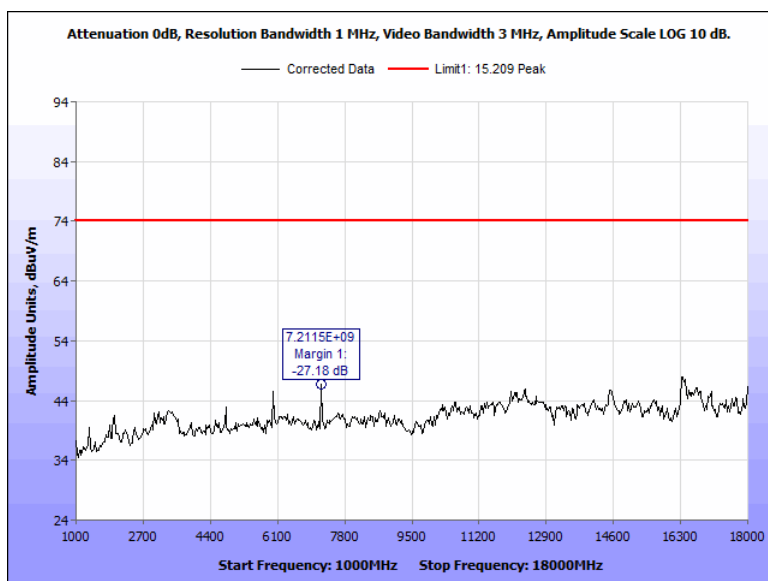
Figure 87: Radiated Spurious Emissions, Terminal, 2402 MHz, 1 GHz - 18 GHz, Peak, Vertical
