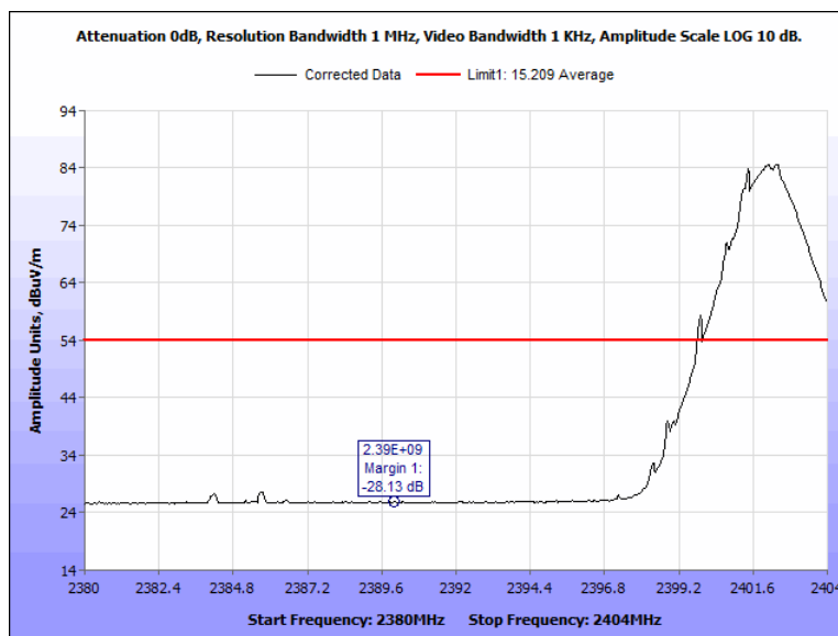
Figure 108: Radiated Band Edge, Pigtail, 2402 MHz, Average, Horizontal
