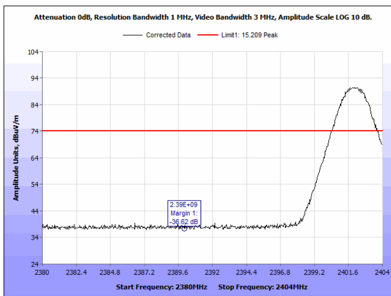
Figure 110: Radiated Band Edge, Pigtail, 2402 MHz, Peak, Horizontal
