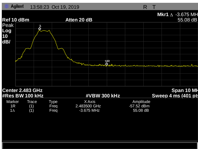
Figure 155: Conducted Band Edge, Terminal, 2480 MHz, 1 Mbps
