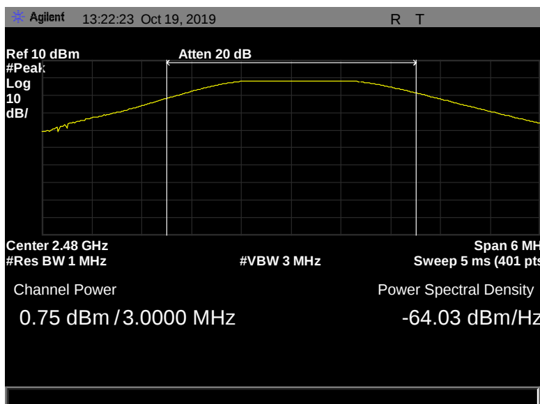
Figure 48: Peak Power Output, Terminal, 2480 MHz, 2 Mbps, 0.75 dBm
