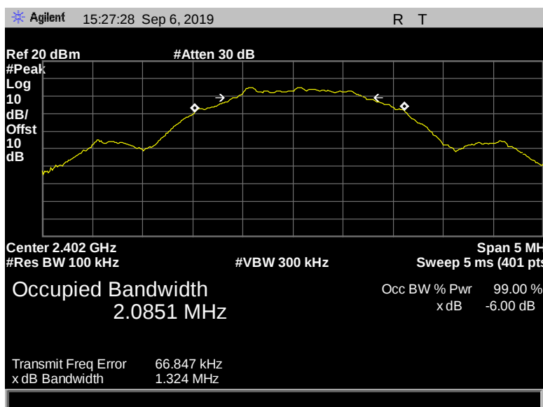
Figure 28: 6 dB Bandwidth, Terminal, 2402 MHz, 2 Mbps, 1.324 MHz
