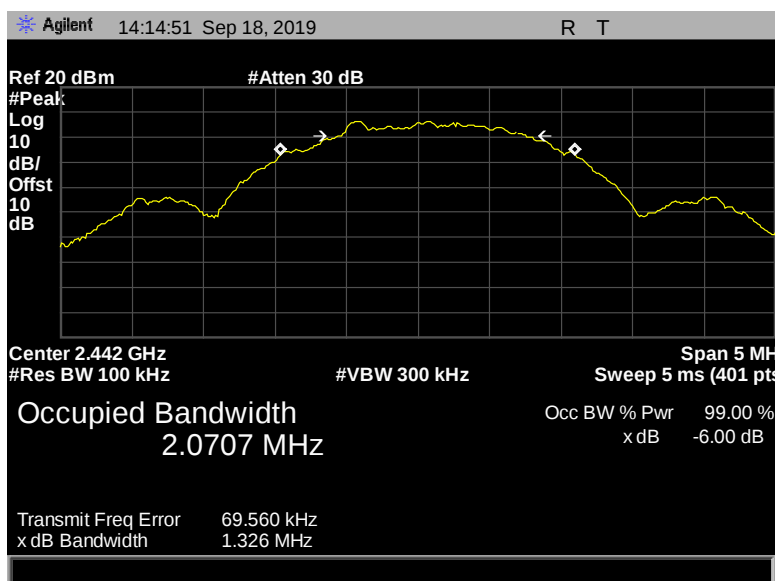
Figure 23: 6 dB Bandwidth, Pigtail, 2442 MHz, 2 Mbps, 1.326 MHz
