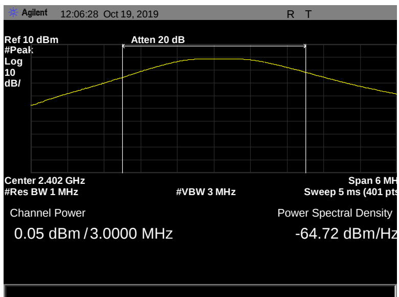
Figure 36: Peak Power Output, Pigtail, 2402 MHz, 1 Mbps, 0.05 dBm
