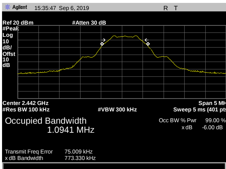
Figure 29: 6 dB Bandwidth, Terminal, 2442 MHz, 1 Mbps, 773.330 kHz
