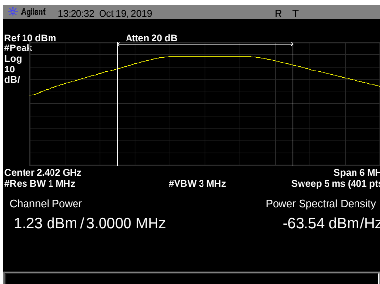
Figure 44: Peak Power Output, Terminal, 2402 MHz, 2 Mbps, 1.23 dBm
