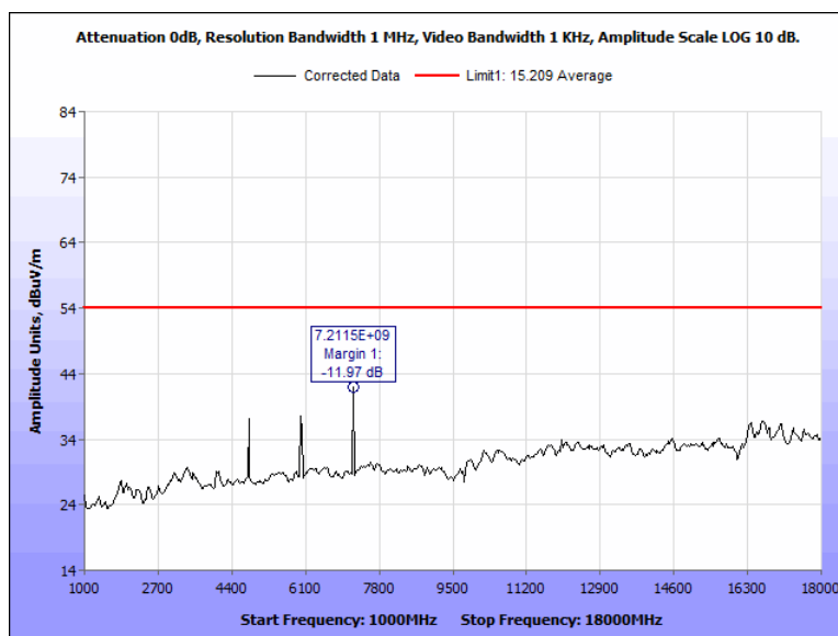
Figure 84: Radiated Spurious Emissions, Terminal, 2402 MHz, 1 GHz - 18 GHz, Average, Vertical
