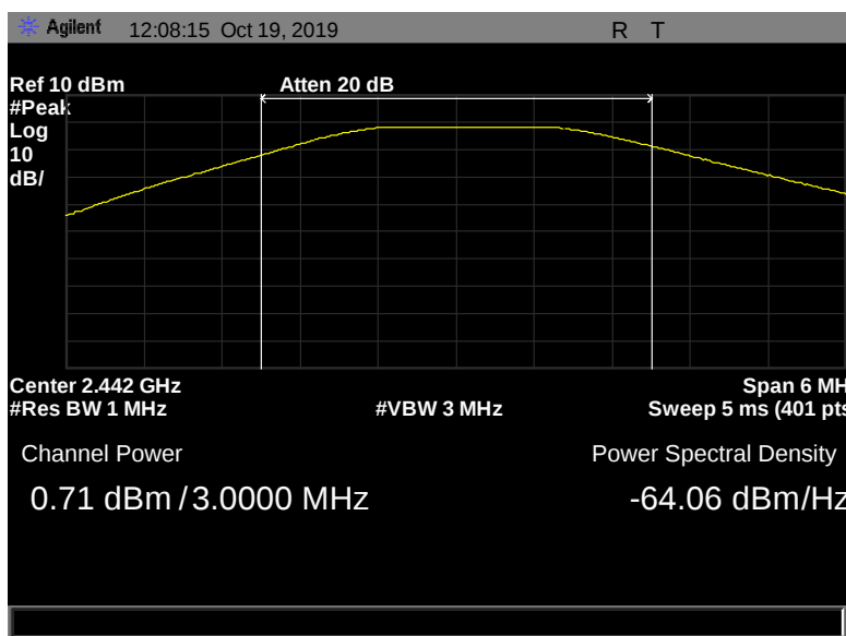
Figure 39: Peak Power Output, Pigtail, 2442 MHz, 2 Mbps, 0.71 dBm
