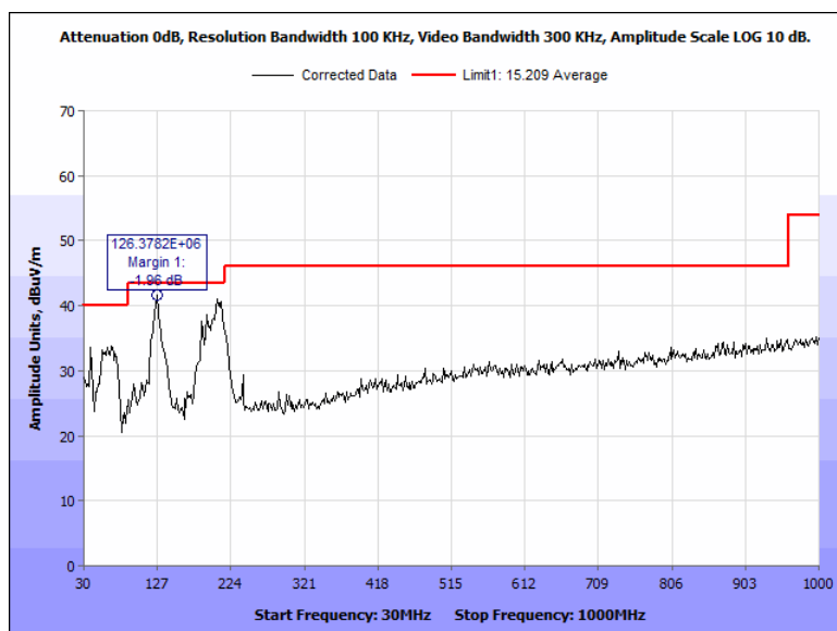
Figure 93: Radiated Spurious Emissions, Terminal, 2442 MHz, 30 MHz - 1000 MHz, Vertical
