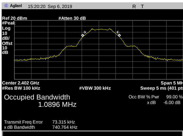
Figure 27: 6 dB Bandwidth, Terminal, 2402 MHz, 1 Mbps, 740.764 kHz
