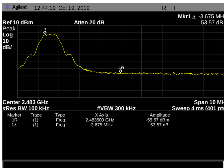
Figure 139: Conducted Band Edge, Pigtail, 2480 MHz, 1 Mbps
