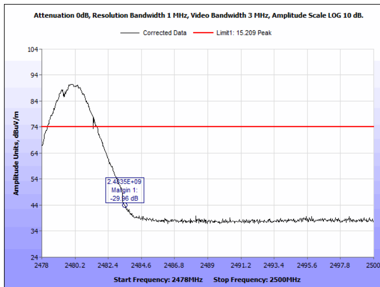
Figure 115: Radiated Band Edge, Pigtail, 2480 MHz, Peak, Vertical
