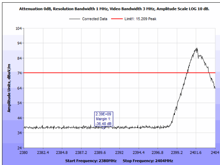
Figure 111: Radiated Band Edge, Pigtail, 2402 MHz, Peak, Vertical
