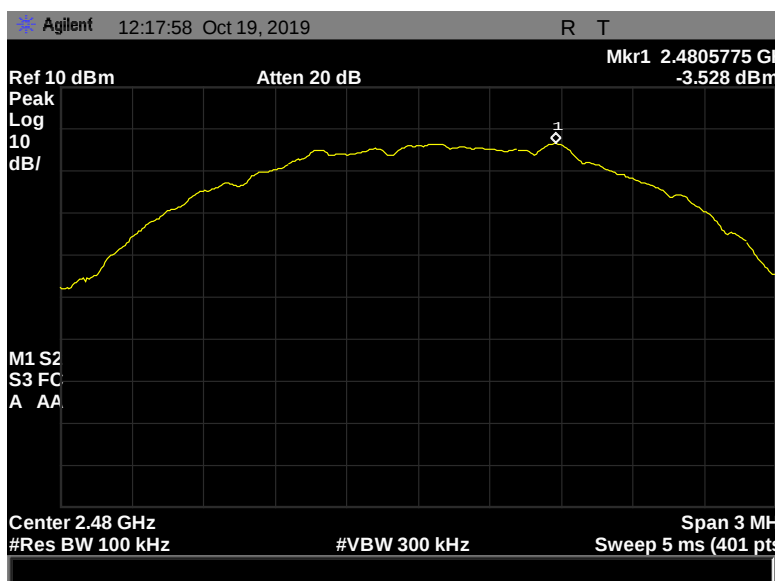
Figure 164: Peak Power Spectral Density, Pigtail, 2480 MHz, 2 Mbps, -3.528 dBm
