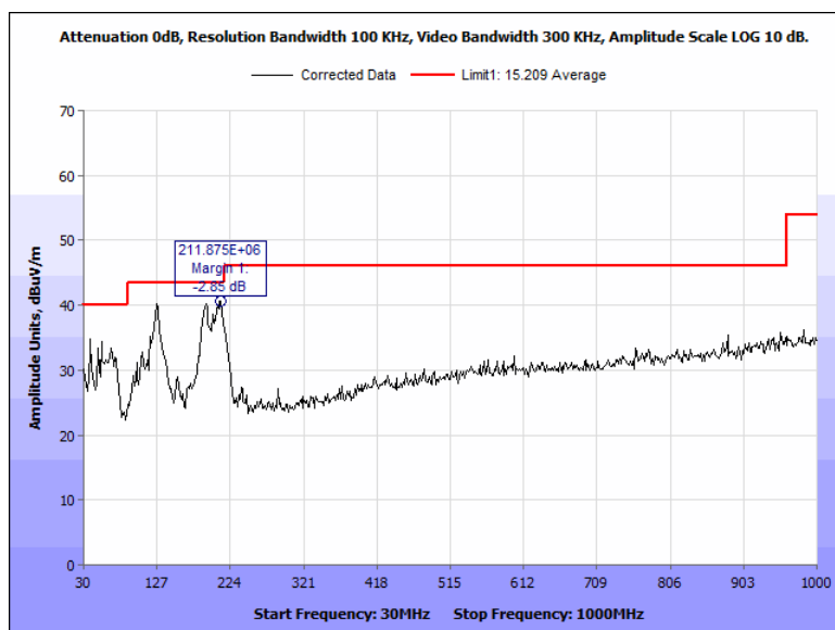
Figure 81: Radiated Spurious Emissions, Terminal, 2402 MHz, 30 MHz - 1000 MHz, Vertical
