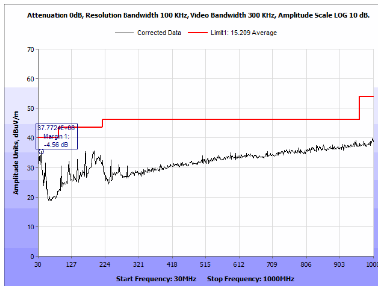
Figure 52: Radiated Spurious Emissions, Pigtail, 2402 MHz, 30 MHz - 1000 MHz, Horizontal
