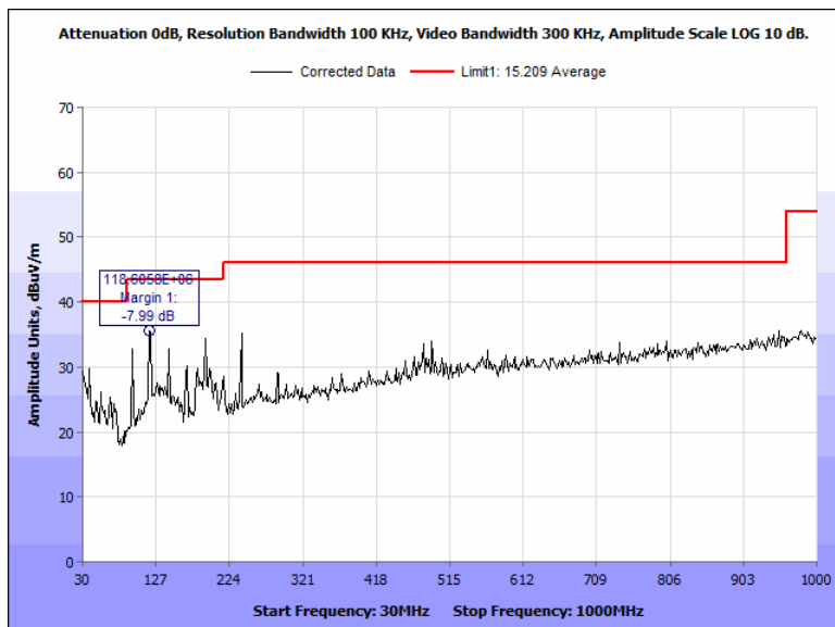
Figure 100: Radiated Spurious Emissions, Terminal, 2480 MHz, 30 MHz - 1000 MHz, Horizontal
