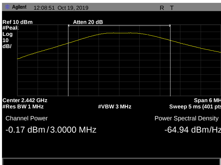
Figure 38: Peak Power Output, Pigtail, 2442 MHz, 1 Mbps, -0.17 dBm
