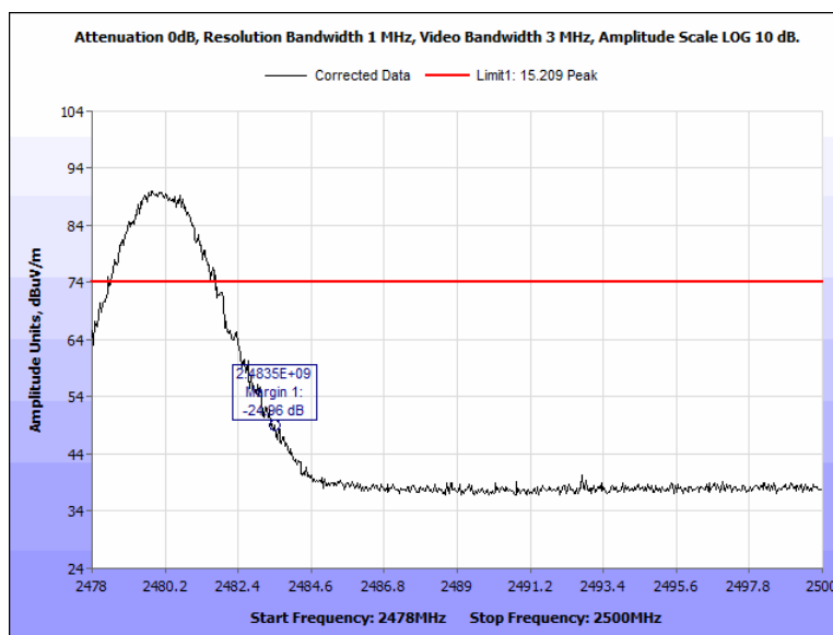
Figure 114: Radiated Band Edge, Pigtail, 2480 MHz, Peak, Horizontal
