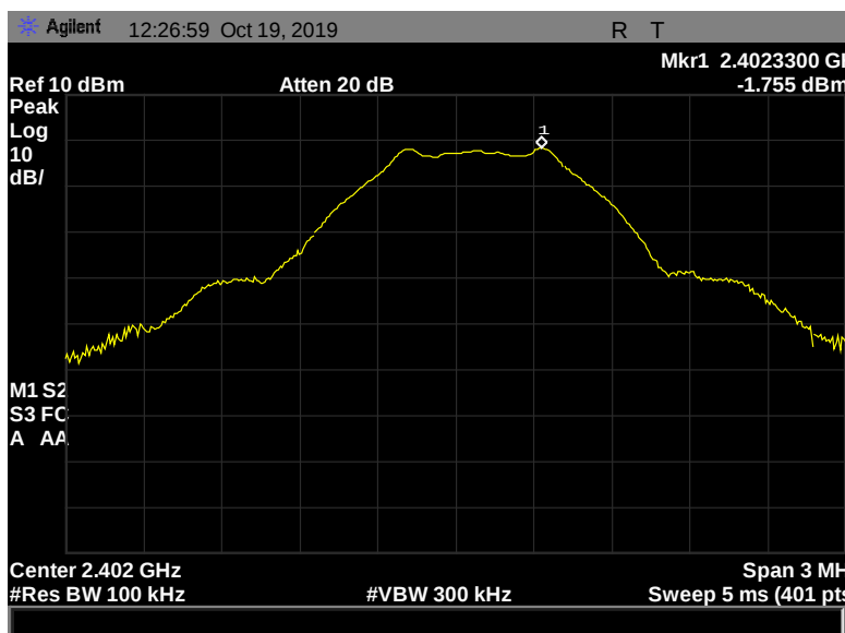
Figure 159: Peak Power Spectral Density, Pigtail, 2402 MHz, 1 Mbps, -1.755 dBm
