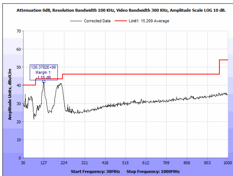
Figure 101: Radiated Spurious Emissions, Terminal, 2480 MHz, 30 MHz - 1000 MHz, Vertical
