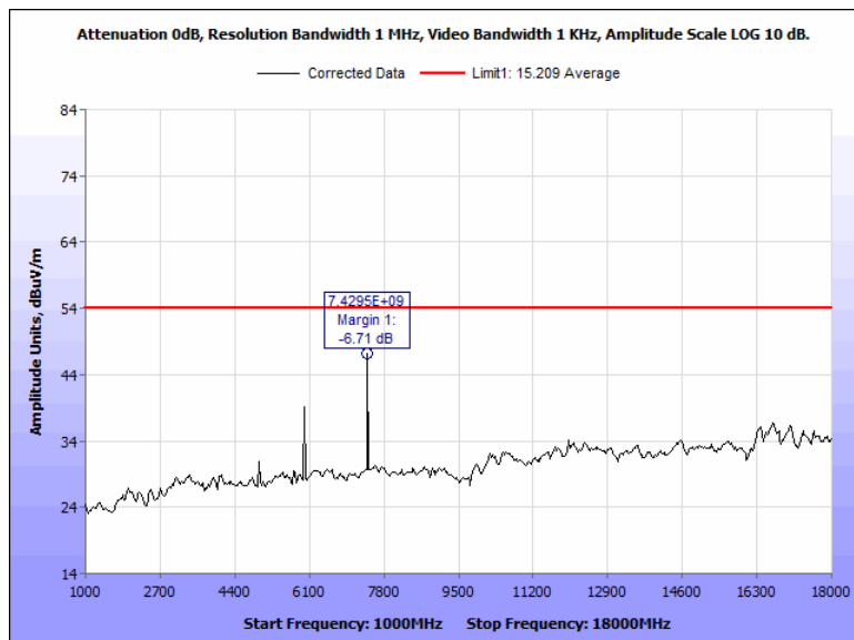
Figure 104: Radiated Spurious Emissions, Terminal, 2480 MHz, 1 GHz - 18 GHz, Average, Vertical
