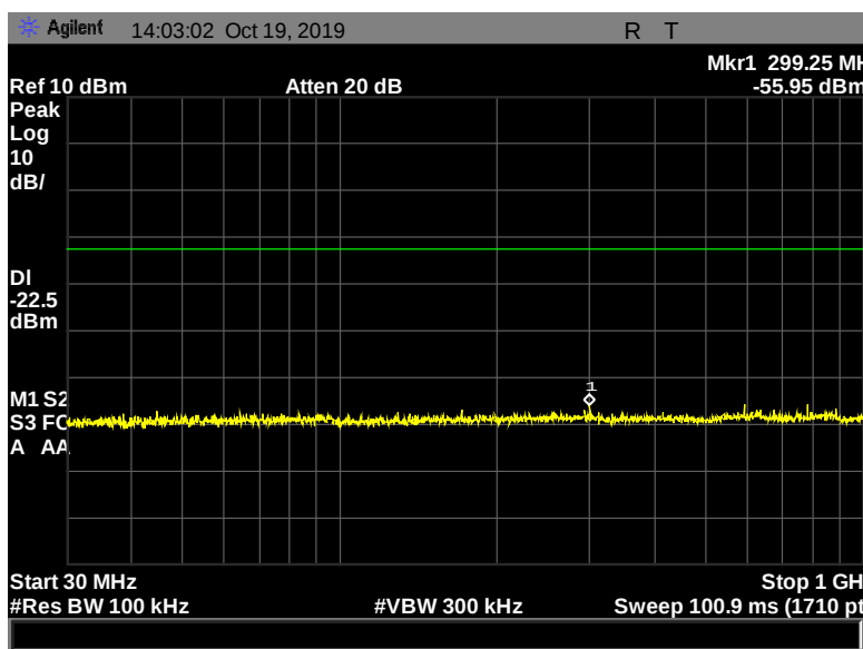
Figure 143: Conducted Spurious Emissions, Terminal, 2402 MHz, 2 Mbps, 30 MHz - 1000 MHz
