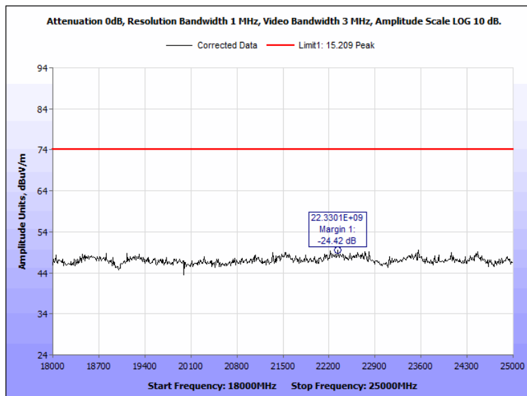
Figure 90: Radiated Spurious Emissions, Terminal, 2402 MHz, 18 GHz - 25 GHz, Peak, Horizontal
