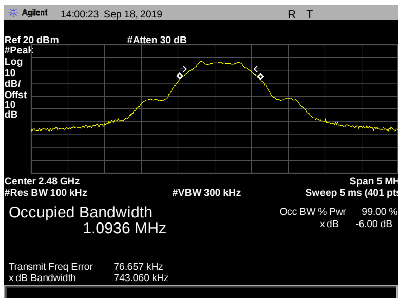
Figure 24: 6 dB Bandwidth, Pigtail, 2480 MHz, 1 Mbps, 743.060 kHz
