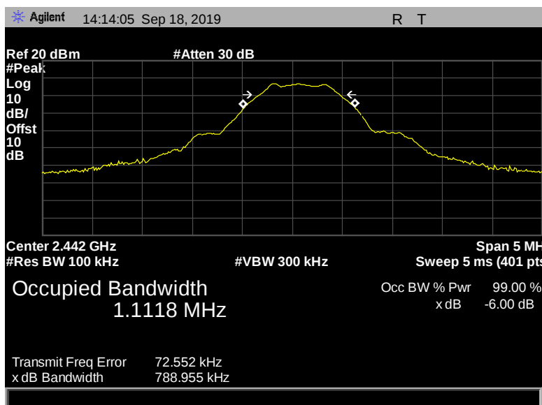
Figure 22: 6 dB Bandwidth, Pigtail, 2442 MHz, 1 Mbps, 788.955 kHz
