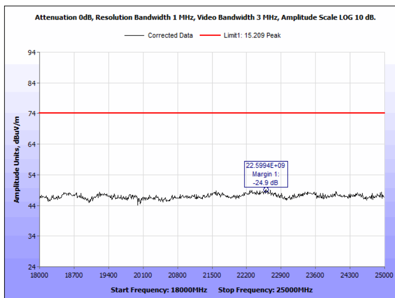
Figure 91: Radiated Spurious Emissions, Terminal, 2402 MHz, 18 GHz - 25 GHz, Peak, Vertical
