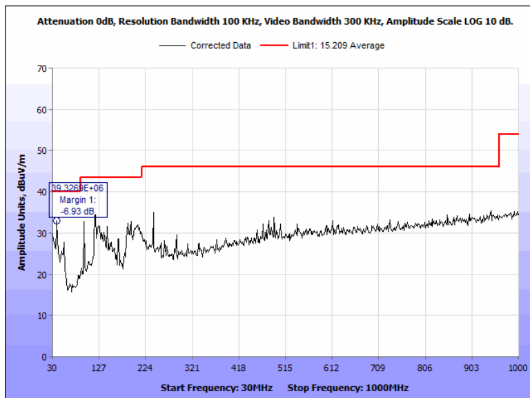
Figure 92: Radiated Spurious Emissions, Terminal, 2442 MHz, 30 MHz - 1000 MHz, Horizontal
