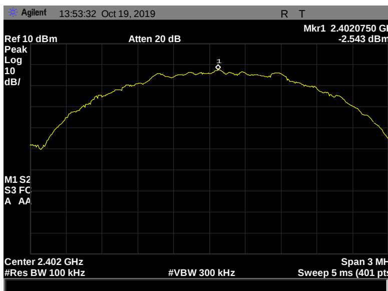
Figure 167: Peak Power Spectral Density, Terminal, 2402 MHz, 2 Mbps, -2.543 dBm
