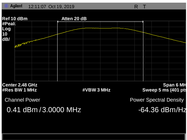
Figure 41: Peak Power Output, Pigtail, 2480 MHz, 2 Mbps, 0.41 dBm
