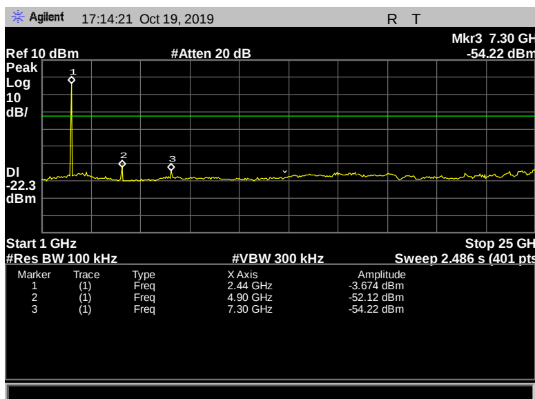
Figure 132: Conducted Spurious Emissions, Pigtail, 2442 MHz, 2 Mbps, 1 GHz - 25 GHz
