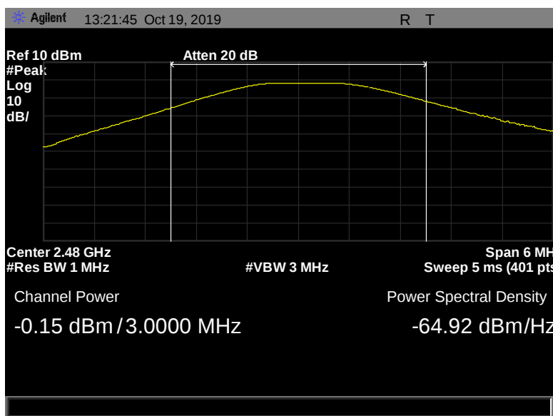
Figure 47: Peak Power Output, Terminal, 2480 MHz, 1 Mbps, -0.15 dBm
