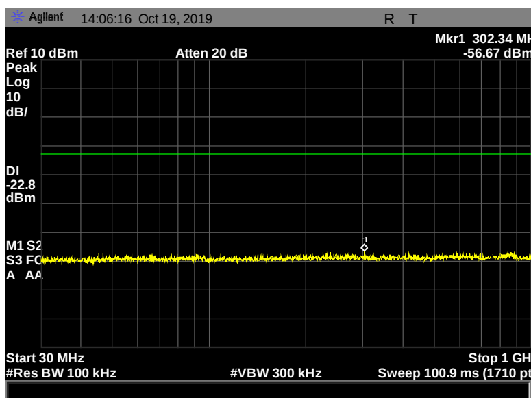
Figure 147: Conducted Spurious Emissions, Terminal, 2442 MHz, 2 Mbps, 30 MHz – 1000 MHz
