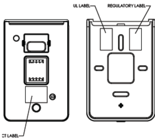
MOUNTING PLATE INSIDE VIEW
