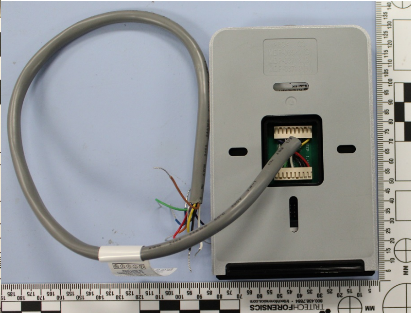
Model 40K (pigtail version) rear side
