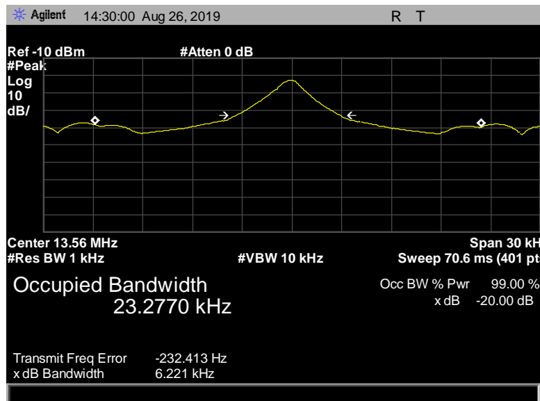
Figure 22: 20 dB Occupied Bandwidth, Terminal, -20dB - 6.221 KHz
