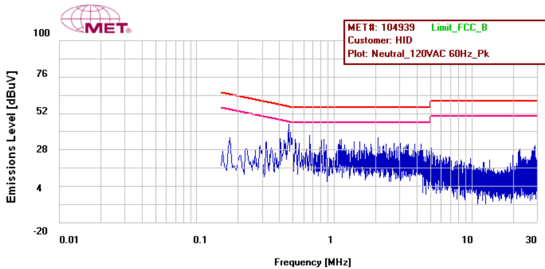
Figure 18: Conducted Emissions Limits, Terminal, Neutral Line, Prescan
