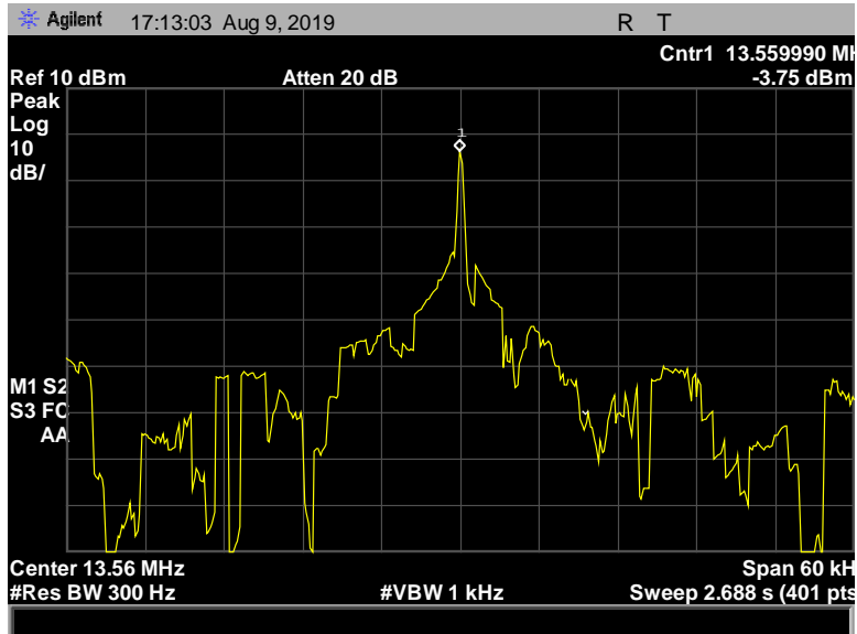
Figure 79: Frequency Stability, Pigtail, (50), 13.8VDC
