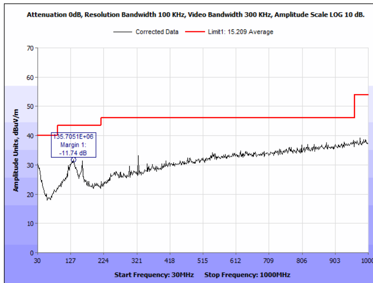
Figure 55: Spurious Emission Limits, outside the bands 13.110 – 14.010 MHz, Pigtail, 30 MHz – 1000 MHz, Horizontal
