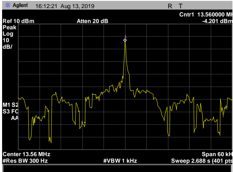
Figure 89: Frequency Stability, Terminal, (50), 13.8VDC
