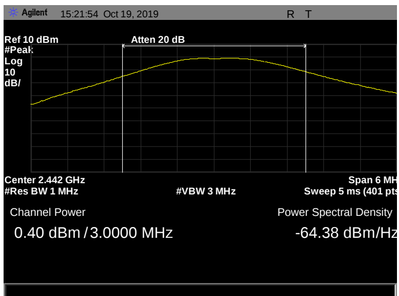
Figure 38: Peak Power Output, Pigtail, 2442 MHz, 1 Mbps, 0.40 dBm
