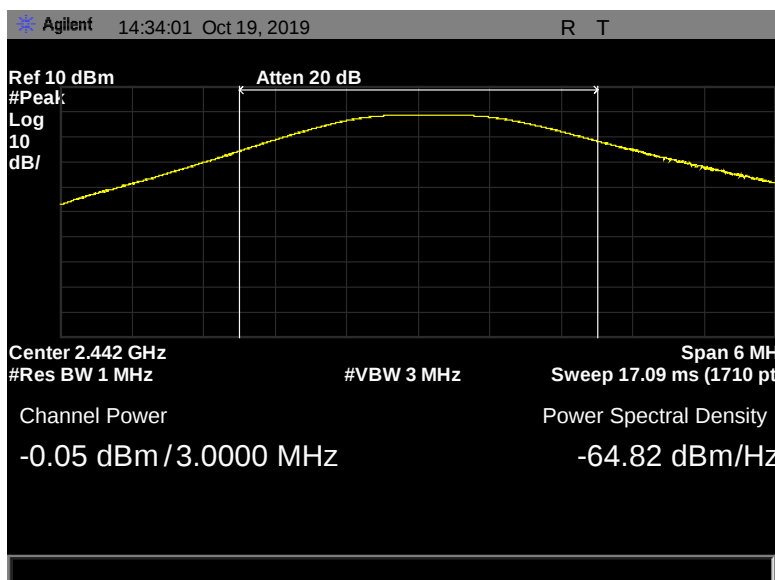
Figure 45: Peak Power Output, Terminal, 2442 MHz, 1 Mbps, -0.05 dBm
