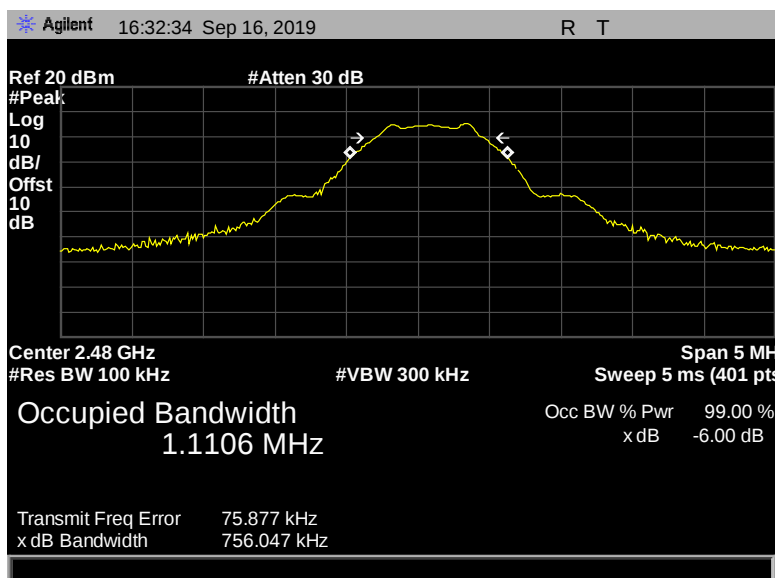
Figure 31: 6 dB Bandwidth, Terminal, 2480 MHz, 1 Mbps, 756.047 kHz
