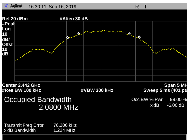
Figure 30: 6 dB Bandwidth, Terminal, 2442 MHz, 2 Mbps, 1.224 MHz
