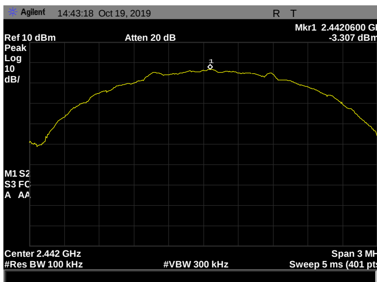
Figure 169: Peak Power Spectral Density, Terminal, 2442 MHz, 2 Mbps, -3.307 dBm
