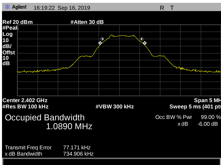
Figure 27: 6 dB Bandwidth, Terminal, 2402 MHz, 1 Mbps, 734.906 kHz
