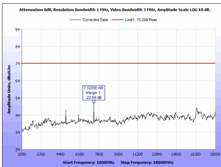
Figure 107: Radiated Spurious Emissions, Terminal, 2442 MHz, 1 GHz – 18 GHz, Peak, Vertical
