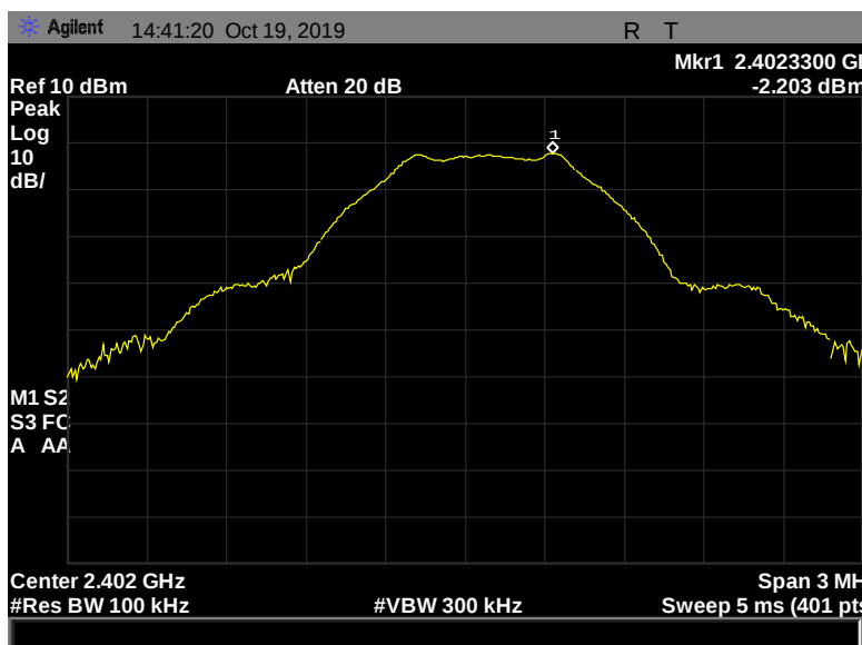
Figure 166: Peak Power Spectral Density, Terminal, 2402 MHz, 1 Mbps, -2.203 dBm
