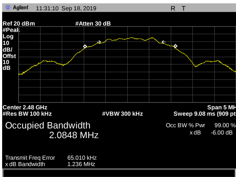
Figure 25: 6 dB Bandwidth, Pigtail, 2480 MHz, 2 Mbps, 1.236 MHz
