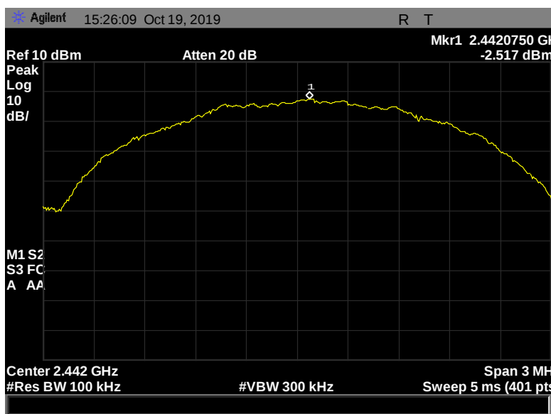
Figure 162: Peak Power Spectral Density, Pigtail, 2442 MHz, 2 Mbps, -2.517 dBm
