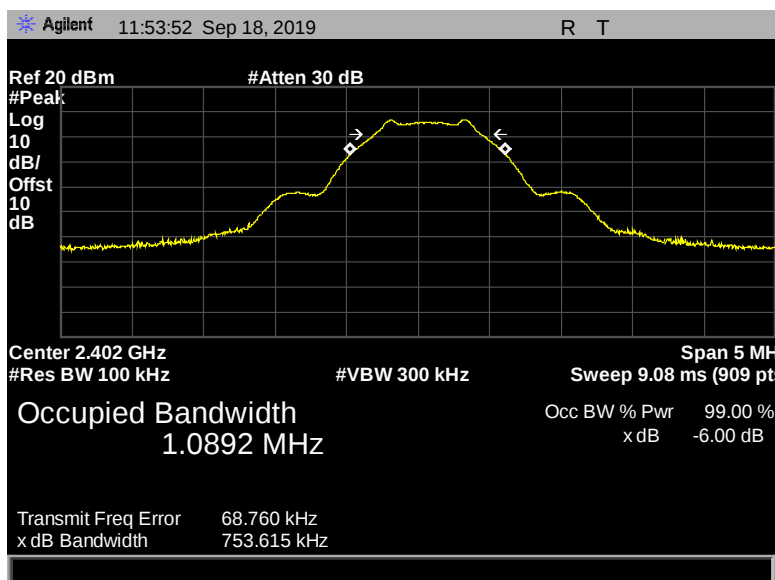
Figure 20: 6 dB Bandwidth, Pigtail, 2402 MHz, 1 Mbps, 753.615 kHz
