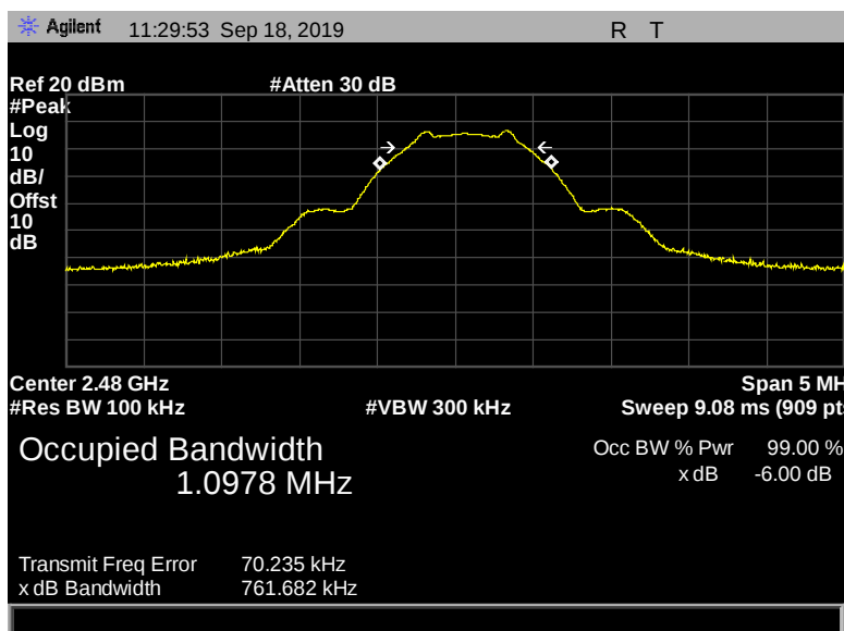
Figure 24: 6 dB Bandwidth, Pigtail, 2480 MHz, 1 Mbps, 761.682 kHz
