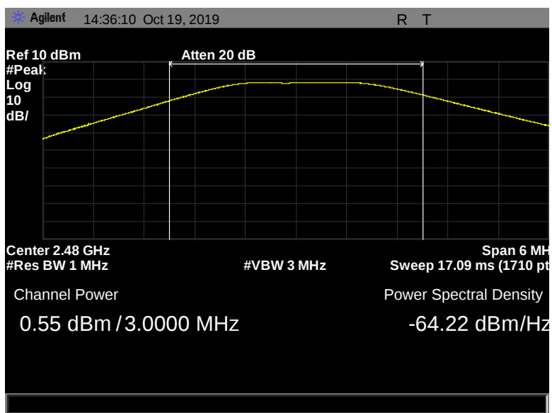
Figure 48: Peak Power Output, Terminal, 2480 MHz, 2 Mbps, 0.55 dBm
