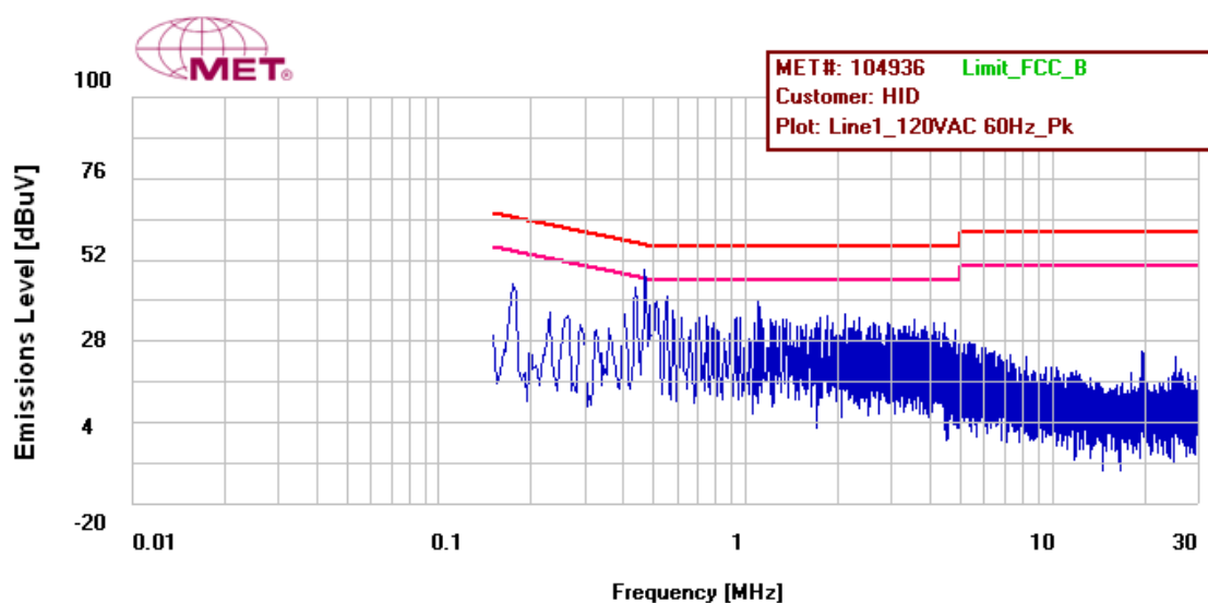
Figure 11: Conducted Emissions Limits, Pigtail, Phase Line, Prescan
