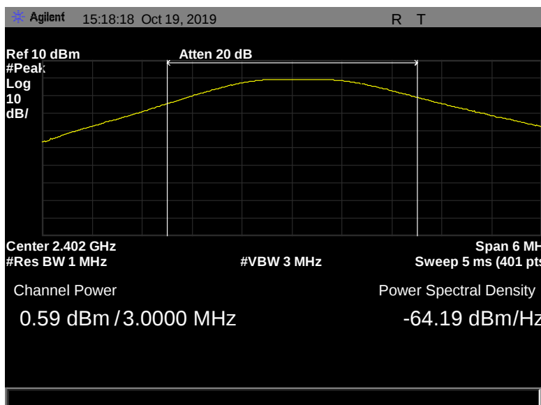
Figure 36: Peak Power Output, Pigtail, 2402 MHz, 1 Mbps, 0.59 dBm
