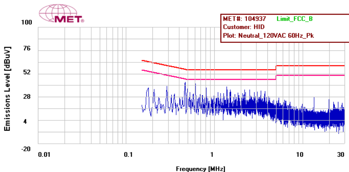
Figure 17: Conducted Emissions Limits, Neutral Line, Terminal, Prescan
