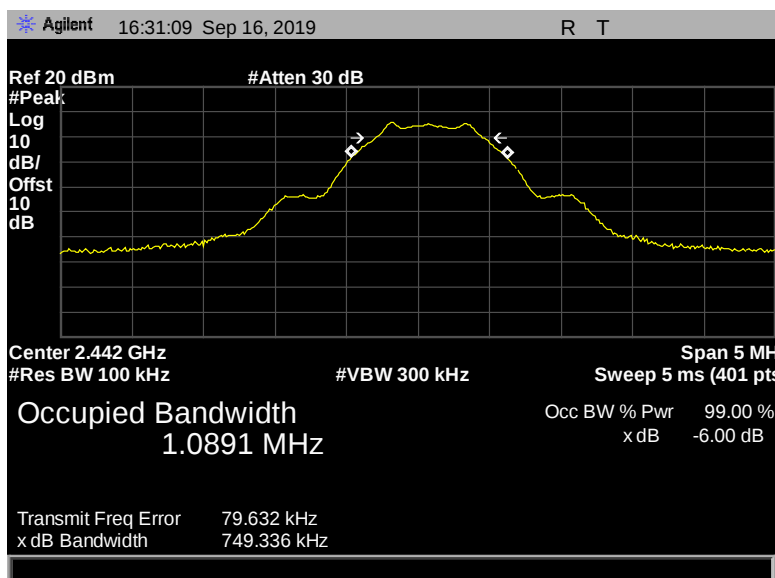
Figure 29: 6 dB Bandwidth, Terminal, 2442 MHz, 1 Mbps, 749.336 kHz
