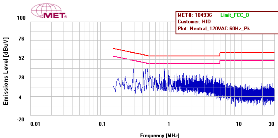
Figure 13: Conducted Emissions Limits, Pigtail, Neutral Line, Prescan
