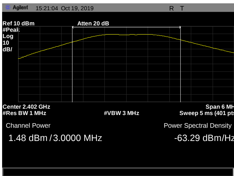
Figure 37: Peak Power Output, Pigtail, 2402 MHz, 2 Mbps, 1.48 dBm
