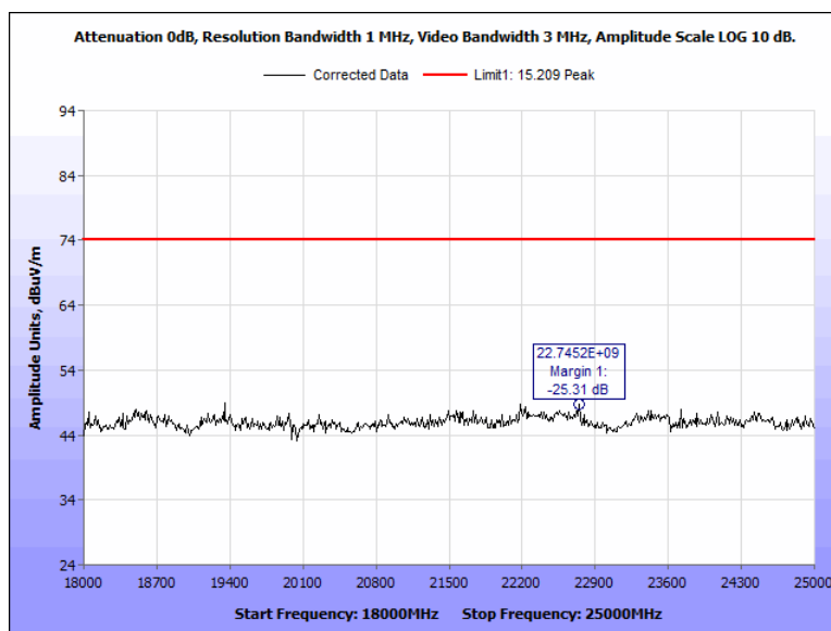
Figure 99: Radiated Spurious Emissions, Terminal, 2402 MHz, 18 GHz – 25 GHz, Peak, Vertical
