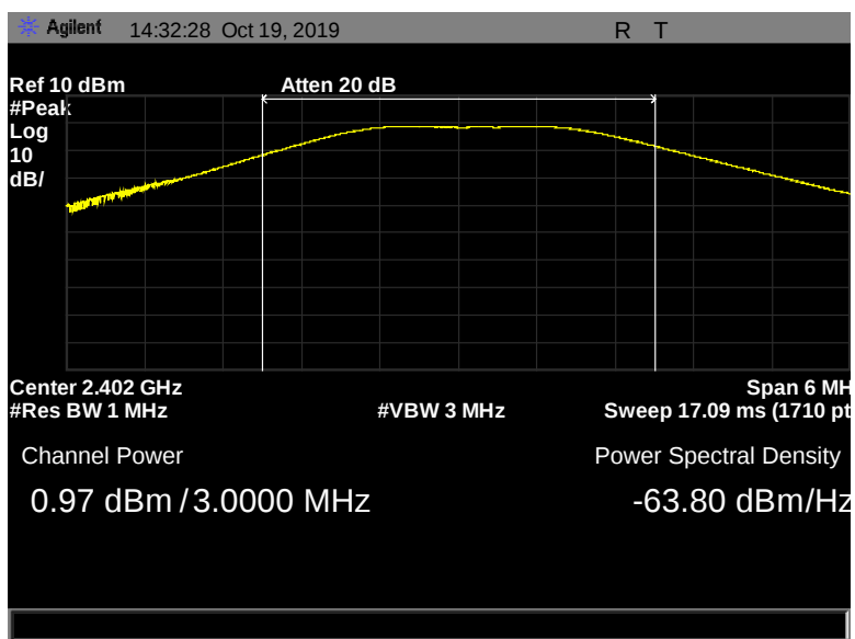
Figure 44: Peak Power Output, Terminal, 2402 MHz, 2 Mbps, 0.97 dBm
