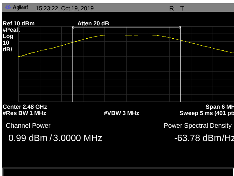
Figure 41: Peak Power Output, Pigtail, 2480 MHz, 2 Mbps, 0.99 dBm
