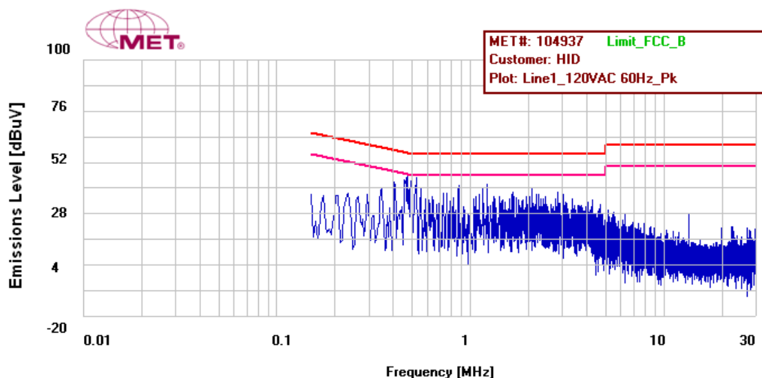
Figure 15: Conducted Emissions Limits, Phase Line, Terminal, Prescan
