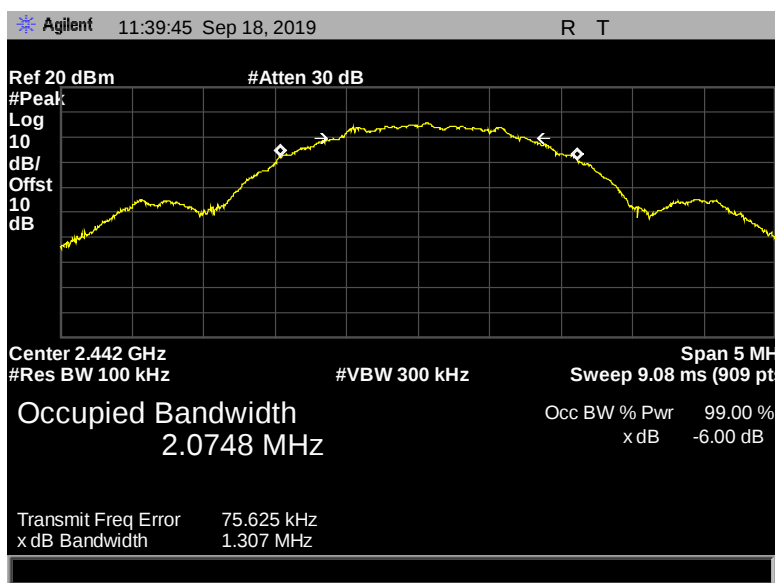
Figure 23: 6 dB Bandwidth, Pigtail, 2442 MHz, 2 Mbps, 1.307 MHz
