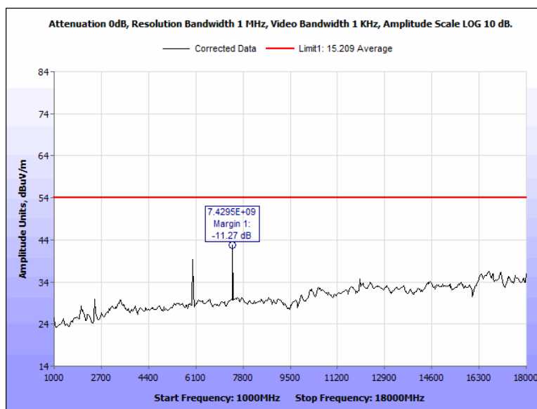
Figure 76: Radiated Spurious Emissions, Pigtail, 2480 MHz, 1 GHz – 18 GHz, Average, Vertical
