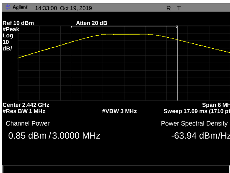
Figure 46: Peak Power Output, Terminal, 2442 MHz, 2 Mbps, 0.85 dBm
