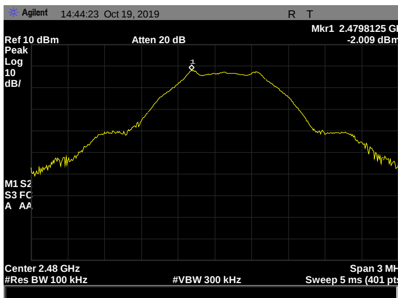
Figure 170: Peak Power Spectral Density, Terminal, 2480 MHz, 1 Mbps, -2.009 dbm
