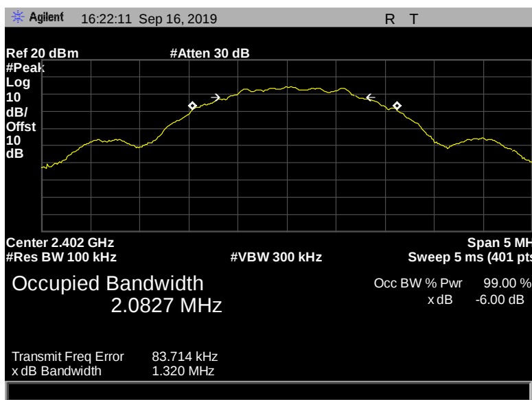
Figure 28: 6 dB Bandwidth, Terminal, 2402 MHz, 2 Mbps, 1.320 MHz
