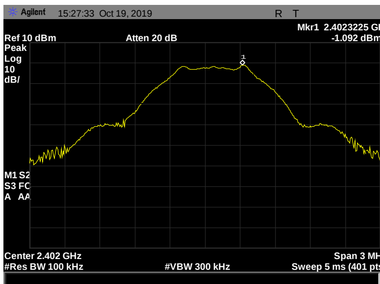
Figure 159: Peak Power Spectral Density, Pigtail, 2402 MHz, 1 Mbps, -1.092 dBm
