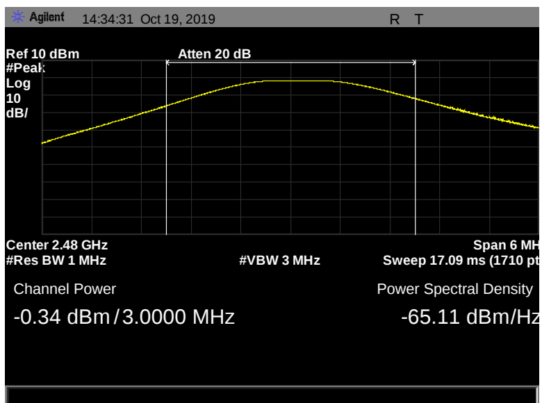
Figure 47: Peak Power Output, Terminal, 2480 MHz, 1 Mbps, -0.34 dBm
