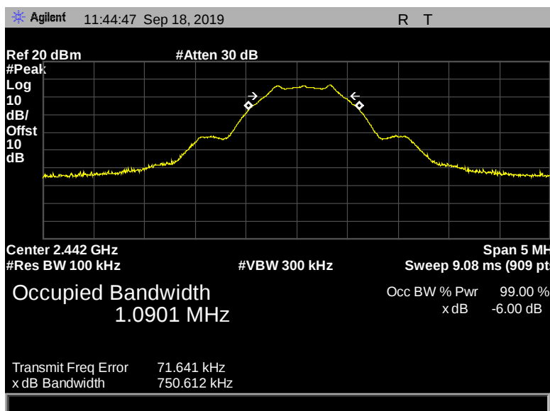
Figure 22: 6 dB Bandwidth, Pigtail, 2442 MHz, 1 Mbps, 750.612 kHz
