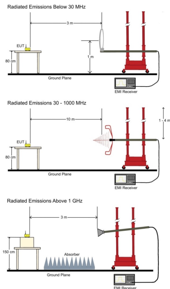
Figure 51: Radiated Emissions Test Setup
