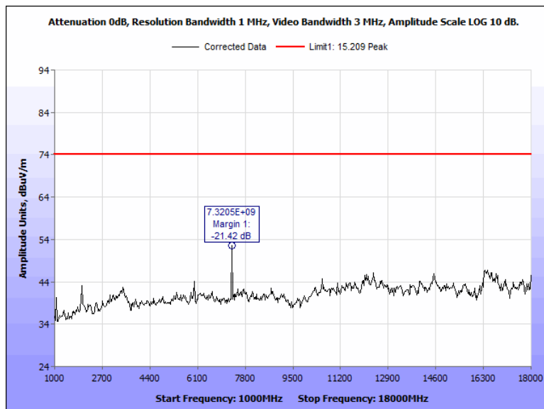
Figure 70: Radiated Spurious Emissions, Pigtail, 2442 MHz, 1 GHz – 18 GHz, Peak, Vertical
