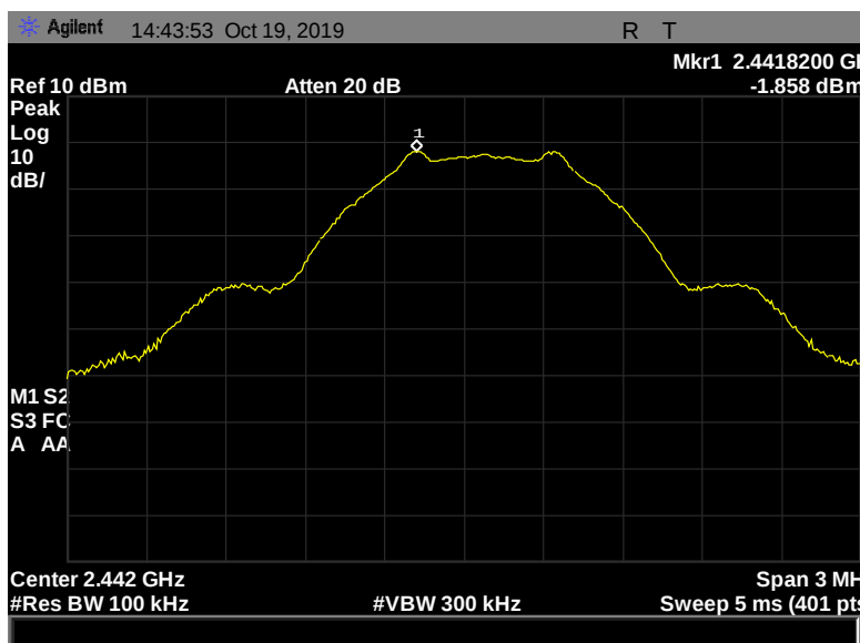
Figure 168: Peak Power Spectral Density, Terminal, 2442 MHz, 1 Mbps, -1.858 dBm
