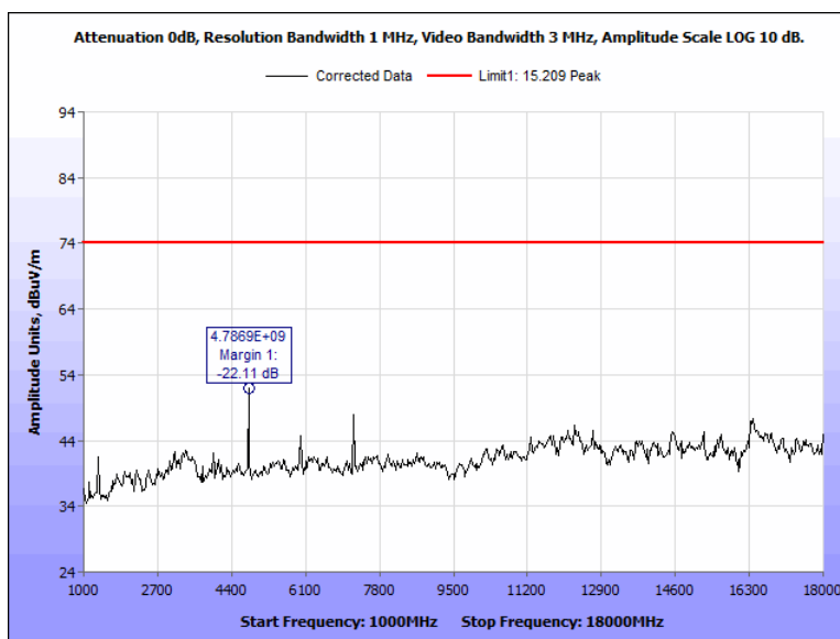
Figure 95: Radiated Spurious Emissions, Terminal, 2402 MHz, 1 GHz – 18 GHz, Peak, Vertical
