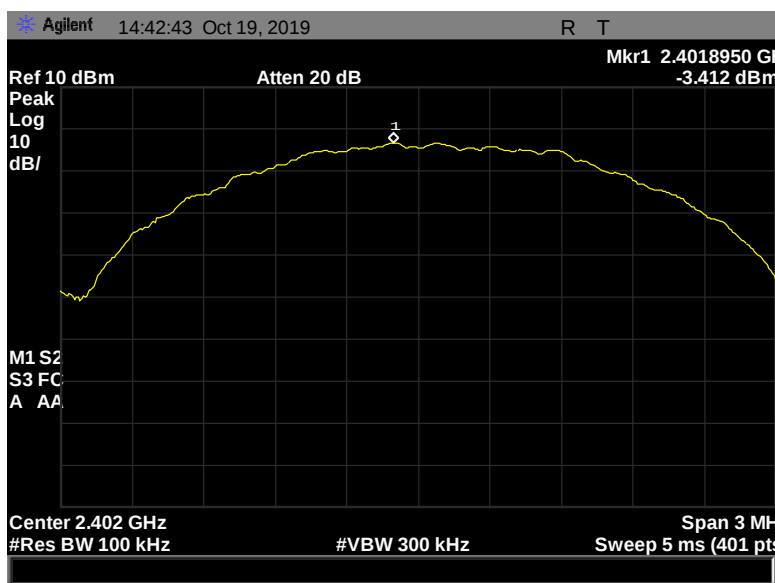
Figure 167: Peak Power Spectral Density, Terminal, 2402 MHz, 2 Mbps, -3.412 dBm
