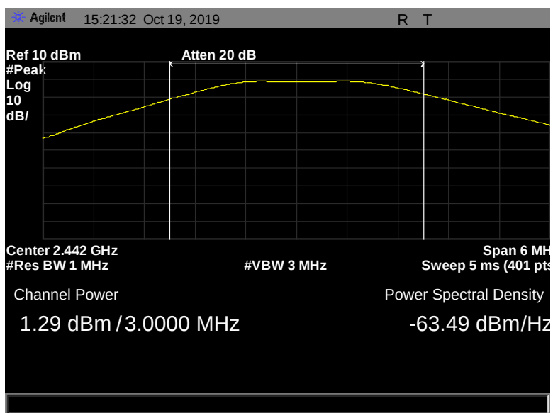
Figure 39: Peak Power Output, Pigtail, 2442 MHz, 2 Mbps, 1.29 dBm
