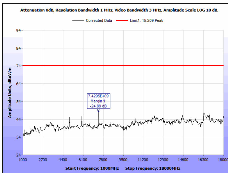
Figure 115: Radiated Spurious Emissions, Terminal, 2480 MHz, 1 GHz – 18 GHz, Peak, Vertical
