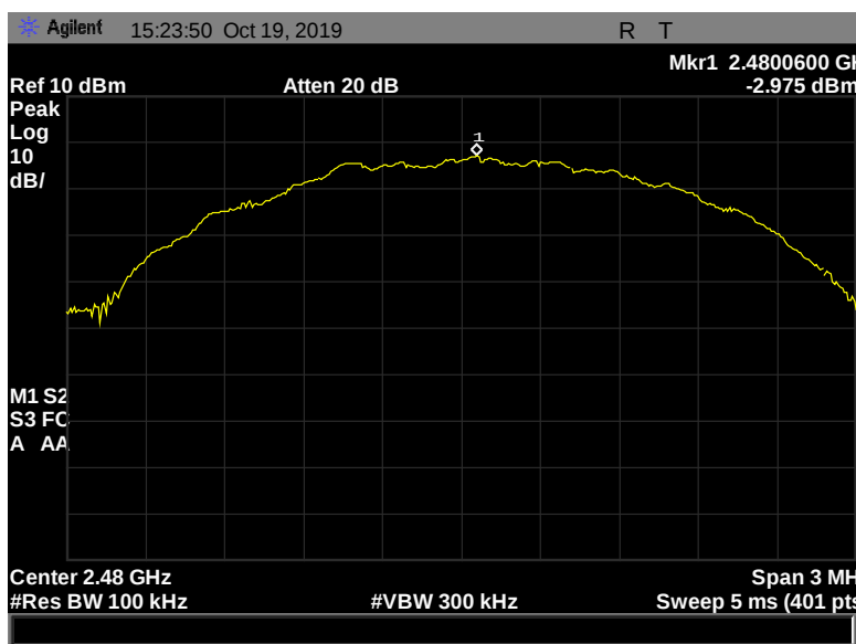
Figure 164: Peak Power Spectral Density, Pigtail, 2480 MHz, 2 Mbps, -2.975 dBm
