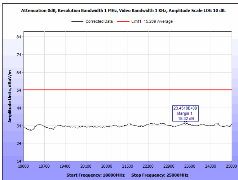
Figure 97: Radiated Spurious Emissions, Terminal, 2402 MHz, 18 GHz – 25 GHz, Average, Vertical
