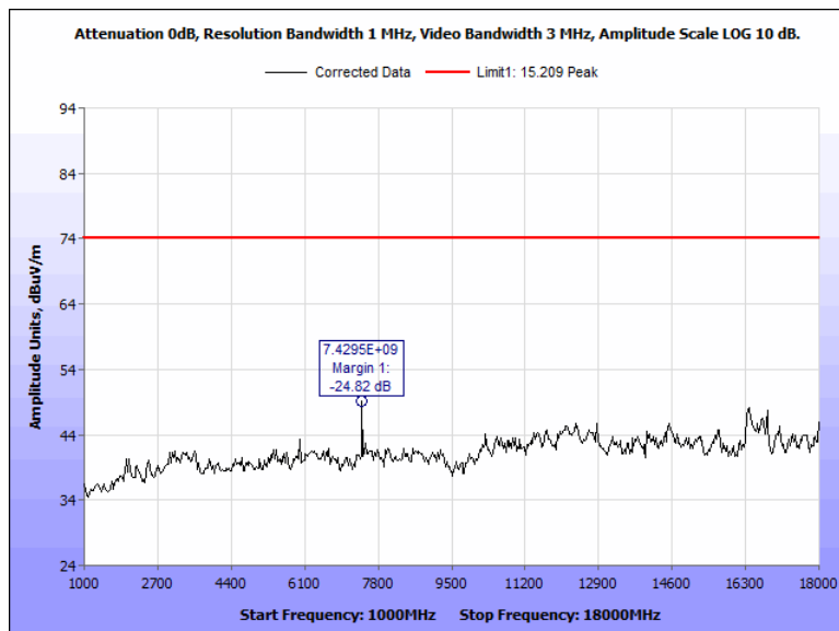
Figure 77: Radiated Spurious Emissions, Pigtail, 2480 MHz, 1 GHz – 18 GHz, Peak, Horizontal
