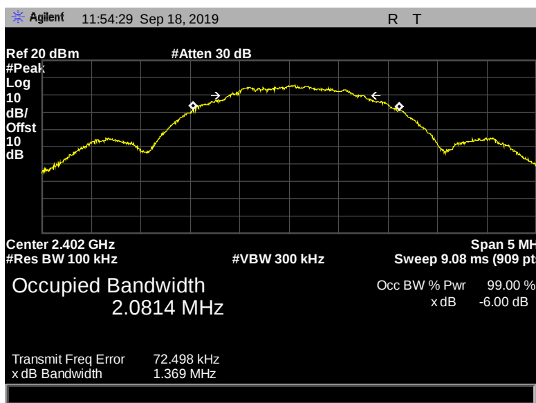
Figure 21: 6 dB Bandwidth, Pigtail, 2402 MHz, 2 Mbps, 1.369 MHz
