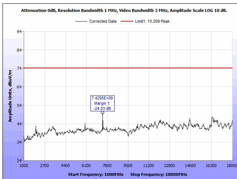
Figure 78: Radiated Spurious Emissions, Pigtail, 2480 MHz, 1 GHz – 18 GHz, Peak, Vertical
