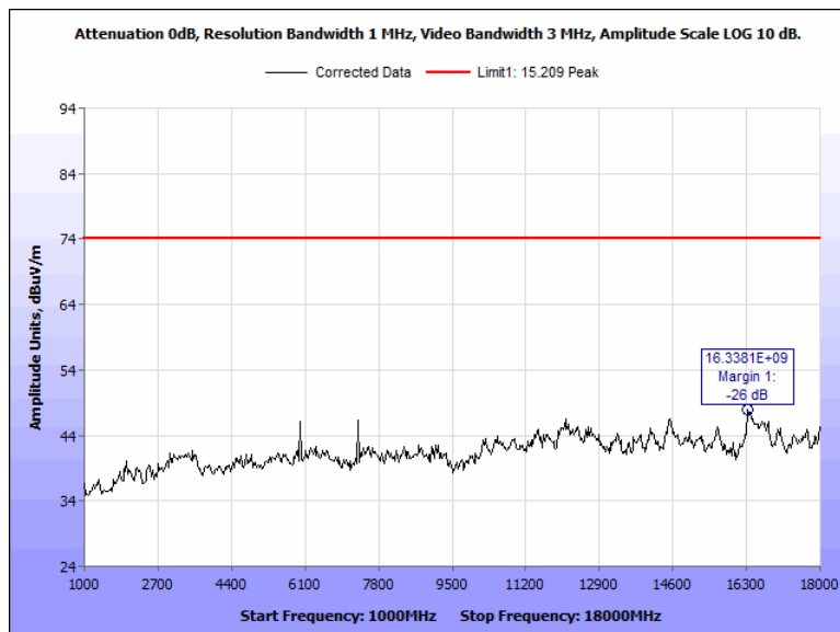
Figure 69: Radiated Spurious Emissions, Pigtail, 2442 MHz, 1 GHz – 18 GHz, Peak, Horizontal
