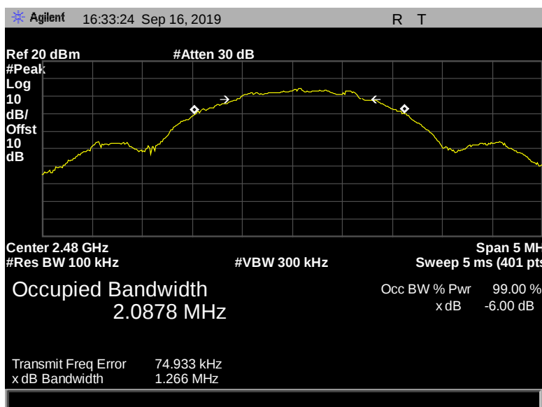
Figure 32: 6 dB Bandwidth, Terminal, 2480 MHz, 2 Mbps, 1.266 MHz
