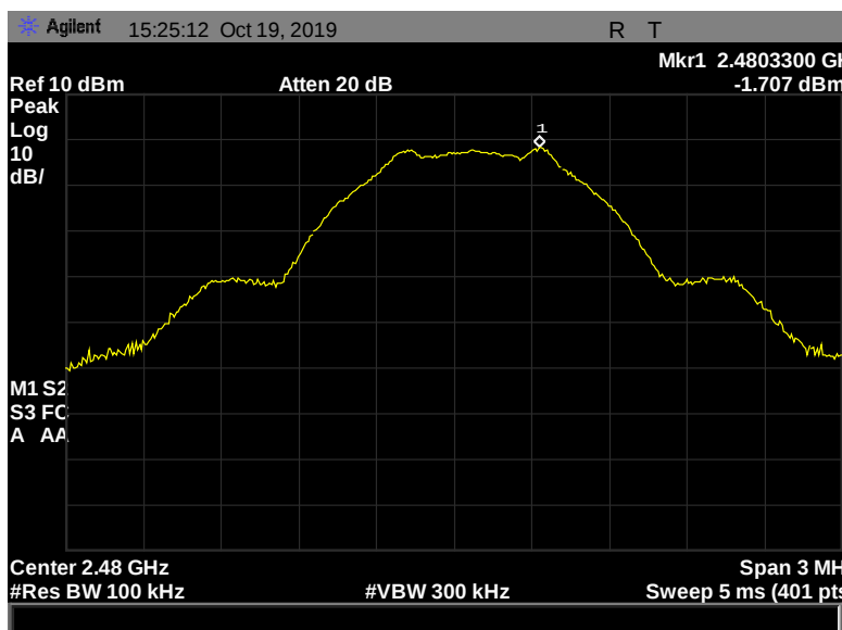
Figure 163: Peak Power Spectral Density, Pigtail, 2480 MHz, 1 Mbps, -1.707 dBm
