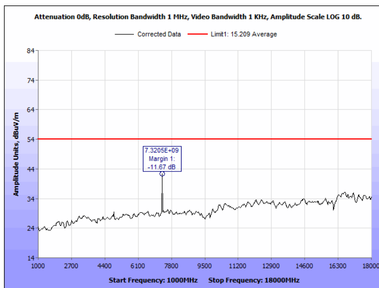
Figure 68: Radiated Spurious Emissions, Pigtail, 2442 MHz, 1 GHz – 18 GHz, Average, Vertical
