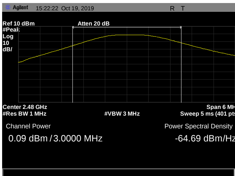
Figure 40: Peak Power Output, Pigtail, 2480 MHz, 1 Mbps, 0.09 dBm
