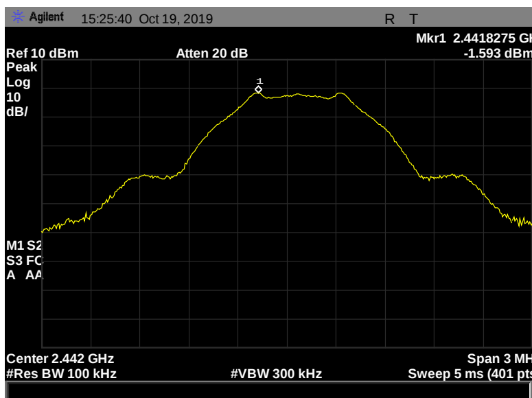
Figure 161: Peak Power Spectral Density, Pigtail, 2442 MHz, 1 Mbps, -1.593 dBm
