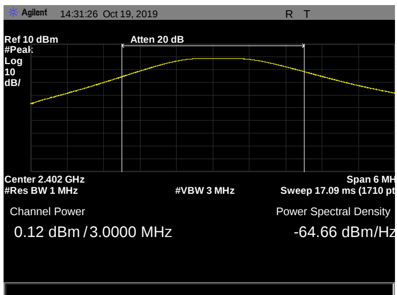
Figure 43: Peak Power Output, Terminal, 2402 MHz, 1 Mbps, 0.12 dBm
