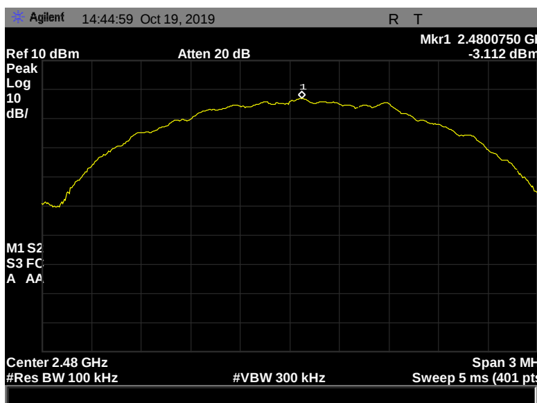
Figure 171: Peak Power Spectral Density, Terminal, 2480 MHz, 2 Mbps, -3.112 dBm
