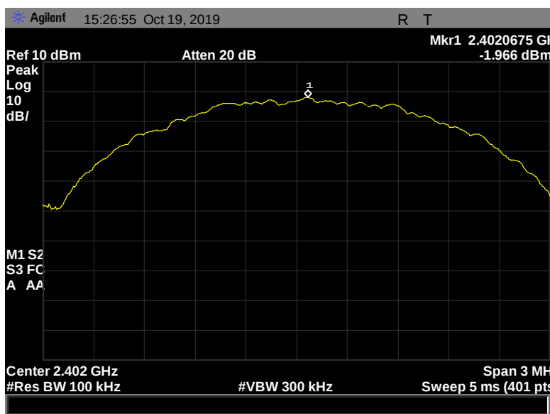
Figure 160: Peak Power Spectral Density, Pigtail, 2402 MHz, 2 Mbps, -1.966 dBm
