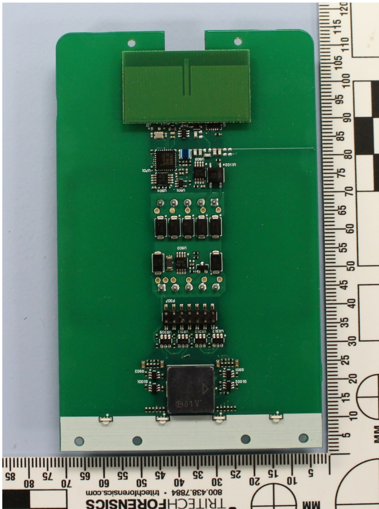
Model 40 (terminal version) main board obverse with patch antenna
