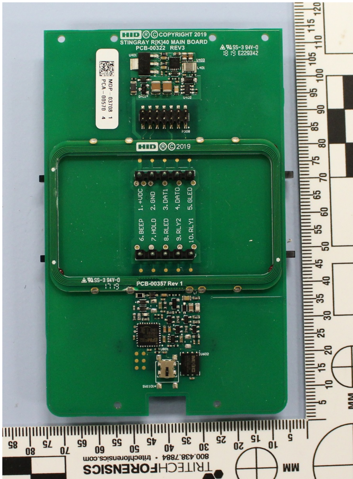
Model 40 (terminal version) main board reverse
