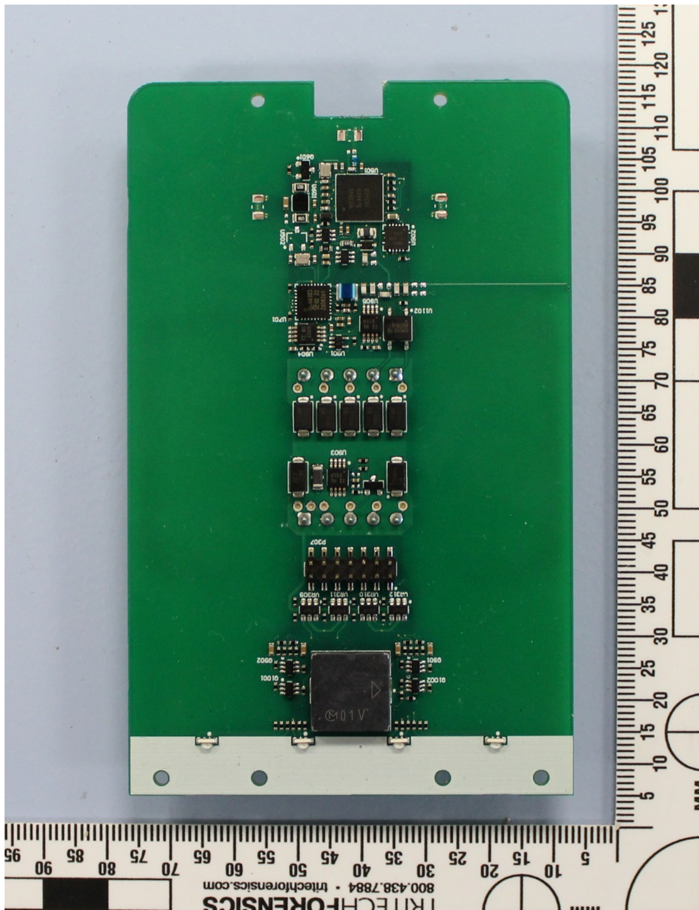
Model 40 (terminal version) main board obverse without patch antenna
