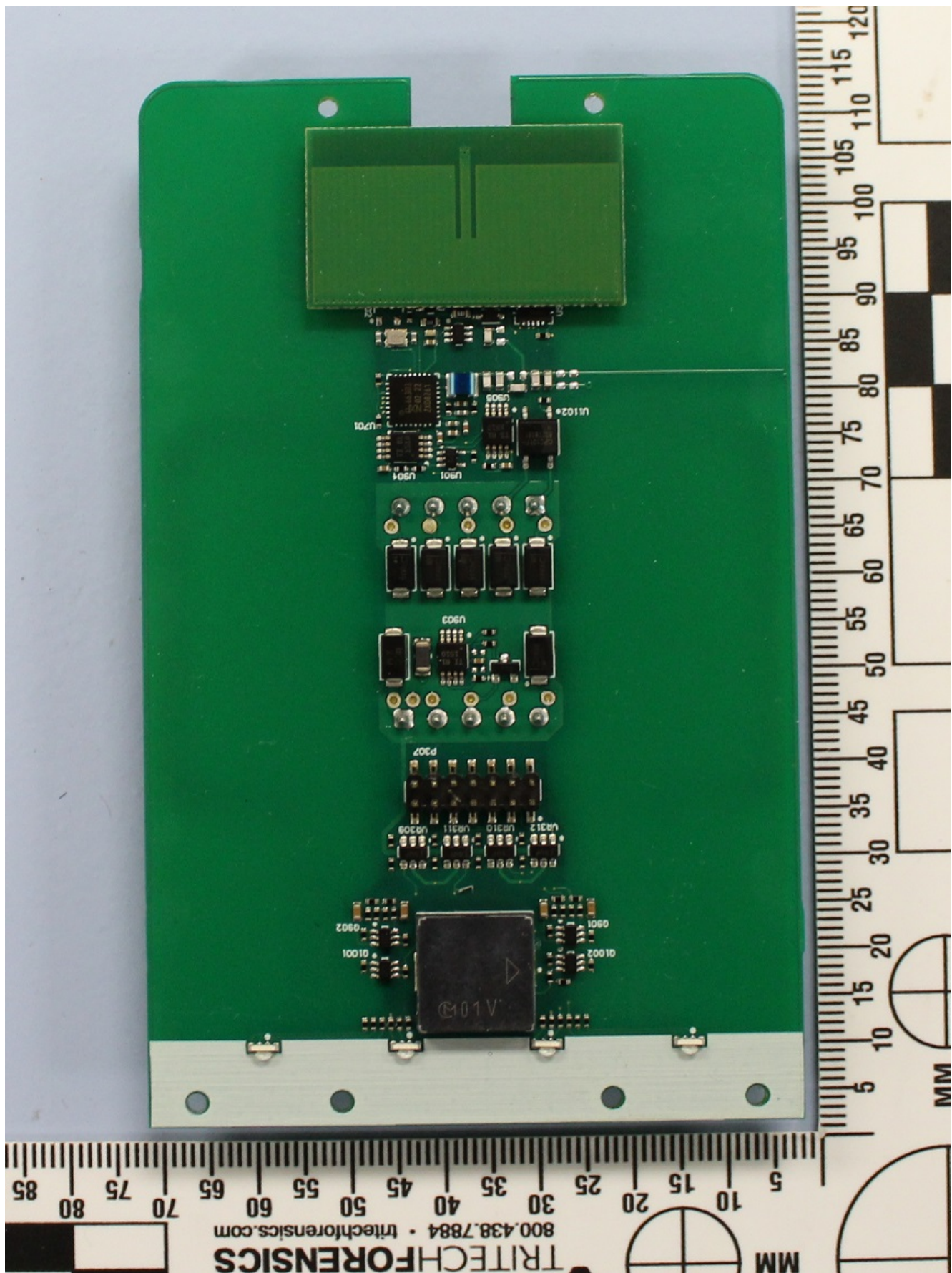
Model 40 (pigtail version) main board obverse with patch antenna
