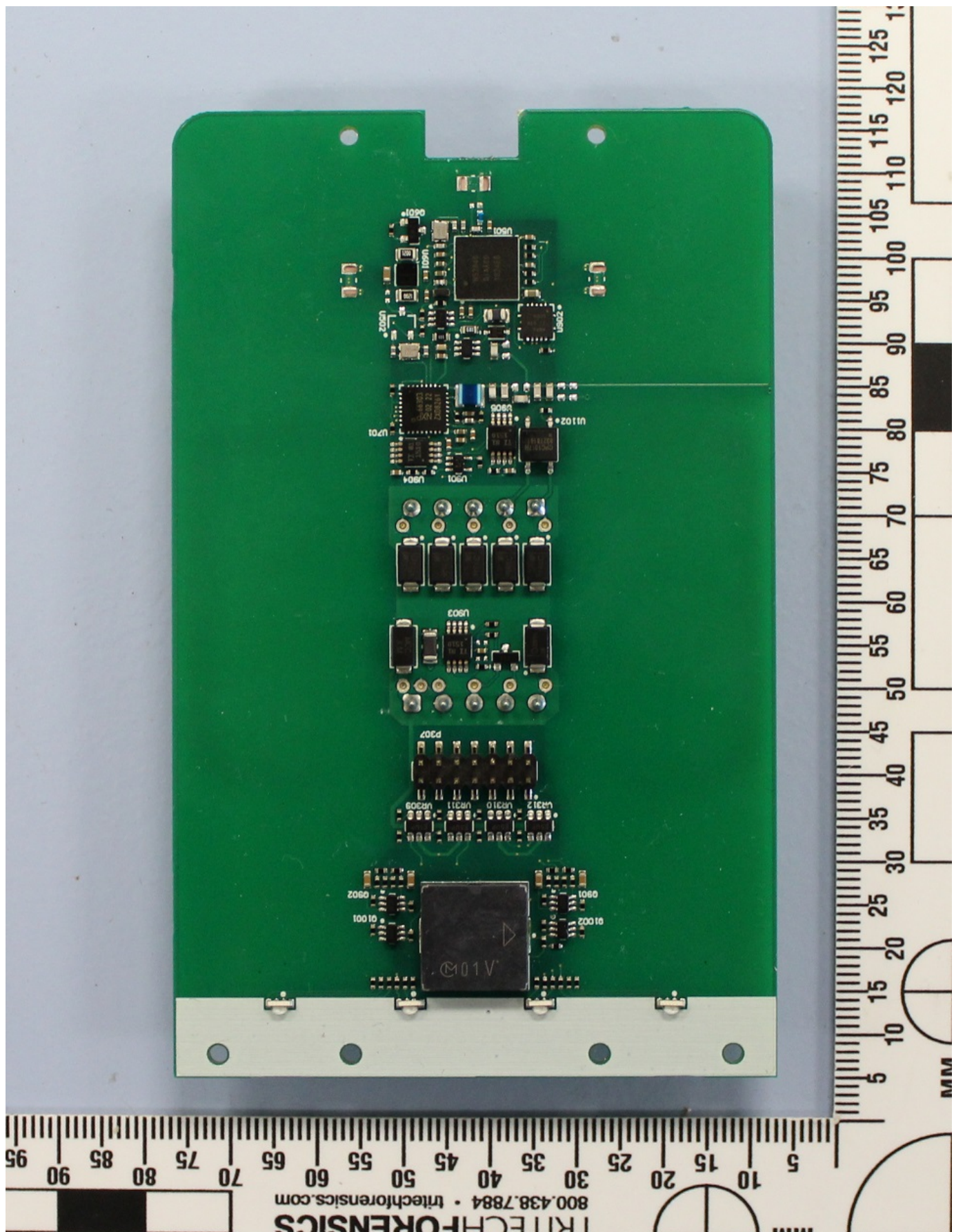
Model 40 (pigtail version) main board obverse without patch antenna
