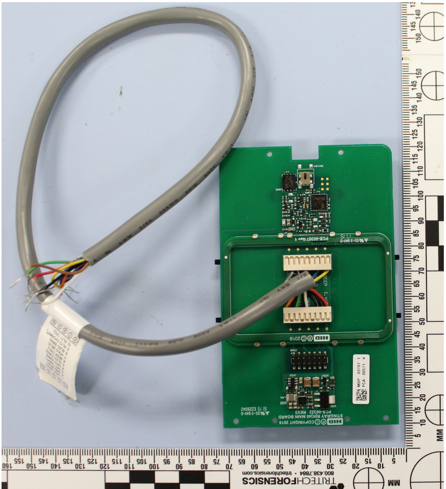
Model 40 (pigtail version) main board reverse
