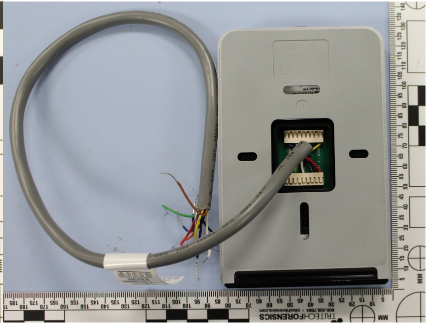
Model 40 (pigtail version) rear side
