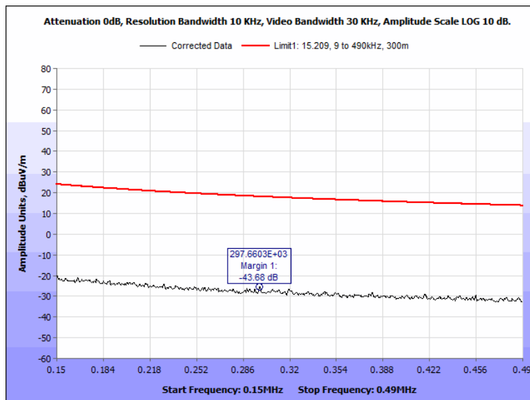
Figure 14: Radiated Spurious Emissions, Pigtail, 0.150 MHz – 0.490 MHz, 90 Deg
