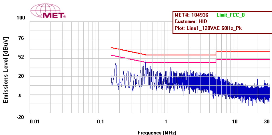
Figure 26: Conducted Emissions Limits, Pigtail, Phase Line, Prescan
