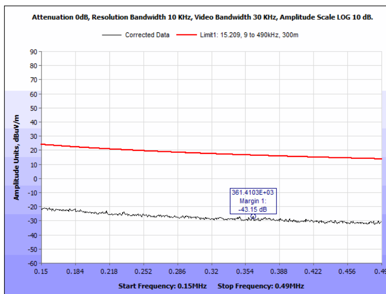
Figure 13: Radiated Spurious Emissions, Pigtail, 0.150 MHz – 0.490 MHz, 0 Deg
