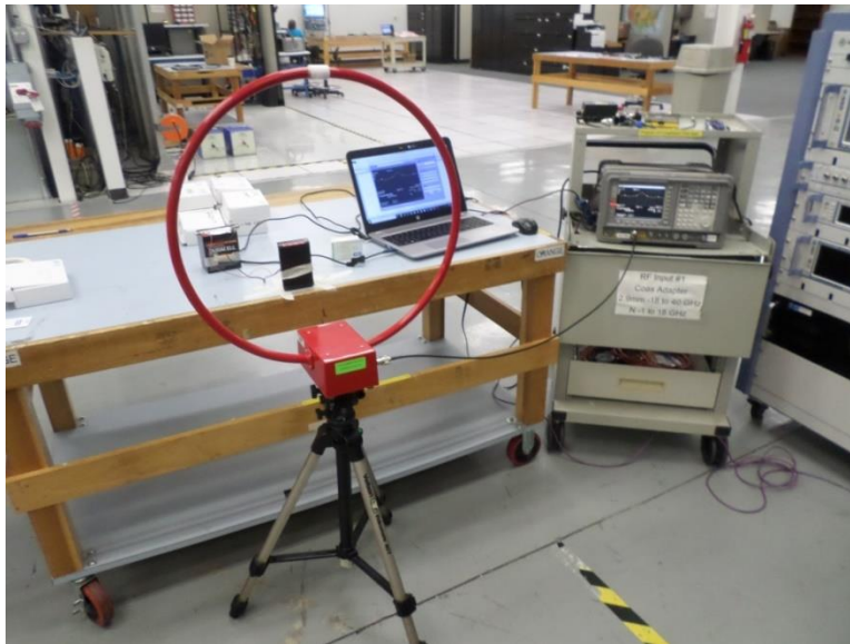
Figure 10: 20 dB Occupied Bandwidth, Terminal, Test Setup
