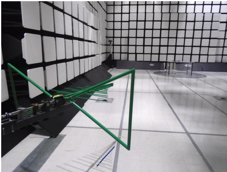
Figure 12: Radiated Spurious Emissions, 30 MHz – 1000 MHz, Test Setup
