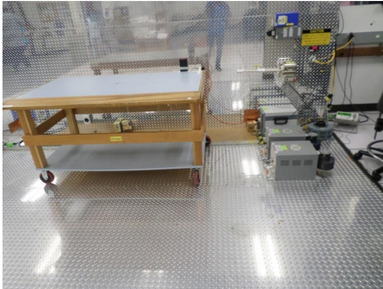
Figure 7: Conducted Emissions Limits, Terminal, Test Setup, Front View
