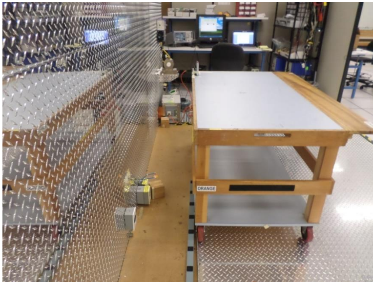
Figure 8: Conducted Emissions Limits, Terminal, Test Setup, Back View
