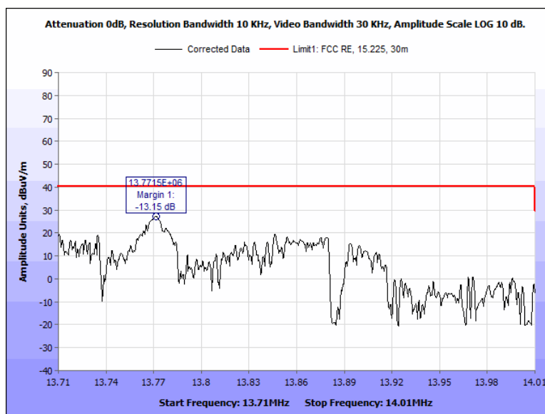
Figure 40: Spurious Emission Limits, within the bands 13.110 – 13.410 MHz and 13.710 – 14.010 MHz, Pigtail, 13.710 MHz – 14.010 MHz, 0 Deg
