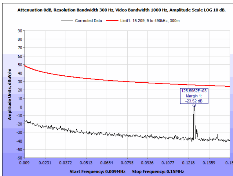
Figure 58: Spurious Emission Limits, outside the bands 13.110 – 14.010 MHz, Terminal, 0.009 MHz – 0.150 MHz, 0 Deg
