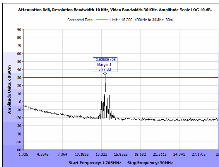
Figure 54: Spurious Emission Limits, outside the bands 13.110 – 14.010 MHz, Pigtail, High Frequency, 1.705 MHz – 30 MHz, 90 Deg
