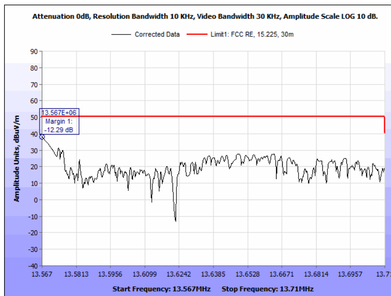
Figure 31: Spurious Emission Limits, within the bands 13.410 – 13.553 MHz and 13.567 – 13.710 MHz, Pigtail, 13.567 MHz – 13.710 MHz, 0 Deg
