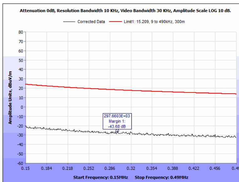
Figure 50: Spurious Emission Limits, outside the bands 13.110 – 14.010 MHz, Pigtail, 0.150 MHz – 0.490 MHz, 90 Deg
