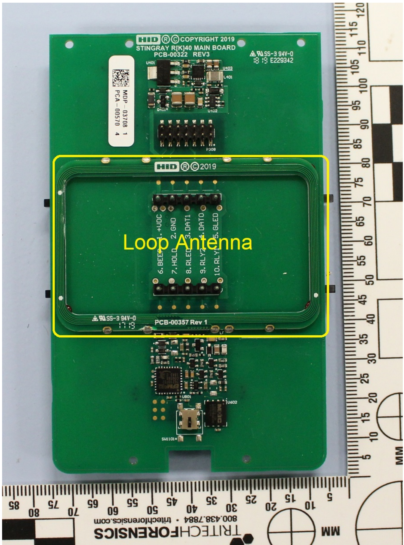
Model 40 and model 40K (terminal version shown) LF loop antenna – 125kHz
