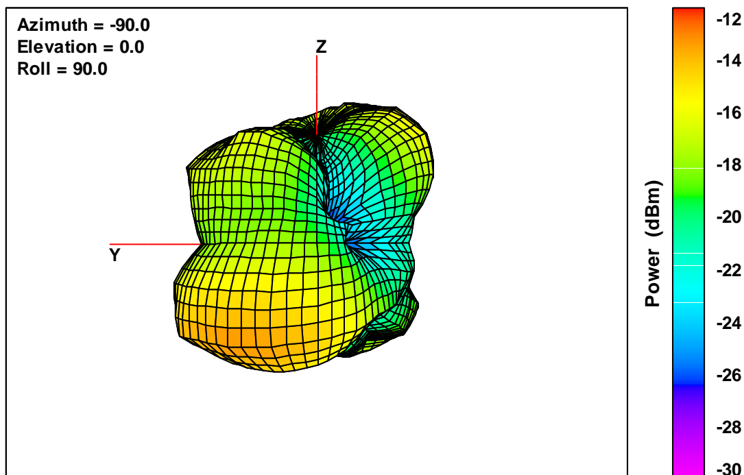
20 V2 Free-Space Total EIRP, Back Face View, 2402 MHz
