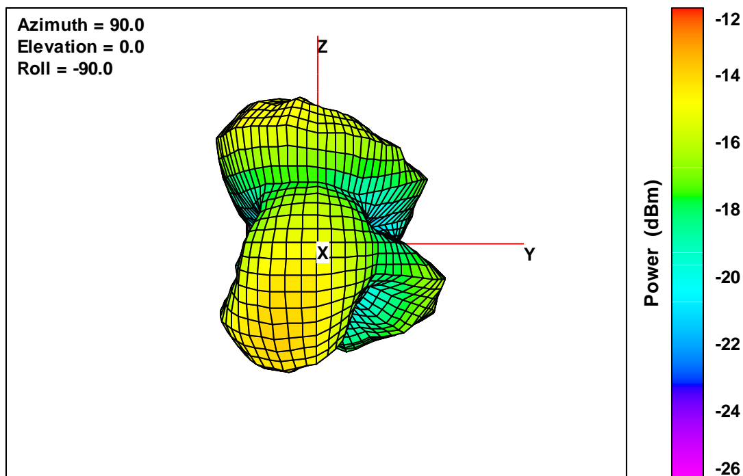
20 V2 Free-Space Total EIRP, Front Face View, 2482 MHz
