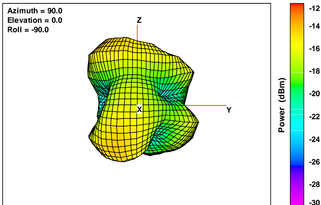
20 V2 Free-Space Total EIRP, Front Face View, 2402 MHz
