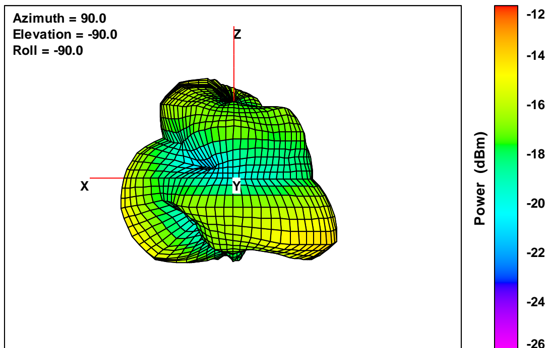
20 V2 Free-Space Total EIRP, Right Side View, 2482 MHz
