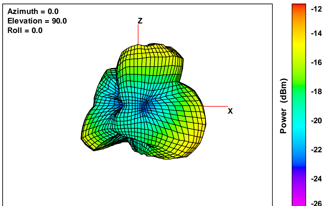
20 V2 Free-Space Total EIRP, Left Side View, 2482 MHz
