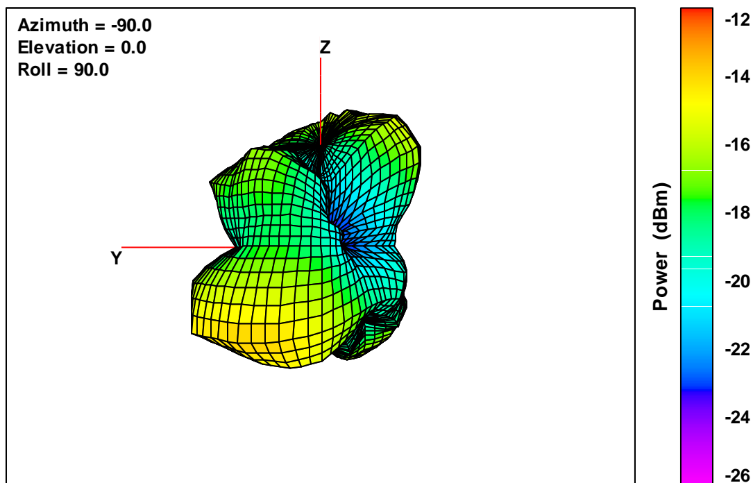
20 V2 Free-Space Total EIRP, Back Face View, 2482 MHz
