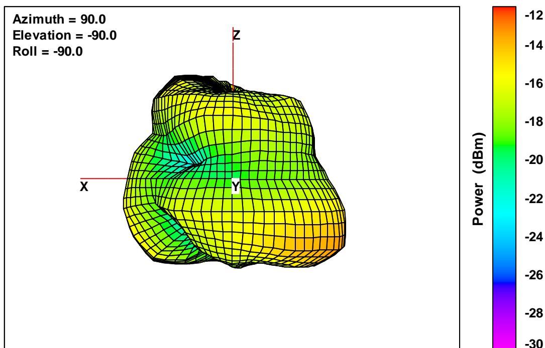
20 V2 Free-Space Total EIRP, Right Side View, 2402 MHz
