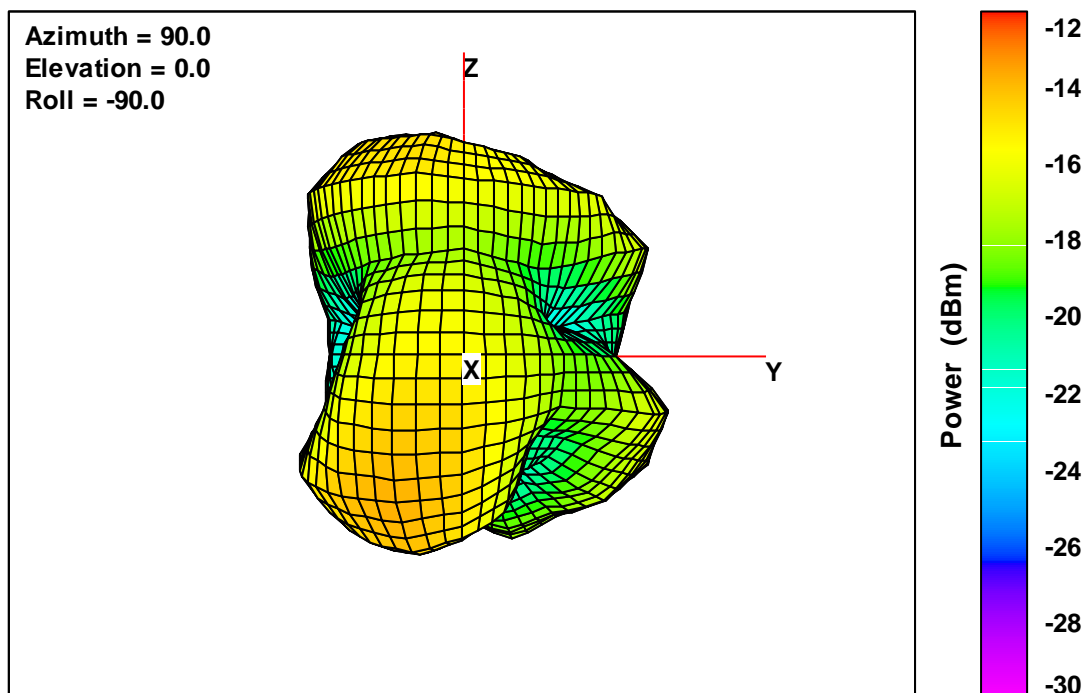
20 V2 Free-Space Total EIRP, Front Face View, 2442 MHz
