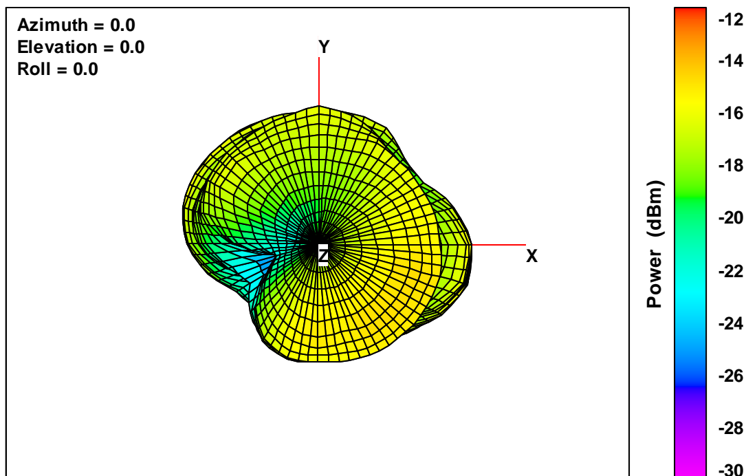
20 V2 Free-Space Total EIRP, Top View, 2442 MHz
