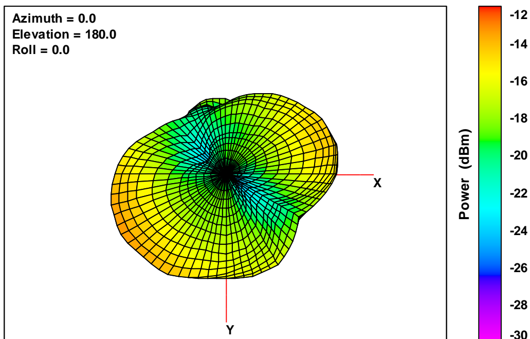
20 V2 Free-Space Total EIRP, Bottom View, 2402 MHz
