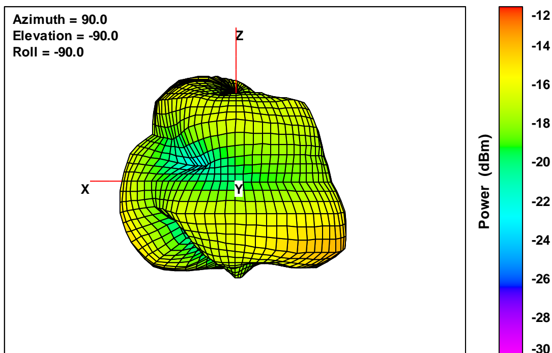
20 V2 Free-Space Total EIRP, Right Side View, 2442 MHz
