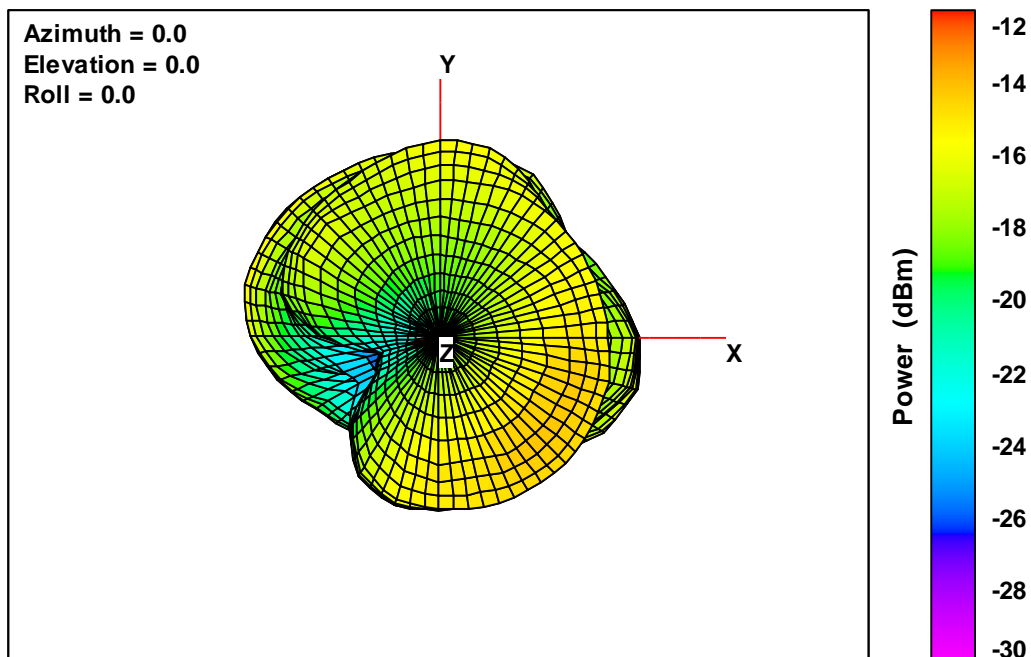
20 V2 Free-Space Total EIRP, Top View, 2402 MHz
