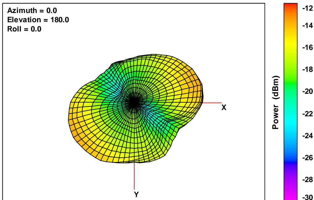
20 V2 Free-Space Total EIRP, Bottom View, 2442 MHz
