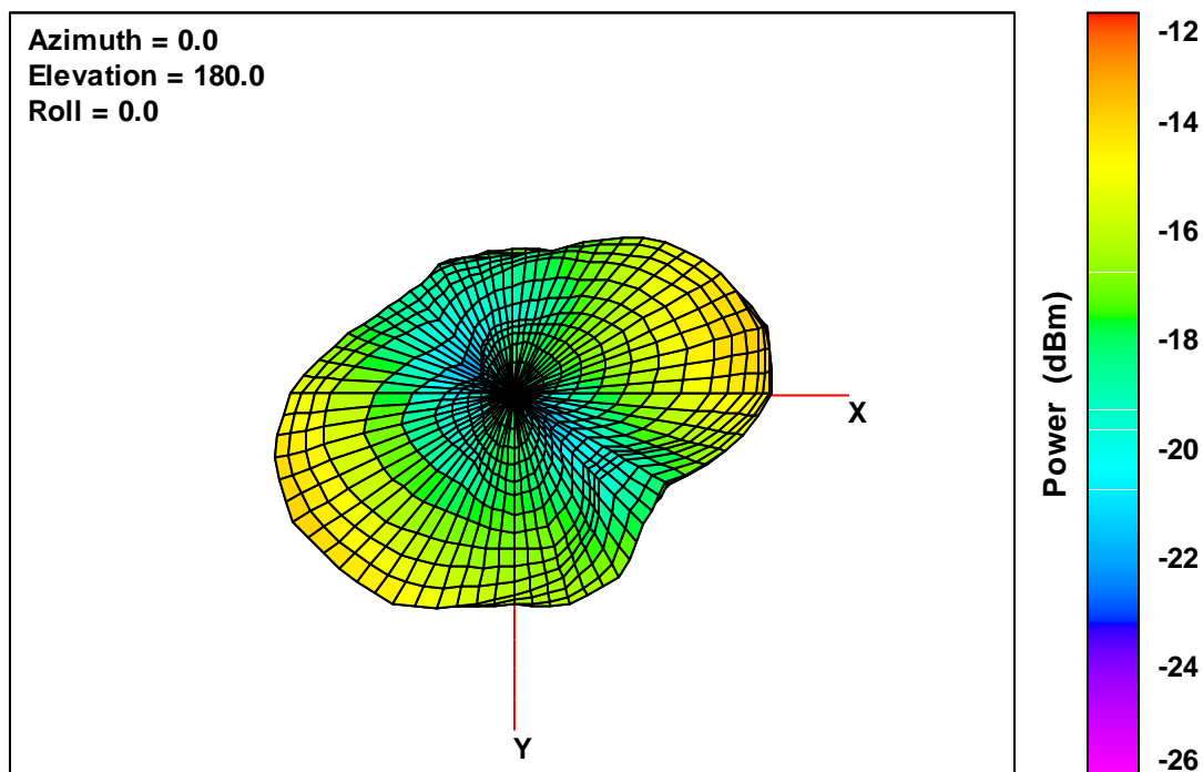
20 V2 Free-Space Total EIRP, Bottom View, 2482 MHz
