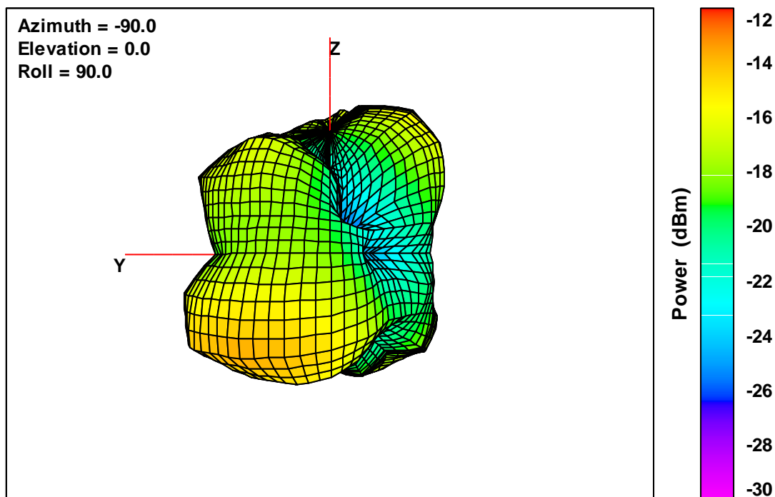
20 V2 Free-Space Total EIRP, Back Face View, 2442 MHz
