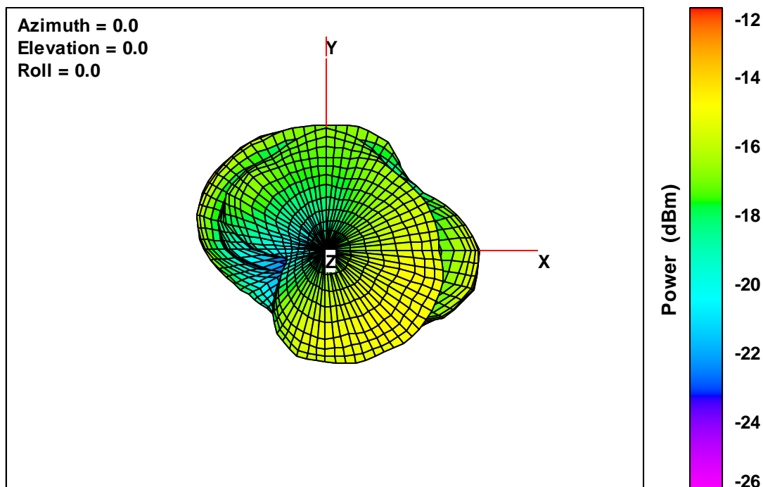
20 V2 Free-Space Total EIRP, Top View, 2482 MHz
