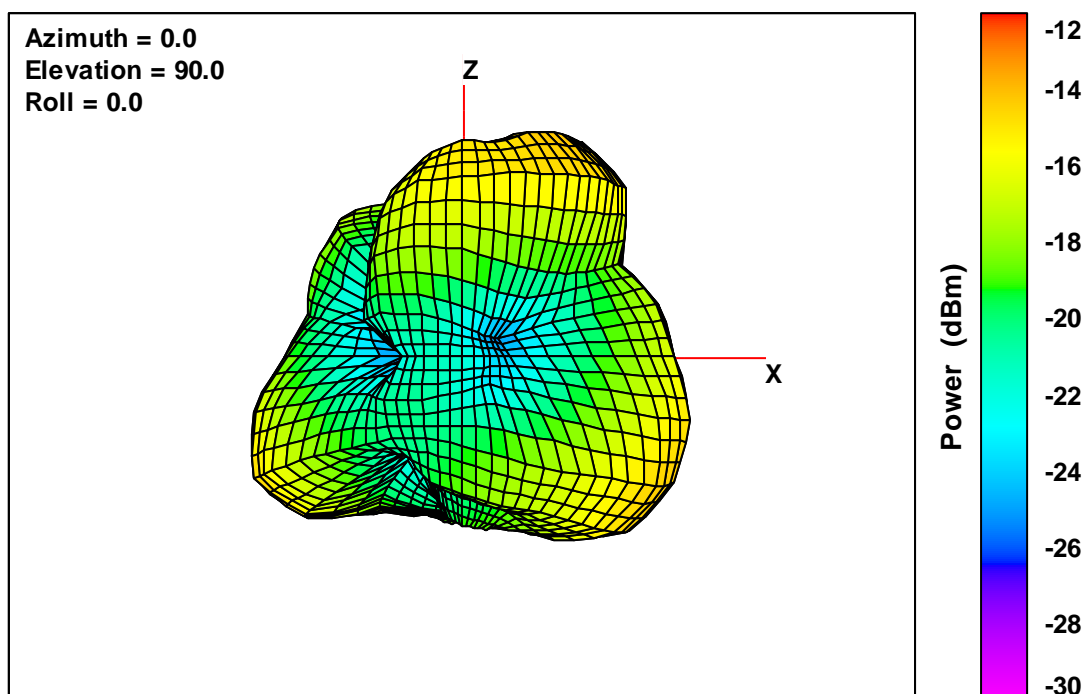
20 V2 Free-Space Total EIRP, Left Side View, 2402 MHz
