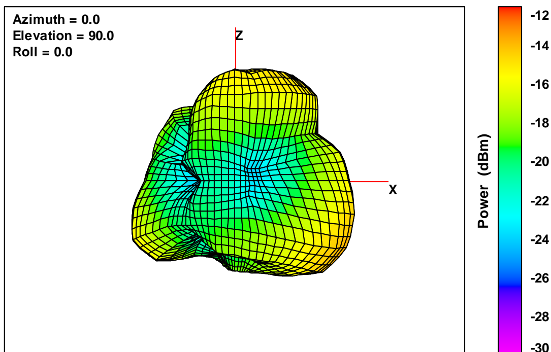
20 V2 Free-Space Total EIRP, Left Side View, 2442 MHz
