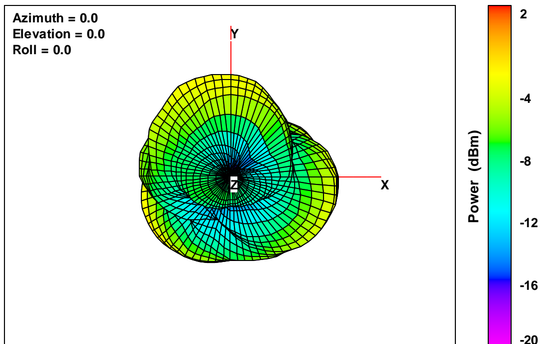
20K V2 Free-Space Total EIRP, Top View, 2442 MHz
