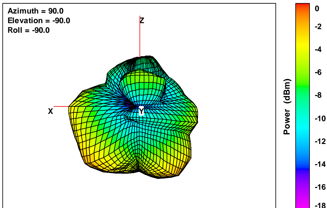
20K V2 Free-Space Total EIRP, Right Side View, 2402 MHz
