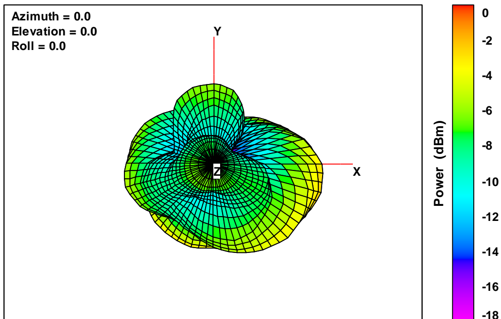
20K V2 Free-Space Total EIRP, Top View, 2402 MHz
