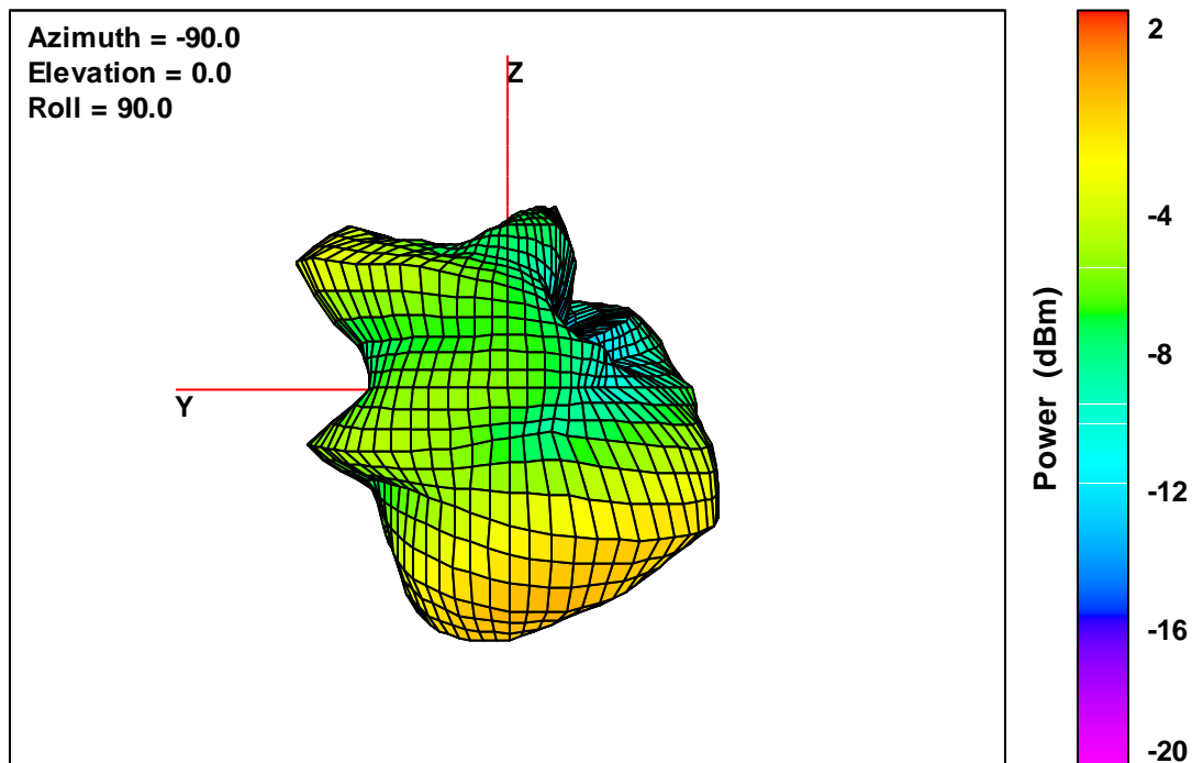
20K V2 Free-Space Total EIRP, Back Face View, 2442 MHz
