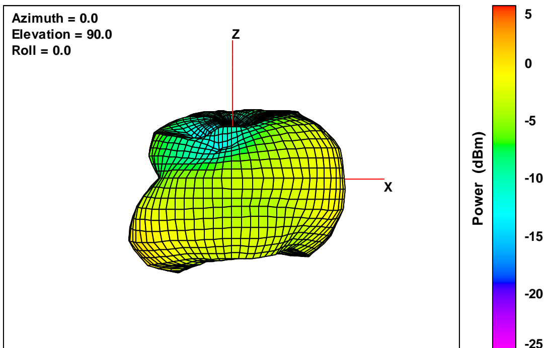
20K V2 Free-Space Total EIRP, Left Side View, 2482 MHz
