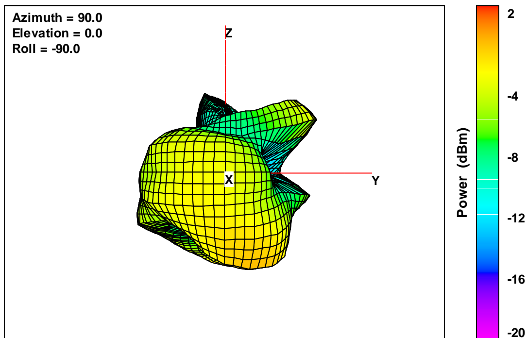
20K V2 Free-Space Total EIRP, Front Face View, 2442 MHz
