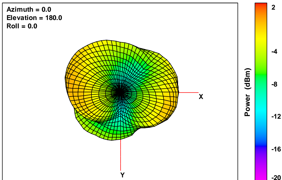
20K V2 Free-Space Total EIRP, Bottom View, 2442 MHz
