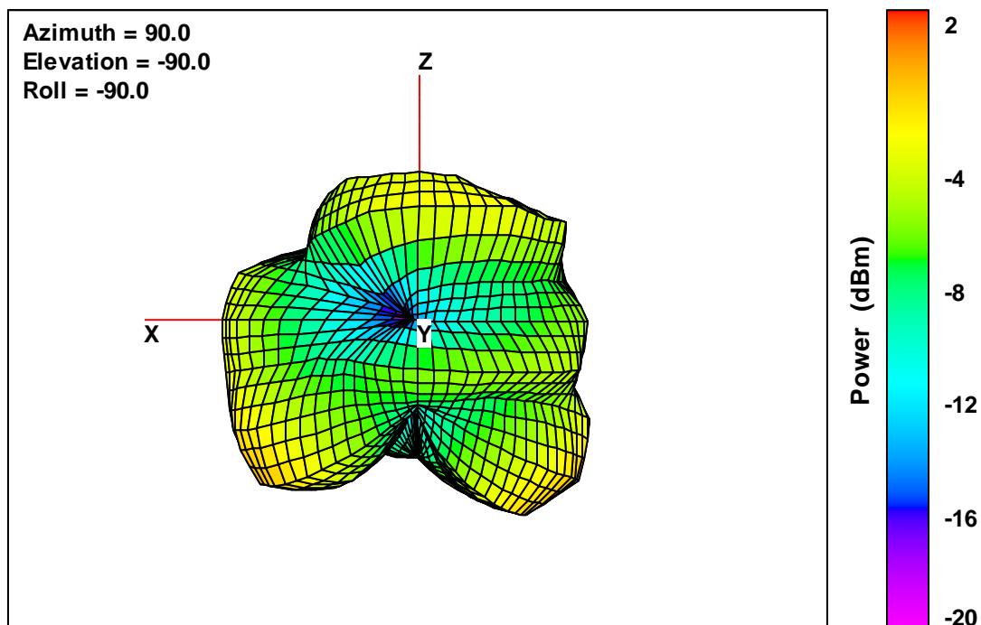
20K V2 Free-Space Total EIRP, Right Side View, 2442 MHz
