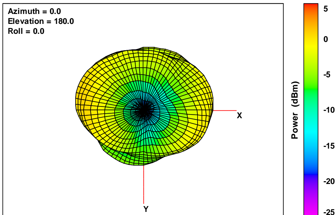
20K V2 Free-Space Total EIRP, Bottom View, 2482 MHz
