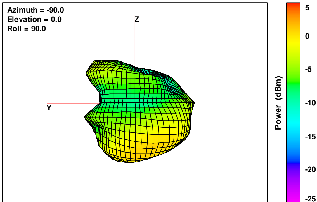
20K V2 Free-Space Total EIRP, Back Face View, 2482 MHz
