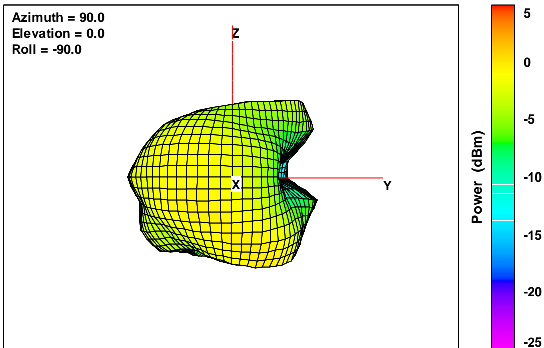
20K V2 Free-Space Total EIRP, Front Face View, 2482 MHz
