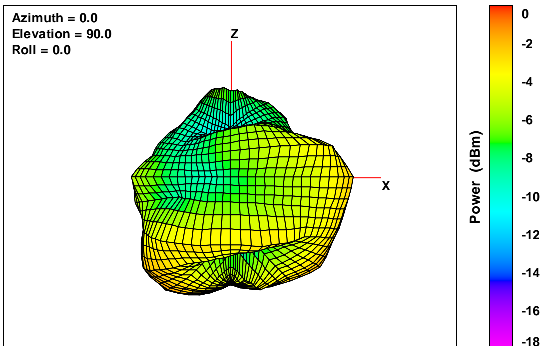
20K V2 Free-Space Total EIRP, Left Side View, 2402 MHz
