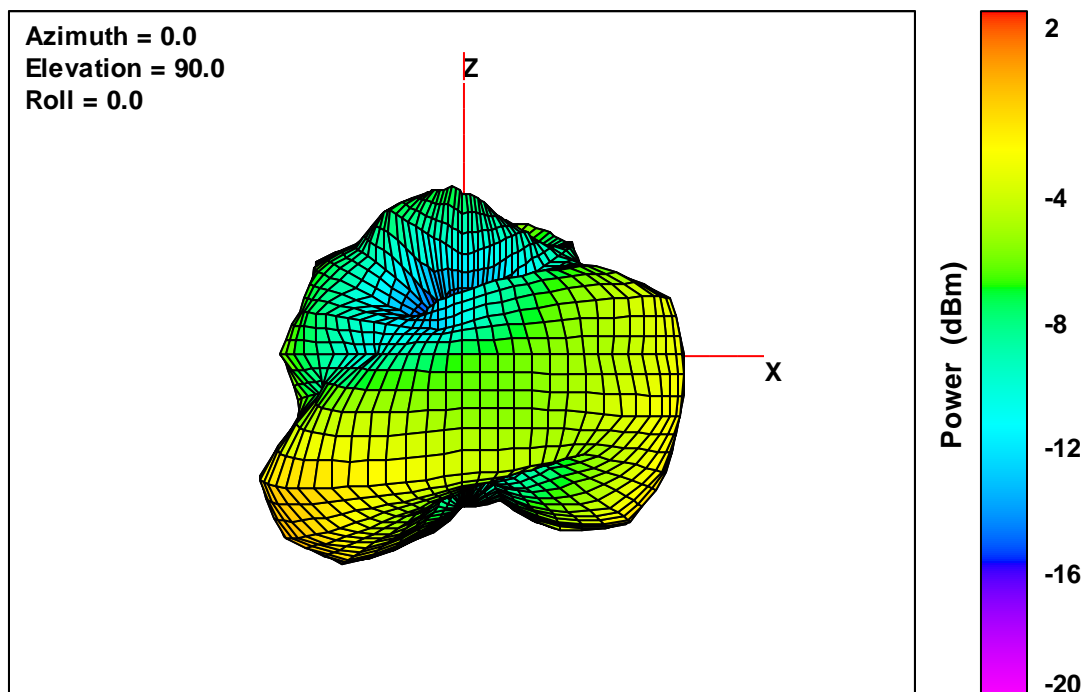
20K V2 Free-Space Total EIRP, Left Side View, 2442 MHz
