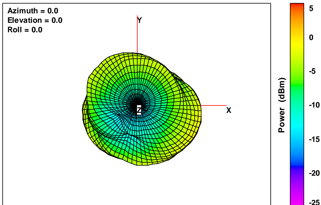
20K V2 Free-Space Total EIRP, Top View, 2482 MHz
