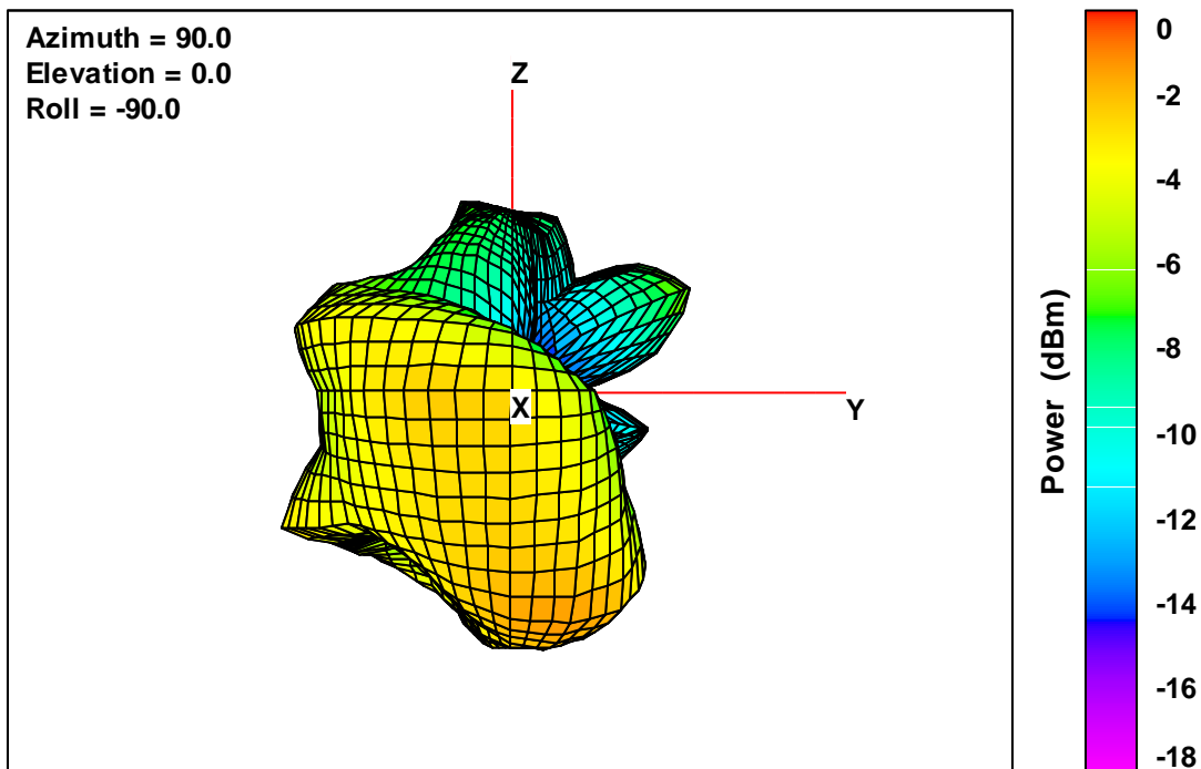
20K V2 Free-Space Total EIRP, Front Face View, 2402 MHz
