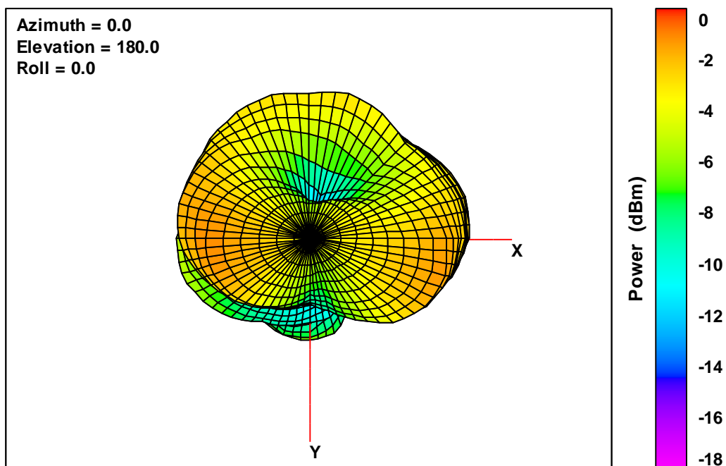
20K V2 Free-Space Total EIRP, Bottom View, 2402 MHz
