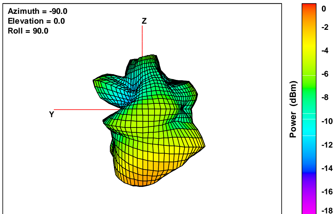
20K V2 Free-Space Total EIRP, Back Face View, 2402 MHz
