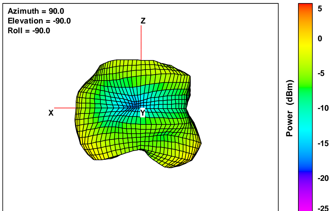
20K V2 Free-Space Total EIRP, Right Side View, 2482 MHz
