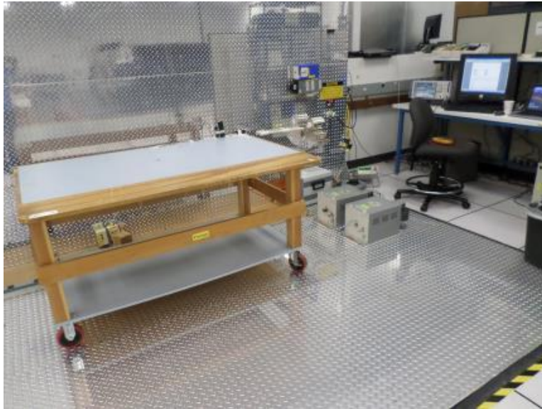
Figure 3: Conducted Emissions Limits, Pigtail, Front View, Test Setup
