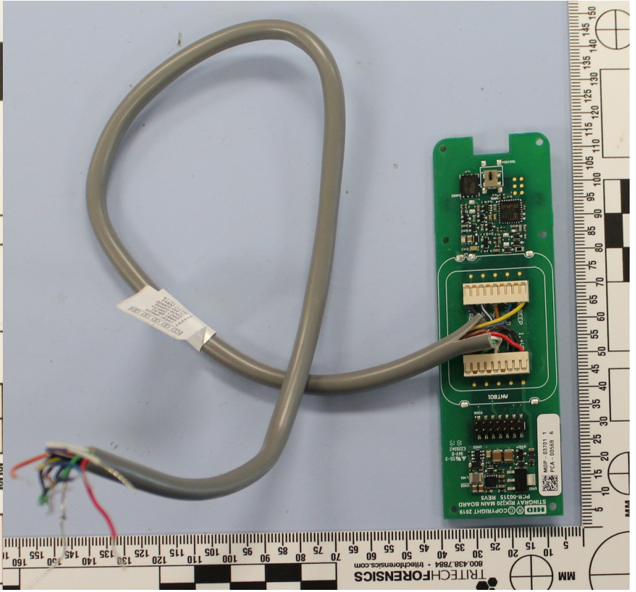
Model 20K (pigtail version) main board reverse
