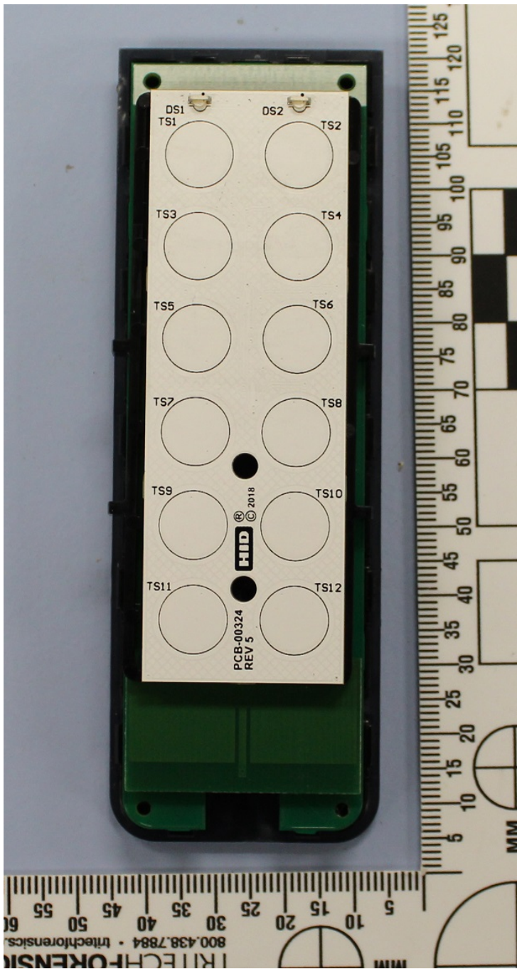
Model 20K (pigtail version) keypad obverse
