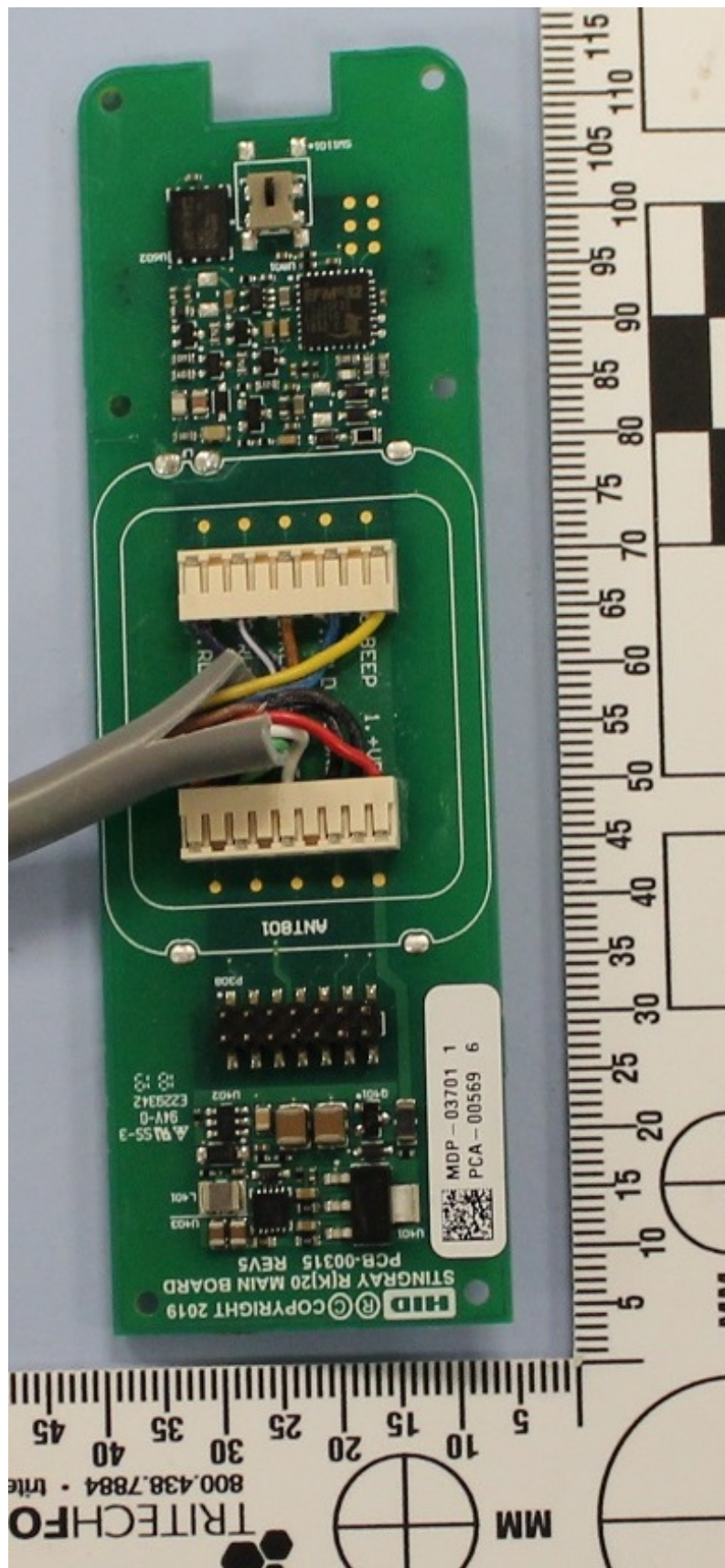
Model 20K (pigtail version) main board reverse detail
