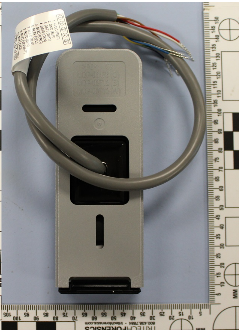
Model 20K (pigtail version) rear side
