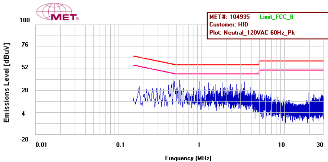
Figure 16: Conducted Emissions Limits, Terminal, Neutral Line, Prescan
