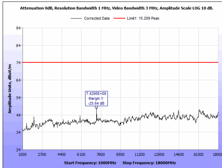
Figure 72: Radiated Spurious Emissions, Pigtail, 2480 MHz, 1 GHz - 18 GHz, Peak, Vertical
