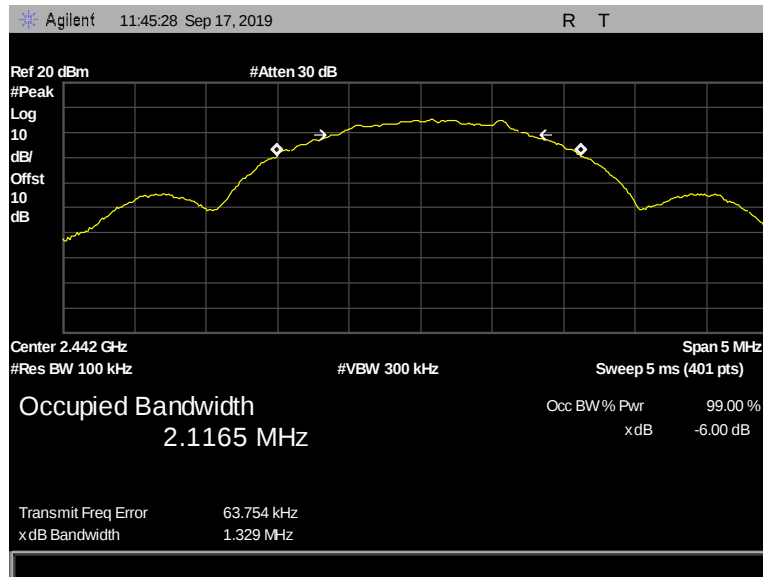
Figure 23: 6 dB Bandwidth, Pigtail, 2442 MHz, 2 Mbps, 1.329 MHz
