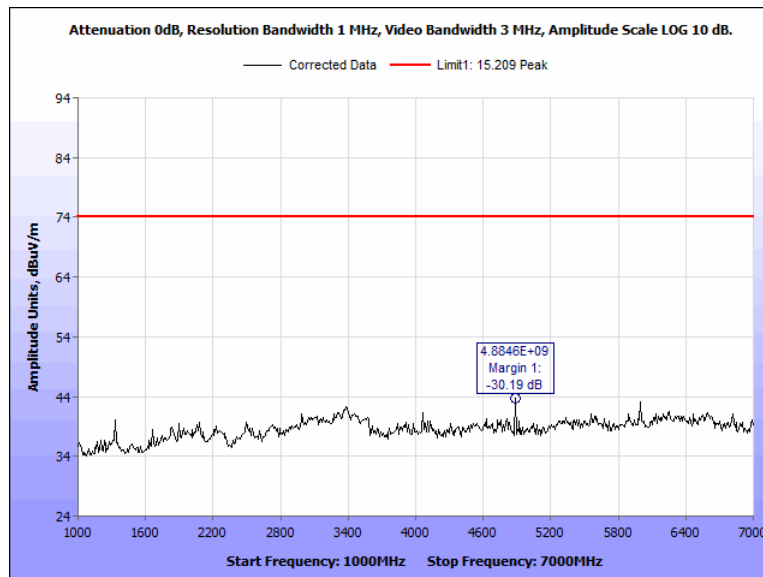
Figure 100: Radiated Spurious Emissions, Terminal, 2442 MHz, 1 GHz - 7 GHz, Peak, Vertical
