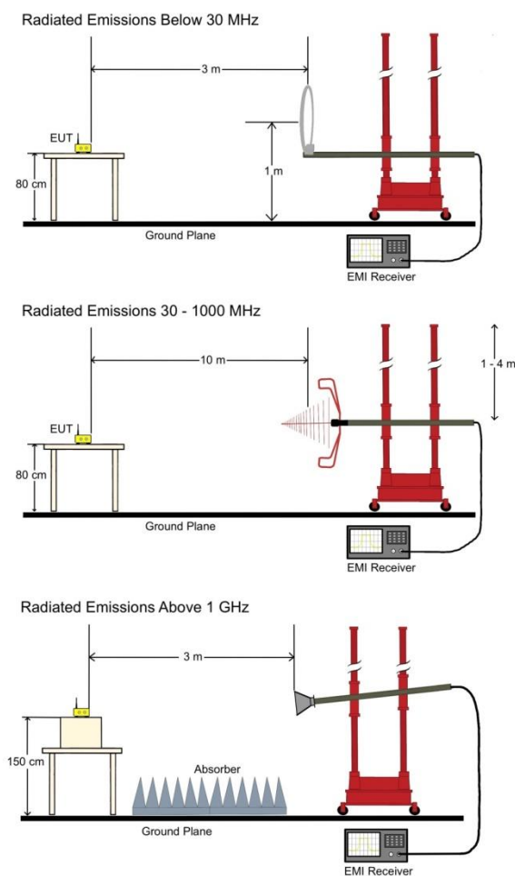
Figure 50. Radiated Emissions Test Setup
