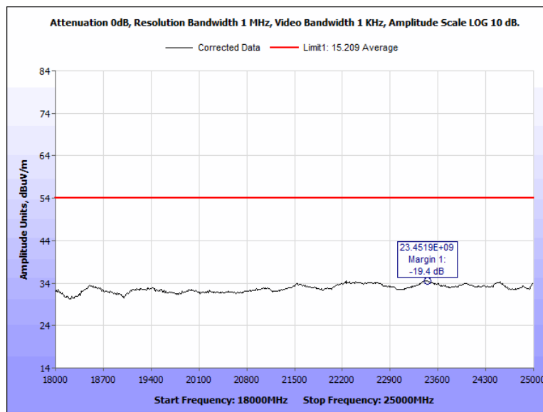
Figure 91: Radiated Spurious Emissions, Terminal, 2402 MHz, 18 GHz - 25 GHz, Average, Horizontal
