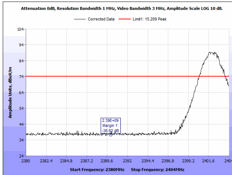
Figure 76: Radiated Band Edge, Pigtail, 2402 MHz, Peak, Vertical
