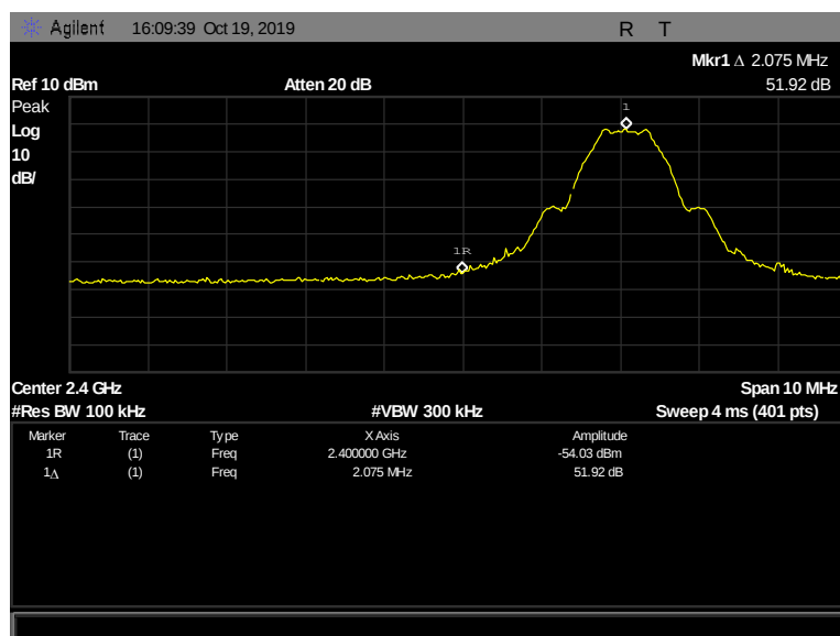
Figure 136: Conducted Band Edge, Pigtail, 2402 MHz, 1 Mbps
