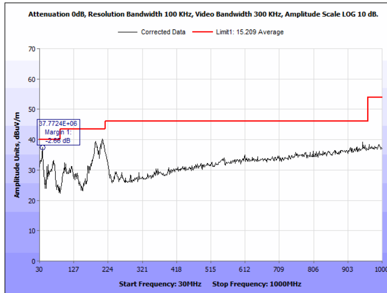
Figure 52: Radiated Spurious Emissions, Pigtail, 2402 MHz, 30 MHz - 1000 MHz, Vertical
