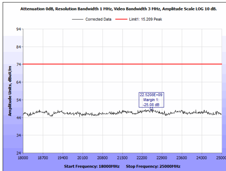
Figure 60: Radiated Spurious Emissions, Pigtail, 2402 MHz, 18 GHz - 25 GHz, Peak, Vertical
