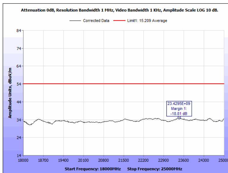
Figure 57: Radiated Spurious Emissions, Pigtail, 2402 MHz, 18 GHz - 25 GHz, Average, Vertical
