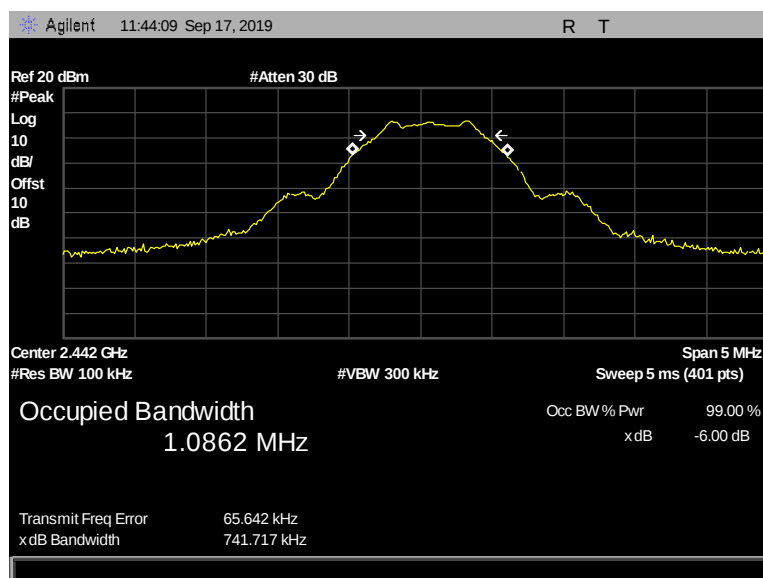
Figure 20: 6 dB Bandwidth, Pigtail, 2442 MHz, 1 Mbps, 741.717 kHz
