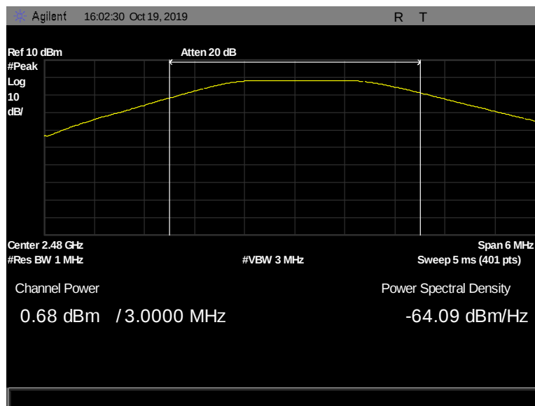
Figure 40: Peak Power Output, Pigtail, 2480 MHz, 2 Mbps, 0.68 dBm
