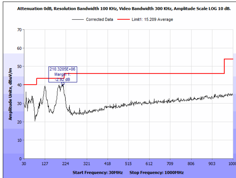
Figure 82: Radiated Spurious Emissions, Terminal, 2402 MHz, 30 MHz - 1000 MHz, Vertical
