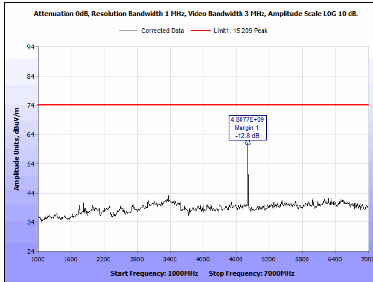
Figure 86: Radiated Spurious Emissions, Terminal, 2402 MHz, 1 GHz - 7 GHz, Peak, Vertical
