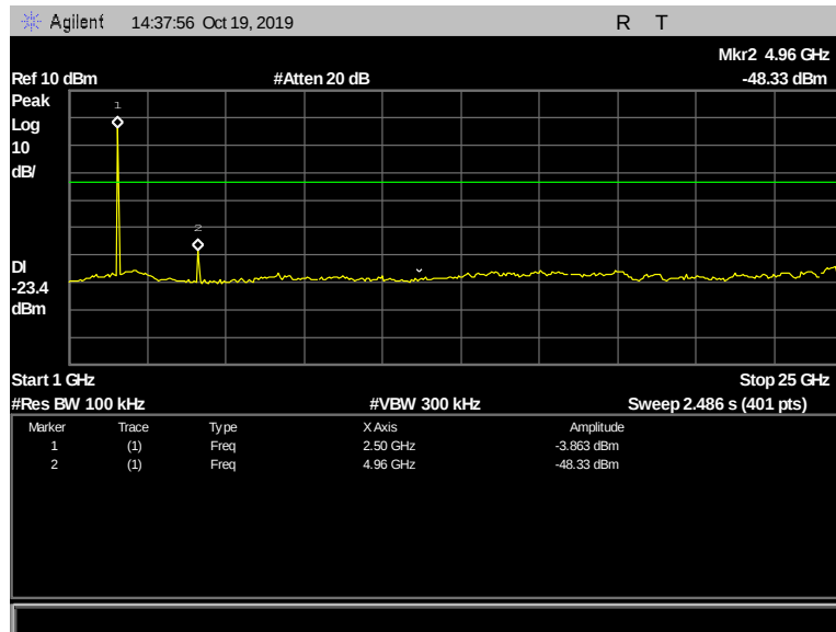
Figure 145: Conducted Spurious Emissions, Terminal, 2442 MHz, 1 Mbps, 1 GHz - 25 GHz
