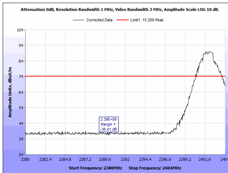
Figure 75: Radiated Band Edge, Pigtail, 2402 MHz, Peak, Horizontal
