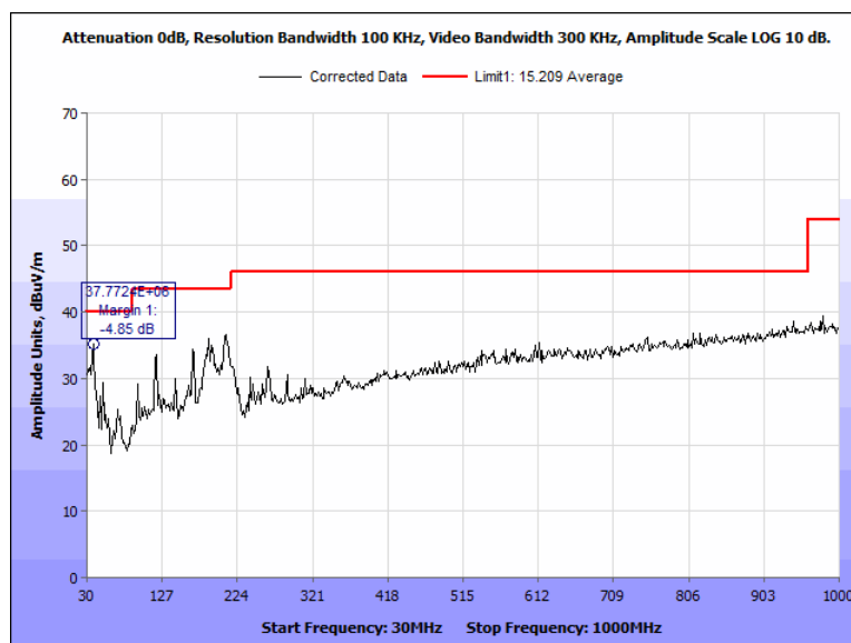
Figure 61: Radiated Spurious Emissions, Pigtail, 2442 MHz, 30 MHz - 1000 MHz, Horizontal
