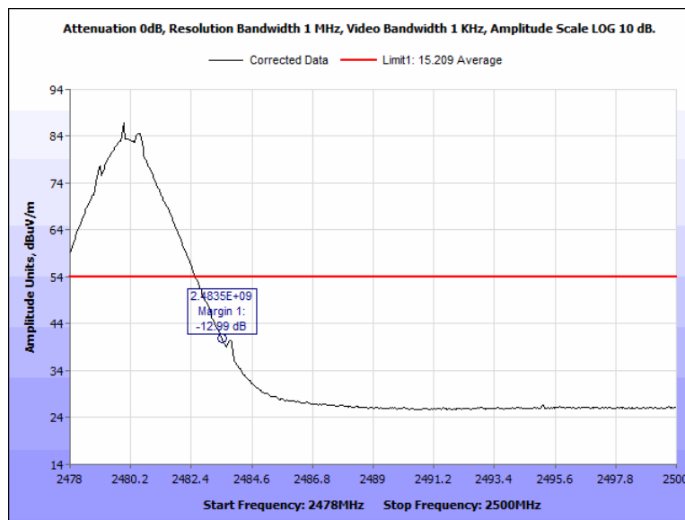
Figure 77: Radiated Band Edge, Pigtail, 2480 MHz, Average, Horizontal
