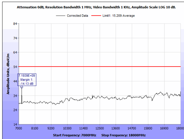
Figure 88: Radiated Spurious Emissions, Terminal, 2402 MHz, 7 GHz - 18 GHz, Average, Vertical
