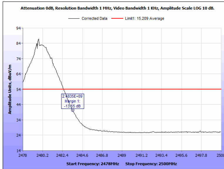
Figure 120: Radiated Band Edge, Terminal, 2480 MHz, Average, Vertical
