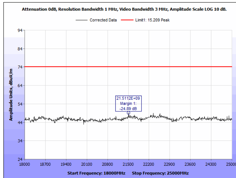
Figure 94: Radiated Spurious Emissions, Terminal, 2402 MHz, 18 GHz - 25 GHz, Peak, Vertical
