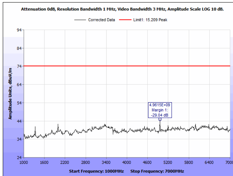
Figure 110: Radiated Spurious Emissions, Terminal, 2480 MHz, 1 GHz - 7 GHz, Peak, Vertical
