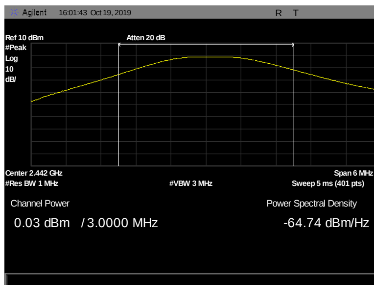
Figure 36: Peak Power Output, Pigtail, 2442 MHz, 1 Mbps, 0.03 dBm
