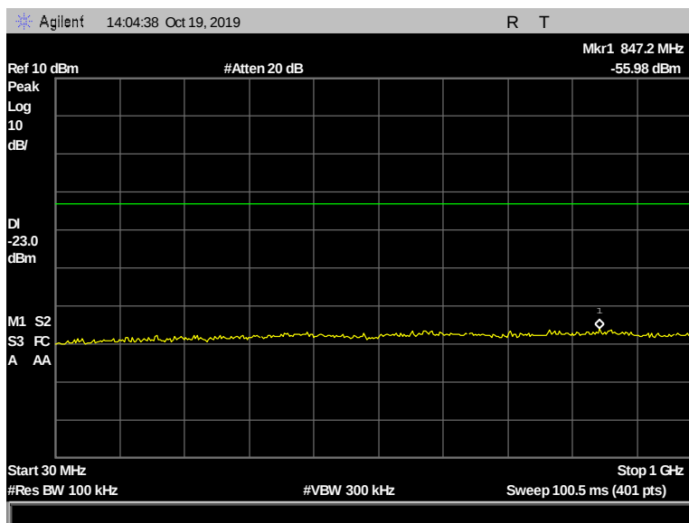
Figure 140: Conducted Spurious Emissions, Terminal, 2402 MHz, 1 Mbps, 30 MHz - 1000 MHz
