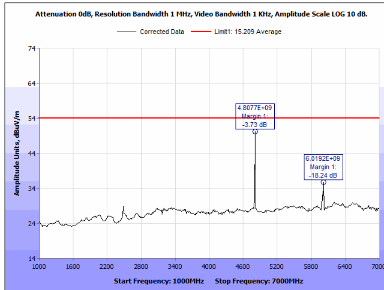
Figure 84: Radiated Spurious Emissions, Terminal, 2402 MHz, 1 GHz - 7 GHz, Average, Vertical
