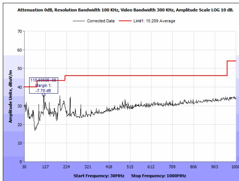
Figure 105: Radiated Spurious Emissions, Terminal, 2480 MHz, 30 MHz - 1000 MHz, Horizontal
