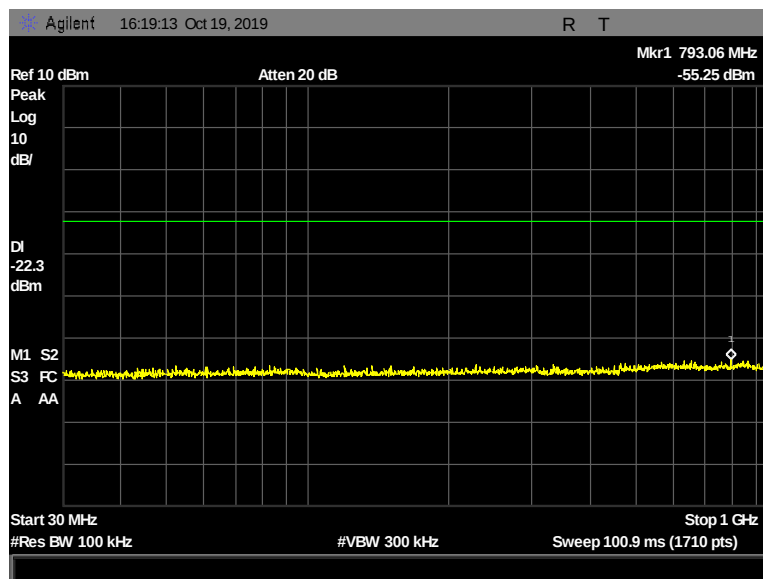
Figure 128: Conducted Spurious Emissions, Pigtail, 2480 MHz, 1 Mbps, 30 MHz - 1000 MHz
