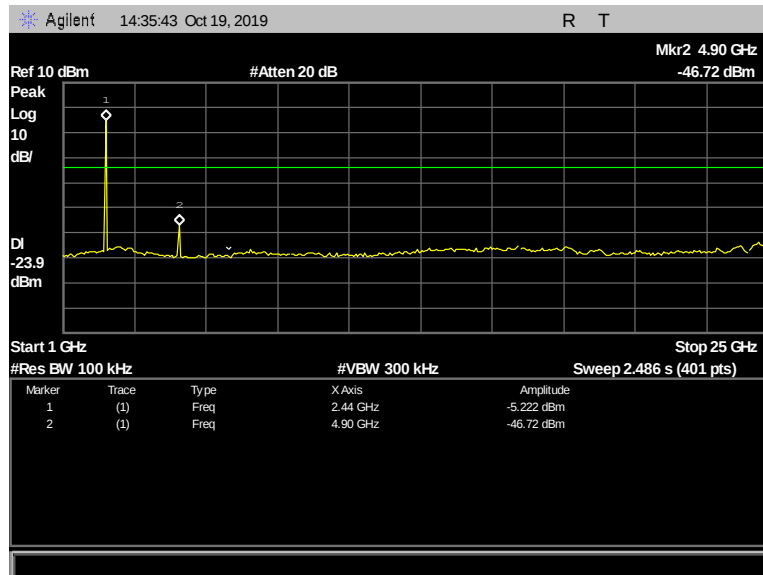
Figure 149: Conducted Spurious Emissions, Terminal, 2442 MHz, 2 Mbps, 1 GHz - 25 GHz
