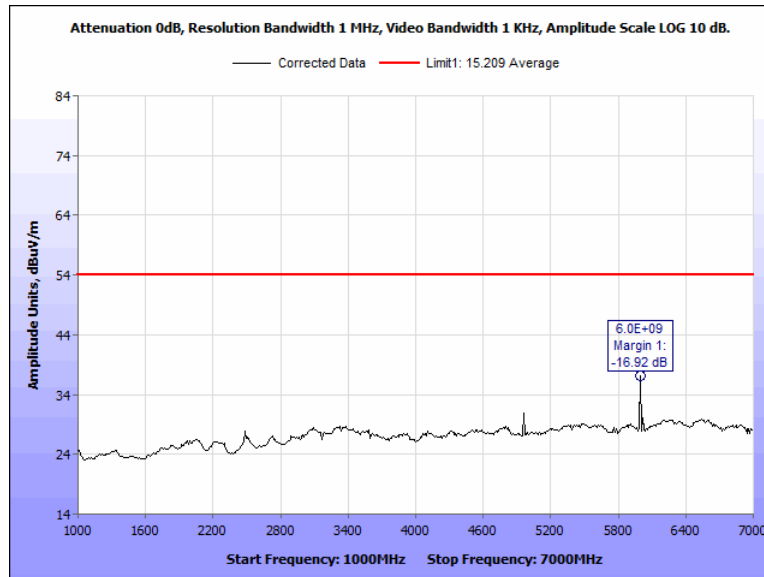
Figure 108: Radiated Spurious Emissions, Terminal, 2480 MHz, 1 GHz - 7 GHz, Average, Horizontal
