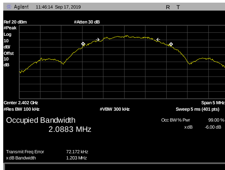
Figure 22: 6 dB Bandwidth, Pigtail, 2402 MHz, 2 Mbps, 1.203 MHz
