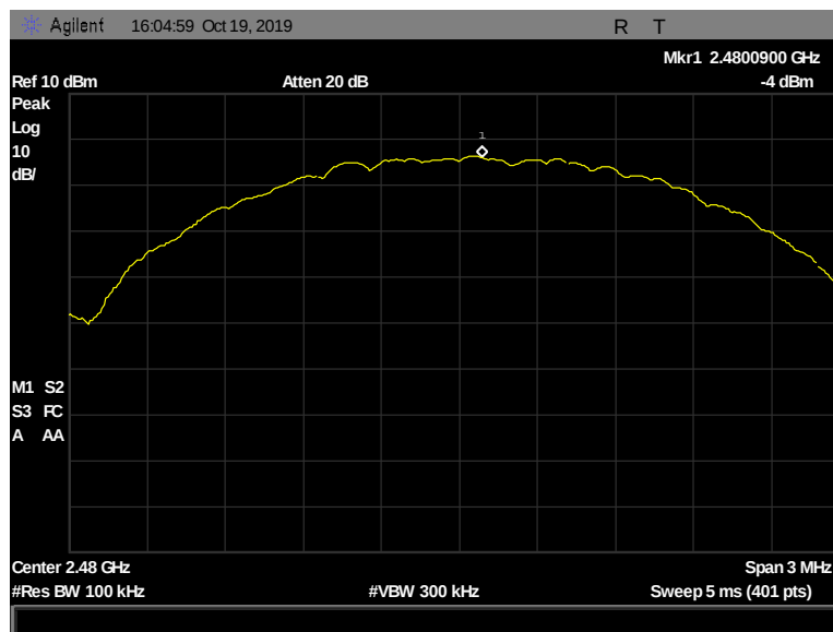
Figure 163: Peak Power Spectral Density, Pigtail, 2480 MHz, 2 Mbps, -4.000 dBm
