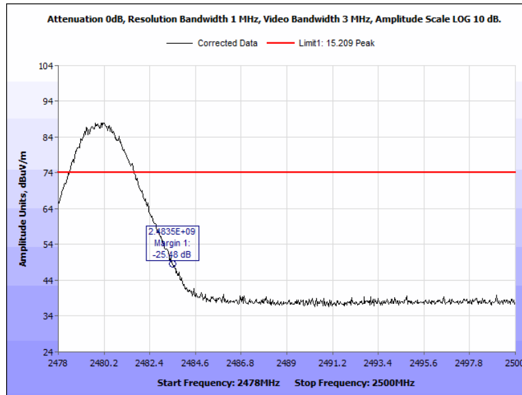
Figure 80: Radiated Band Edge, Pigtail, 2480 MHz, Peak, Vertical
