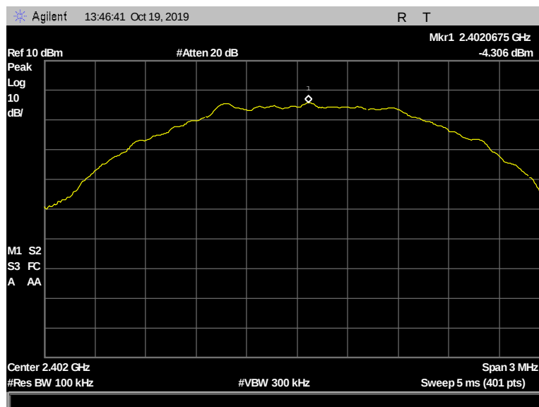
Figure 168: Peak Power Spectral Density, Terminal, 2402 MHz, 2 Mbps, -4.306 dBm
