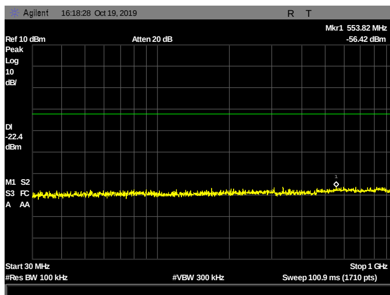
Figure 132: Conducted Spurious Emissions, Pigtail, 2442 MHz, 2 Mbps, 30 MHz - 1000 MHz
