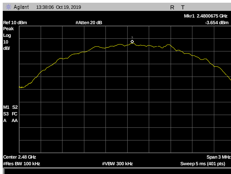
Figure 170: Peak Power Spectral Density, Terminal, 2480 MHz, 2 Mbps, -3.654 dBm
