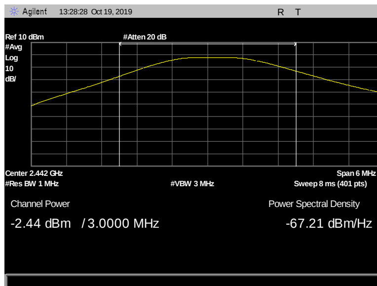
Figure 43: Peak Power Output, Terminal, 2442 MHz, 1 Mbps, -2.44 dBm
