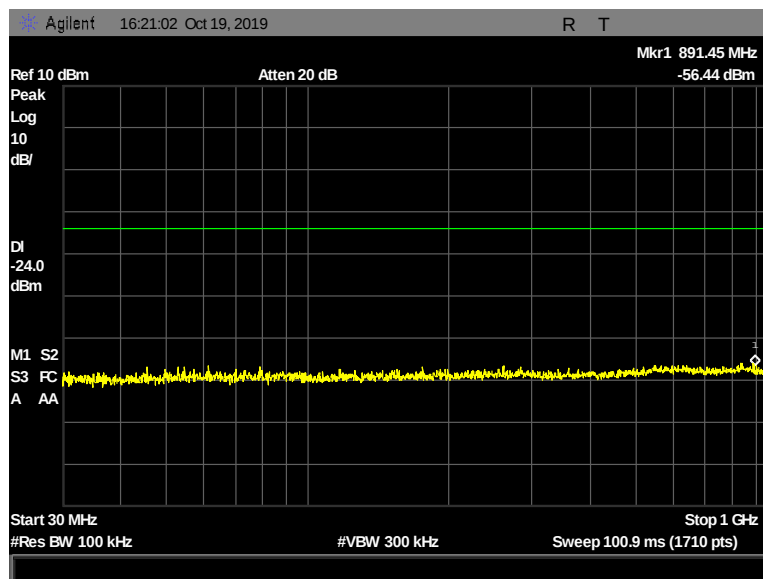
Figure 134: Conducted Spurious Emissions, Pigtail, 2480 MHz, 2 Mbps, 30 MHz - 1000 MHz
