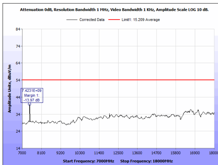
Figure 111: Radiated Spurious Emissions, Terminal, 2480 MHz, 7 GHz - 18 GHz, Average, Horizontal
