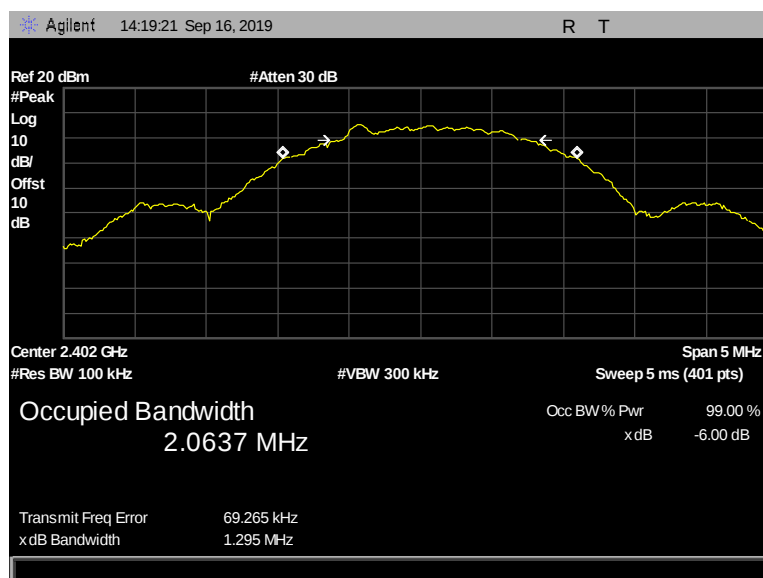
Figure 29: 6 dB Bandwidth, Terminal, 2402 MHz, 2 Mbps, 1.295 MHz
