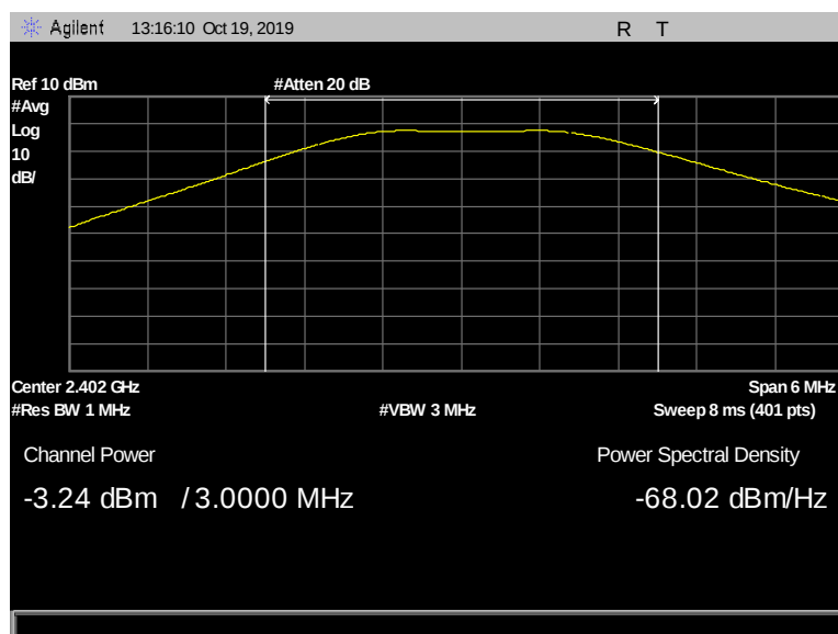
Figure 45: Peak Power Output, Terminal, 2402 MHz, 2 Mbps, -3.24 dBm
