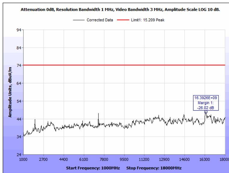
Figure 65: Radiated Spurious Emissions, Pigtail, 2442 MHz, 1 GHz - 18 GHz, Peak, Horizontal
