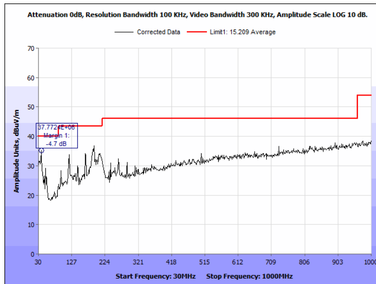
Figure 51: Radiated Spurious Emissions, Pigtail, 2402 MHz, 30 MHz - 1000 MHz, Horizontal
