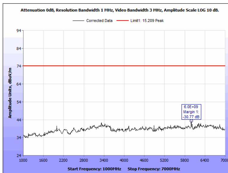
Figure 99: Radiated Spurious Emissions, Terminal, 2442 MHz, 1 GHz - 7 GHz, Peak, Horizontal
