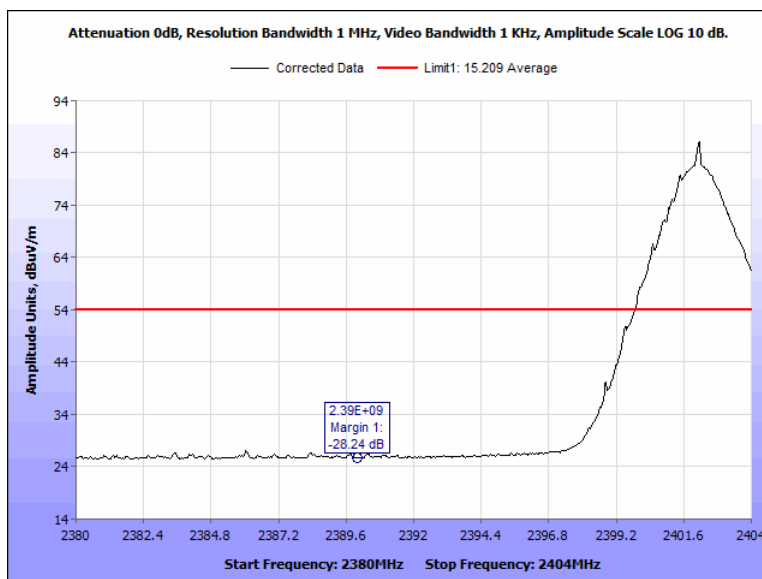
Figure 115: Radiated Band Edge, Terminal, 2402 MHz, Average, Horizontal
