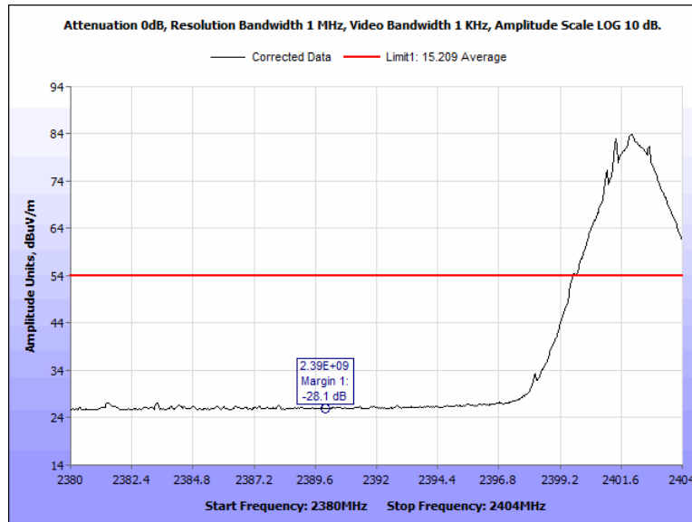
Figure 116: Radiated Band Edge, Terminal, 2402 MHz, Average, Vertical
