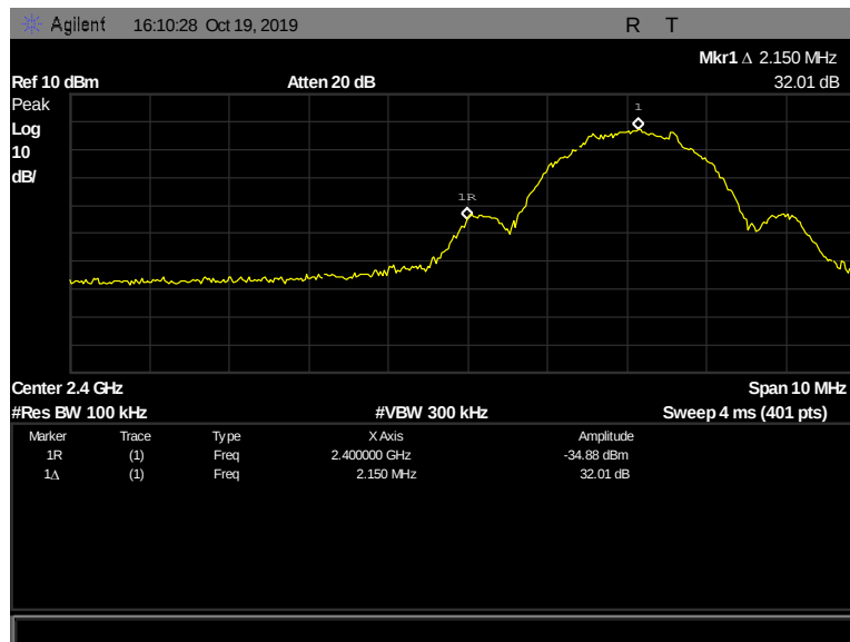
Figure 137: Conducted Band Edge, Pigtail, 2402 MHz, 2 Mbps
