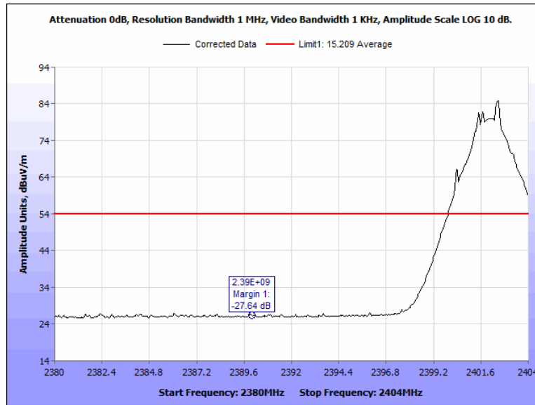
Figure 74: Radiated Band Edge, Pigtail, 2402 MHz, Average, Vertical
