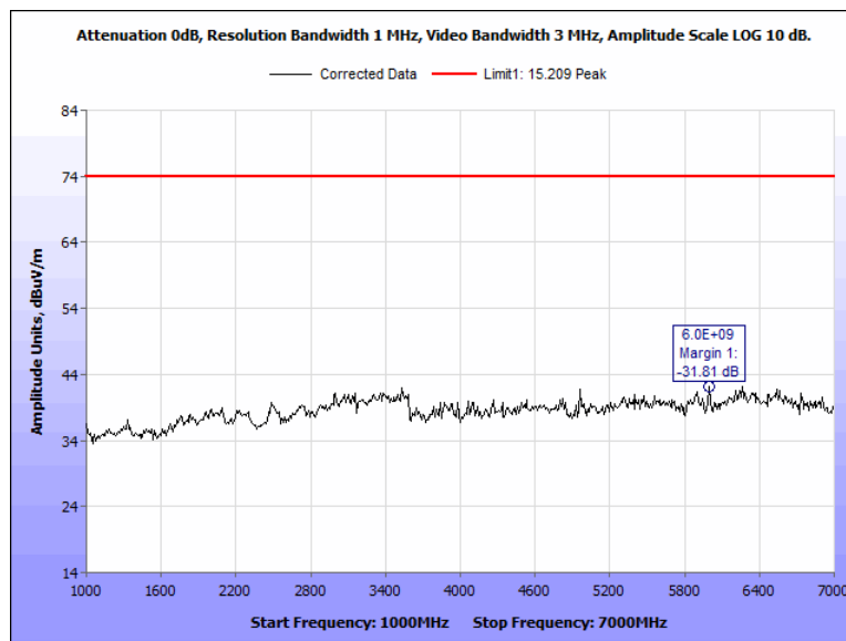
Figure 109: Radiated Spurious Emissions, Terminal, 2480 MHz, 1 GHz - 7 GHz, Peak, Horizontal
