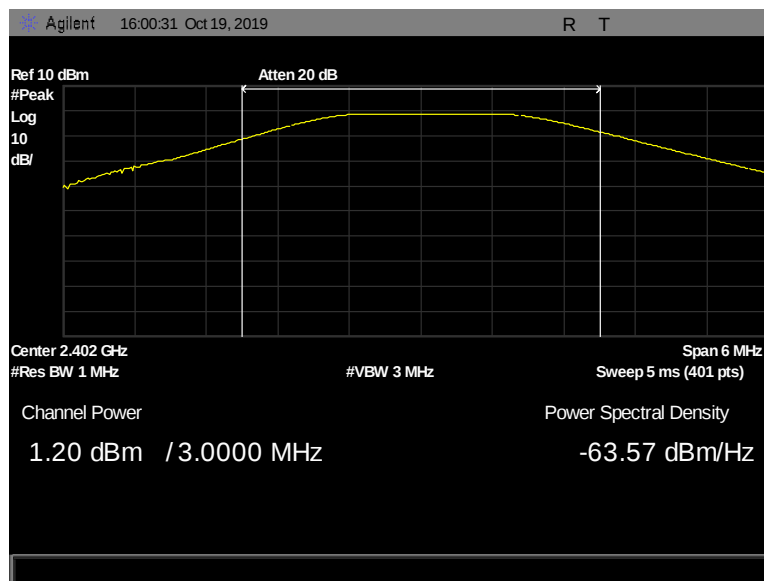
Figure 38: Peak Power Output, Pigtail, 2402 MHz, 2 Mbps, 1.20 dBm
