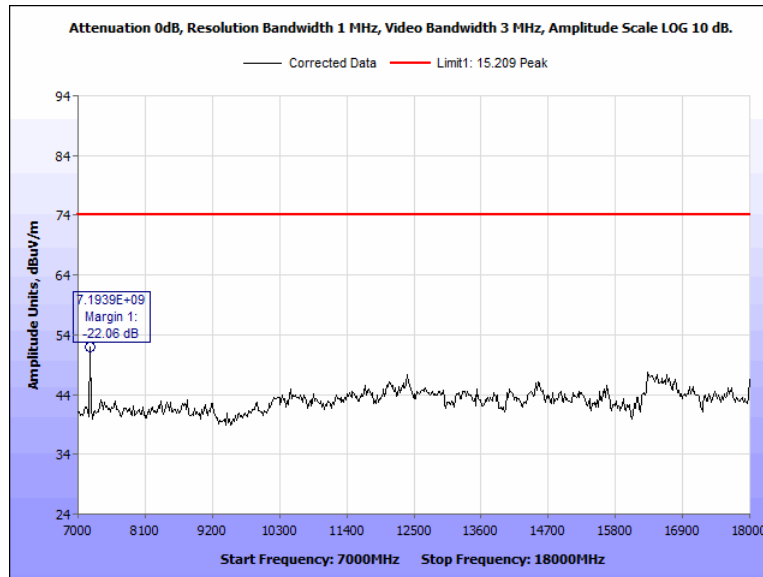
Figure 90: Radiated Spurious Emissions, Terminal, 2402 MHz, 7 GHz - 18 GHz, Peak, Vertical
