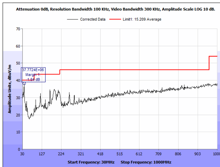
Figure 67: Radiated Spurious Emissions, Pigtail, 2480 MHz, 30 MHz - 1000 MHz, Horizontal
