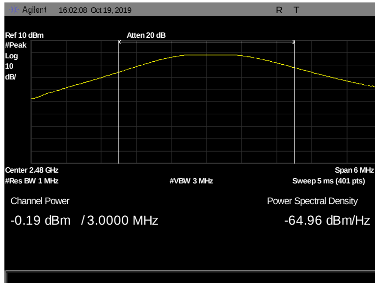
Figure 37: Peak Power Output, Pigtail, 2480 MHz, 1 Mbps, -0.19 dBm
