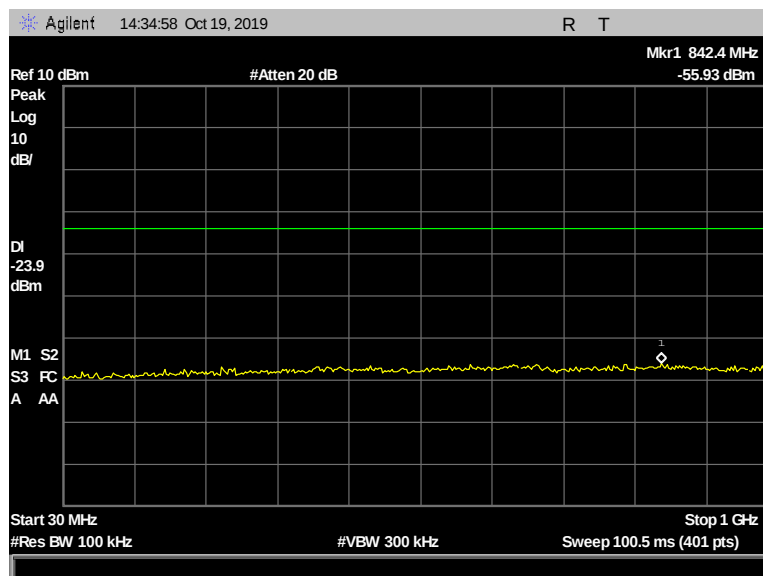
Figure 148: Conducted Spurious Emissions, Terminal, 2442 MHz, 2 Mbps, 30 MHz - 1000 MHz
