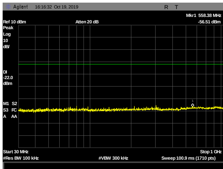
Figure 126: Conducted Spurious Emissions, Pigtail, 2442 MHz, 1 Mbps, 30 MHz - 1000 MHz
