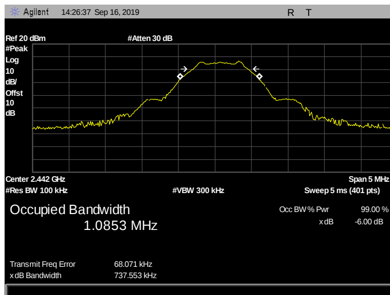
Figure 27: 6 dB Bandwidth, Terminal, 2442 MHz, 1 Mbps, 737.553 kHz
