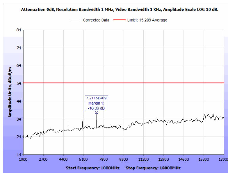
Figure 53: Radiated Spurious Emissions, Pigtail, 2402 MHz, 1 GHz - 18 GHz, Average, Horizontal
