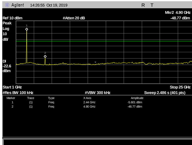
Figure 143: Conducted Spurious Emissions, Terminal, 2442 MHz, 1 Mbps, 1 GHz - 25 GHz
