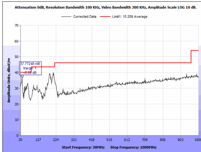
Figure 68: Radiated Spurious Emissions, Pigtail, 2480 MHz, 30 MHz - 1000 MHz, Vertical
