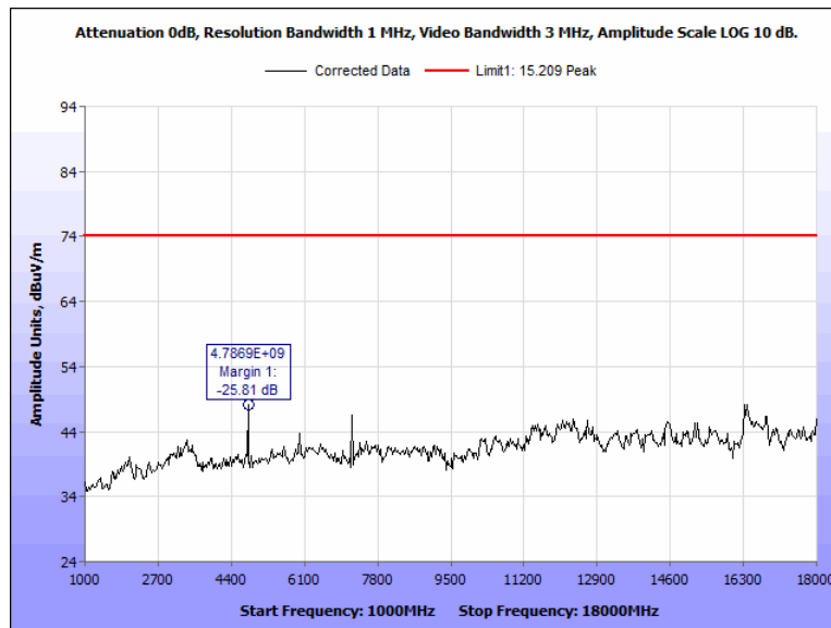
Figure 56: Radiated Spurious Emissions, Pigtail, 2402 MHz, 1 GHz - 18 GHz, Peak, Vertical
