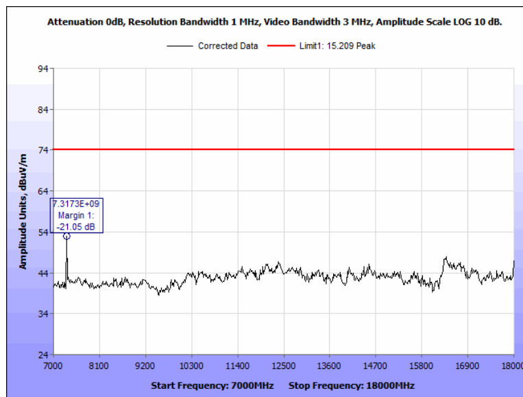
Figure 103: Radiated Spurious Emissions, Terminal, 2442 MHz, 7 GHz - 18 GHz, Peak, Horizontal
