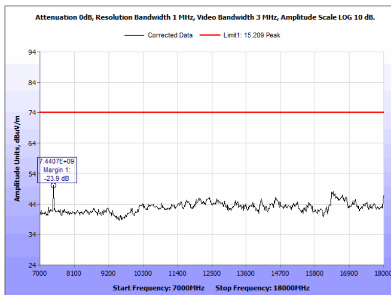
Figure 113: Radiated Spurious Emissions, Terminal, 2480 MHz, 7 GHz - 18 GHz, Peak, Horizontal
