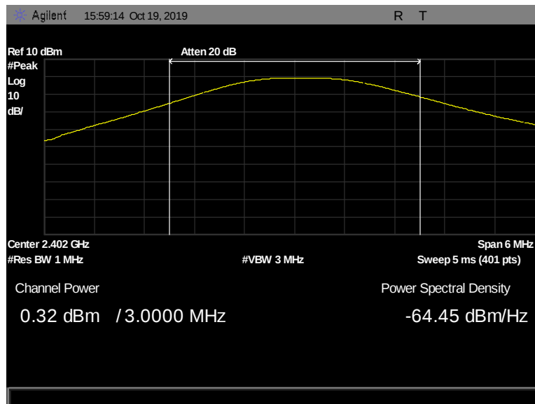
Figure 35: Peak Power Output, Pigtail, 2402 MHz, 1 Mbps, 0.32 dBm
