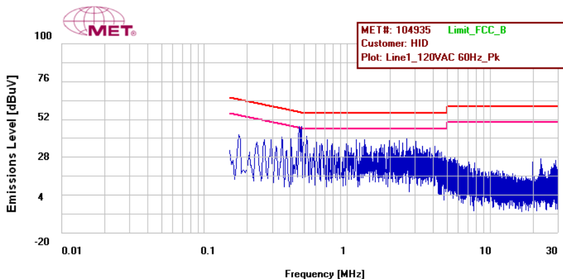
Figure 14: Conducted Emissions Limits, Terminal, Phase Line, Prescan
