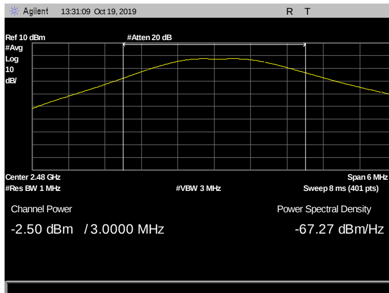
Figure 44: Peak Power Output, Terminal, 2480 MHz, 1 Mbps, -2.50 dBm
