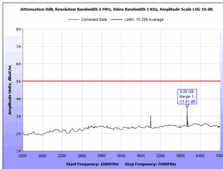
Figure 97: Radiated Spurious Emissions, Terminal, 2442 MHz, 1 GHz - 7 GHz, Average, Horizontal
