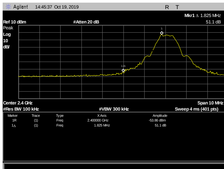
Figure 152: Conducted Band Edge, Terminal, 2402 MHz, 1 Mbps
