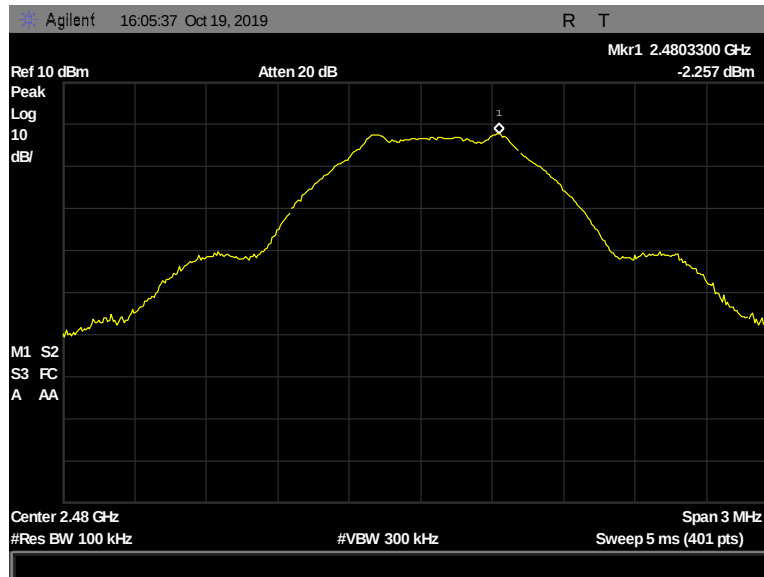
Figure 160: Peak Power Spectral Density, Pigtail, 2480 MHz, 1 Mbps, -2.257 dBm
