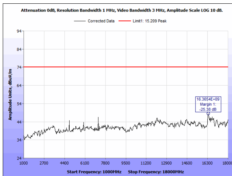
Figure 55: Radiated Spurious Emissions, Pigtail, 2402 MHz, 1 GHz - 18 GHz, Peak, Horizontal
