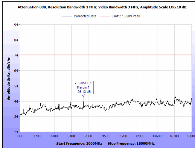
Figure 66: Radiated Spurious Emissions, Pigtail, 2442 MHz, 1 GHz - 18 GHz, Peak, Vertical
