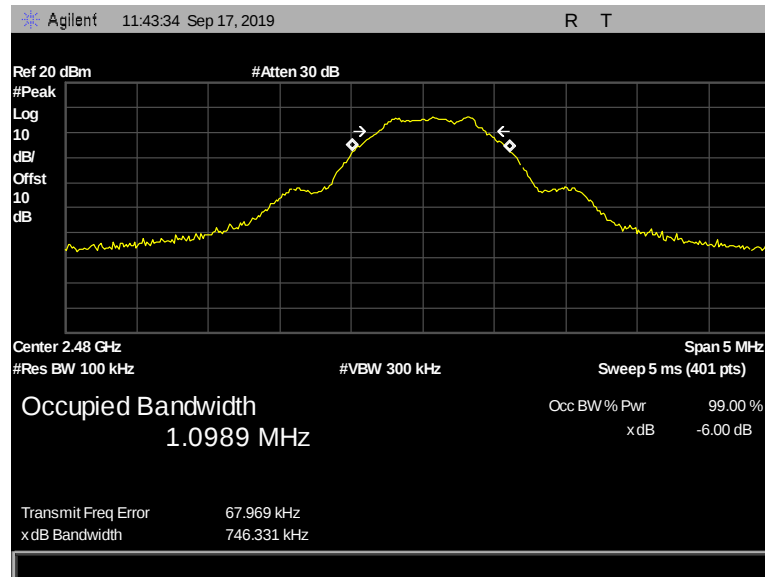
Figure 21: 6 dB Bandwidth, Pigtail, 2480 MHz, 1 Mbps, 746.331 kHz
