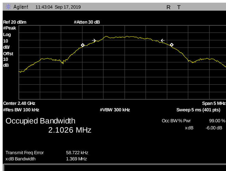
Figure 24: 6 dB Bandwidth, Pigtail, 2480 MHz, 2 Mbps, 1.369 MHz
