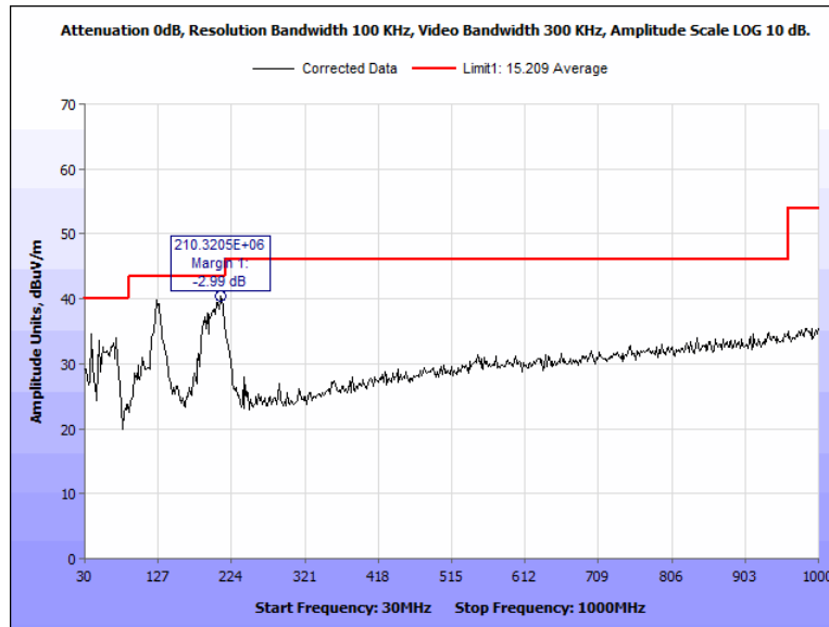
Figure 96: Radiated Spurious Emissions, Terminal, 2442 MHz, 30 MHz - 1000 MHz, Vertical
