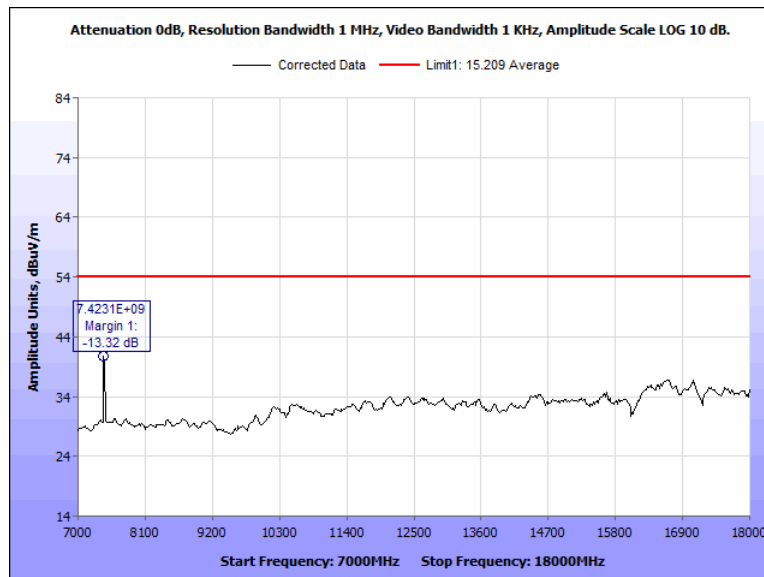
Figure 112: Radiated Spurious Emissions, Terminal, 2480 MHz, 7 GHz - 18 GHz, Average, Vertical
