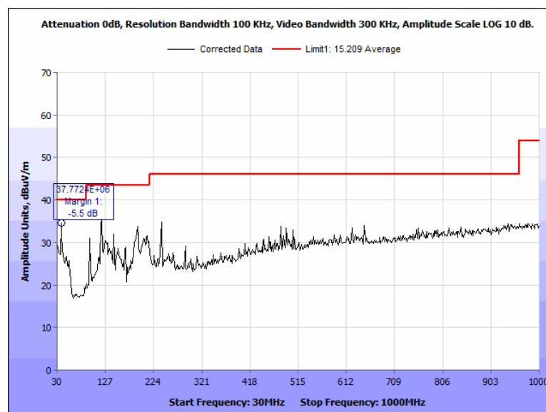
Figure 95: Radiated Spurious Emissions, Terminal, 2442 MHz, 30 MHz - 1000 MHz, Horizontal
