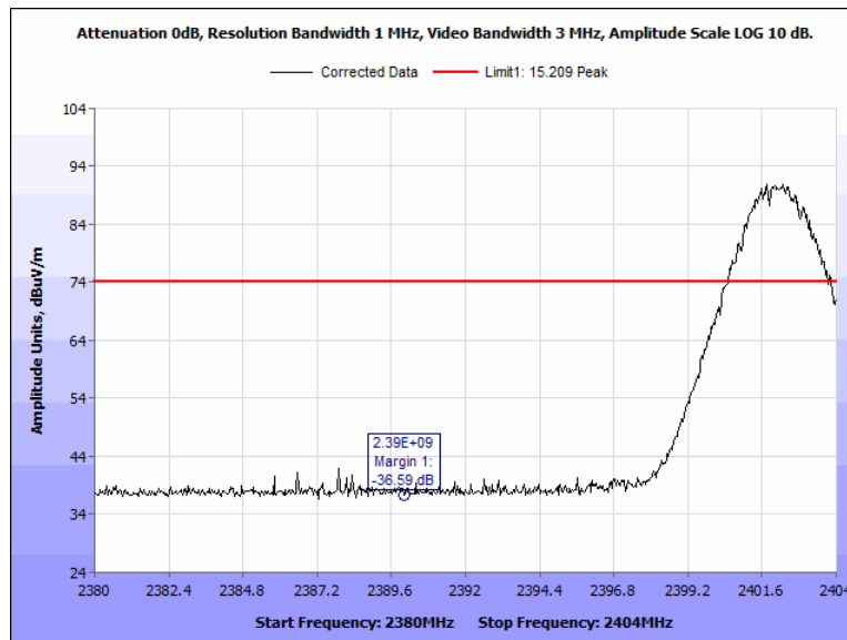
Figure 118: Radiated Band Edge, Terminal, 2402 MHz, Peak, Vertical
