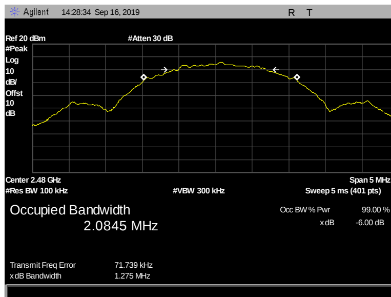
Figure 31: 6 dB Bandwidth, Terminal, 2480 MHz, 2 Mbps, 1.275 MHz
