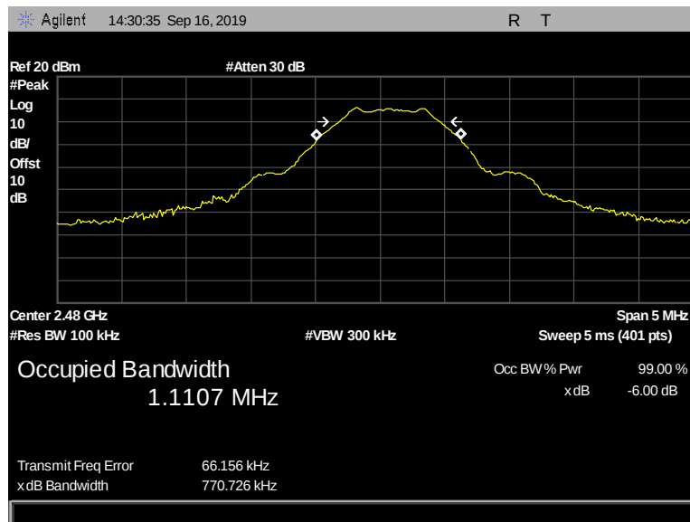
Figure 28: 6 dB Bandwidth, Terminal, 2480 MHz, 1 Mbps, 770.726 kHz
