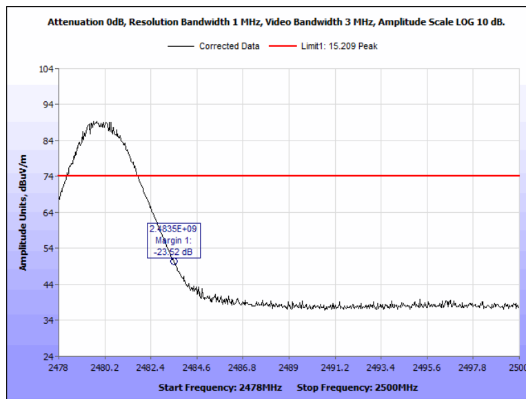
Figure 121: Radiated Band Edge, Terminal, 2480 MHz, Peak, Horizontal
