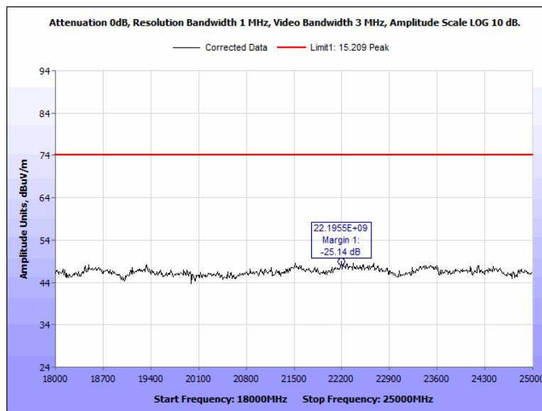
Figure 59: Radiated Spurious Emissions, Pigtail, 2402 MHz, 18 GHz - 25 GHz, Peak, Horizontal
