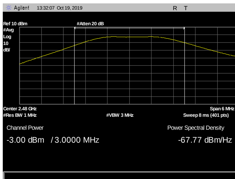
Figure 47: Peak Power Output, Terminal, 2480 MHz, 2 Mbps, -3.00 dBm
