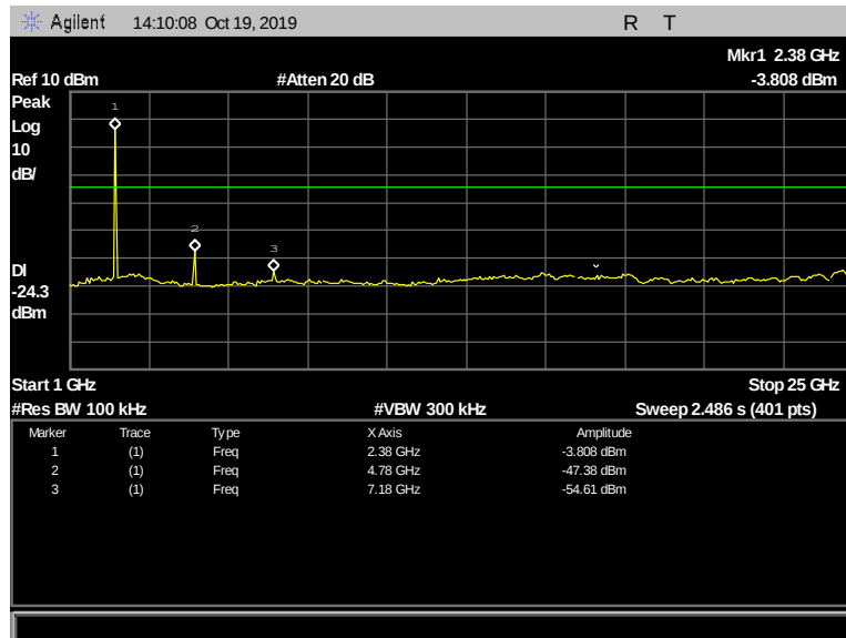
Figure 147: Conducted Spurious Emissions, Terminal, 2402 MHz, 2 Mbps, 1 GHz - 25 GHz
