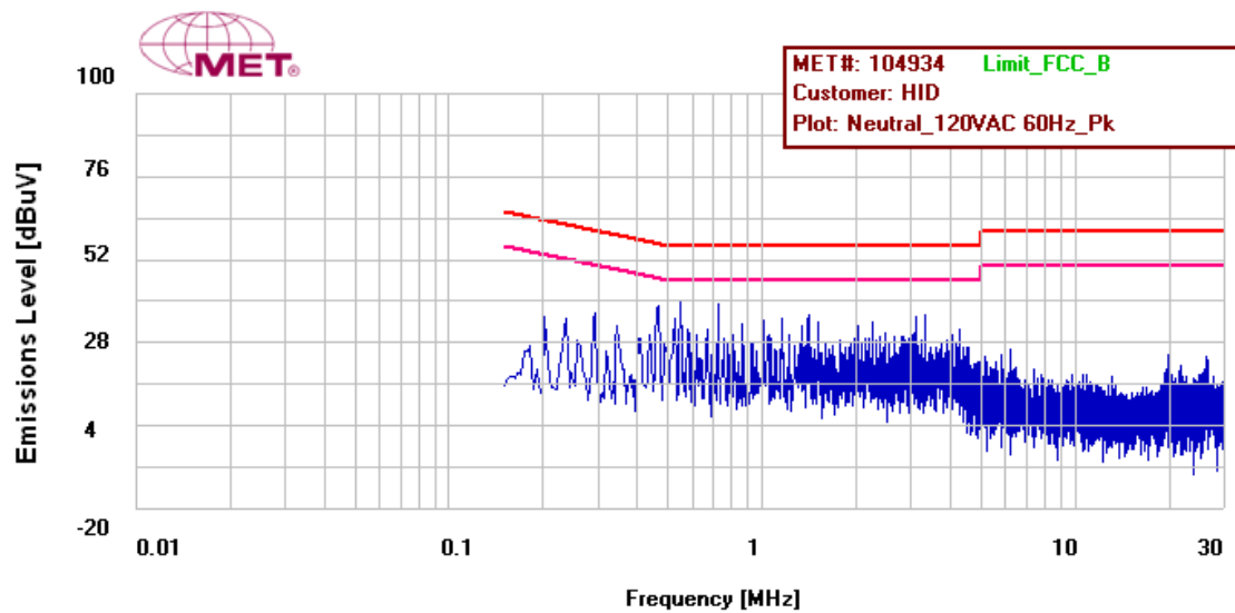
Figure 12: Conducted Emissions Limits, Pigtail, Neutral Line, Prescan
