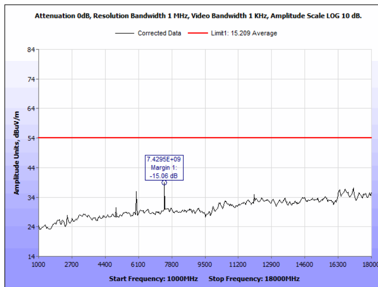
Figure 69: Radiated Spurious Emissions, Pigtail, 2480 MHz, 1 GHz - 18 GHz, Average, Horizontal
