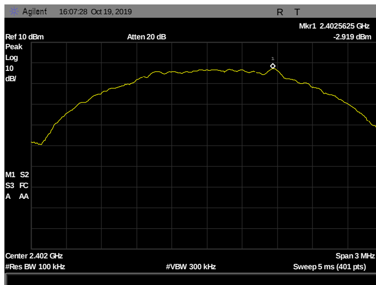
Figure 161: Peak Power Spectral Density, Pigtail, 2402 MHz, 2 Mbps, -2.919 dBm
