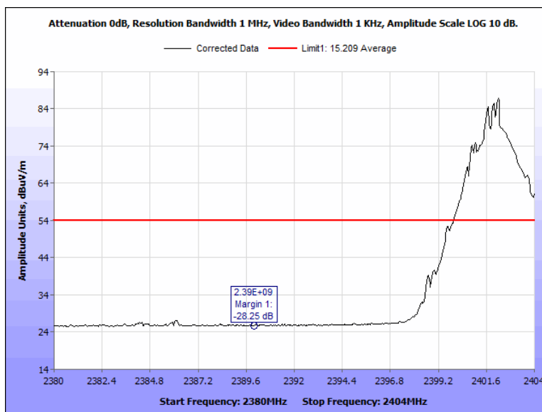
Figure 73: Radiated Band Edge, Pigtail, 2402 MHz, Average, Horizontal
