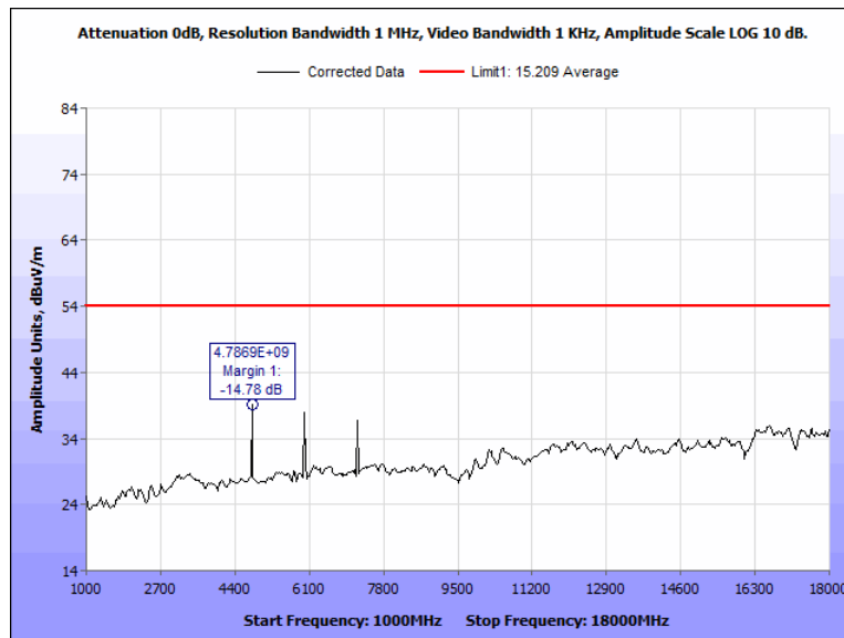
Figure 54: Radiated Spurious Emissions, Pigtail, 2402 MHz, 1 GHz - 18 GHz, Average, Vertical
