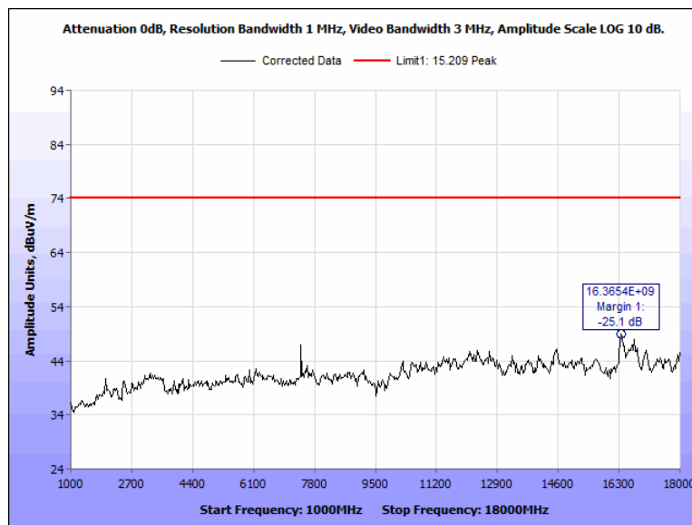
Figure 71: Radiated Spurious Emissions, Pigtail, 2480 MHz, 1 GHz - 18 GHz, Peak, Horizontal
