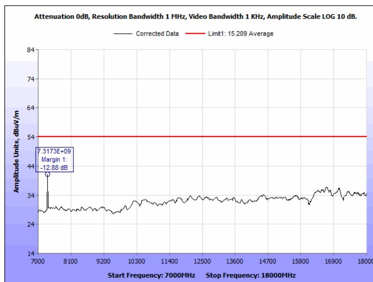
Figure 101: Radiated Spurious Emissions, Terminal, 2442 MHz, 7 GHz - 18 GHz, Average, Horizontal
