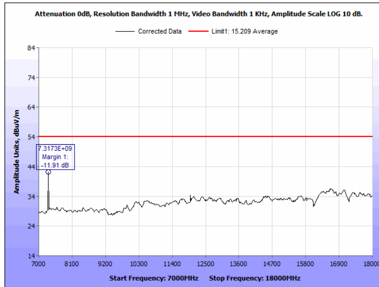
Figure 102: Radiated Spurious Emissions, Terminal, 2442 MHz, 7 GHz - 18 GHz, Average, Vertical
