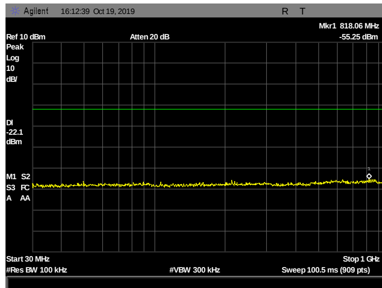
Figure 124: Conducted Spurious Emissions, Pigtail, 2402 MHz, 1 Mbps, 30 MHz - 1000 MHz
