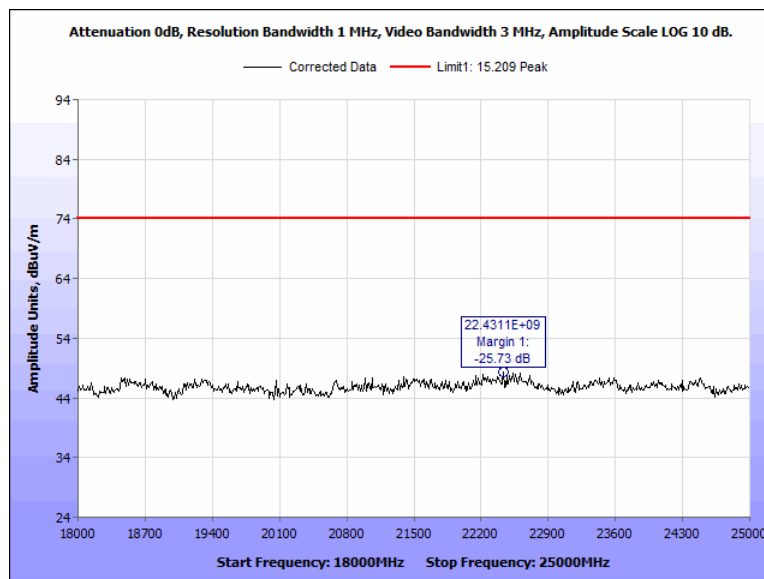
Figure 93: Radiated Spurious Emissions, Terminal, 2402 MHz, 18 GHz - 25 GHz, Peak, Horizontal
