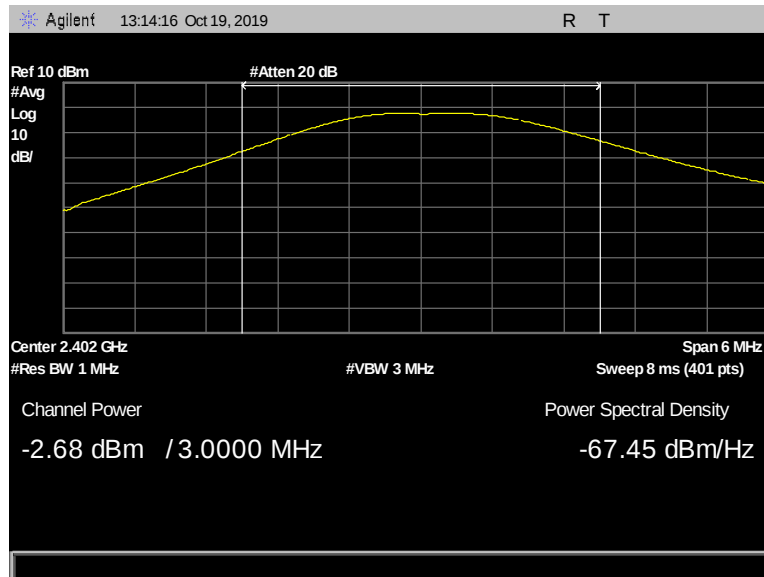
Figure 42: Peak Power Output, Terminal, 2402 MHz, 1 Mbps, -2.68 dBm
