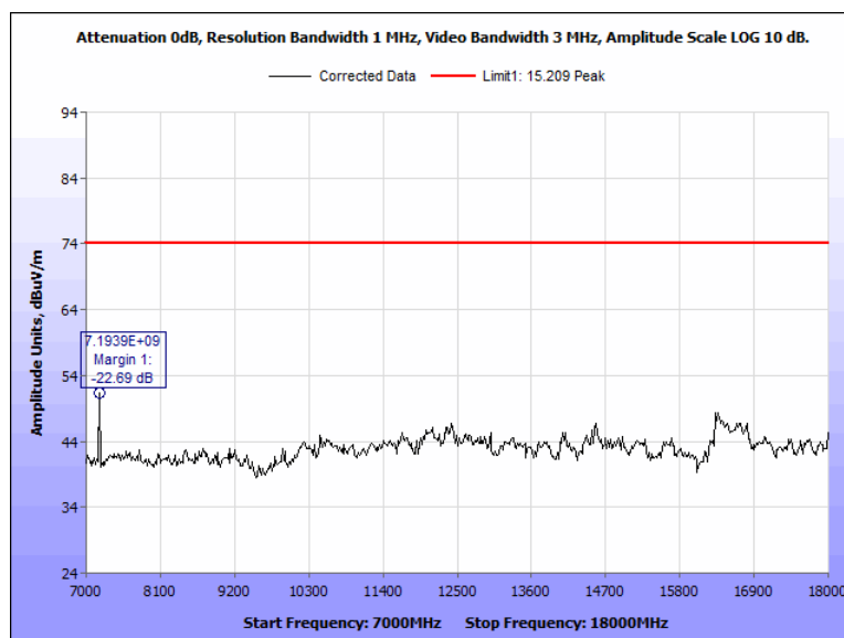
Figure 89: Radiated Spurious Emissions, Terminal, 2402 MHz, 7 GHz - 18 GHz, Peak, Horizontal
