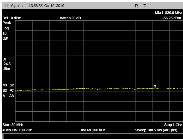
Figure 146: Conducted Spurious Emissions, Terminal, 2402 MHz, 2 Mbps, 30 MHz - 1000 MHz
