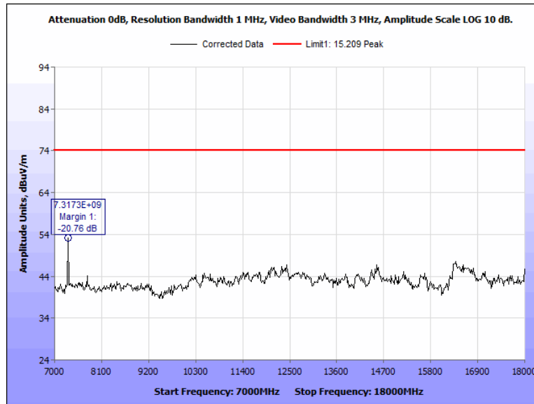
Figure 104: Radiated Spurious Emissions, Terminal, 2442 MHz, 7 GHz - 18 GHz, Peak, Vertical
