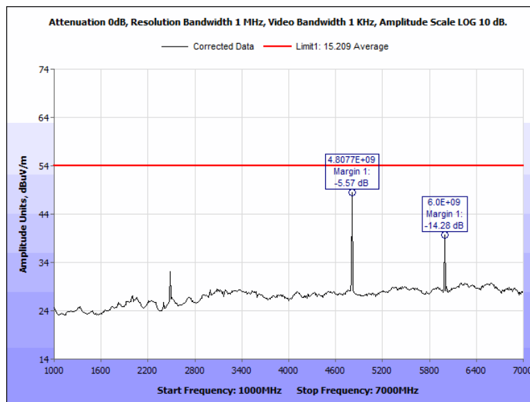
Figure 83: Radiated Spurious Emissions, Terminal, 2402 MHz, 1 GHz - 7 GHz, Average, Horizontal
