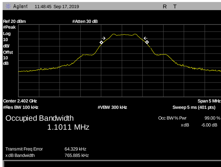
Figure 19: 6 dB Bandwidth, Pigtail, 2402 MHz, 1 Mbps, 765.885 kHz
