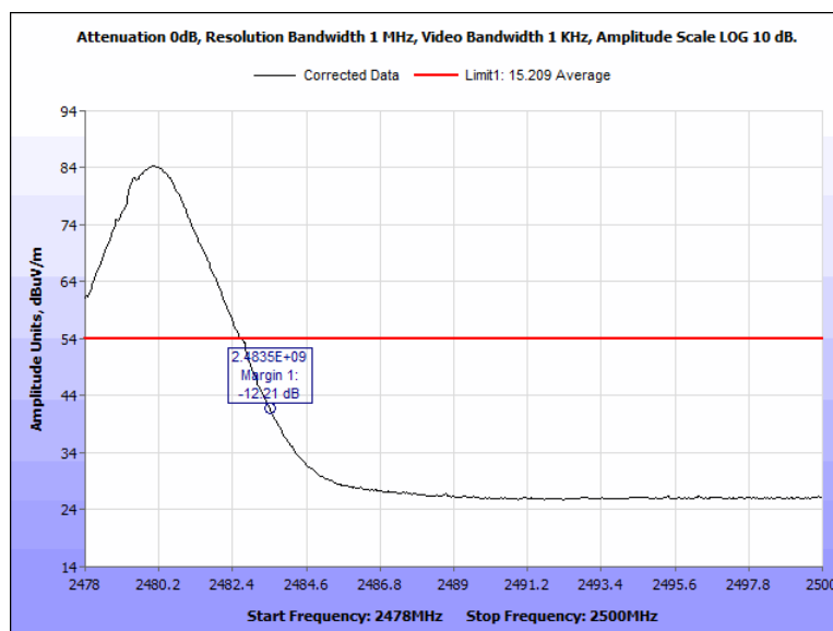
Figure 119: Radiated Band Edge, Terminal, 2480 MHz, Average, Horizontal
