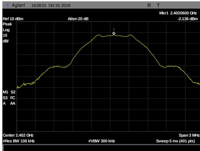
Figure 158: Peak Power Spectral Density, Pigtail, 2402 MHz, 1 Mbps, -2.136 dBm
