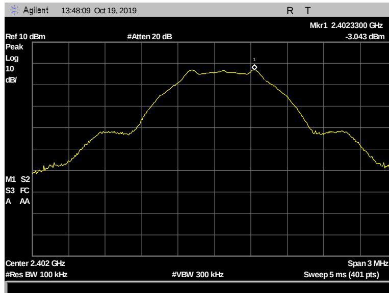
Figure 165: Peak Power Spectral Density, Terminal, 2402 MHz, 1 Mbps, -3.043 dBm
