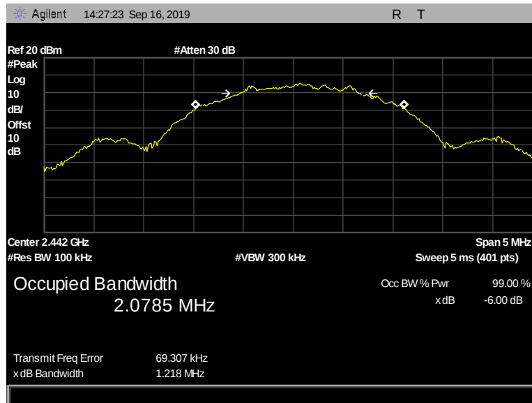
Figure 30: 6 dB Bandwidth, Terminal, 2442 MHz, 2 Mbps, 1.218 MHz
