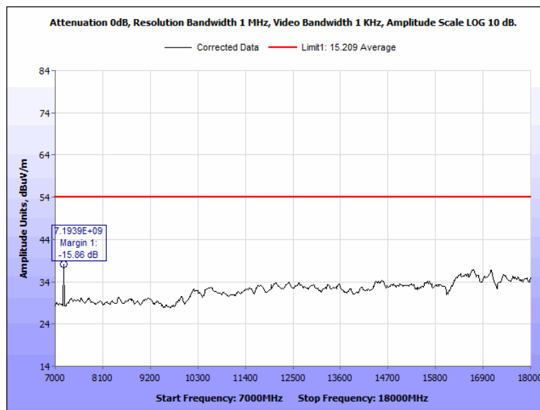
Figure 87: Radiated Spurious Emissions, Terminal, 2402 MHz, 7 GHz - 18 GHz, Average, Horizontal
