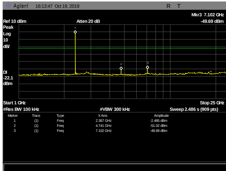
Figure 125: Conducted Spurious Emissions, Pigtail, 2402 MHz, 1 Mbps, 1 GHz - 25 GHz
