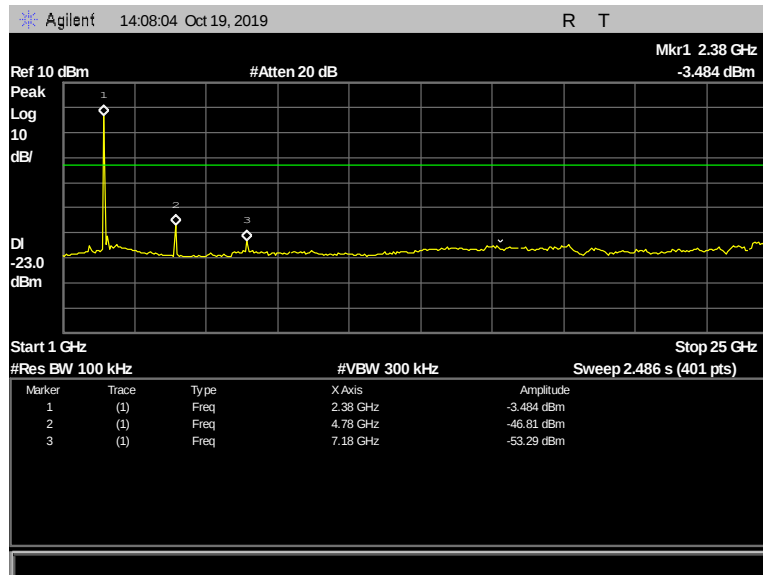
Figure 141: Conducted Spurious Emissions, Terminal, 2402 MHz, 1 Mbps, 1 GHz - 25 GHz
