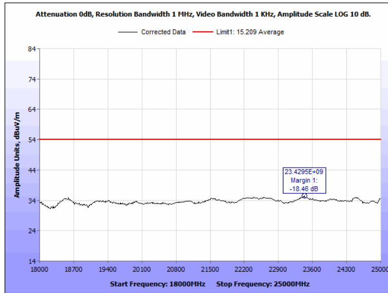
Figure 92: Radiated Spurious Emissions, Terminal, 2402 MHz, 18 GHz - 25 GHz, Average, Vertical
