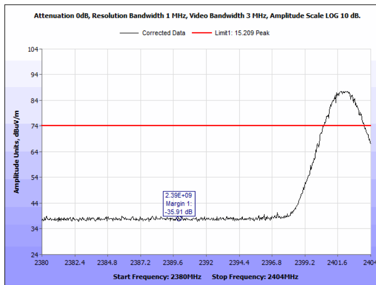
Figure 117: Radiated Band Edge, Terminal, 2402 MHz, Peak, Horizontal
