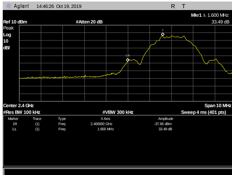
Figure 153: Conducted Band Edge, Terminal, 2402 MHz, 2 Mbps
