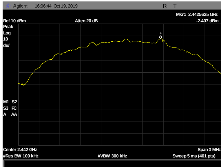
Figure 162: Peak Power Spectral Density, Pigtail, 2442 MHz, 2 Mbps, -2.407 dBm
