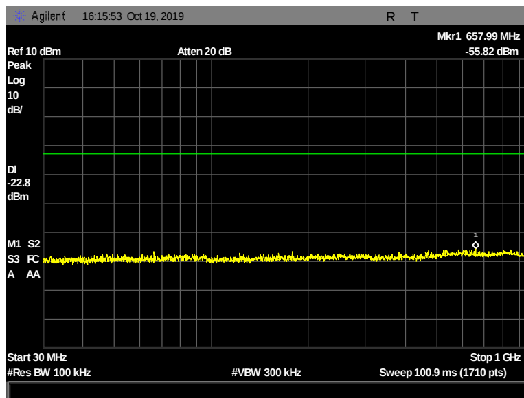
Figure 130: Conducted Spurious Emissions, Pigtail, 2402 MHz, 2 Mbps, 30 MHz - 1000 MHz
