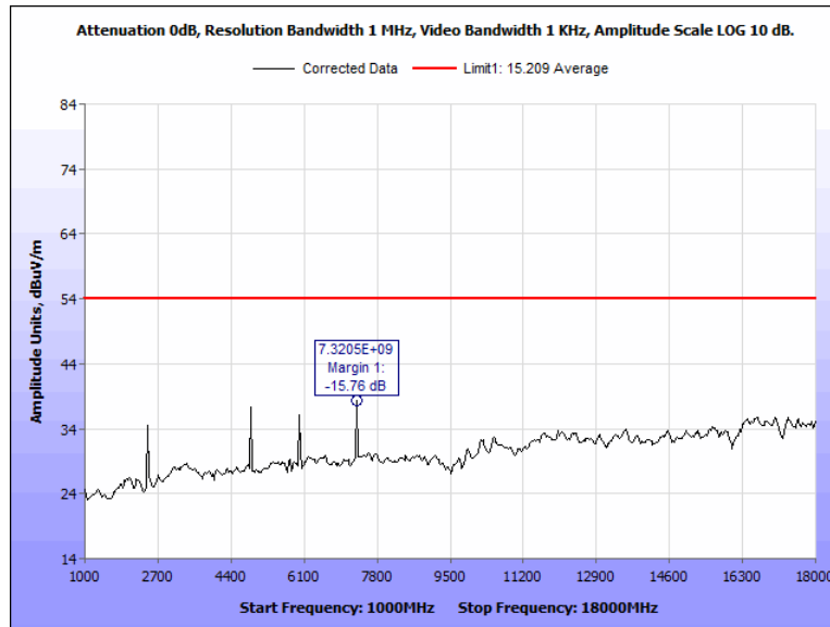
Figure 64: Radiated Spurious Emissions, Pigtail, 2442 MHz, 1 GHz - 18 GHz, Average, Vertical
