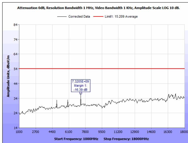
Figure 63: Radiated Spurious Emissions, Pigtail, 2442 MHz, 1 GHz - 18 GHz, Average, Horizontal
