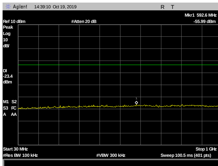
Figure 144: Conducted Spurious Emissions, Terminal, 2480 MHz, 1 Mbps, 30 MHz - 1000 MHz
