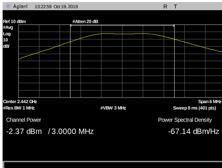
Figure 46: Peak Power Output, Terminal, 2442 MHz, 2 Mbps, -2.37 dBm
