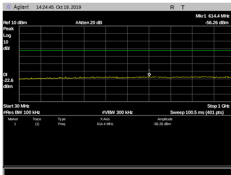
Figure 142: Conducted Spurious Emissions, Terminal, 2442 MHz, 1 Mbps, 30 MHz - 1000 MHz
