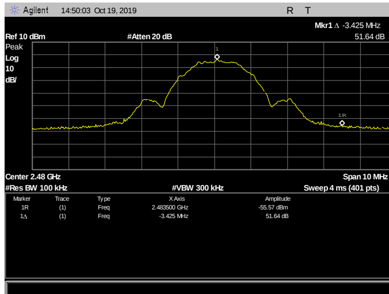
Figure 155: Conducted Band Edge, Terminal, 2480 MHz, 2 Mbps
