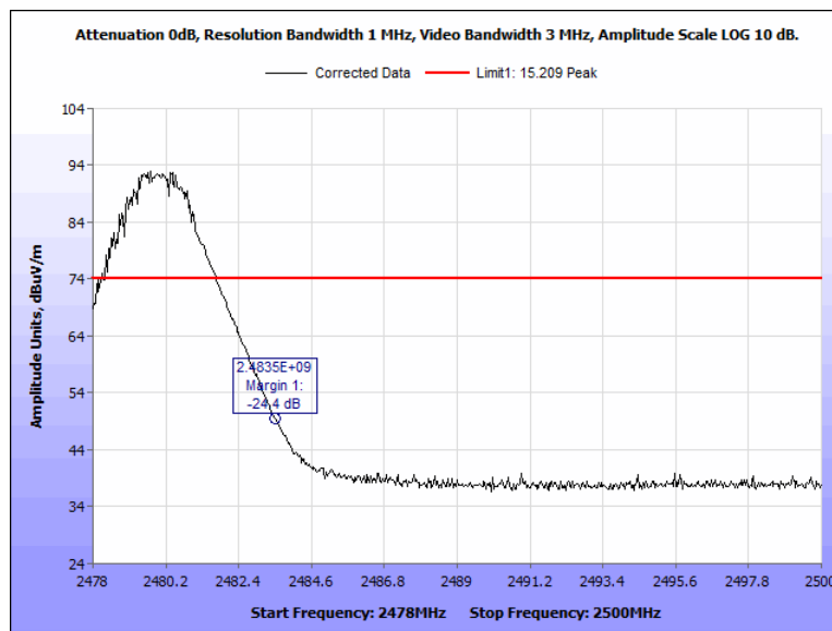
Figure 79: Radiated Band Edge, Pigtail, 2480 MHz, Peak, Horizontal
