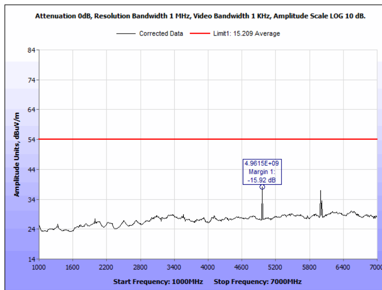
Figure 107: Radiated Spurious Emissions, Terminal, 2480 MHz, 1 GHz - 7 GHz, Average, Vertical
