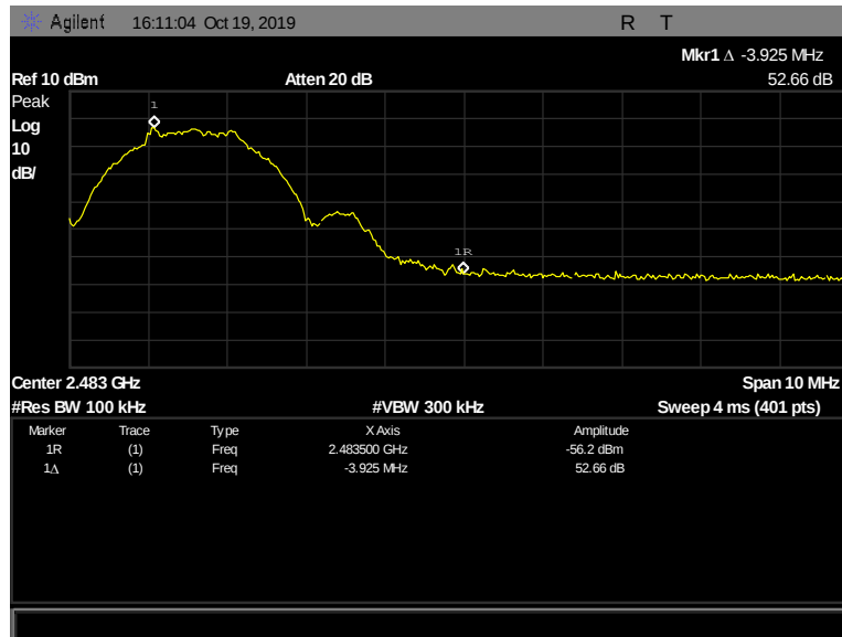
Figure 139: Conducted Band Edge, Pigtail, 2480 MHz, 2 Mbps
