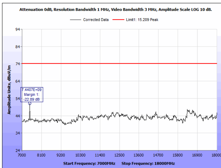
Figure 114: Radiated Spurious Emissions, Terminal, 2480 MHz, 7 GHz - 18 GHz, Peak, Vertical
