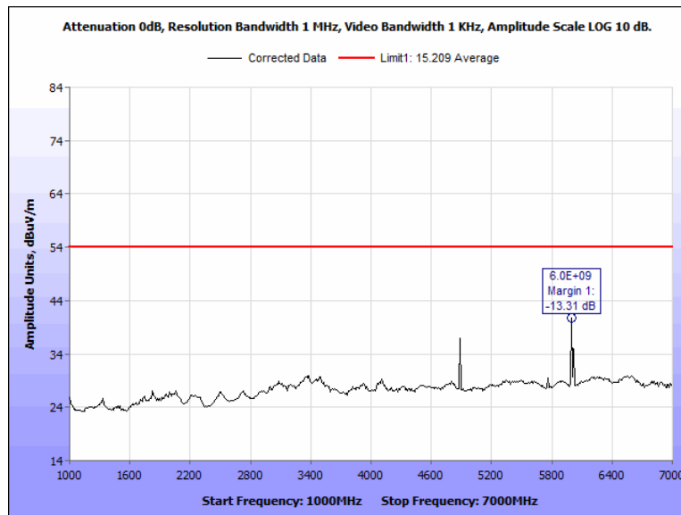
Figure 98: Radiated Spurious Emissions, Terminal, 2442 MHz, 1 GHz - 7 GHz, Average, Vertical
