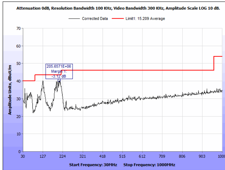
Figure 106: Radiated Spurious Emissions, Terminal, 2480 MHz, 30 MHz - 1000 MHz, Vertical
