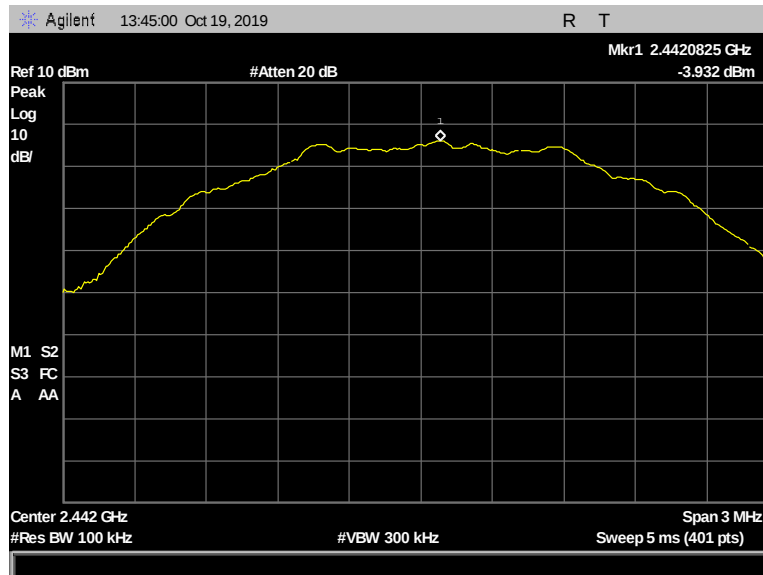
Figure 169: Peak Power Spectral Density, Terminal, 2442 MHz, 2 Mbps, -3.932 dBm
