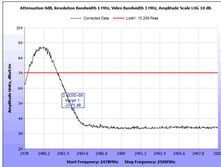
Figure 122: Radiated Band Edge, Terminal, 2480 MHz, Peak, Vertical
