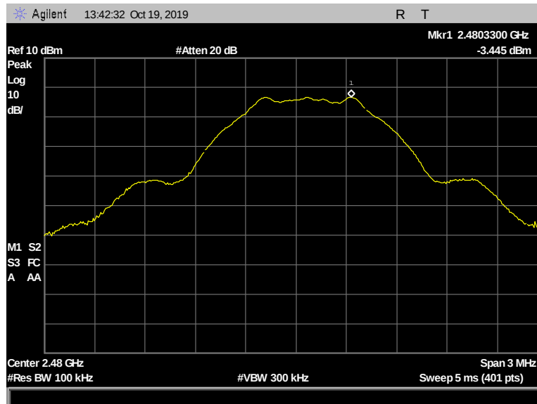
Figure 167: Peak Power Spectral Density, Terminal, 2480 MHz, 1 Mbps, -3.445 dBm
