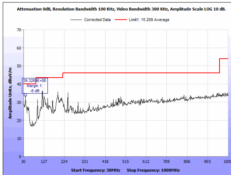
Figure 81: Radiated Spurious Emissions, Terminal, 2402 MHz, 30 MHz - 1000 MHz, Horizontal
