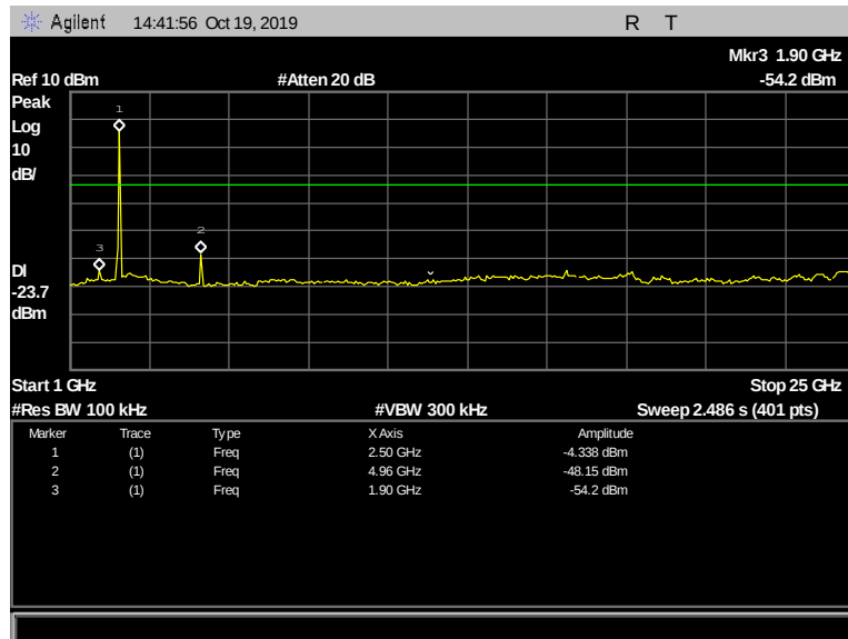
Figure 151: Conducted Spurious Emissions, Terminal, 2480 MHz, 2 Mbps, 1 GHz - 25 GHz
