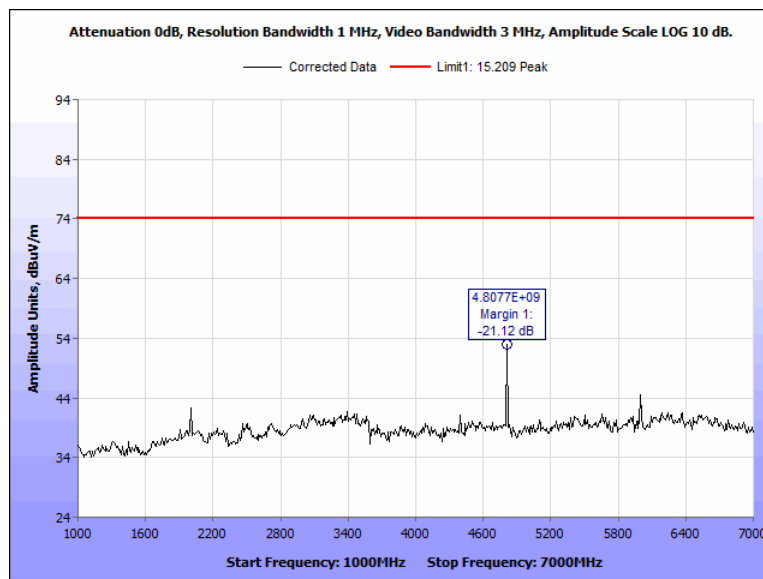
Figure 85: Radiated Spurious Emissions, Terminal, 2402 MHz, 1 GHz - 7 GHz, Peak, Horizontal
