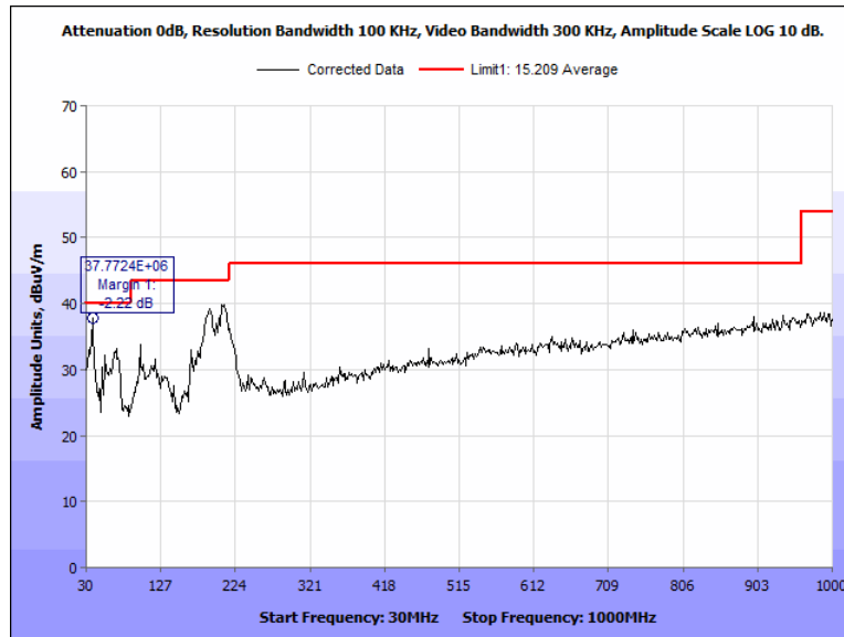
Figure 62: Radiated Spurious Emissions, Pigtail, 2442 MHz, 30 MHz - 1000 MHz, Vertical
