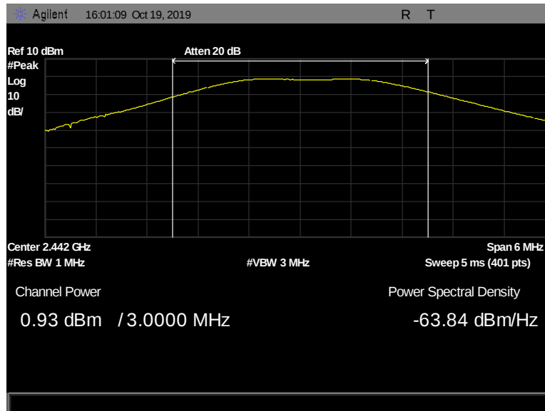
Figure 39: Peak Power Output, Pigtail, 2442 MHz, 2 Mbps, 0.93 dBm
