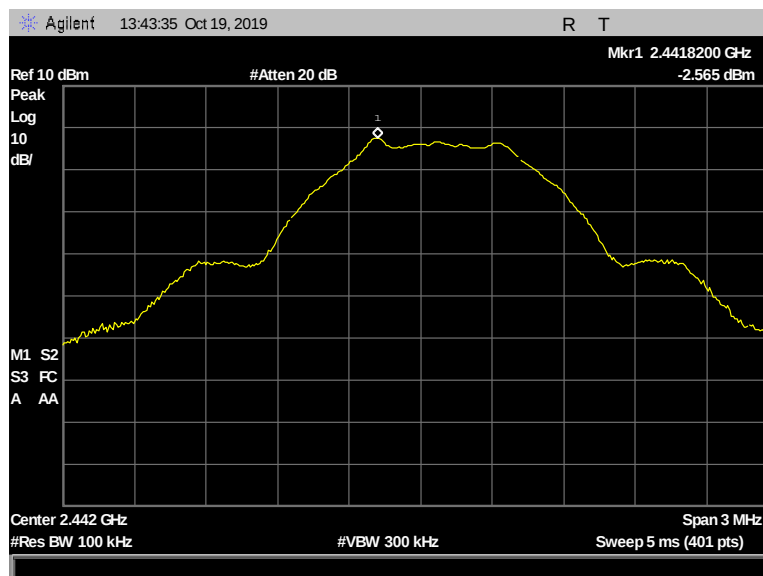
Figure 166: Peak Power Spectral Density, Terminal, 2442 MHz, 1 Mbps, -2.565 dBm
