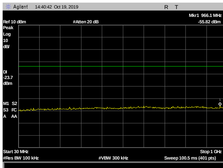
Figure 150: Conducted Spurious Emissions, Terminal, 2480 MHz, 2 Mbps, 30 MHz - 1000 MHz
