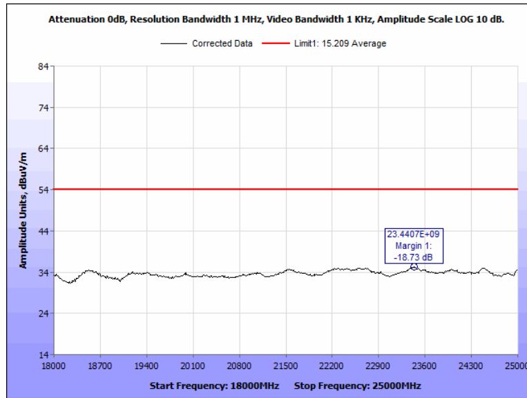
Figure 58: Radiated Spurious Emissions, Pigtail, 2402 MHz, 18 GHz - 25 GHz, Average, Horizontal
