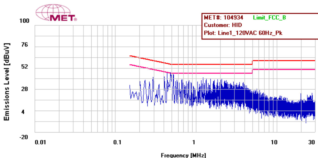
Figure 10: Conducted Emissions Limits, Pigtail, Phase Line, Prescan
