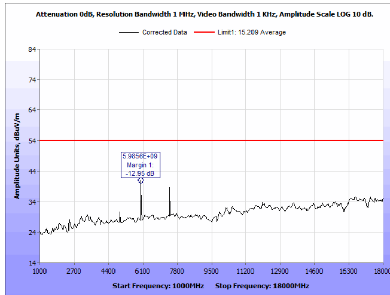
Figure 70: Radiated Spurious Emissions, Pigtail, 2480 MHz, 1 GHz - 18 GHz, Average, Vertical
