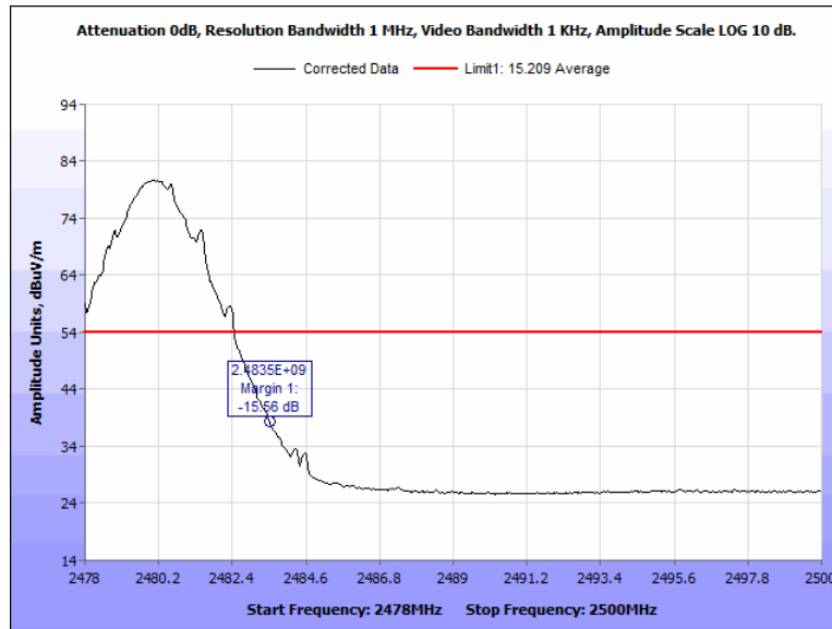
Figure 78: Radiated Band Edge, Pigtail, 2480 MHz, Average, Vertical
