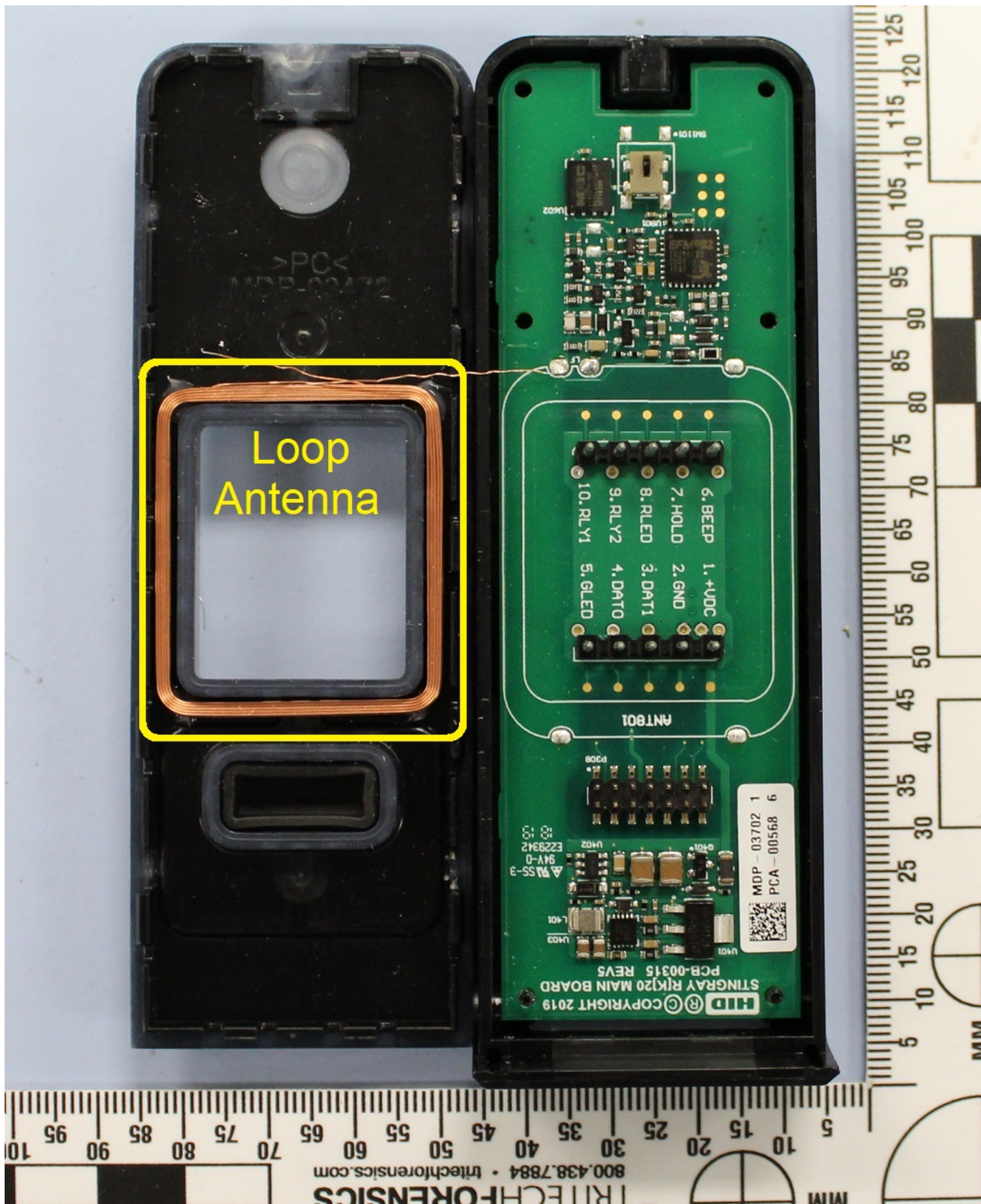
Model 20 and model 20K (terminal version shown) LF loop antenna – 125kHz
