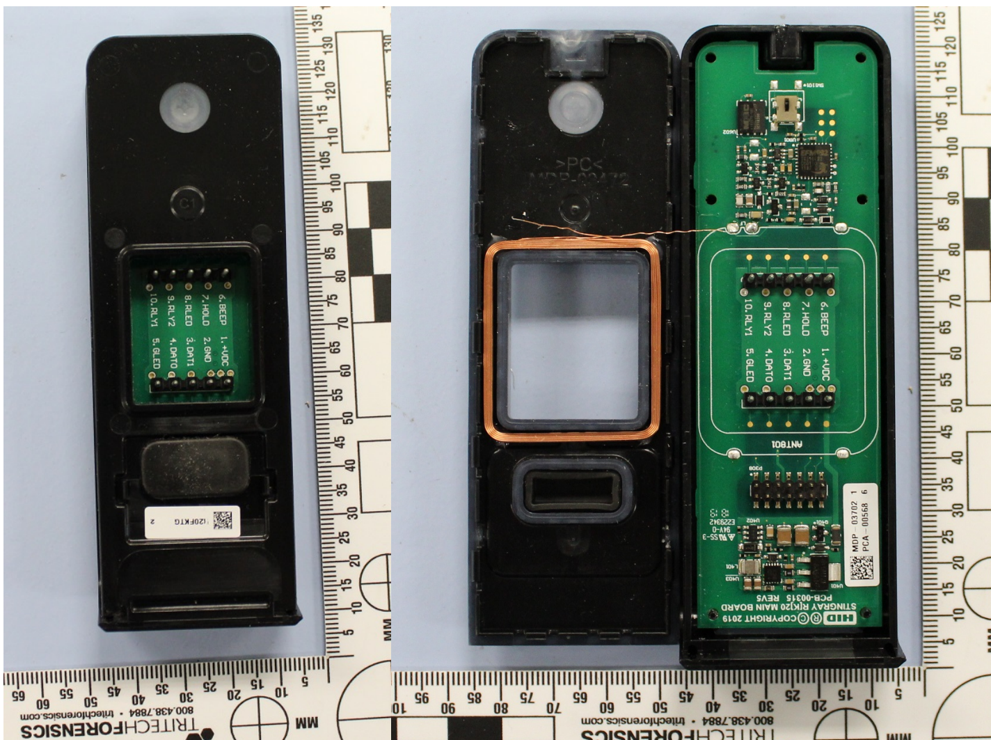
Model 20K (terminal version) no cover
