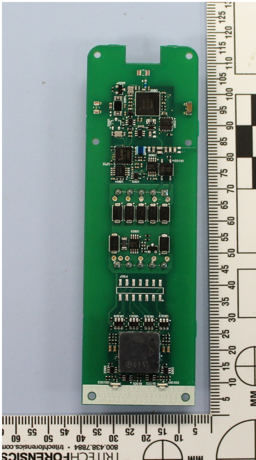
Model 20K (terminal version) main board obverse without patch antenna
