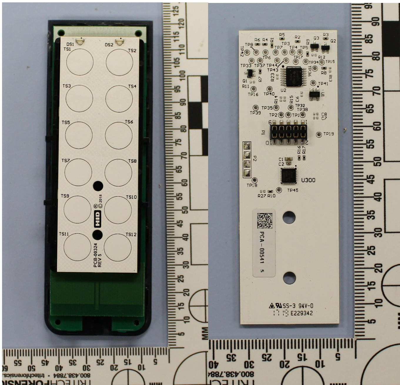
Model 20K (terminal version) keypad obverse
