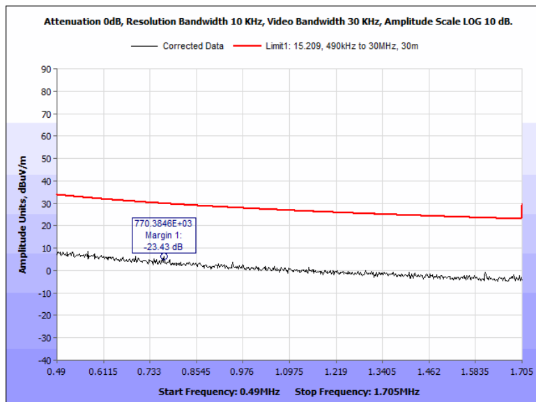
Figure 22: Radiated Spurious Emissions, Terminal, 0.490 MHz – 1.705 MHz, 90 Deg
