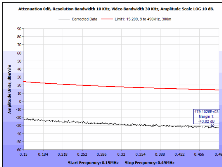
Figure 14: Radiated Spurious Emissions, Pigtail, 0.15 MHz – 0.490 MHz, 90 Deg
