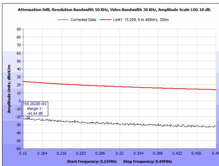
Figure 19: Radiated Spurious Emissions, Terminal, 0.150 MHz – 0.490 MHz, 0 Deg
