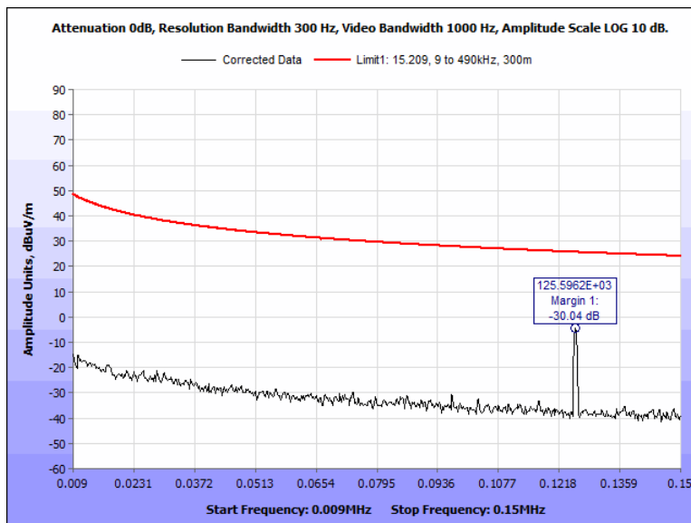
Figure 18: Radiated Spurious Emissions, Terminal, 0.009 MHz – 0.150 MHz, 90 Deg
