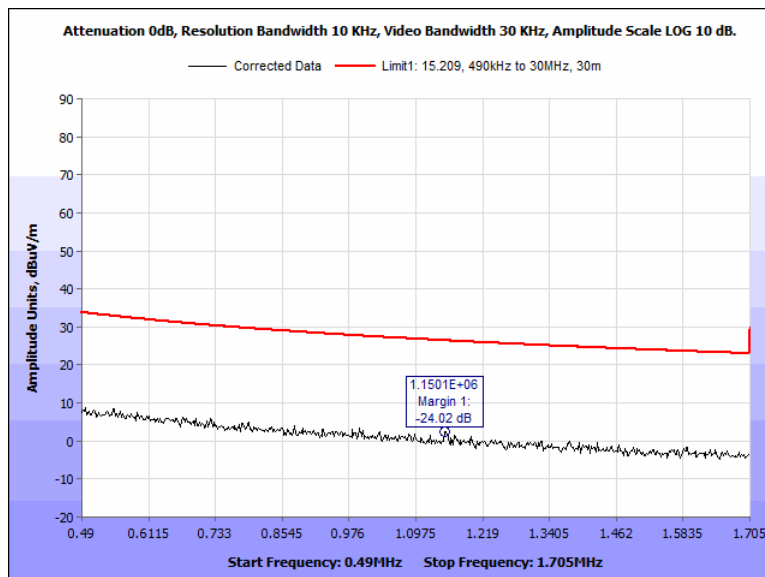
Figure 16: Radiated Spurious Emissions, Pigtail, 0.490 MHz – 1.705 MHz, 90 Deg
