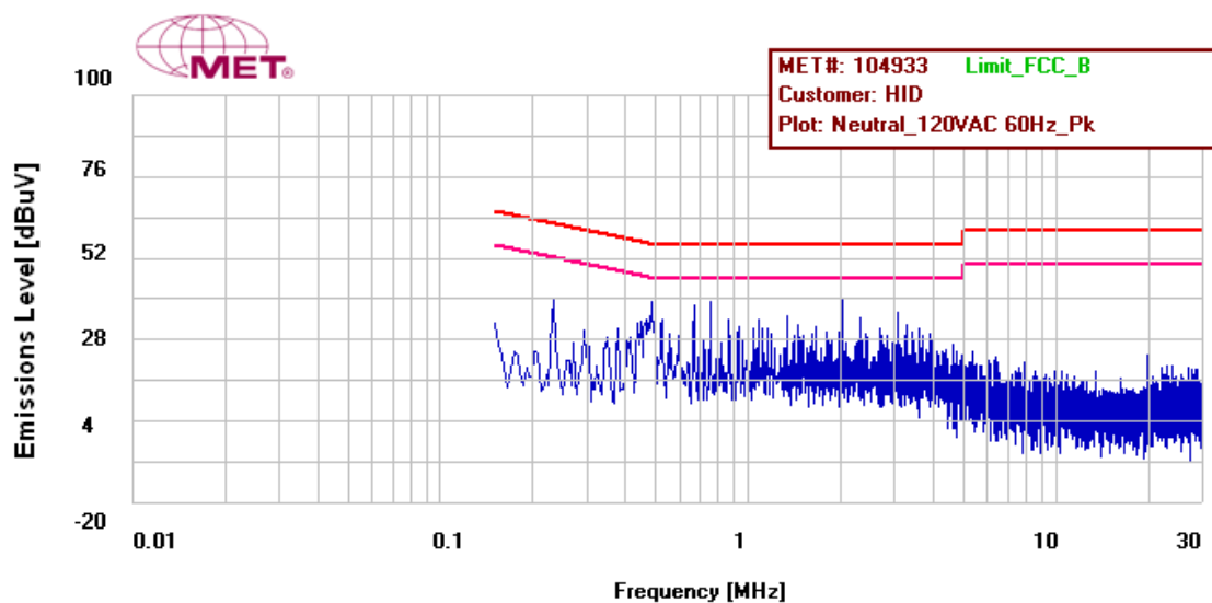
Figure 32: Conducted Emissions Limits, Terminal, Neutral Line, Prescan
