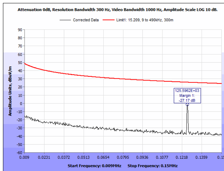
Figure 11: Radiated Spurious Emissions, Pigtail, 0.009 MHz – 0.150 MHz, 0 Deg
