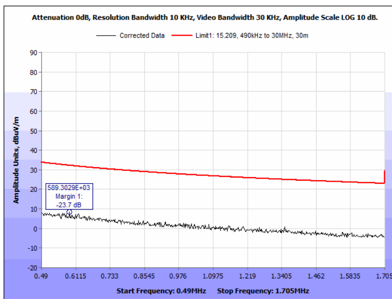
Figure 21: Radiated Spurious Emissions, Terminal, 0.490 MHz – 1.705 MHz, 0 Deg
