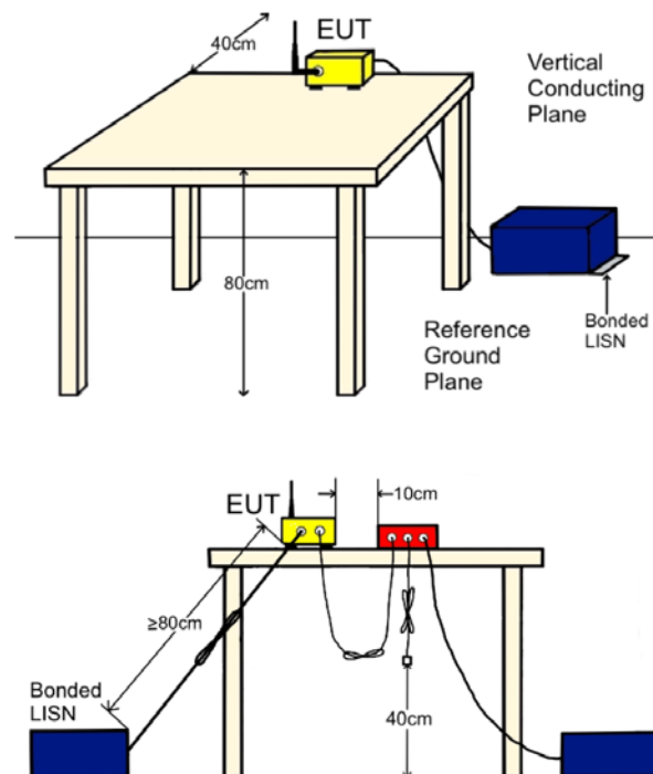
Figure 24: CEV Test Setup
