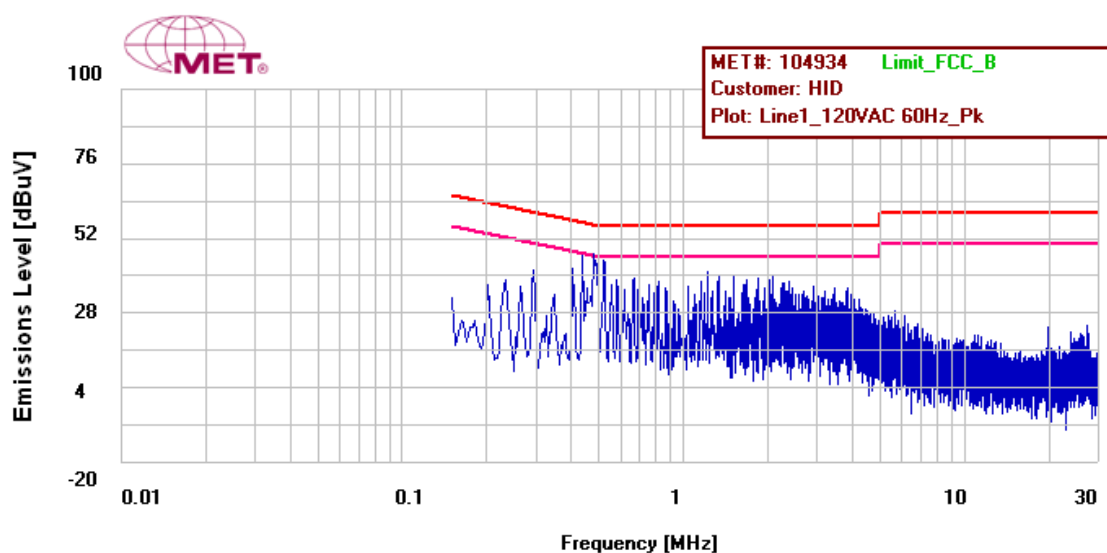
Figure 26: Conducted Emissions Limits, Pigtail, Phase Line, Prescan
