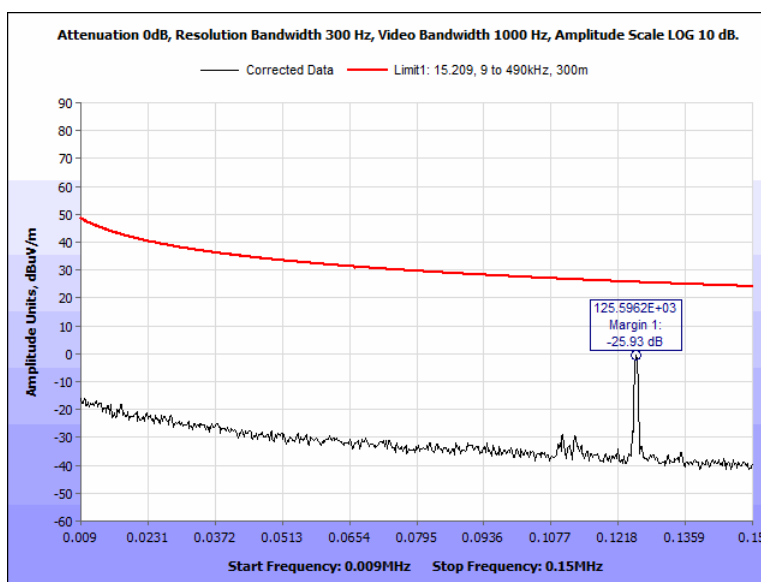
Figure 17: Radiated Spurious Emissions, Terminal, 0.009 MHz – 0.150 MHz, 0 Deg
