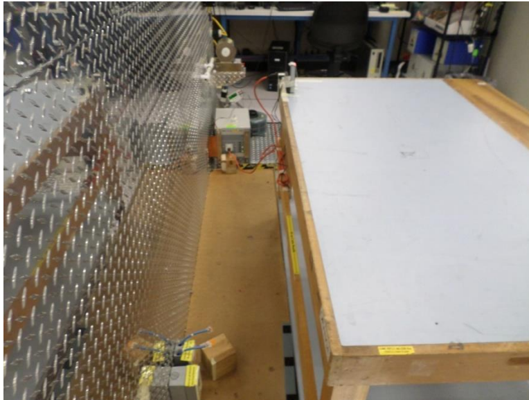
Figure 7: Conducted Emissions Limits, Terminal, Test Setup, Back View
