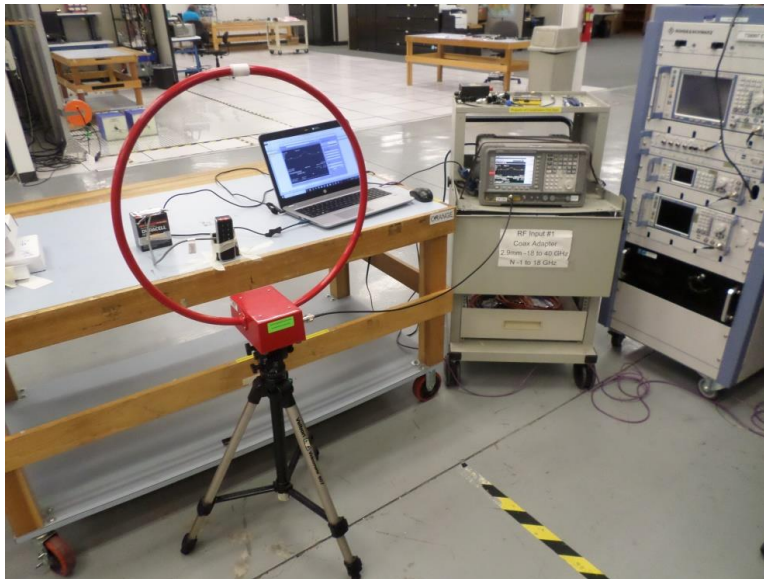
Figure 8: 20 dB Occupied Bandwidth, Pigtail, Test Setup
