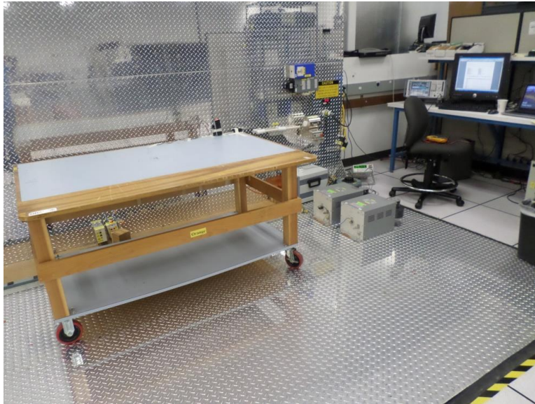
Figure 3: Conducted Emissions Limits, Pigtail, Setup Front View
