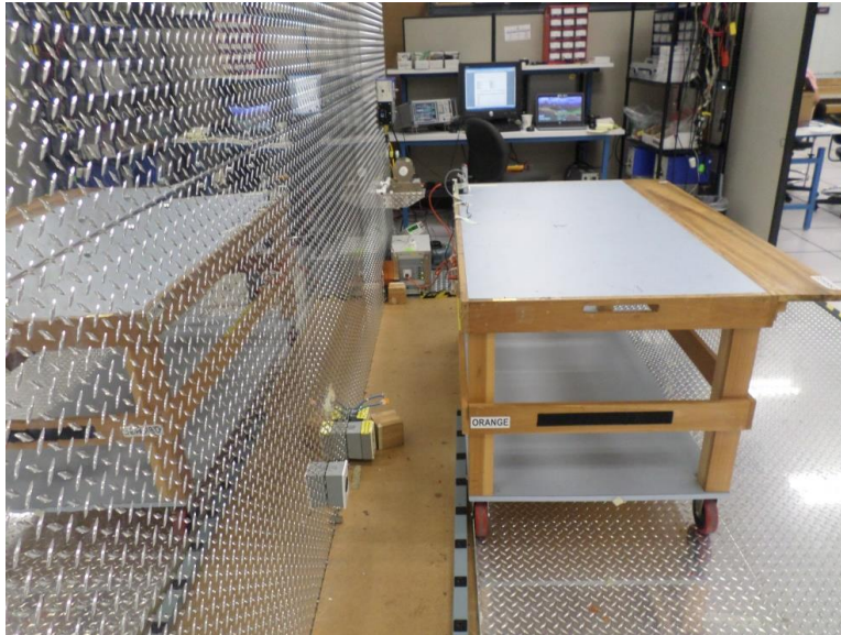
Figure 1: Conducted Emissions Limits, Pigtail, Setup Back View
