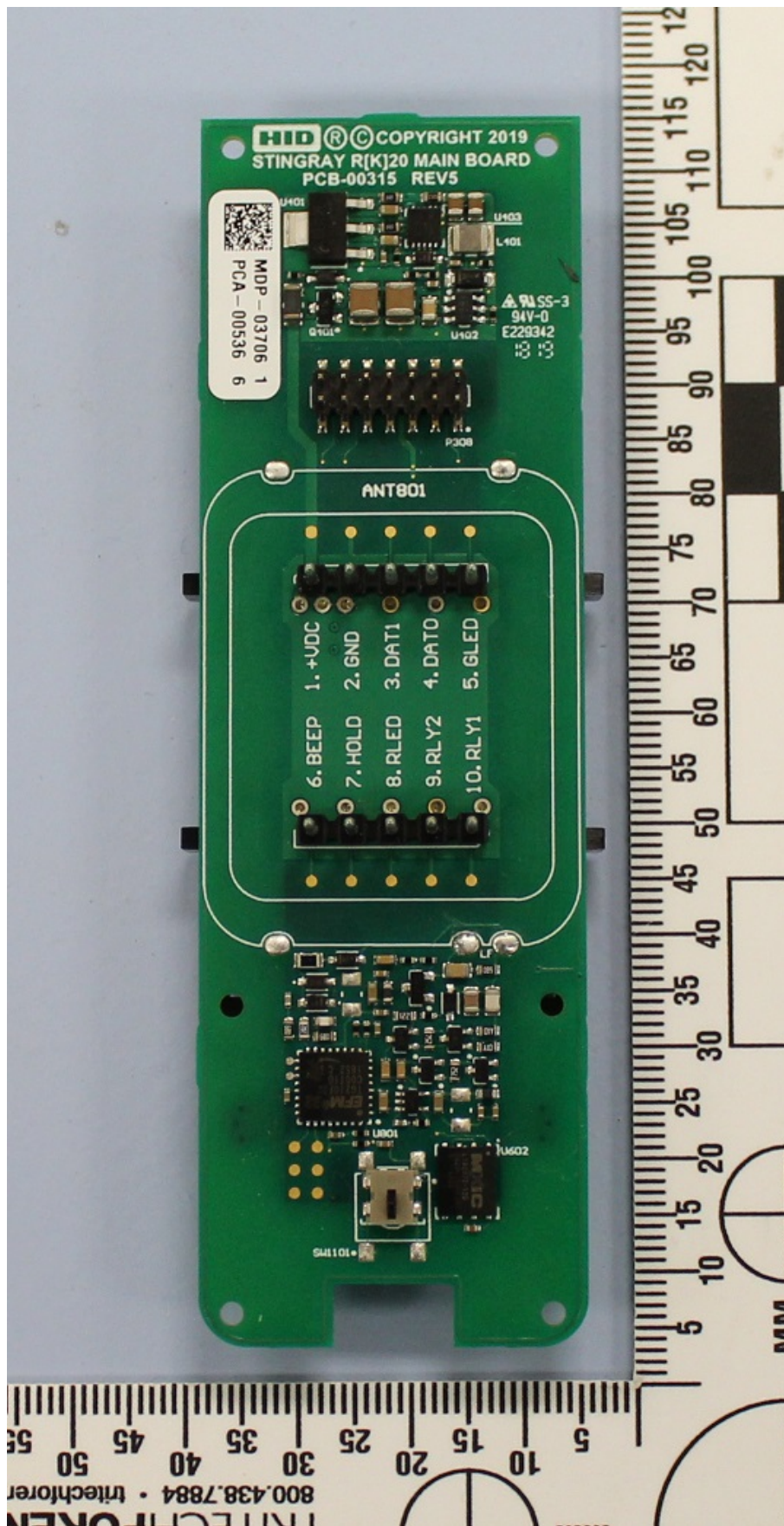
Model 20K (terminal version) main board reverse
