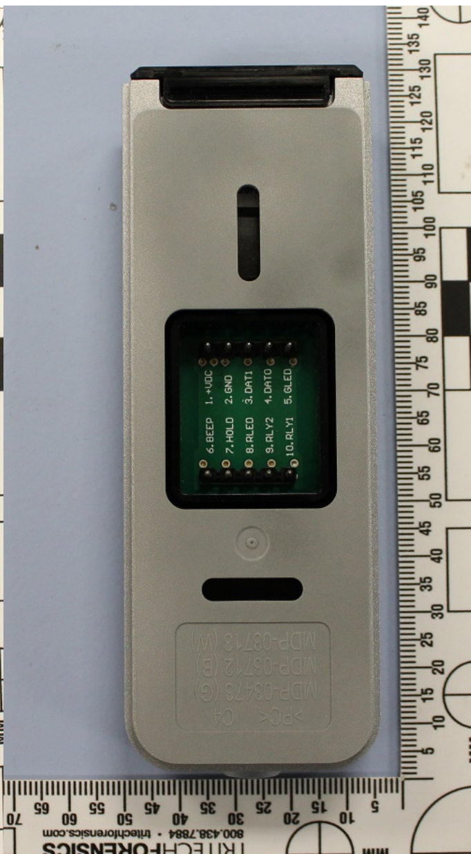
Model 20K (terminal version) rear side
