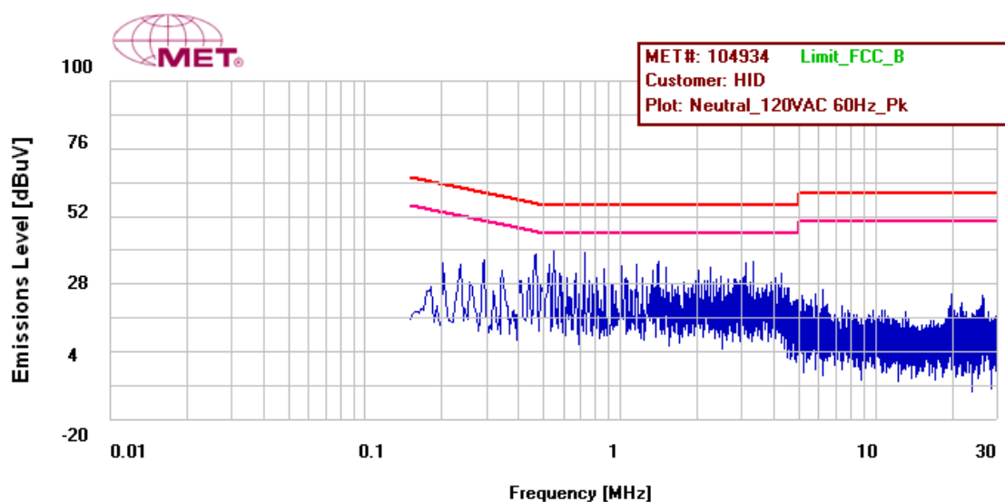
Figure 14: Conducted Emissions Limits, Pigtail, Neutral Line, Prescan
