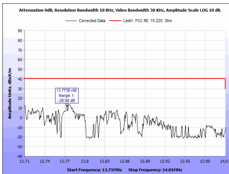
Figure 44: Spurious Emission Limits, within the bands 13.110 – 13.410 MHz and 13.710 – 14.010 MHz, Terminal, 13.710 MHz – 14.010 MHz, 0 Deg
