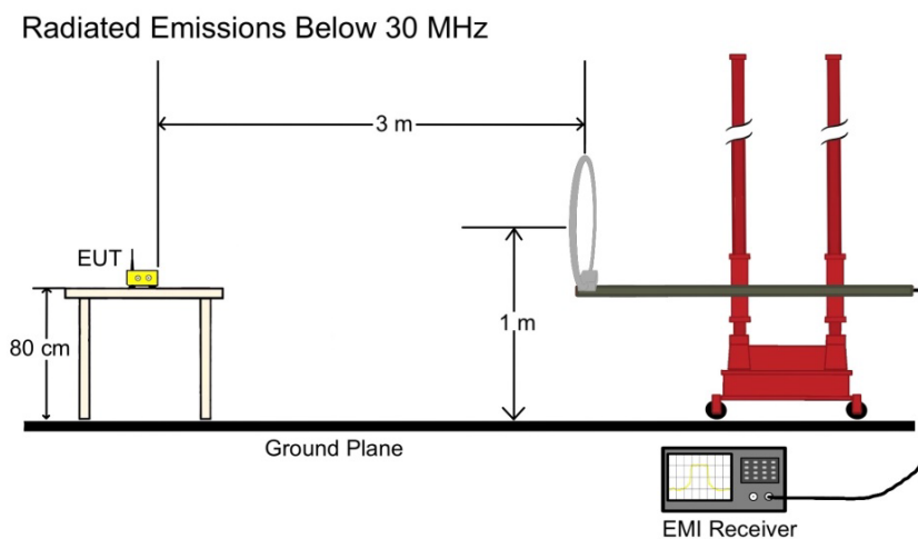
Figure 23: Radiated Emissions, Test Setup
