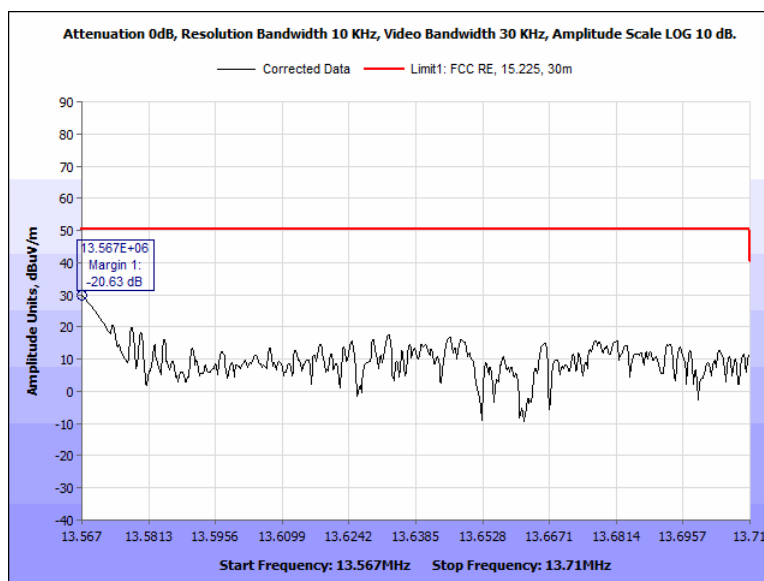
Figure 31: Spurious Emission Limits, within the bands 13.410 – 13.553 MHz and 13.567 – 13.710 MHz, Pigtail, 13.567 – 13.710 MHz, 0 Deg
