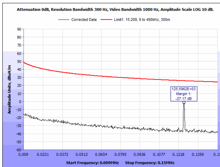
Figure 47: Spurious Emission Limits, outside the bands 13.110 – 14.010 MHz, Pigtail, 0.009 MHz – 0.150 MHz, 0 Deg
