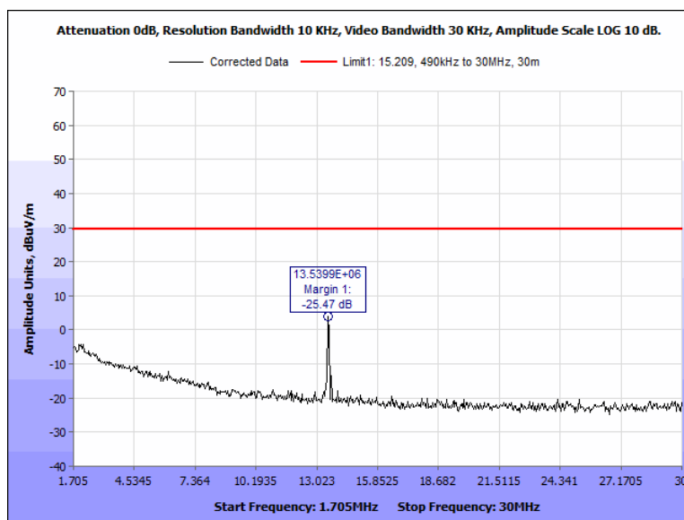
Figure 65: Spurious Emission Limits, outside the bands 13.110 – 14.010 MHz, Terminal, 1.705 MHz – 30 MHz, 90 Deg
