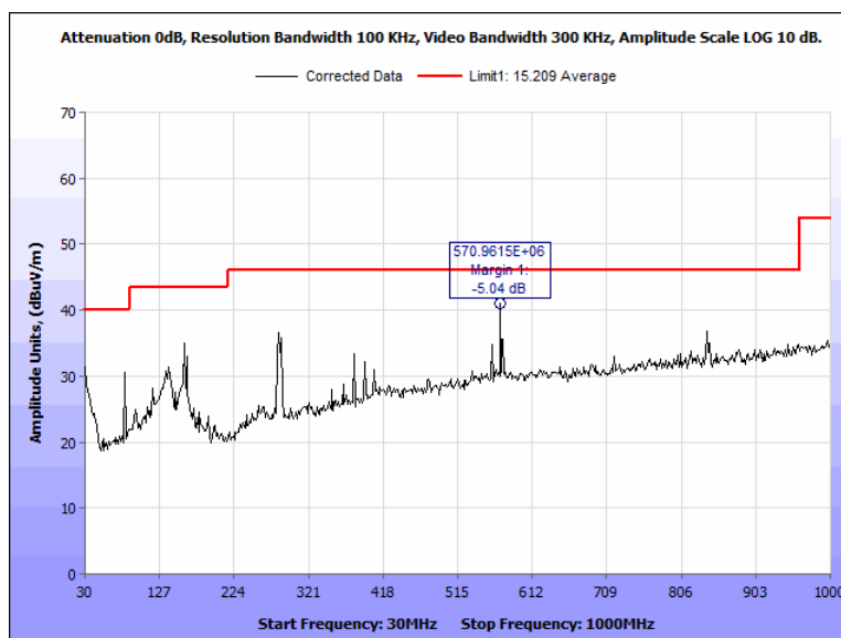
Figure 56: Spurious Emission Limits, outside the bands 13.110 – 14.010 MHz, Pigtail, 30 MHz – 1000 MHz, Vertical
