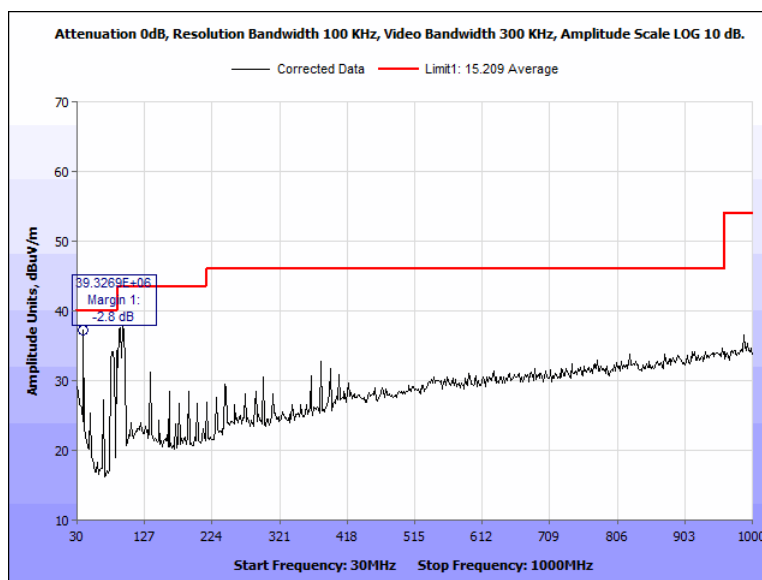
Figure 67: Spurious Emission Limits, outside the bands 13.110 – 14.010 MHz, Terminal, 30 MHz – 1000 MHz, Vertical
