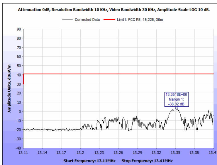
Figure 43: Spurious Emission Limits, within the bands 13.110 – 13.410 MHz and 13.710 – 14.010 MHz, Terminal, 13.110 MHz – 13.410 MHz, 90 Deg
