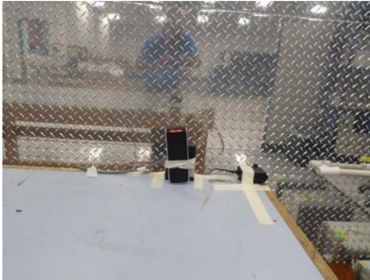
Figure 1: Conducted Emissions Limits, Pigtail, EUT Front View
