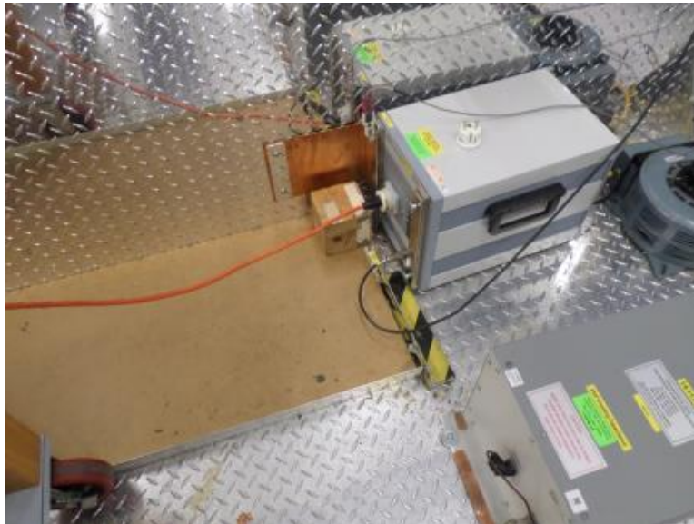
Figure 4: Conducted Emissions Limits, Pigtail, LISN View, Test Setup
