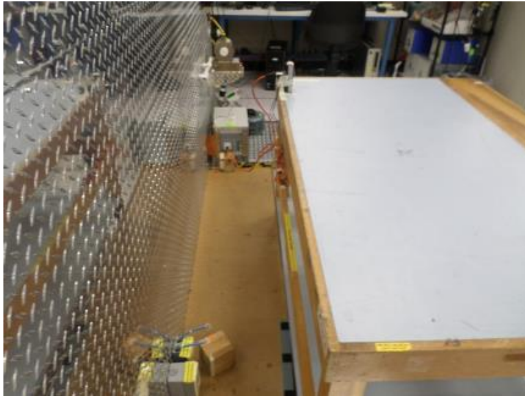
Figure 5: Conducted Emissions Limits, Terminal, Back View, Test Setup
