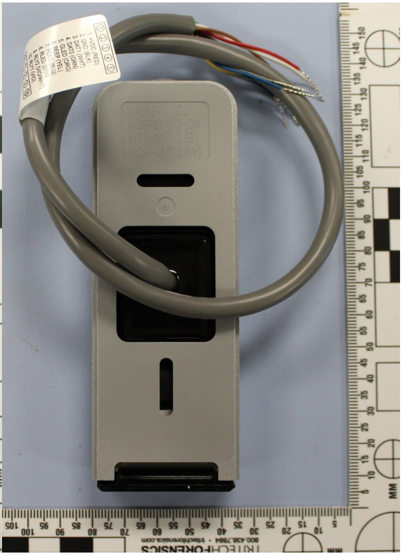
Model 20 (pigtail version) rear side
