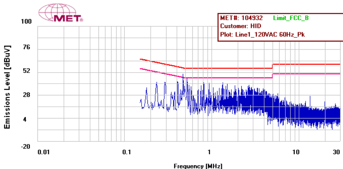
Figure 11: Conducted Emission Limits, Pigtail, Phase Line, Prescan
