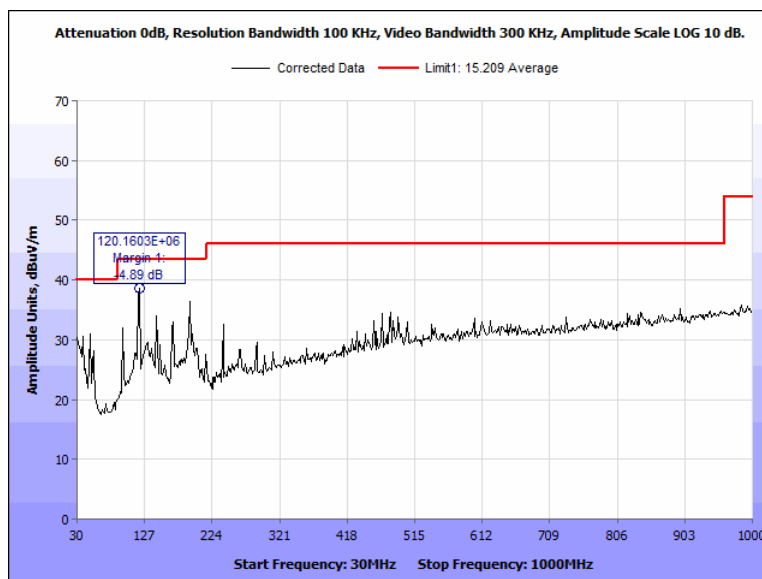
Figure 88: Radiated Spurious Emissions, Terminal, 2402 MHz, 30 MHz – 1000 MHz, Horizontal
