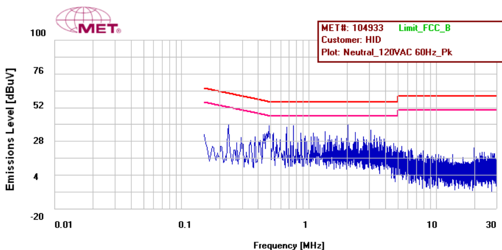
Figure 32: Conducted Emissions Limits, Terminal, Neutral Line, Prescan
