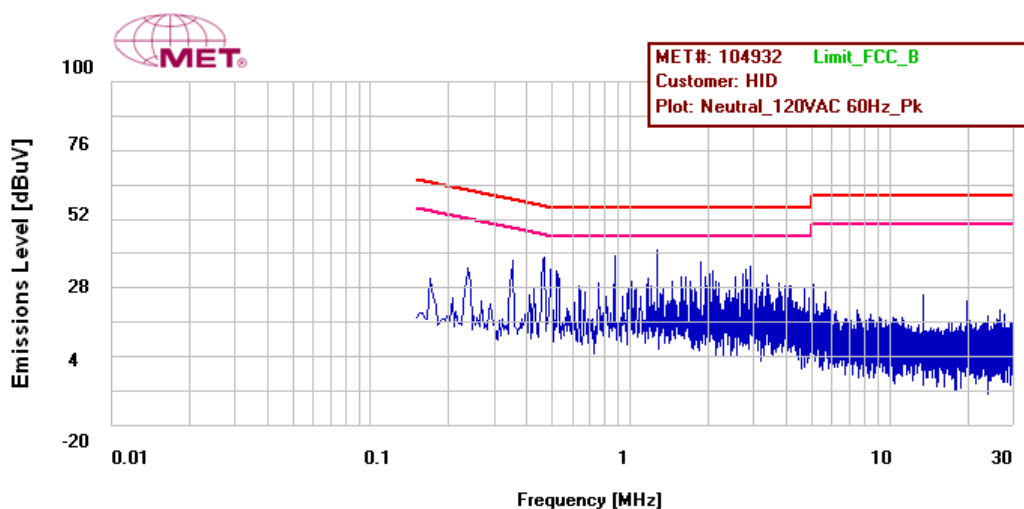
Figure 28: Conducted Emission Limits, Pigtail, Neutral Line, Prescan
