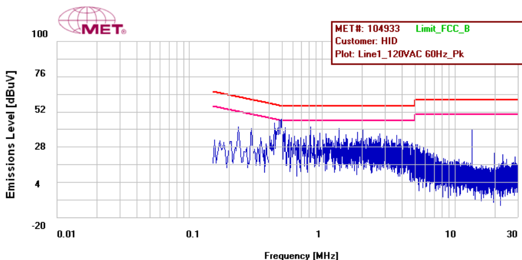
Figure 30: Conducted Emissions Limits, Terminal, Phase Line, Prescan
