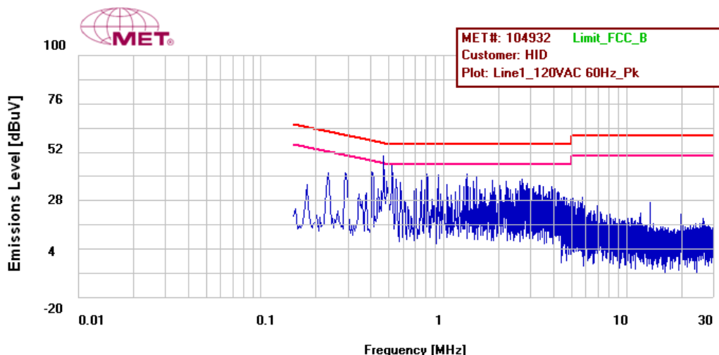
Figure 26: Conducted Emission Limits, Pigtail, Phase Line, Prescan
