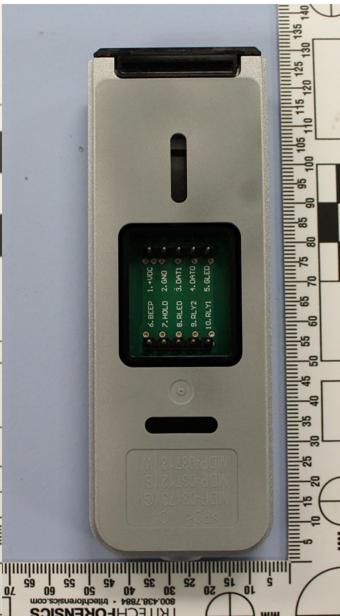
Model 20 (terminal version) rear side
