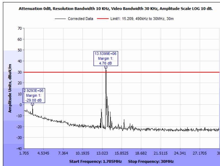
Figure 53: Spurious Emission Limits, outside the bands 13.110 – 14.010 MHz, Pigtail, 1.705 MHz – 30 MHz, 0 Deg
