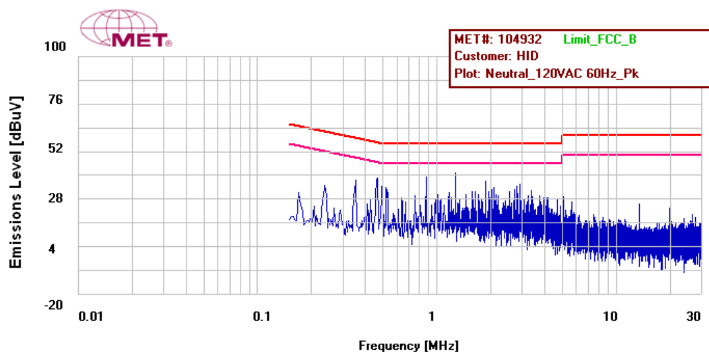
Figure 14: Conducted Emission Limits, Pigtail, Neutral Line, Prescan
