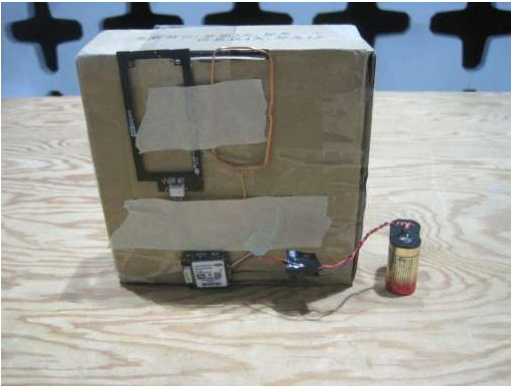
Radiated Emission Test Setup – Zoom in View
