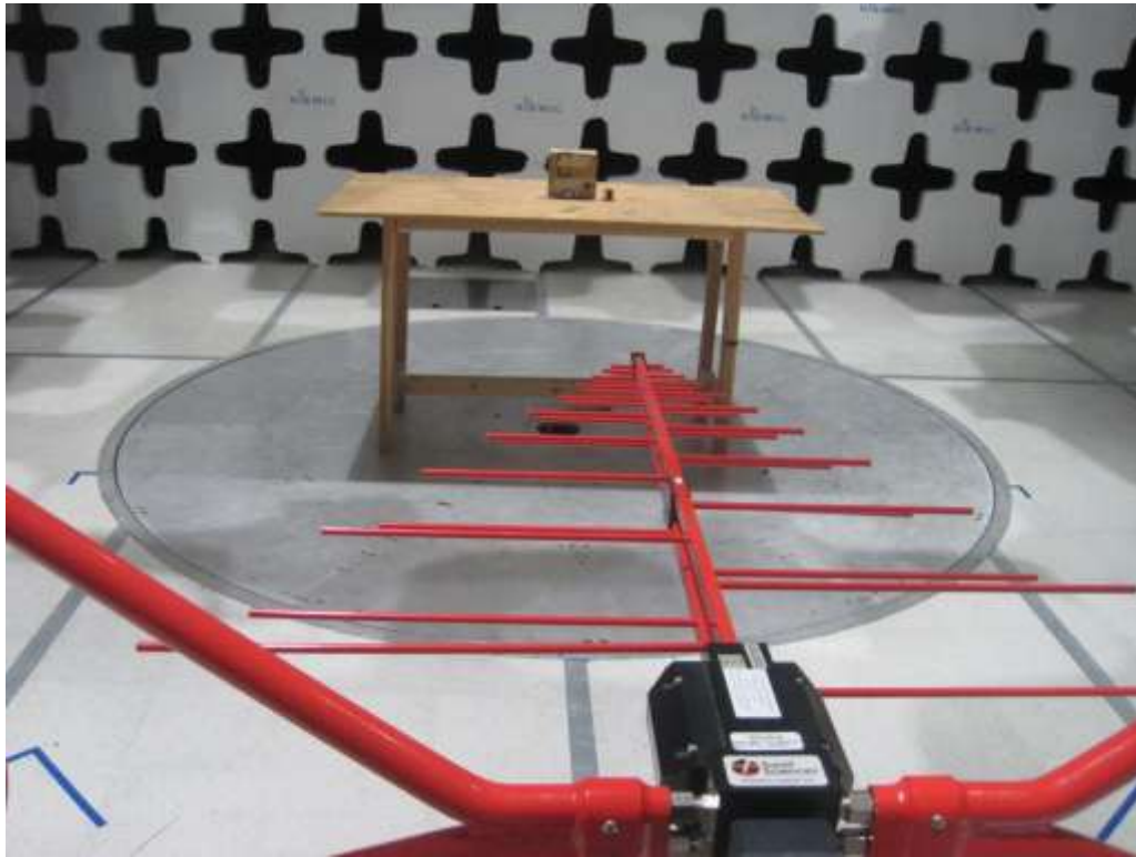
Radiated Emission>30MHz Test Setup – Front View
