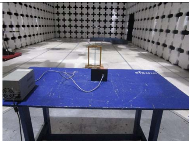
Radiated Emissions (<30MHz) - Rear View
