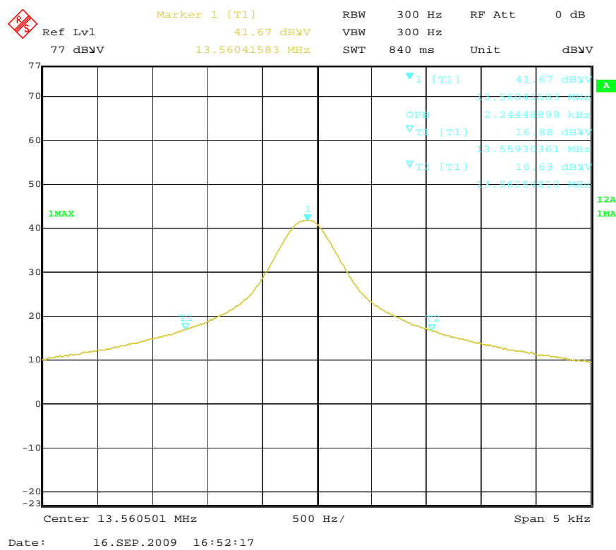
Plots: 13.56 MHz
