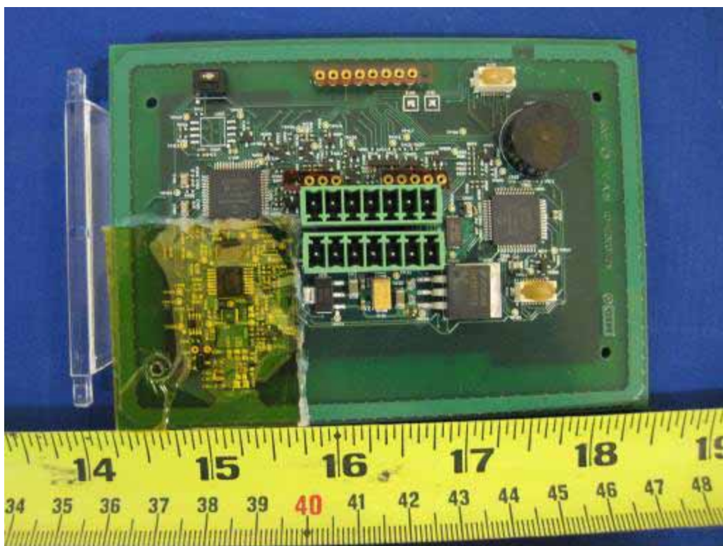
13.56MHz RDID radio board – Bottom
