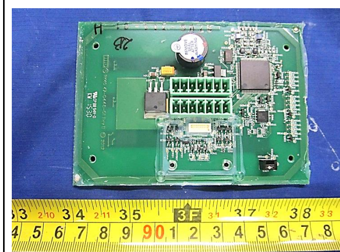
PCBA 1 Top View 1 without PCBA2
