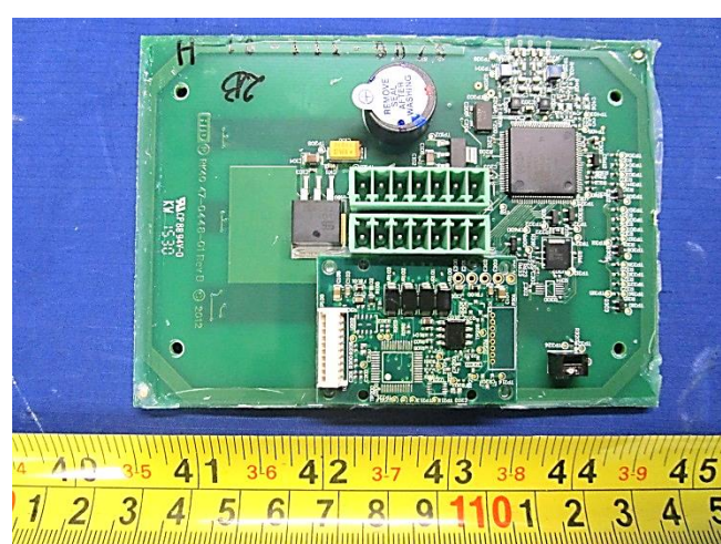
PCBA 1 Top View 2 with PCBA2
